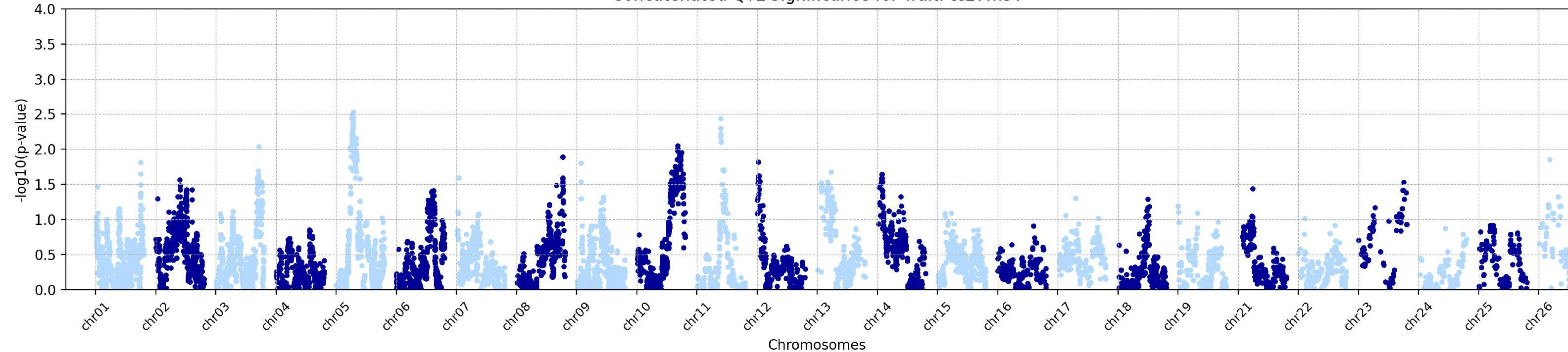
Concatenated QTL Significance for Trait: tc27m3T
