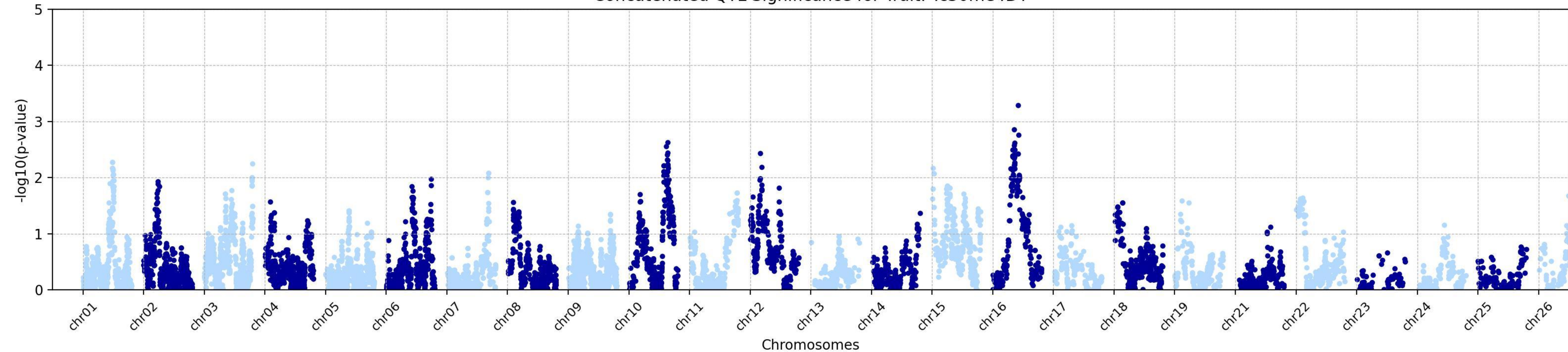
Concatenated QTL Significance for Trait: Tc30me4DT
