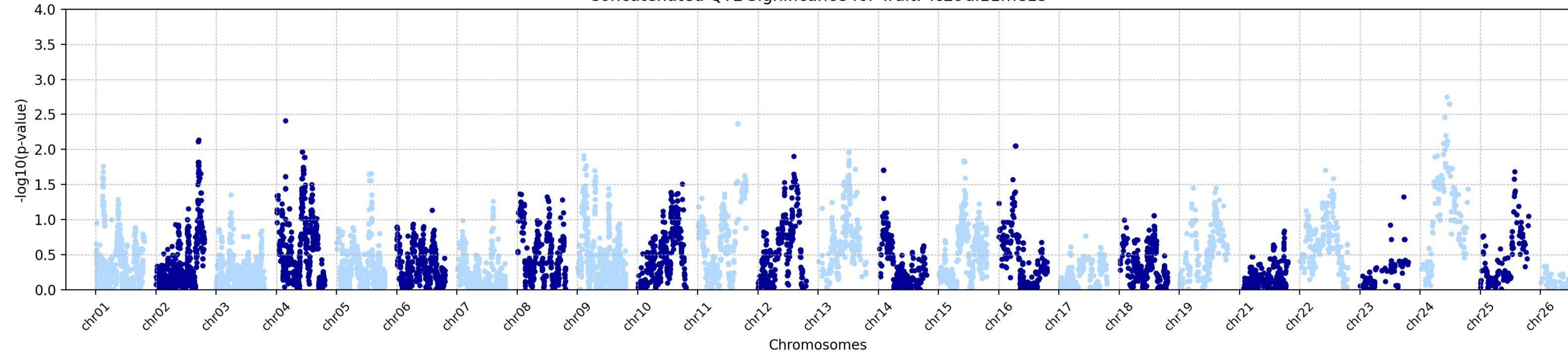
Concatenated QTL Significance for Trait: Tc29di11me15
