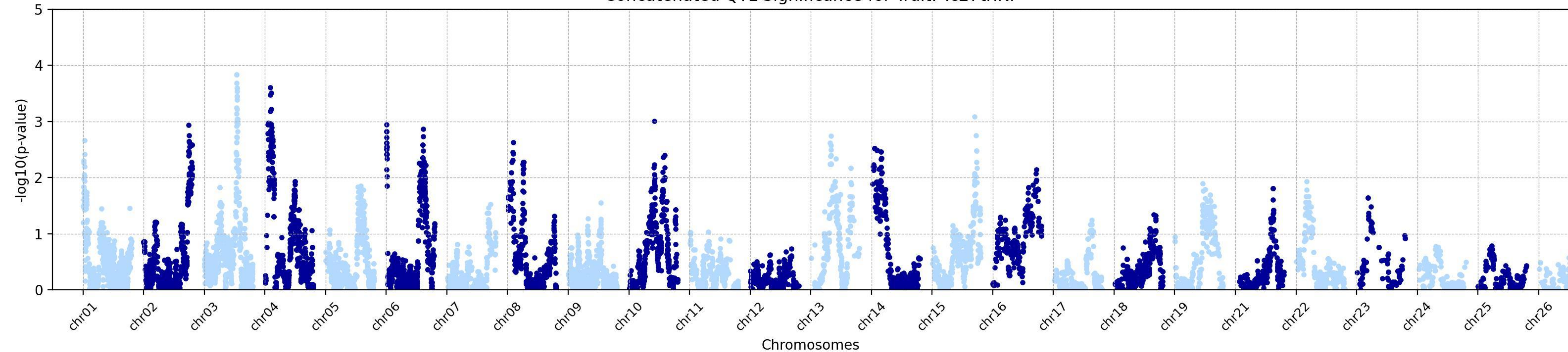
Concatenated QTL Significance for Trait: Tc27triKT
