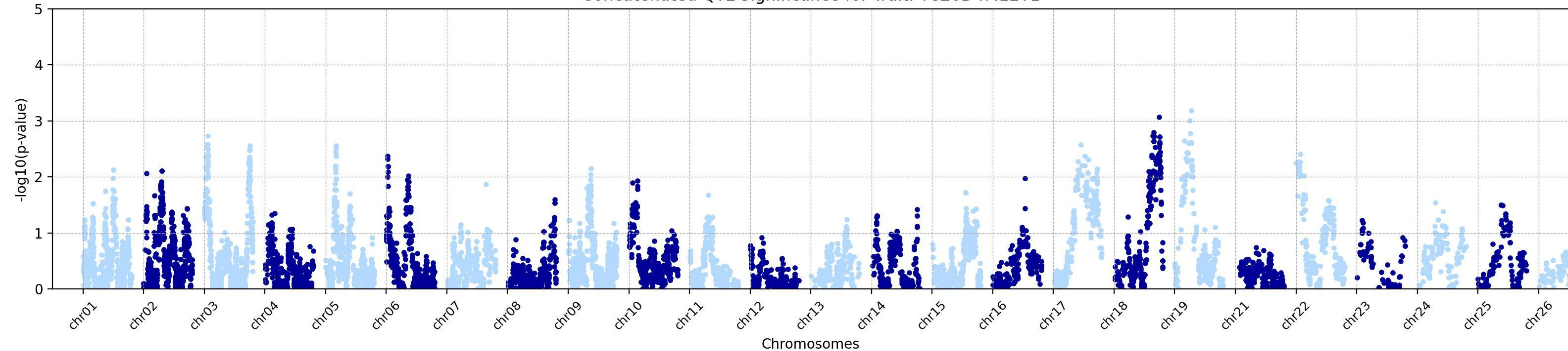
Concatenated QTL Significance for Trait: TC26D4M12T1
