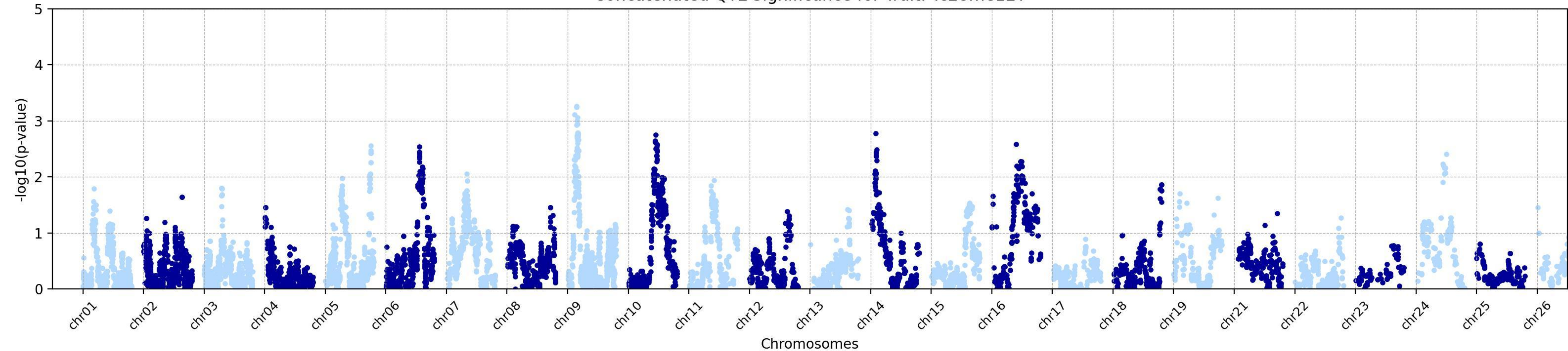
Concatenated QTL Significance for Trait: Tc28me12T
