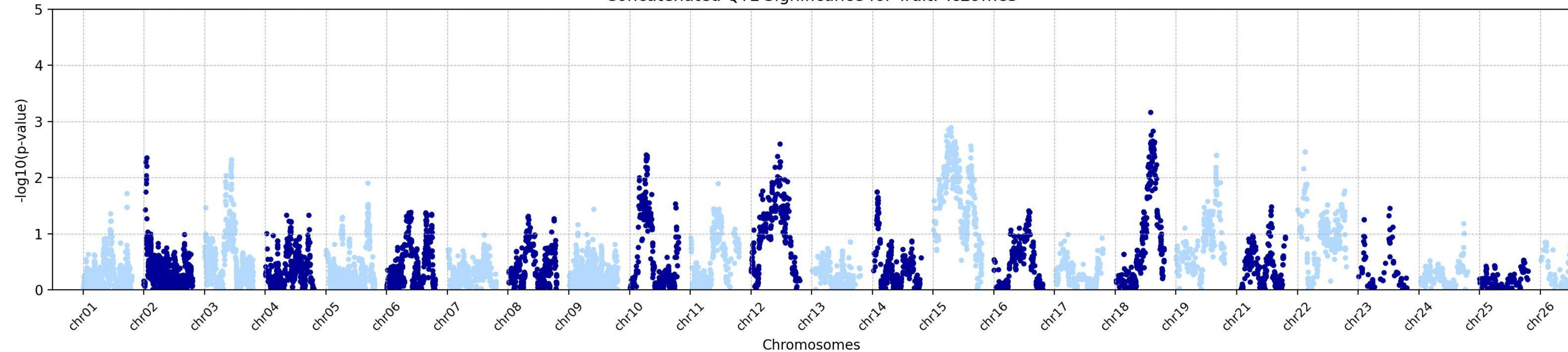
Concatenated QTL Significance for Trait: Tc29me3
