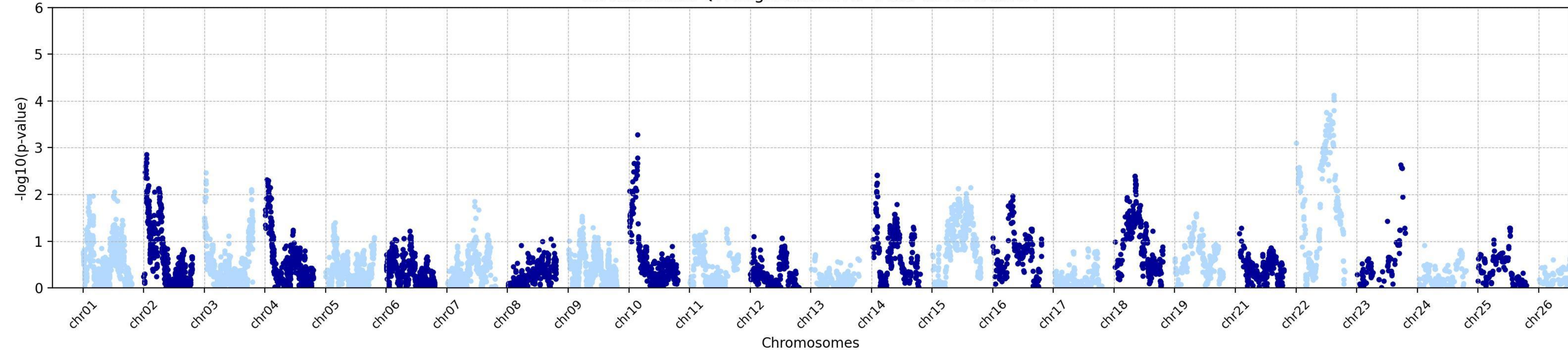
Concatenated QTL Significance for Trait: Tc31t711m15T
