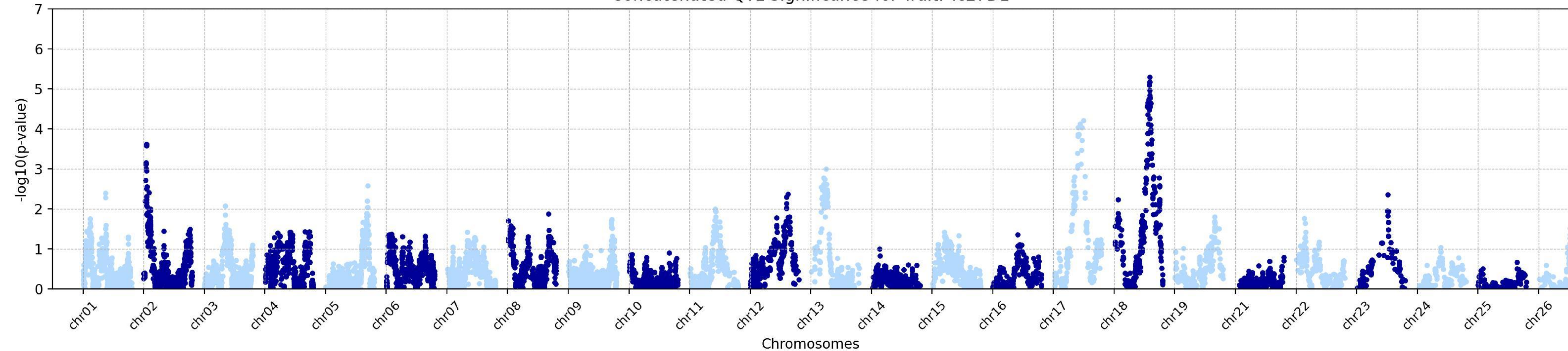
Concatenated QTL Significance for Trait: Tc27D1
