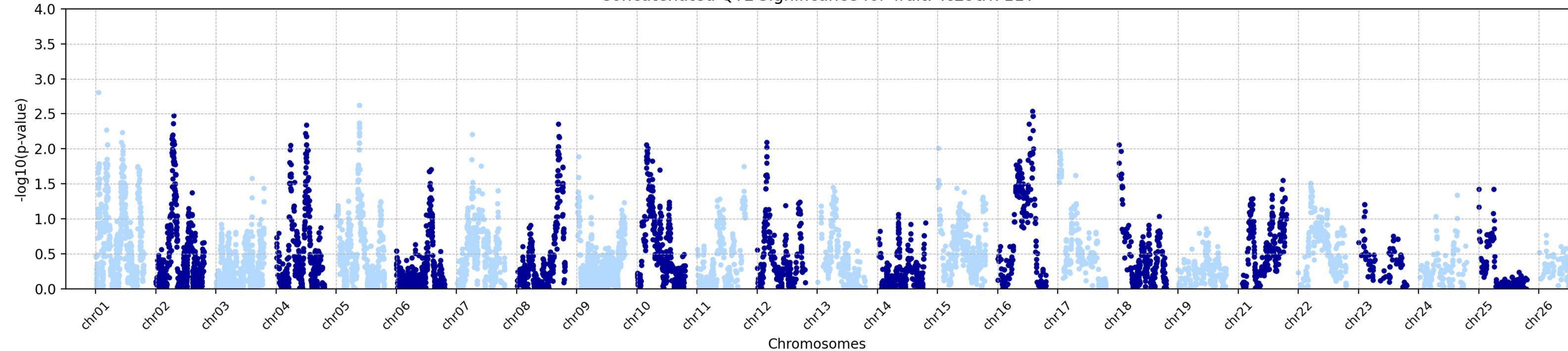
Concatenated QTL Significance for Trait: Tc29tri711T
