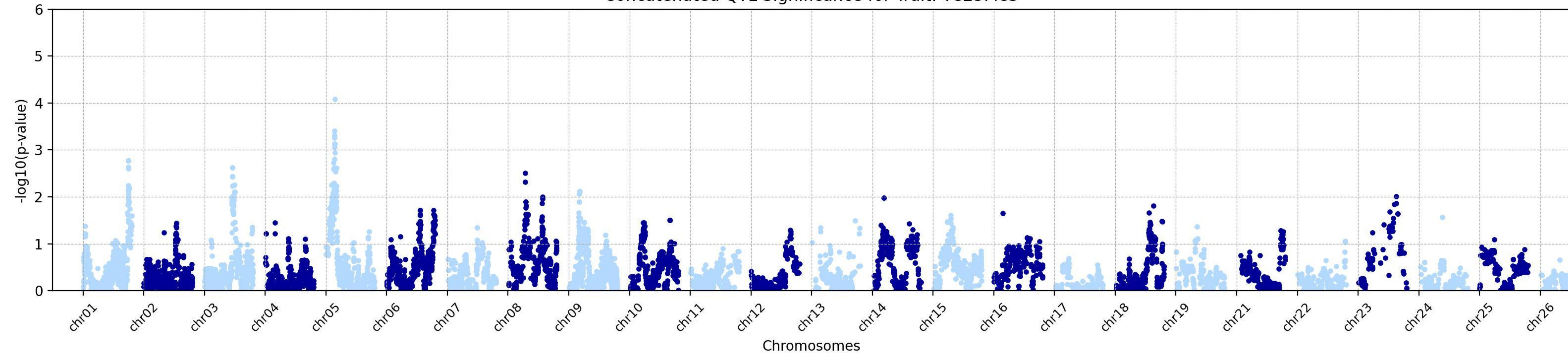
Concatenated QTL Significance for Trait: TC25Me3
