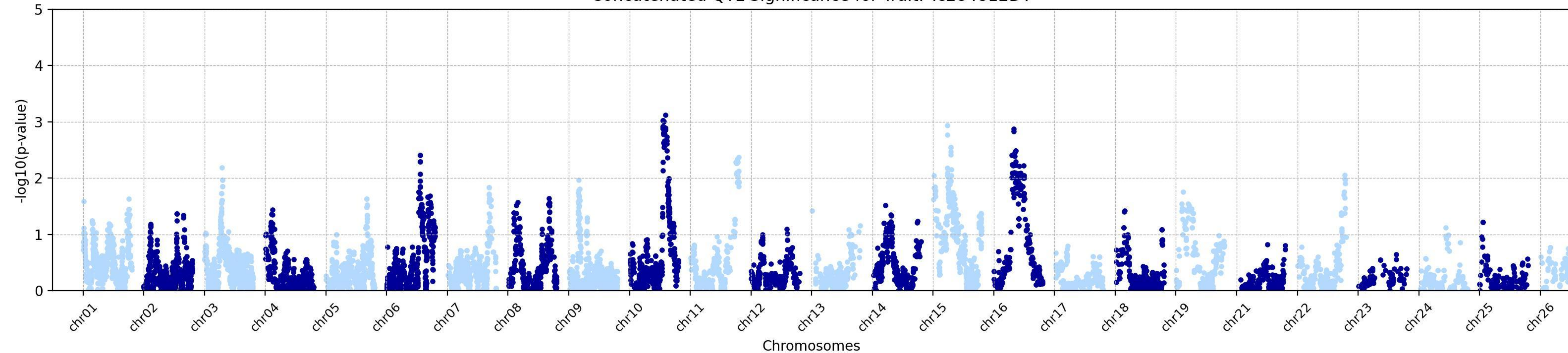
Concatenated QTL Significance for Trait: Tc284812DT
