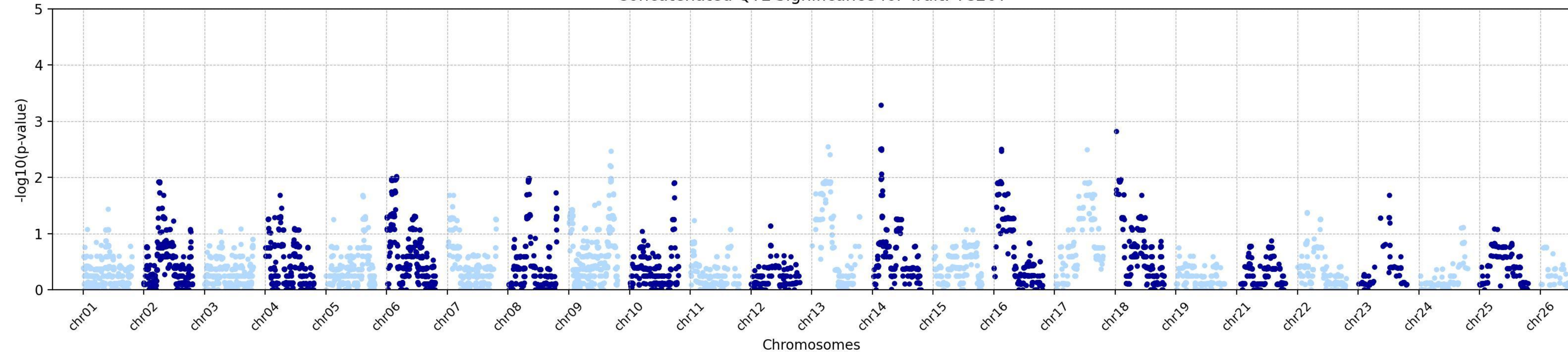
Concatenated QTL Significance for Trait: TC26T
