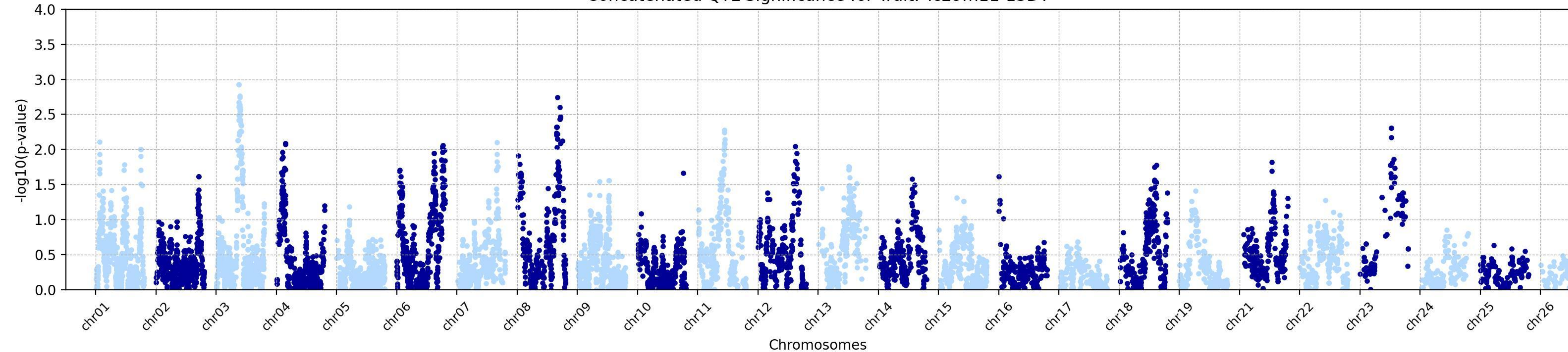
Concatenated QTL Significance for Trait: Tc29m11-13DT
