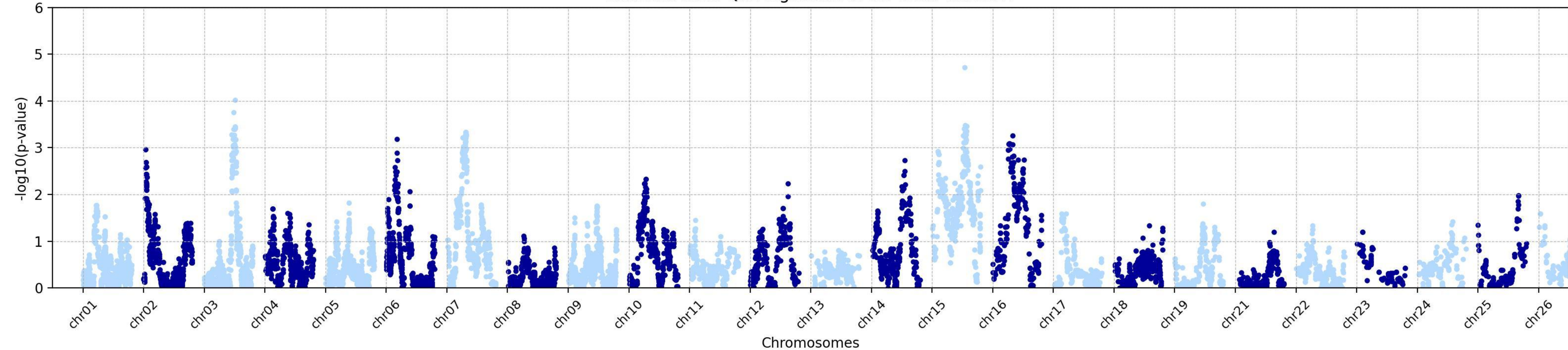
Concatenated QTL Significance for Trait: TotalD1T
