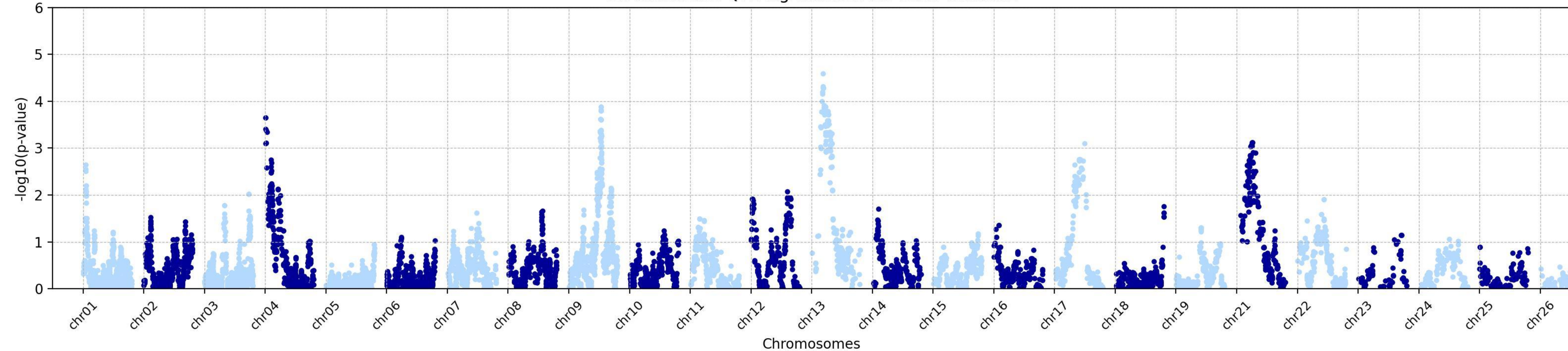
Concatenated QTL Significance for Trait: Tc30me2
