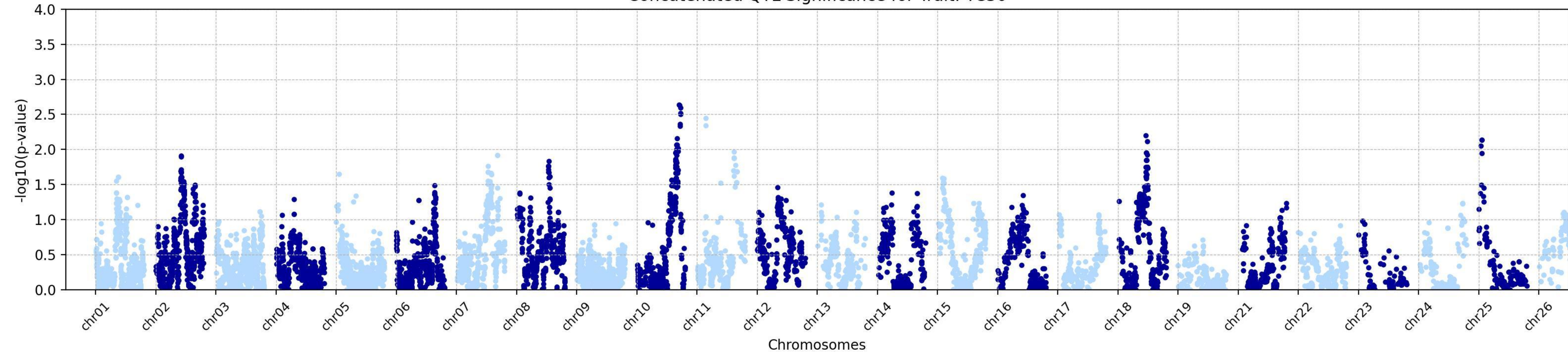
Concatenated QTL Significance for Trait: TC30
