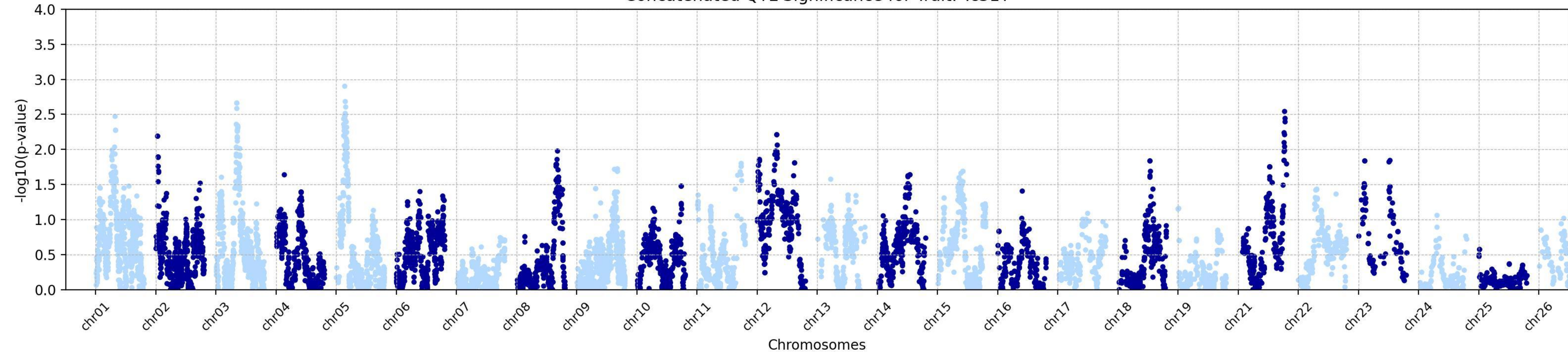
Concatenated QTL Significance for Trait: Tc31T
