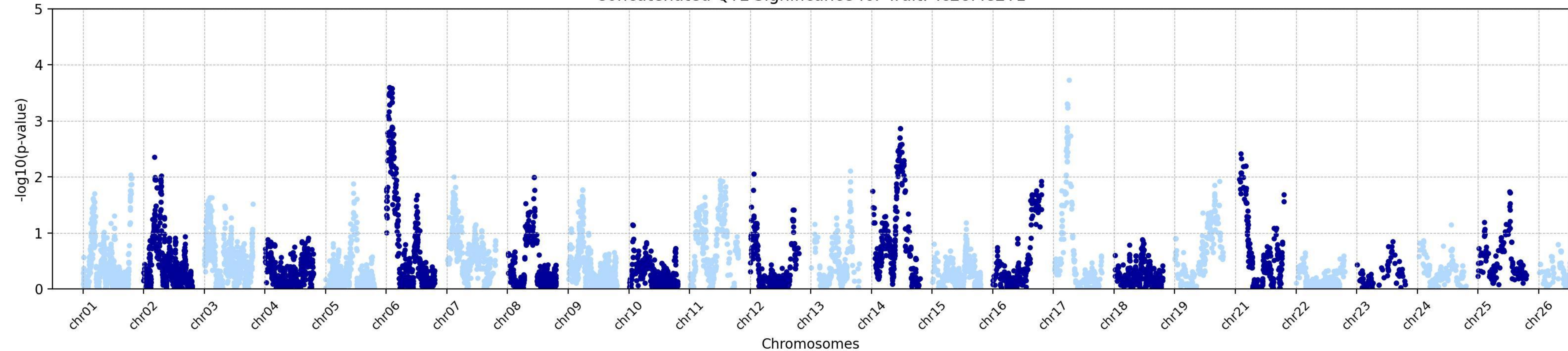
Concatenated QTL Significance for Trait: Tc28Me2T1
