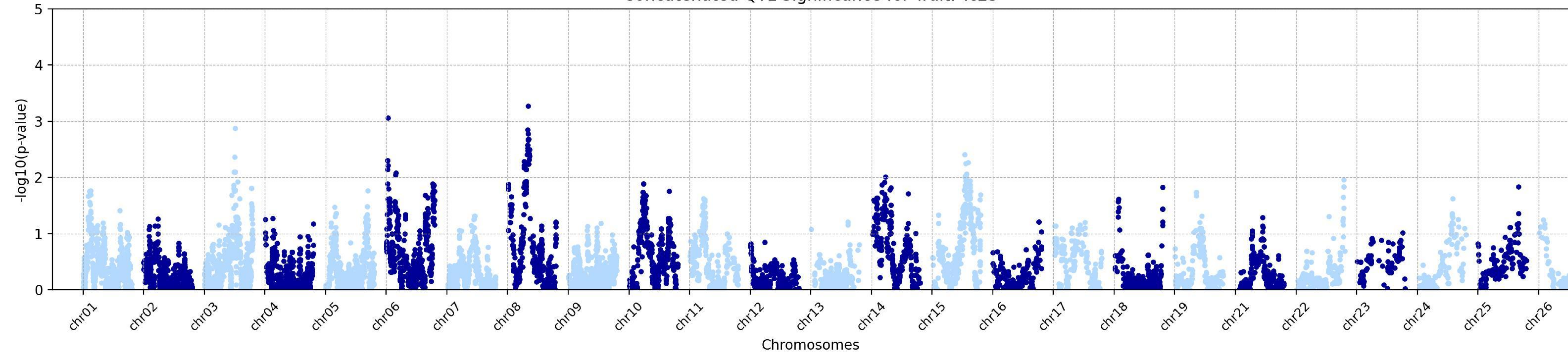
Concatenated QTL Significance for Trait: Tc25
