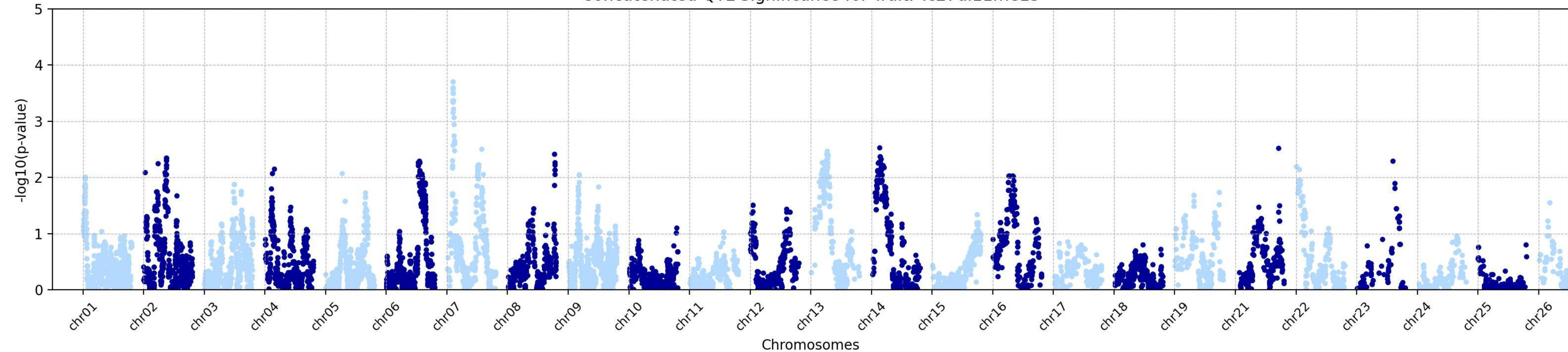
Concatenated QTL Significance for Trait: Tc27di11me15
