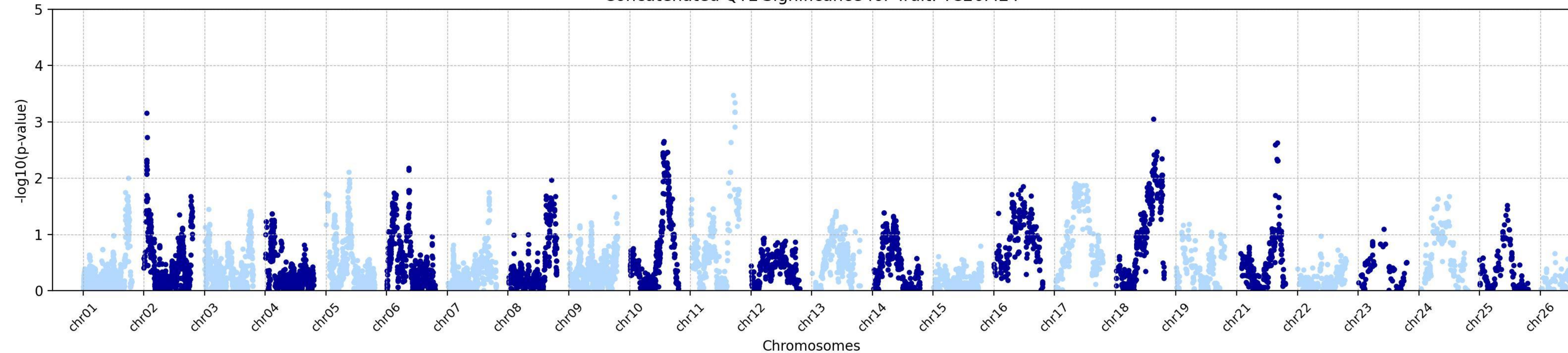
Concatenated QTL Significance for Trait: TC26ME4
