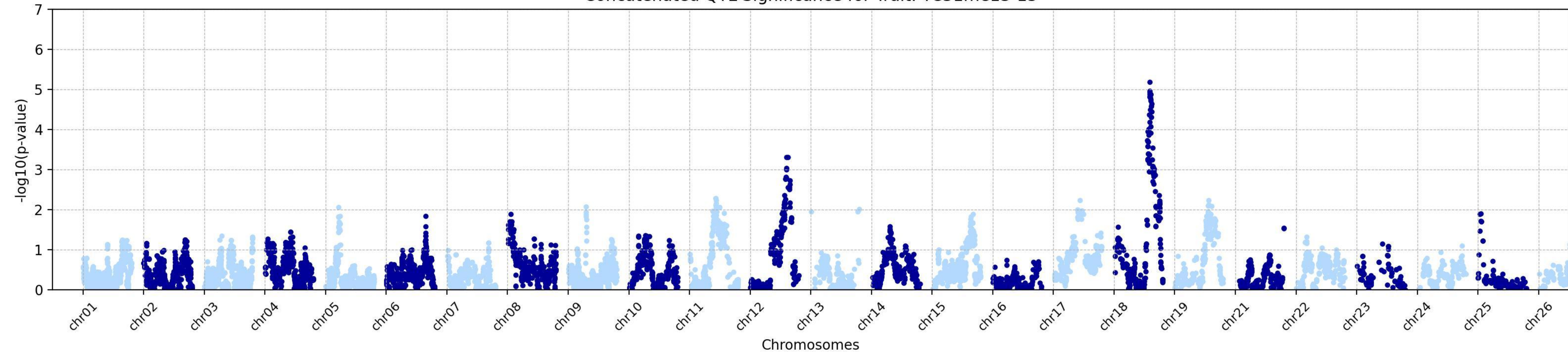
Concatenated QTL Significance for Trait: TC31me13-15
