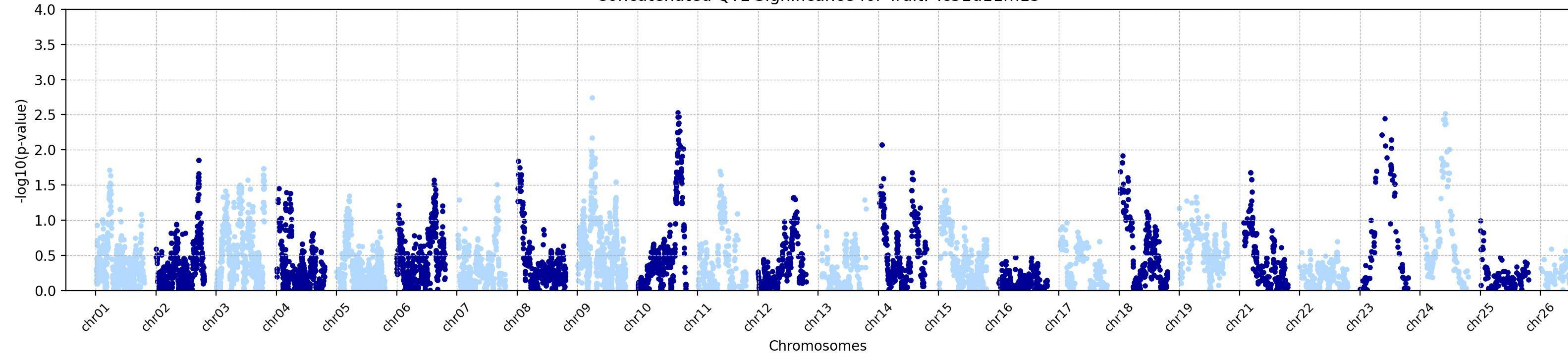
Concatenated QTL Significance for Trait: Tc31d11m15
