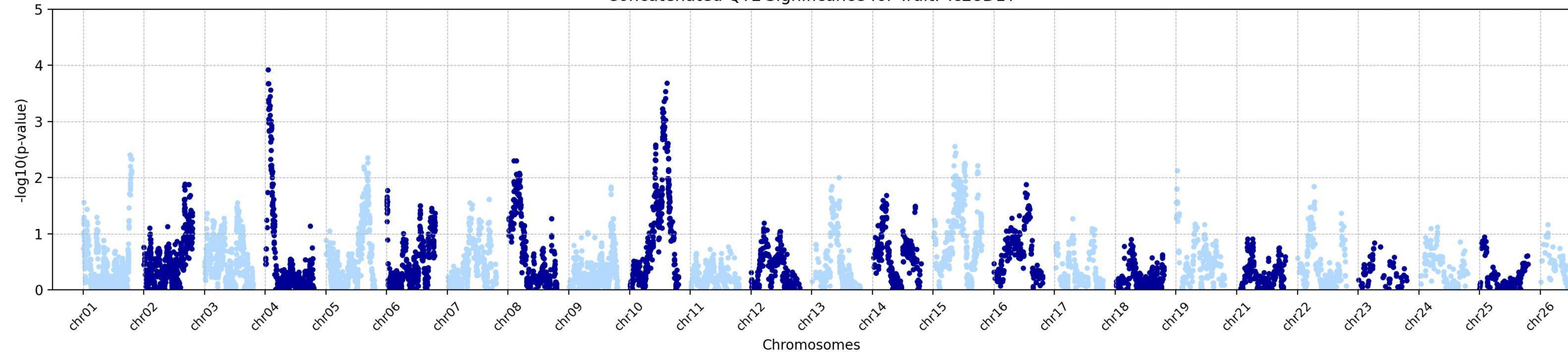
Concatenated QTL Significance for Trait: Tc28D1T
