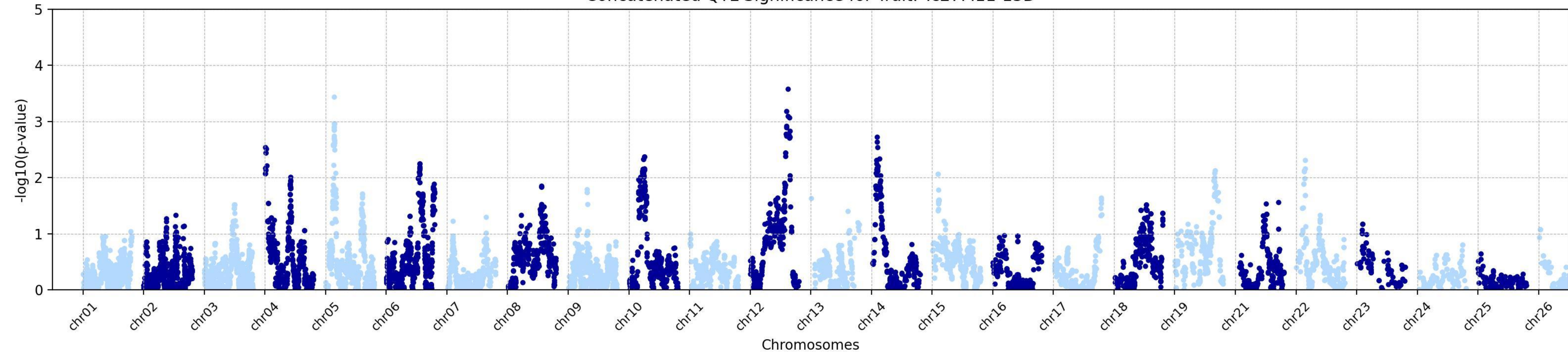
Concatenated QTL Significance for Trait: Tc27M11-13D
