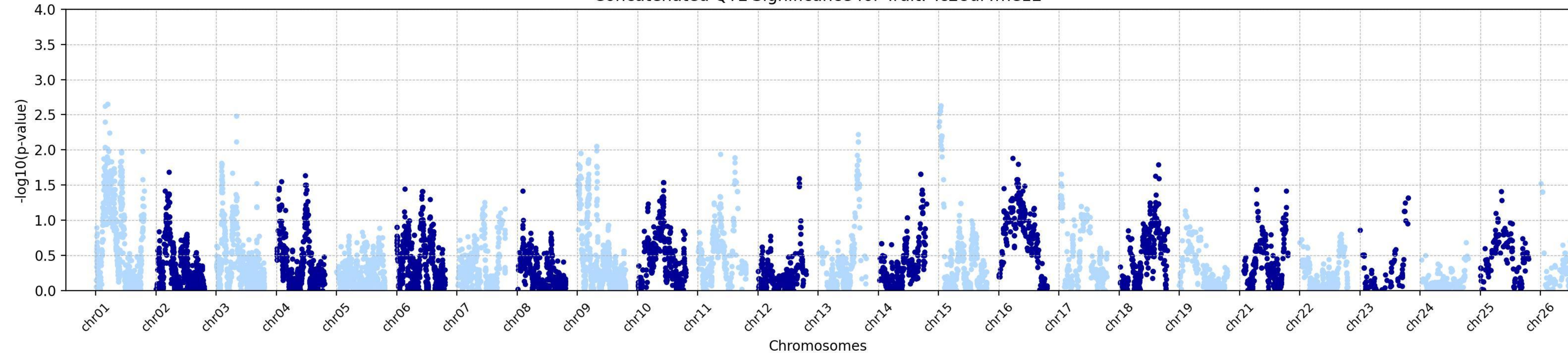
Concatenated QTL Significance for Trait: Tc28di4me12
