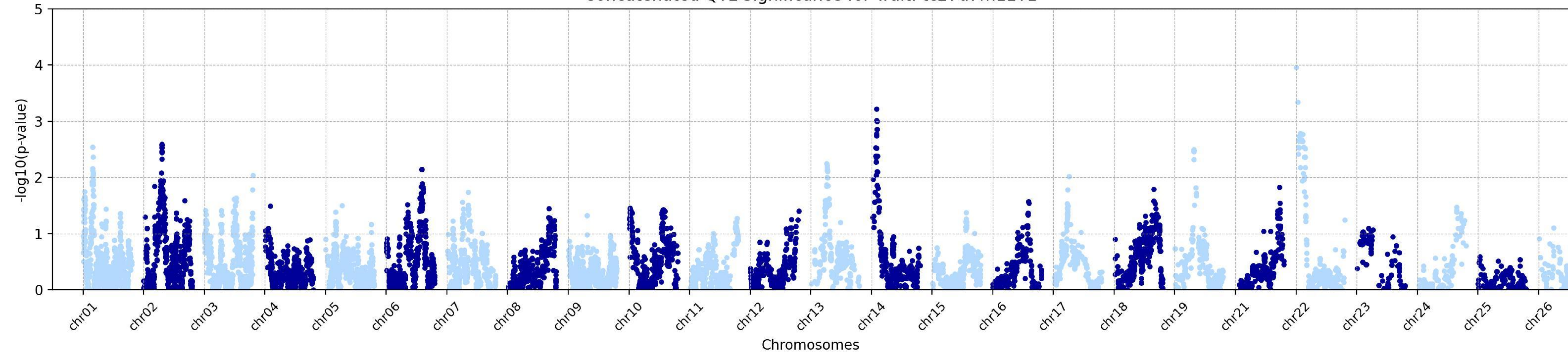
Concatenated QTL Significance for Trait: tc27d7m11T1
