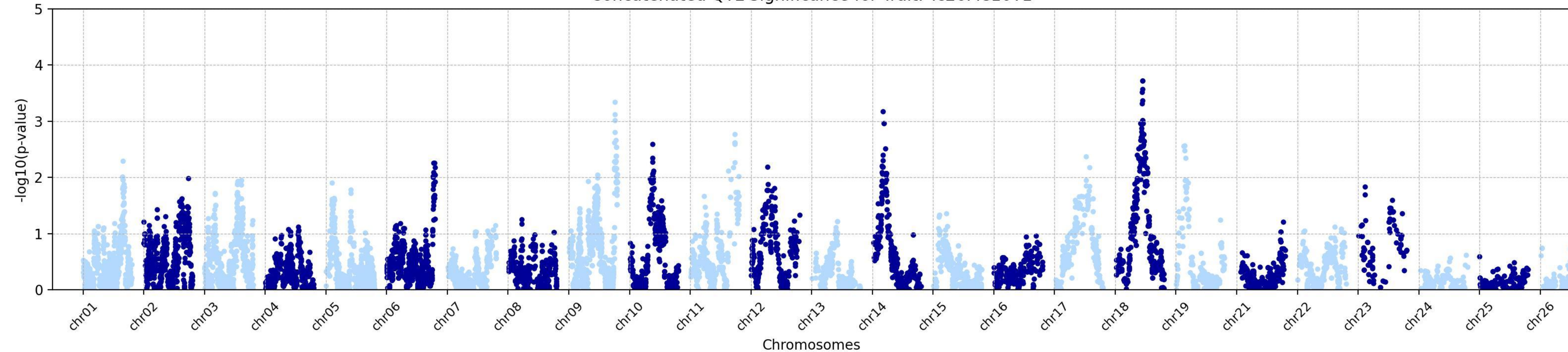
Concatenated QTL Significance for Trait: Tc26Me10T1
