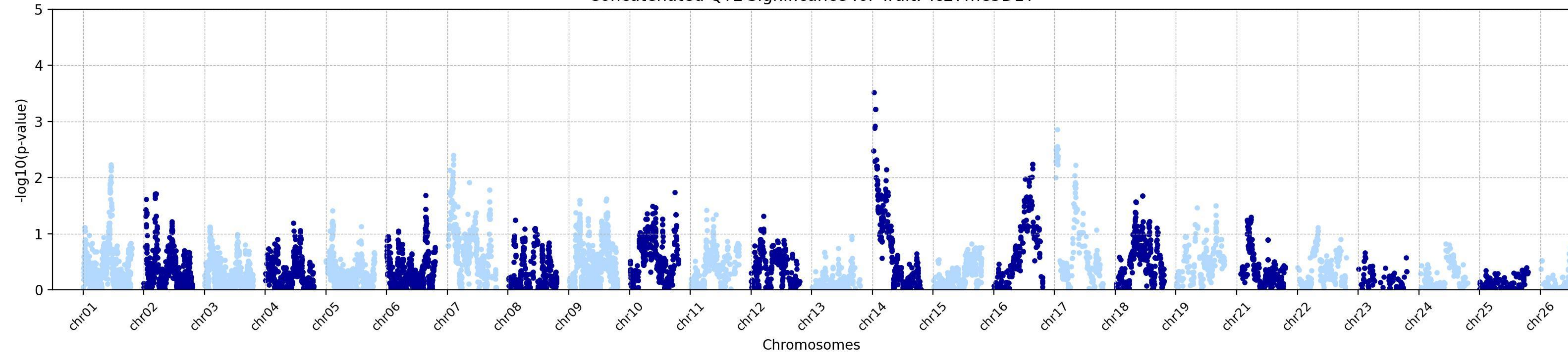
Concatenated QTL Significance for Trait: Tc27me5D1T
