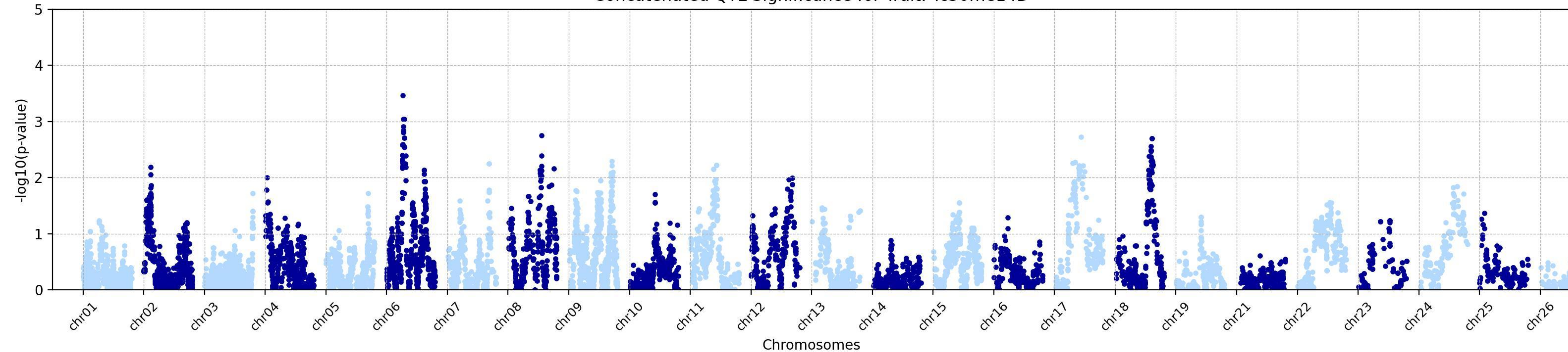
Concatenated QTL Significance for Trait: Tc30me14D
