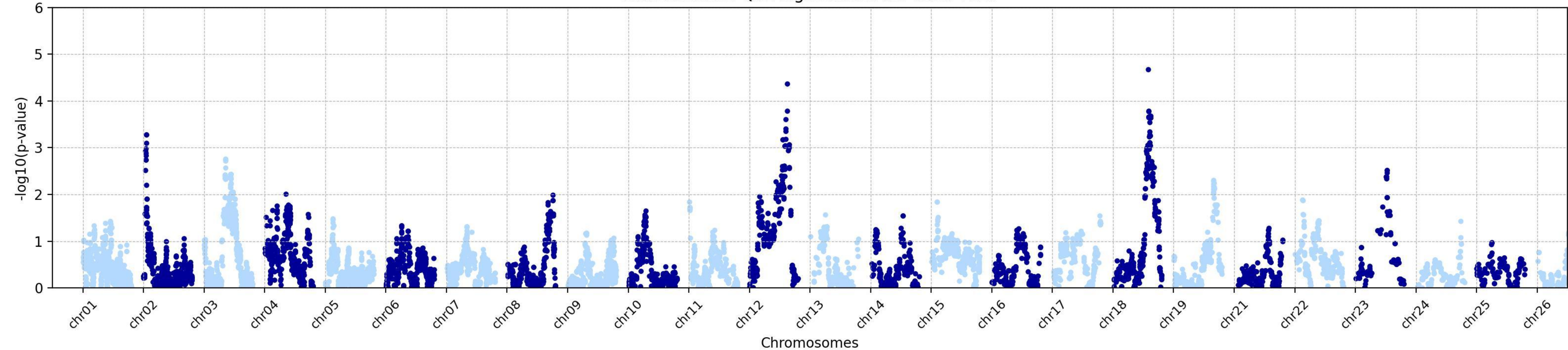
Concatenated QTL Significance for Trait: TC29
