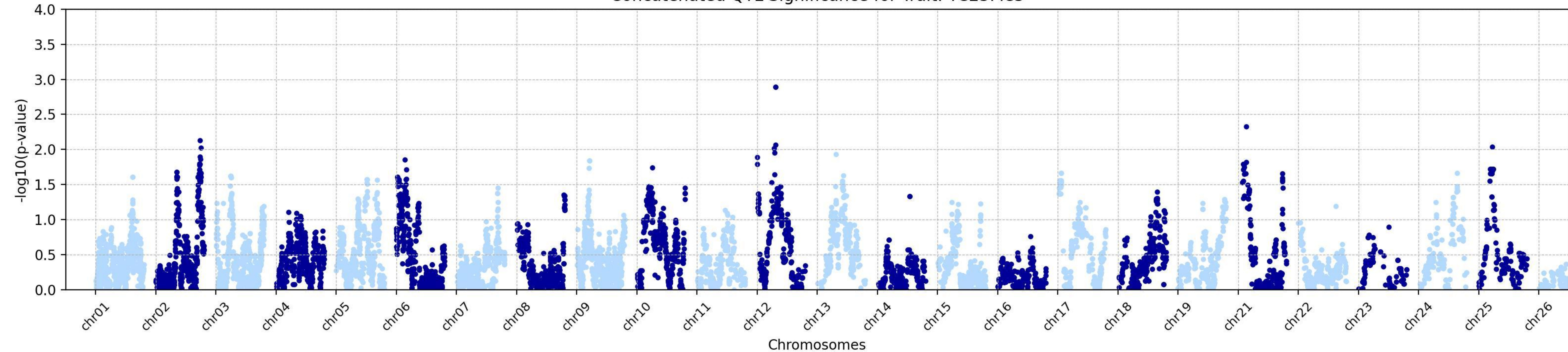
Concatenated QTL Significance for Trait: TC25Me5
