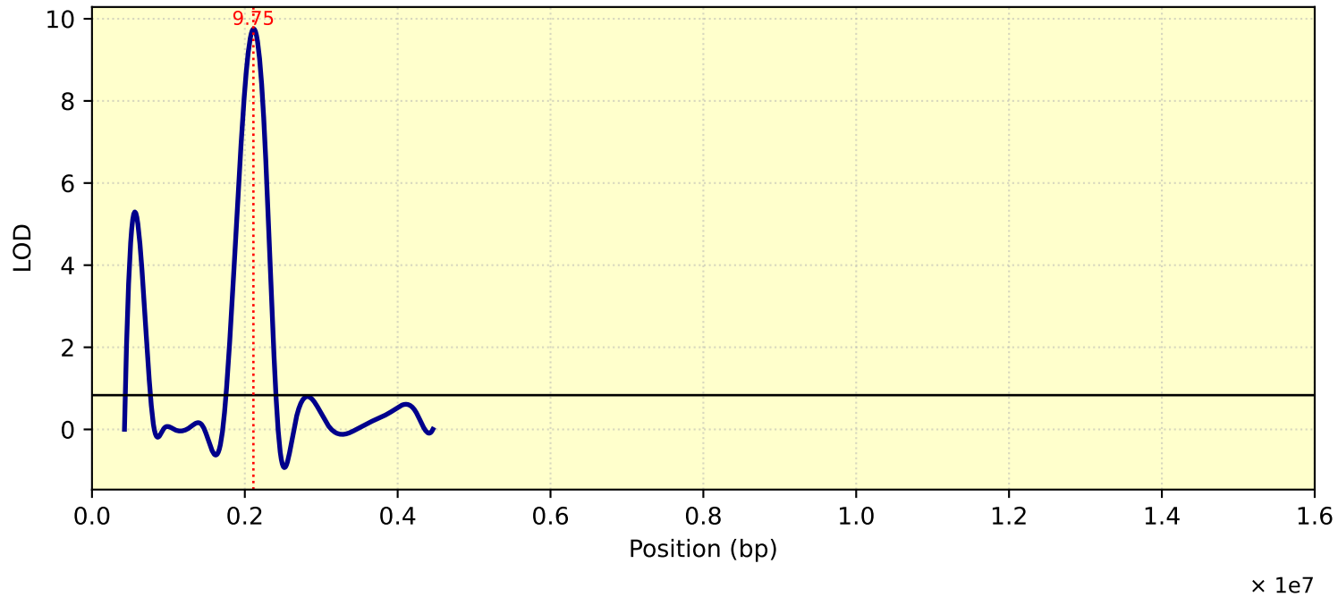
LOD Curve - chr22 - TC26ME4
