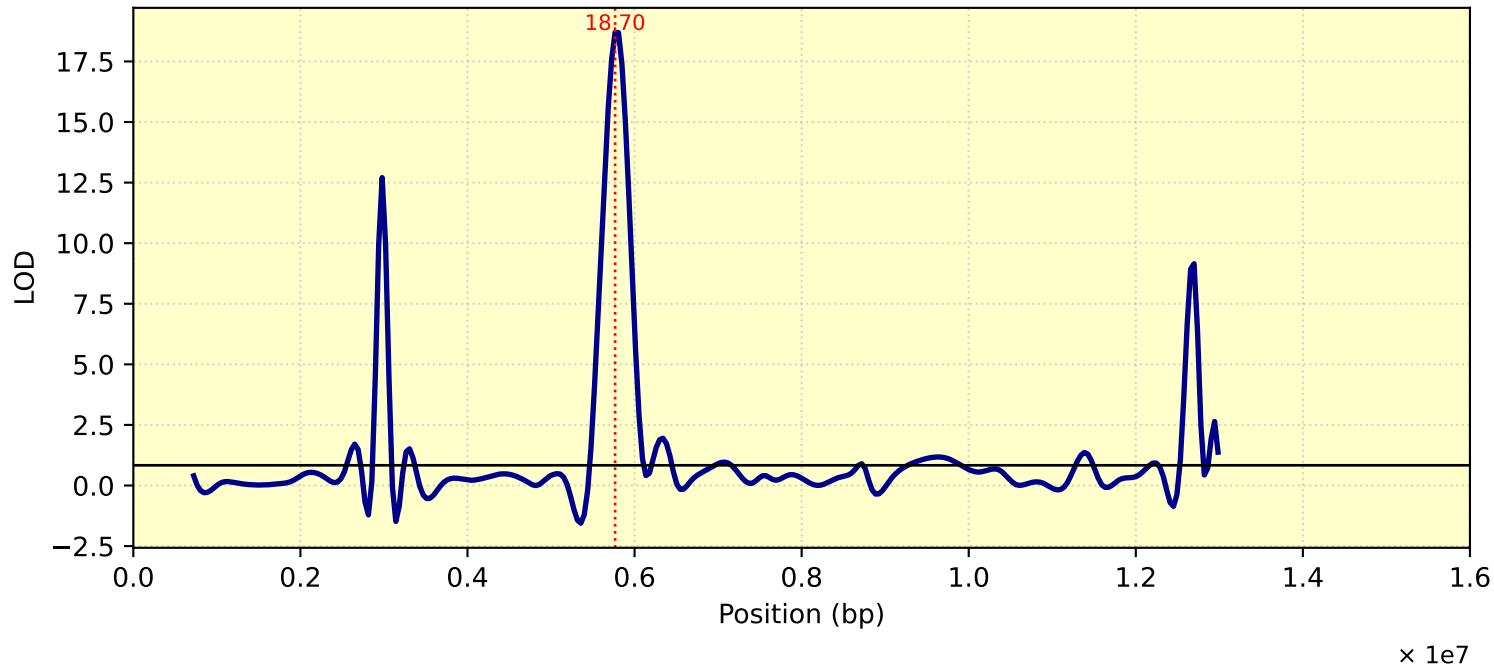
LOD Curve - chr09 - TC26ME4
