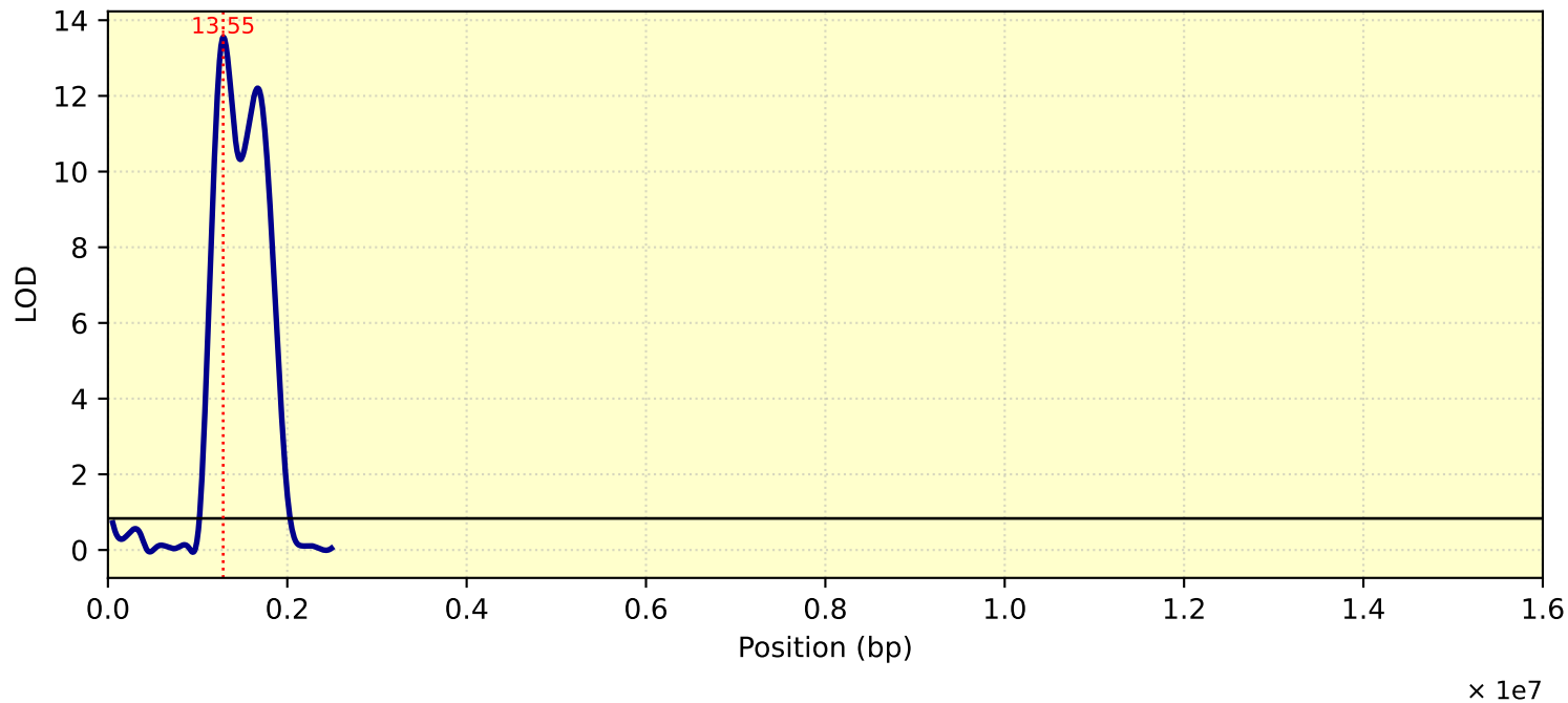
LOD Curve - chr25 - TC26ME4
