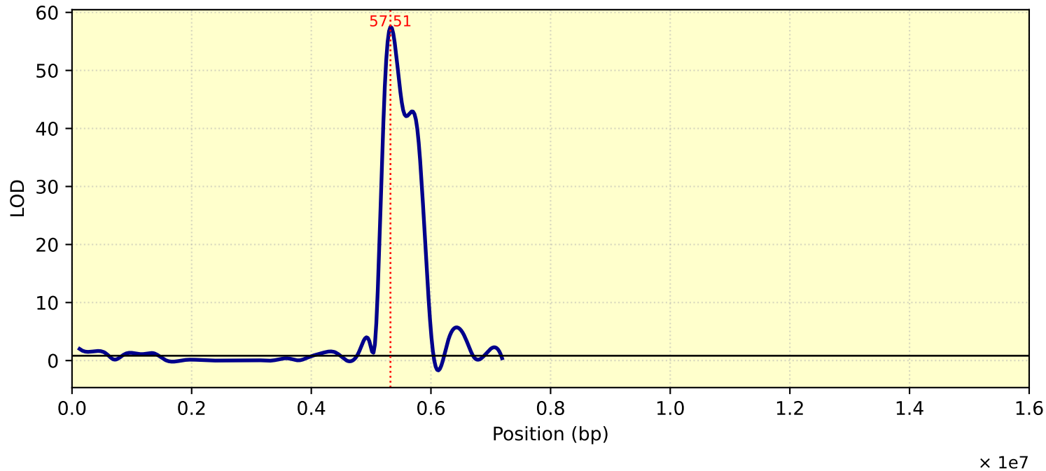
LOD Curve - chr10 - TC26ME4
