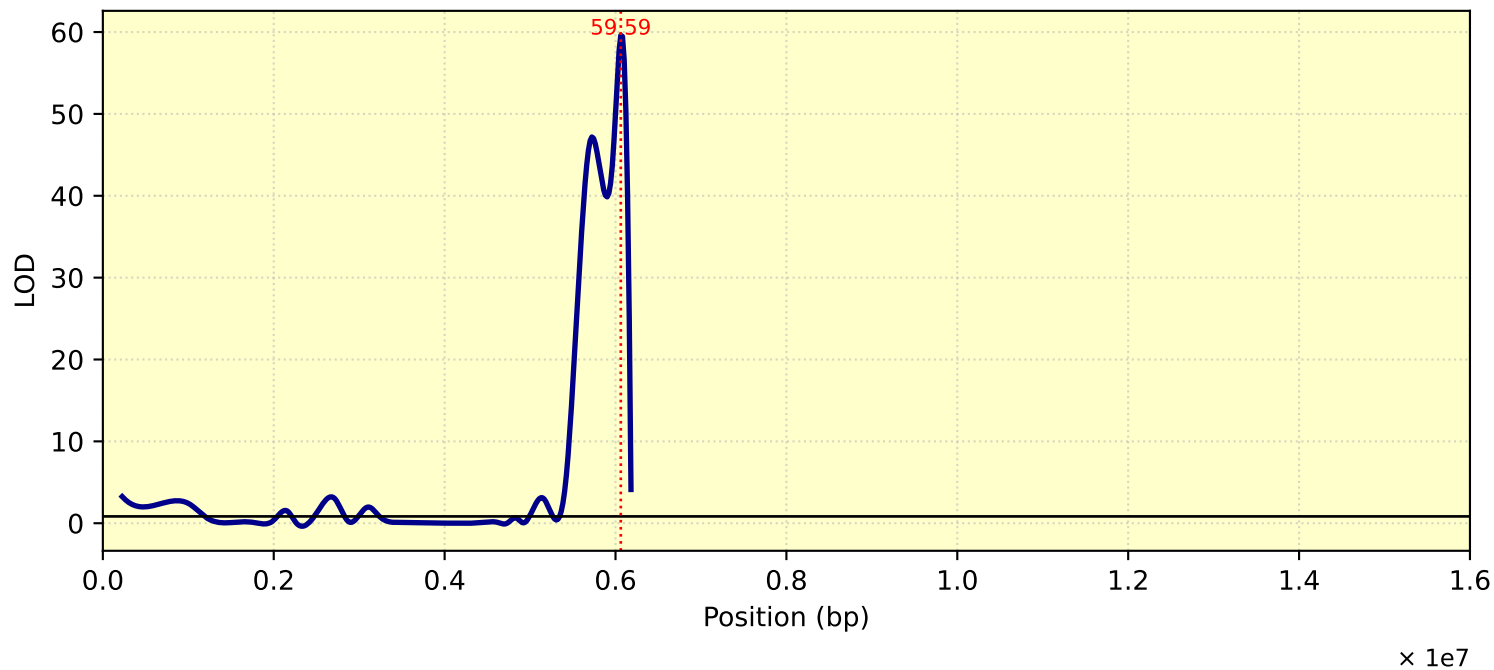
LOD Curve - chr11 - TC26ME4
