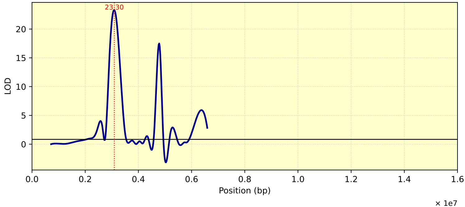
LOD Curve - chr13 - TC26ME4
