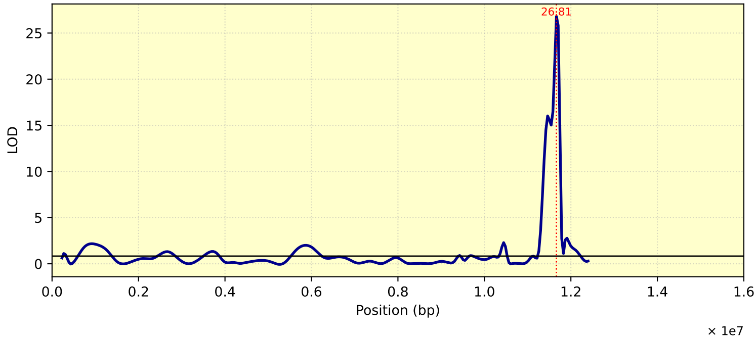
LOD Curve - chr03 - TC26ME4
