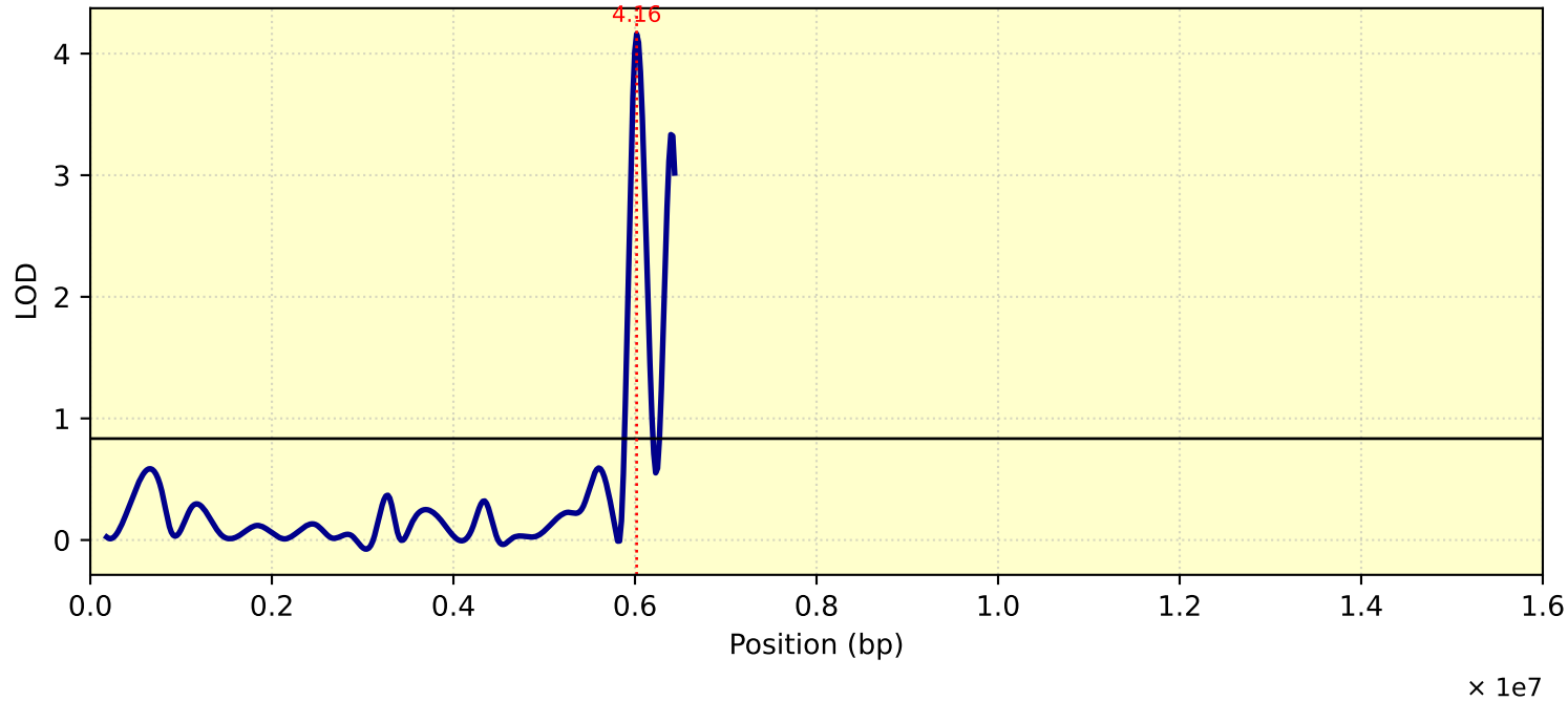
LOD Curve - chr15 - TC26ME4
