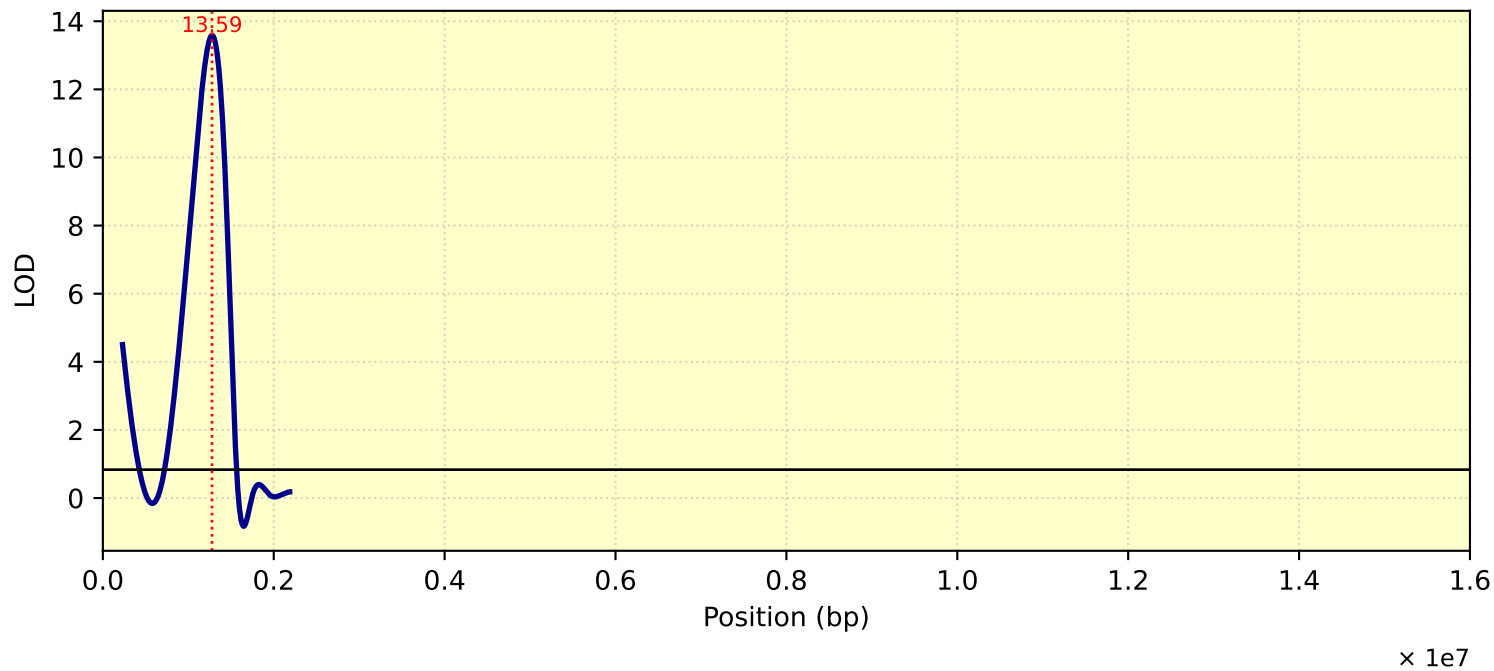
LOD Curve - chr23 - TC26ME4
