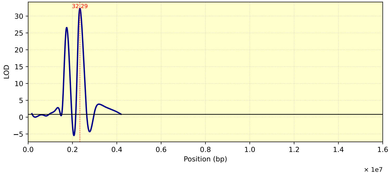
LOD Curve - chr16 - TC26ME4
