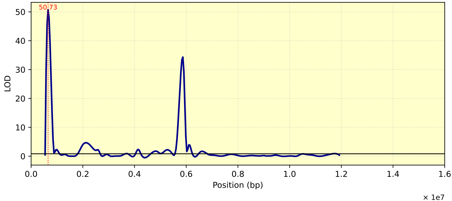
LOD Curve - chr05 - TC26ME4
