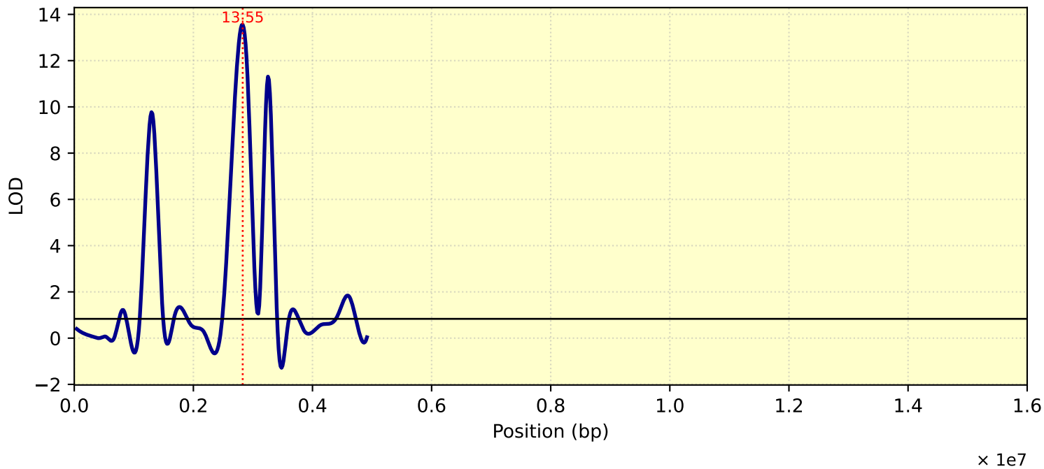
LOD Curve - chr12 - TC26ME4
