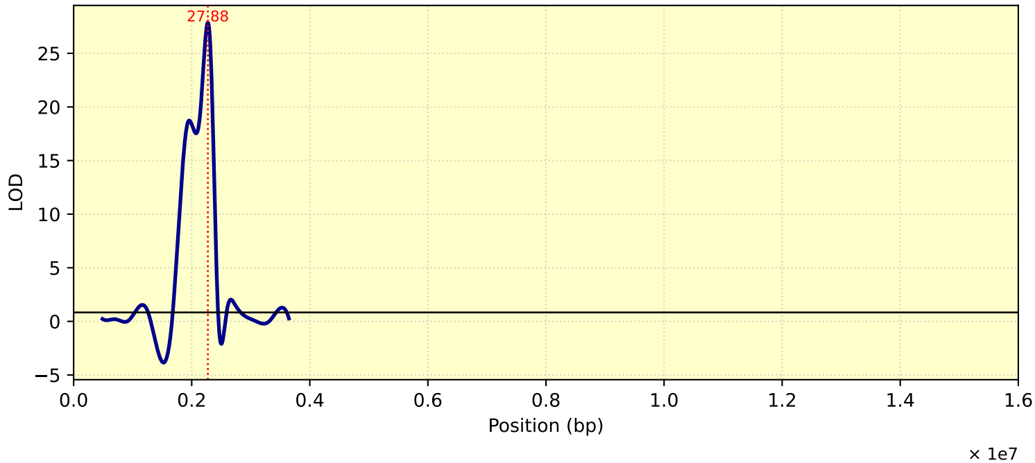
LOD Curve - chr24 - TC26ME4
