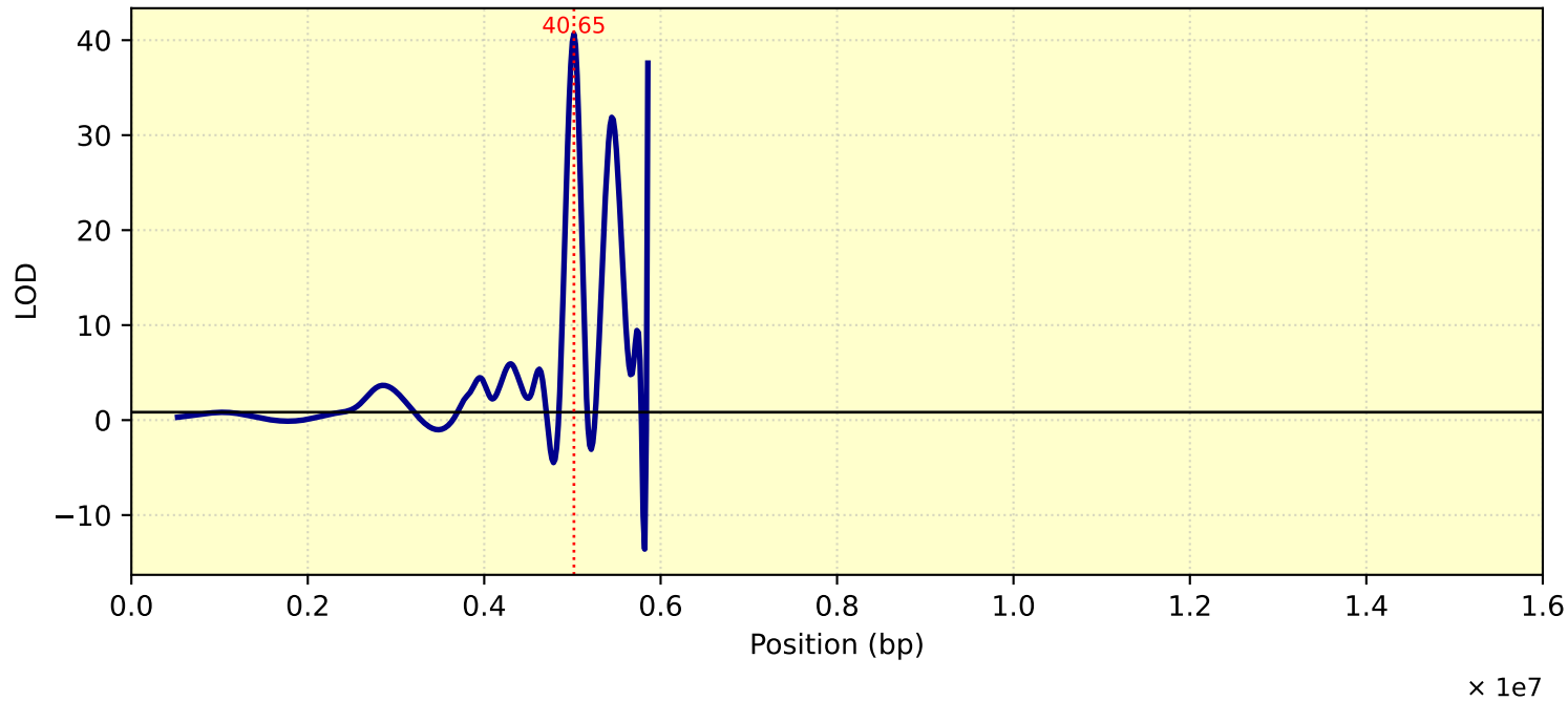
LOD Curve - chr18 - TC26ME4
