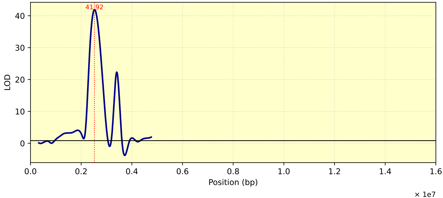
LOD Curve - chr17 - TC26ME4
