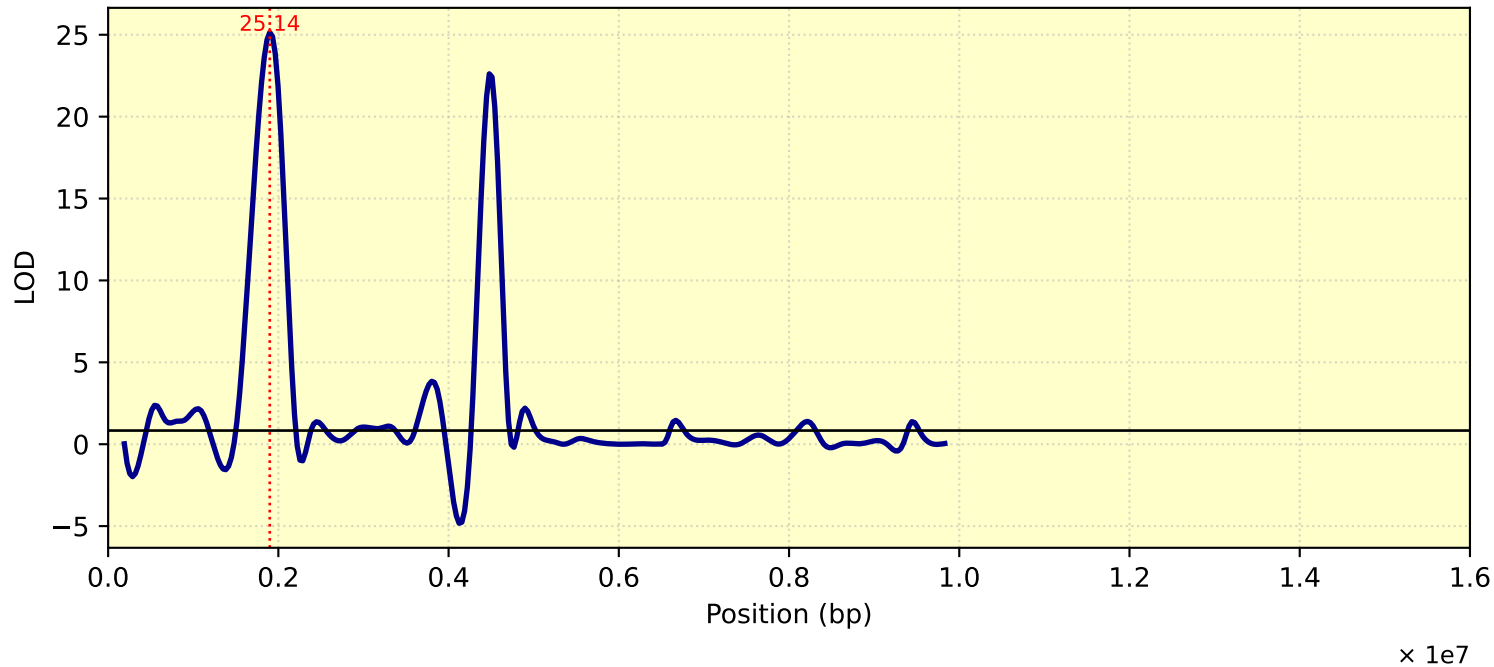
LOD Curve - chr06 - TC26ME4
