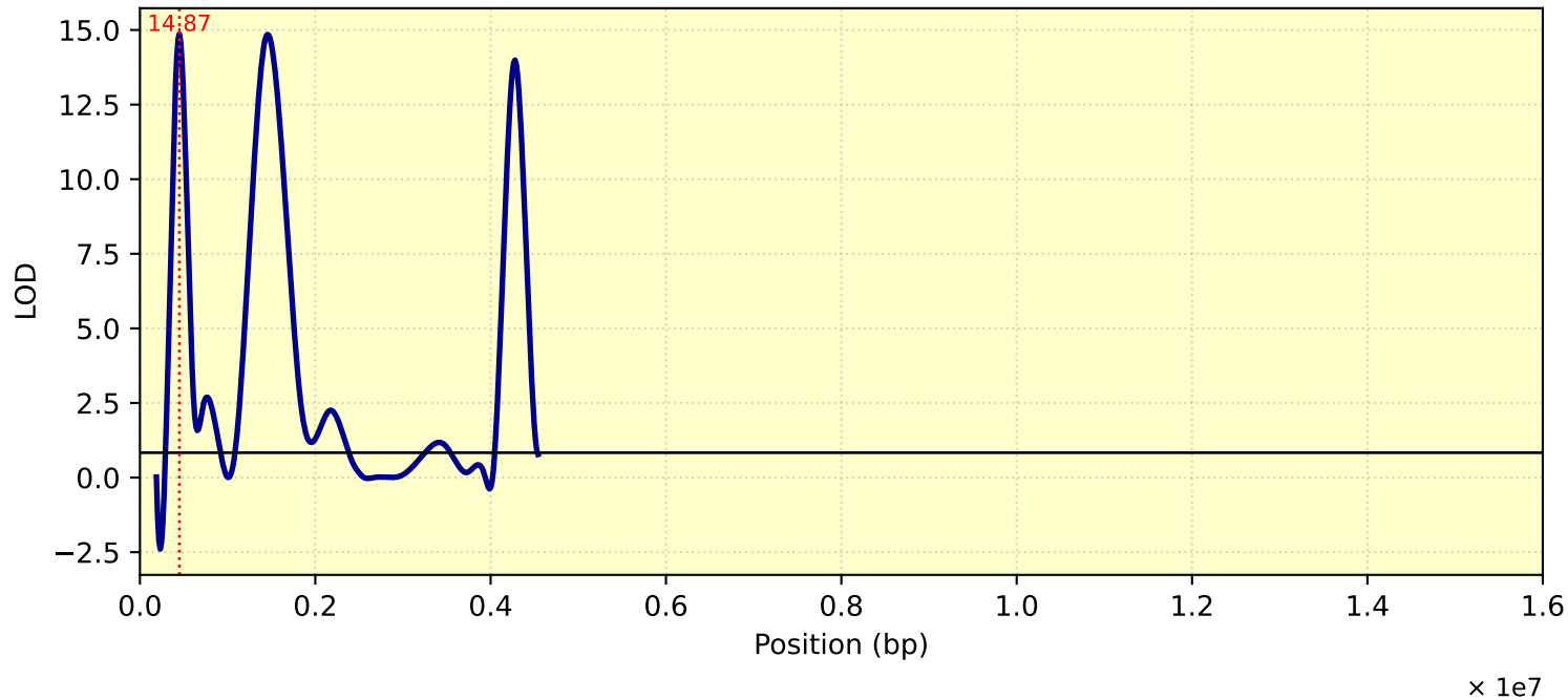
LOD Curve - chr19 - TC26ME4
