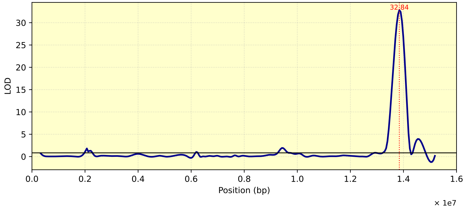
LOD Curve - chr01 - TC26ME4
