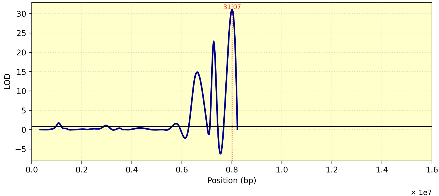
LOD Curve - chr07 - TC26ME4
