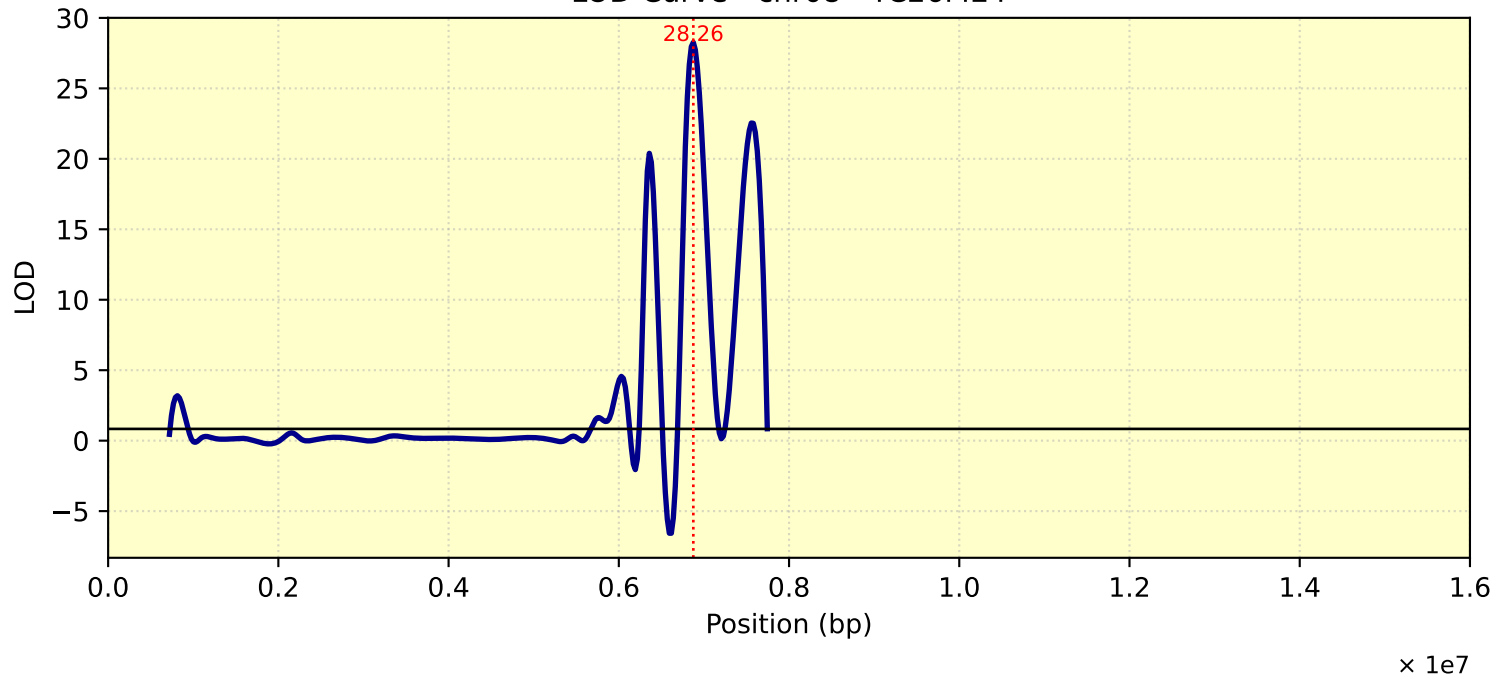
LOD Curve - chr08 - TC26ME4
