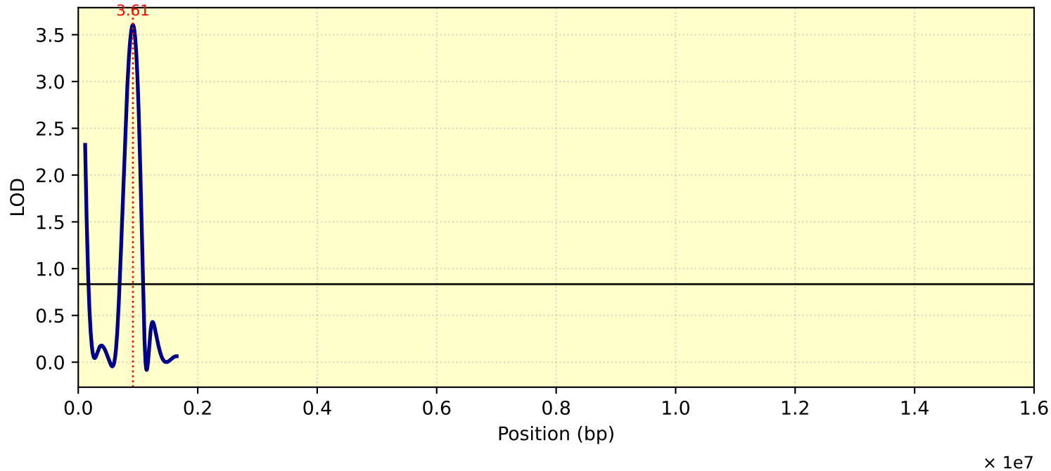
LOD Curve - chr26 - TC26ME4
