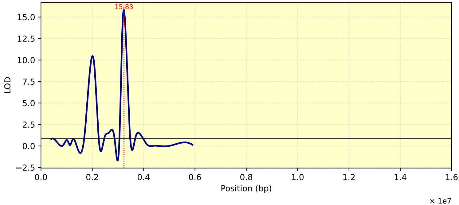
LOD Curve - chr14 - TC26ME4
