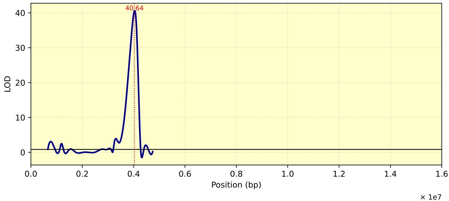
LOD Curve - chr21 - TC26ME4
