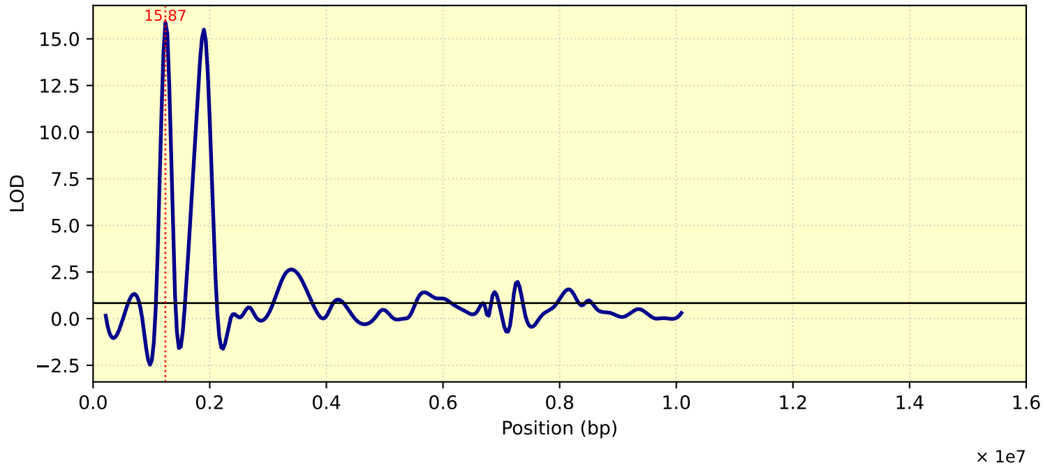
LOD Curve - chr04 - TC26ME4
