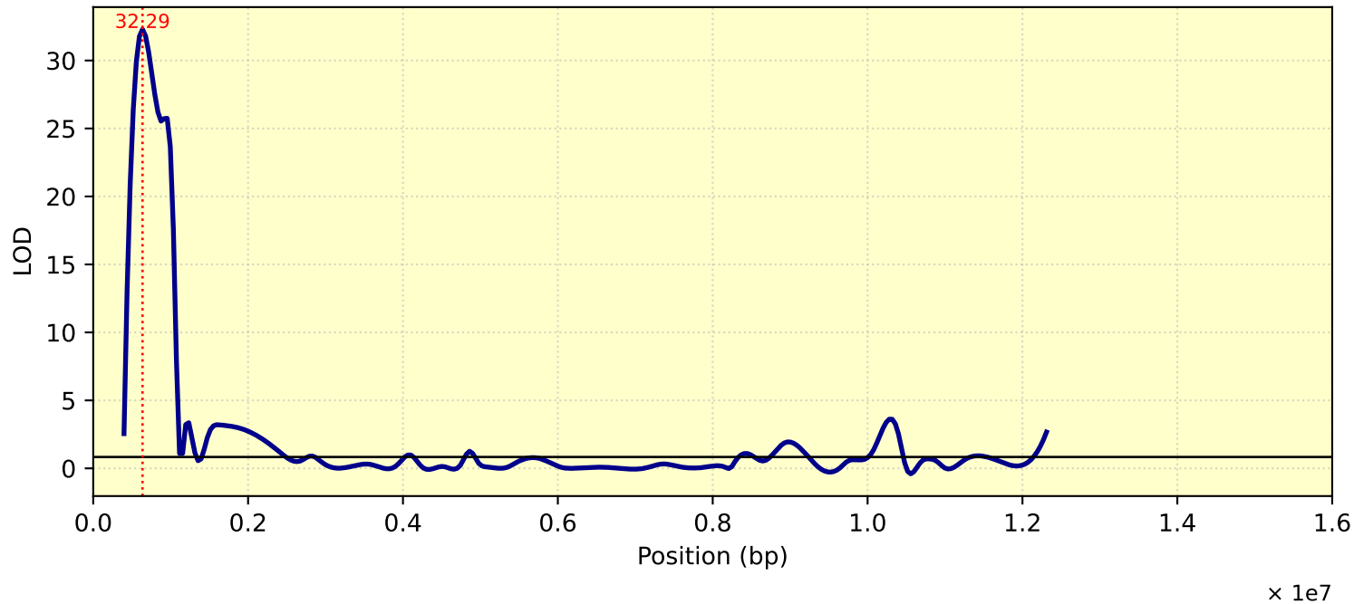
LOD Curve - chr02 - TC26ME4
