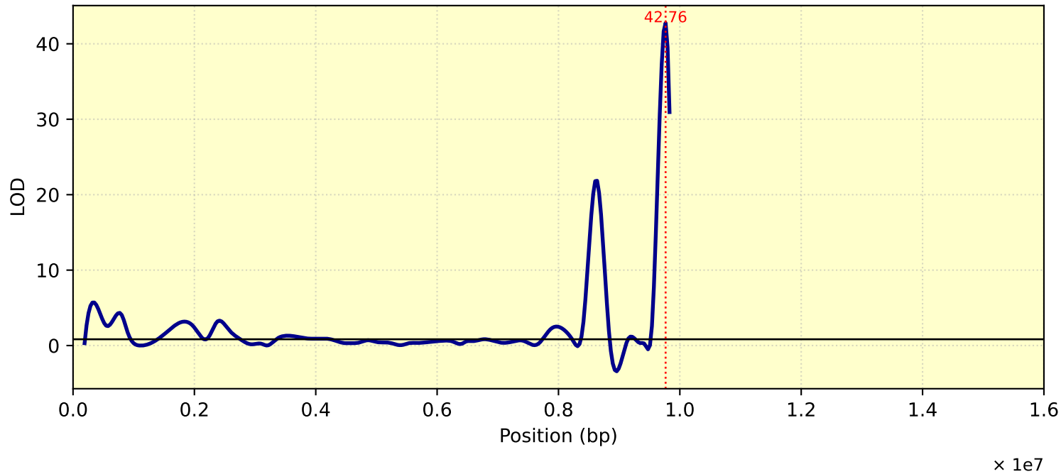
LOD Curve - chr06 - Tc25
