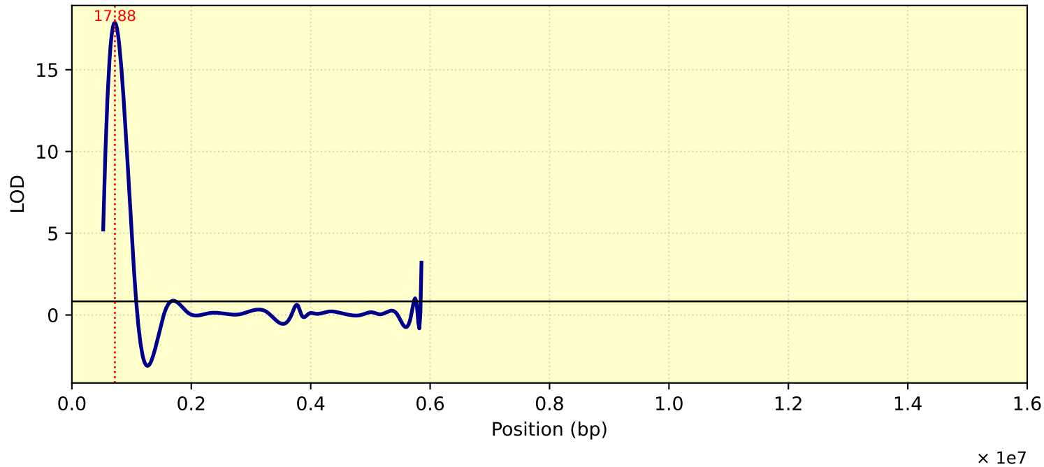
LOD Curve - chr18 - Tc25
