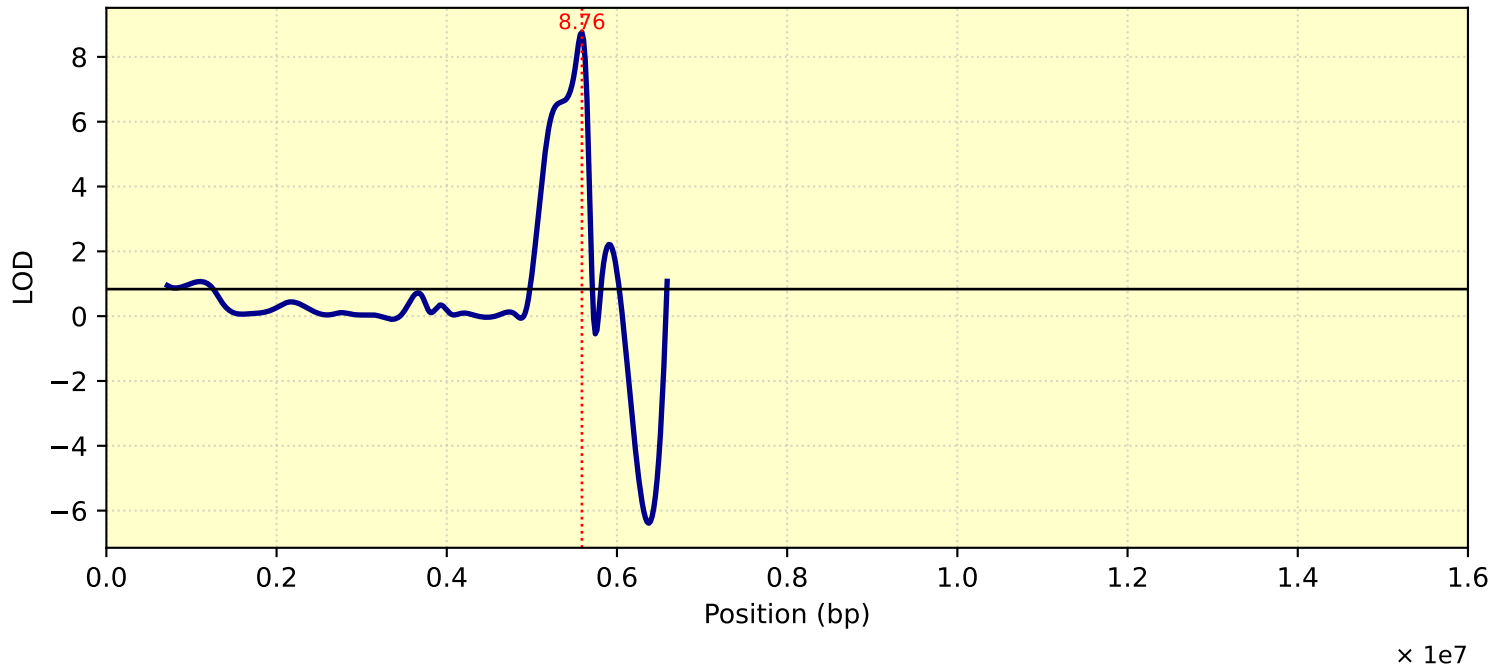
LOD Curve - chr13 - Tc25
