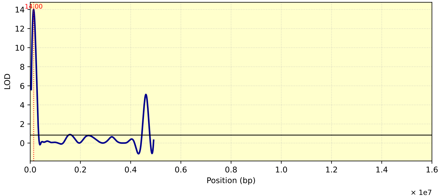
LOD Curve - chr12 - Tc25
