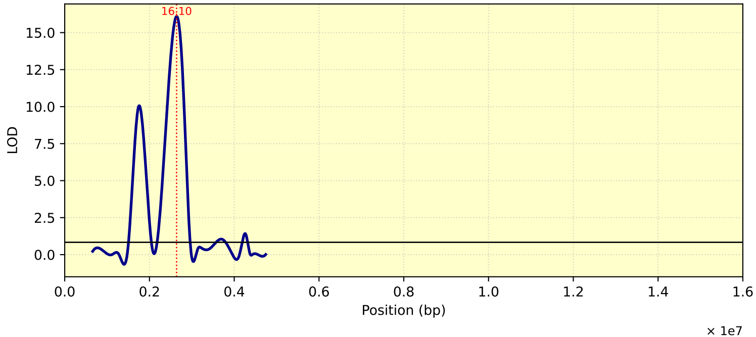
LOD Curve - chr21 - Tc25
