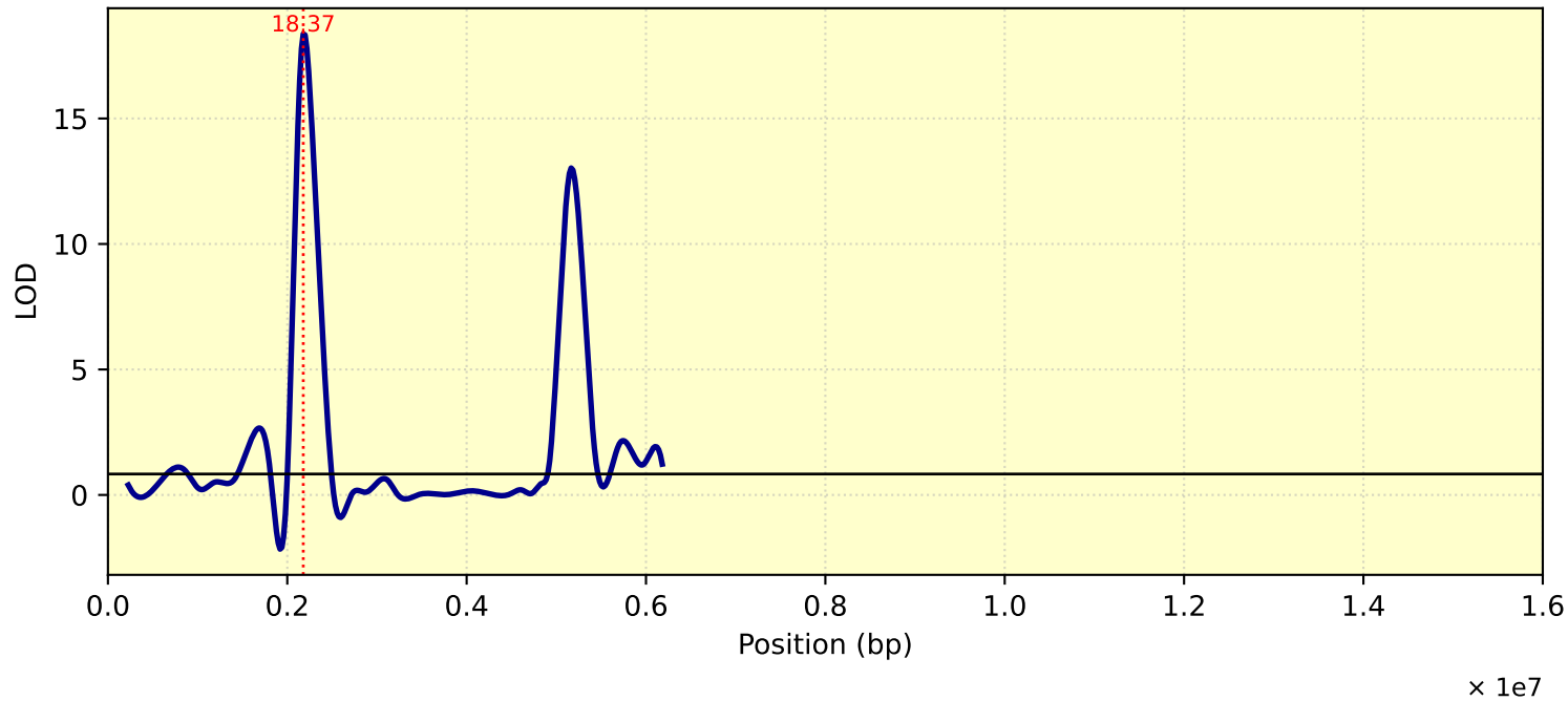
LOD Curve - chr11 - Tc25
