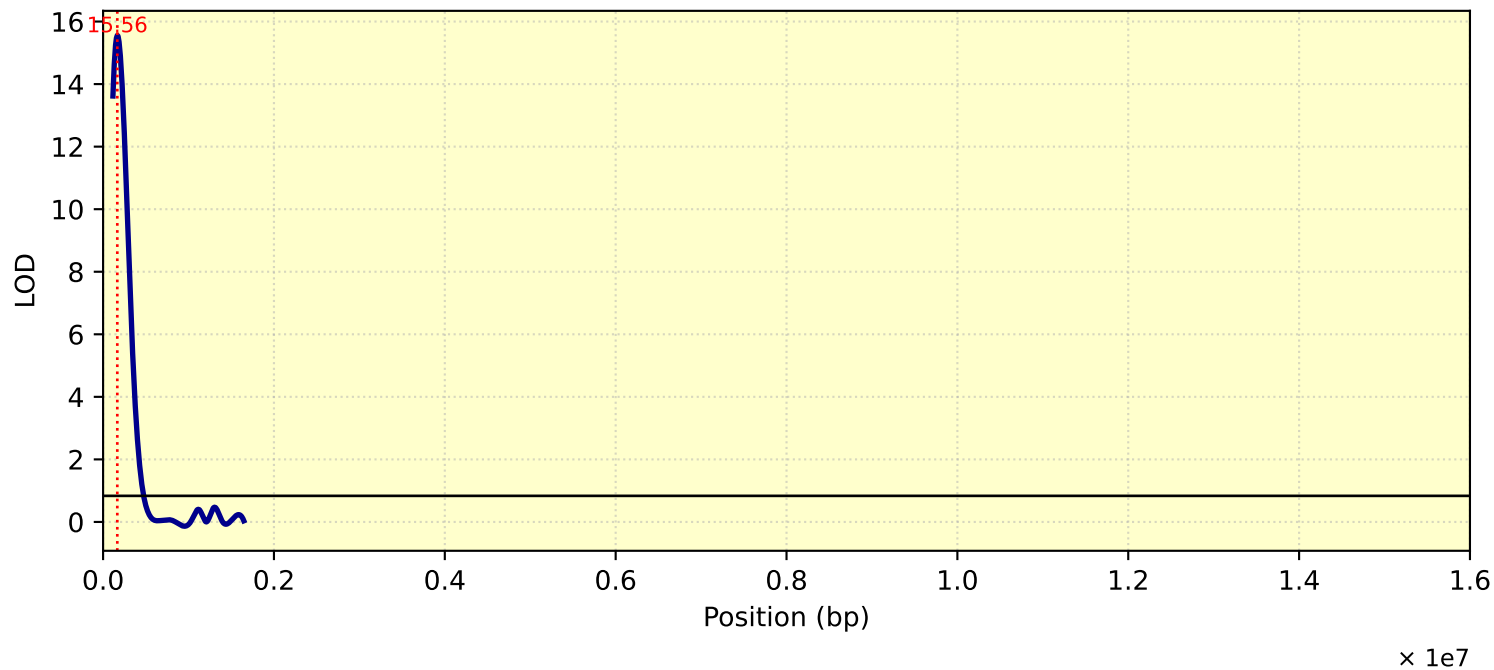
LOD Curve - chr26 - Tc25
