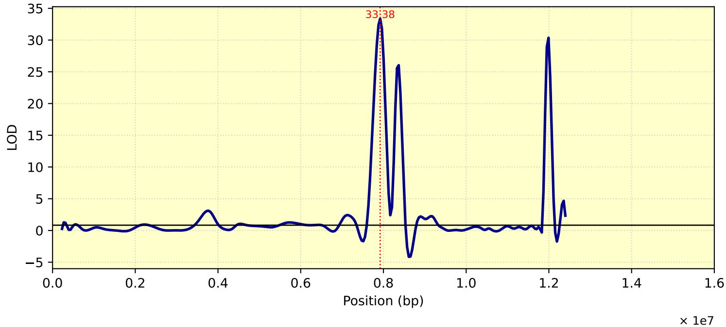
LOD Curve - chr03 - Tc25
