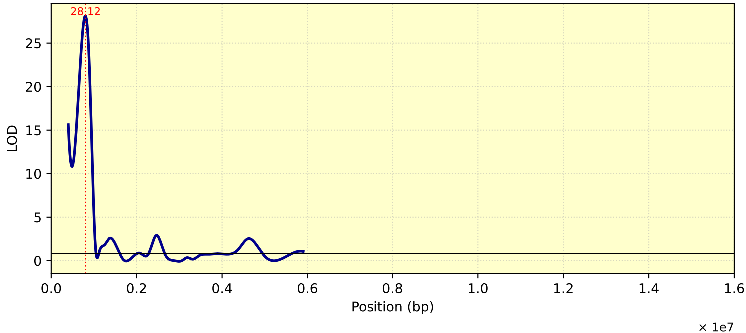
LOD Curve - chr14 - Tc25
