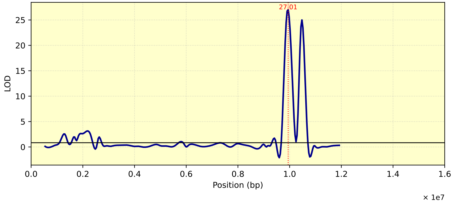
LOD Curve - chr05 - Tc25
