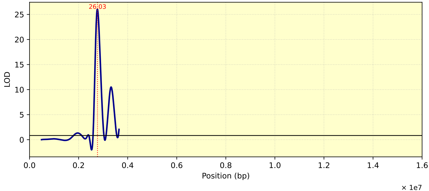
LOD Curve - chr24 - Tc25
