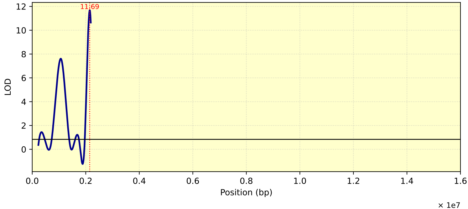
LOD Curve - chr23 - Tc25
