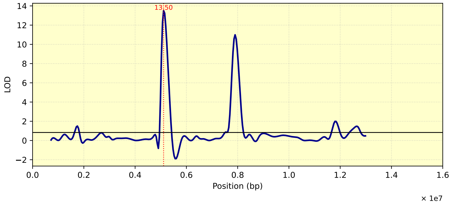
LOD Curve - chr09 - Tc25
