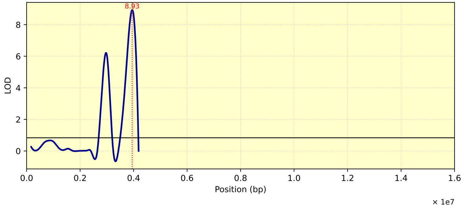
LOD Curve - chr16 - Tc25
