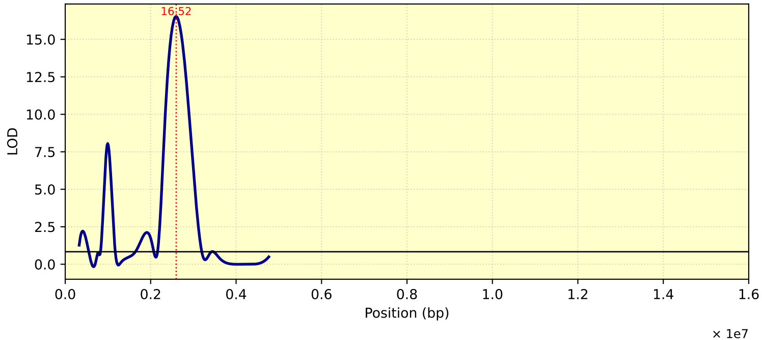
LOD Curve - chr17 - Tc25
