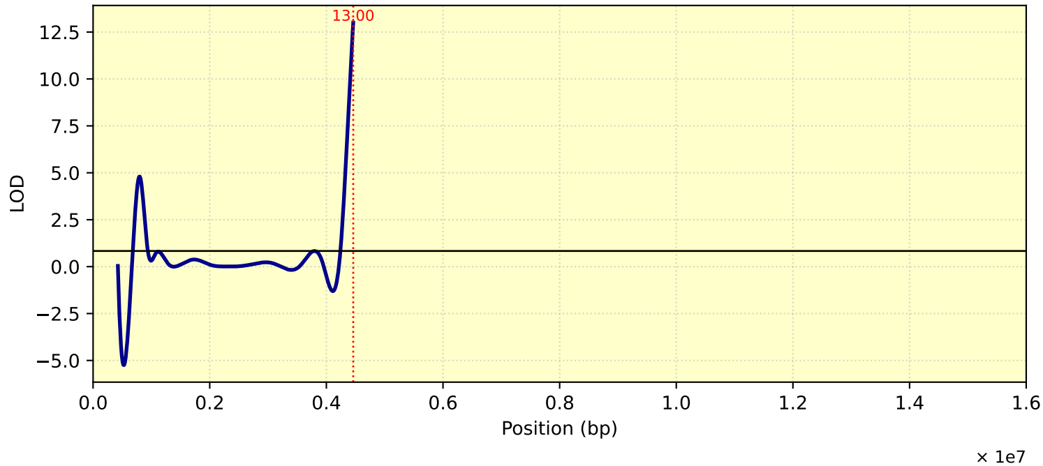
LOD Curve - chr22 - Tc25
