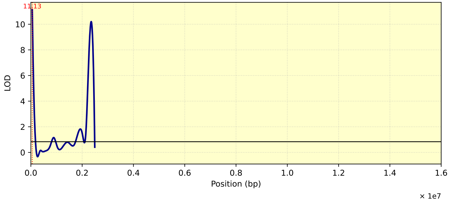
LOD Curve - chr25 - Tc25
