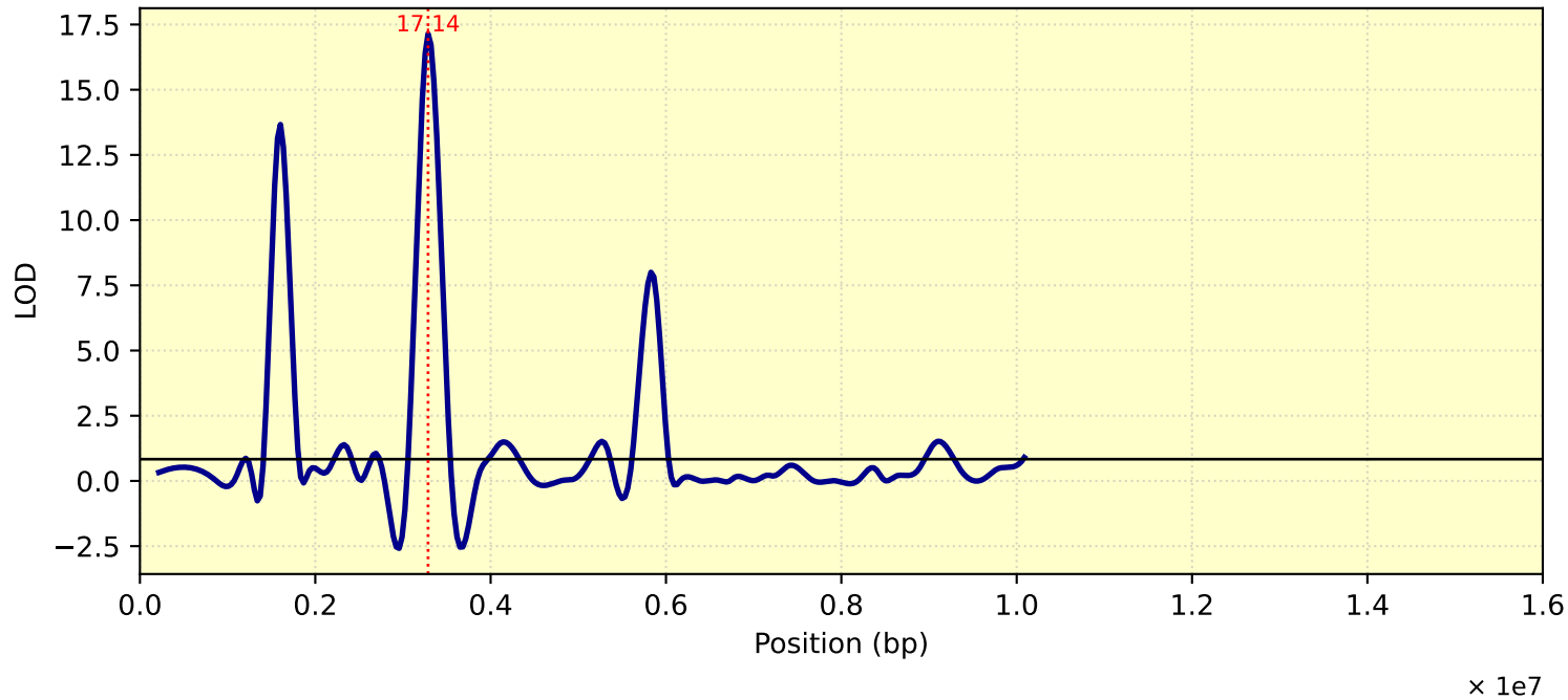
LOD Curve - chr04 - Tc25
