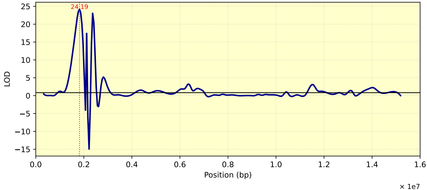
LOD Curve - chr01 - Tc25
