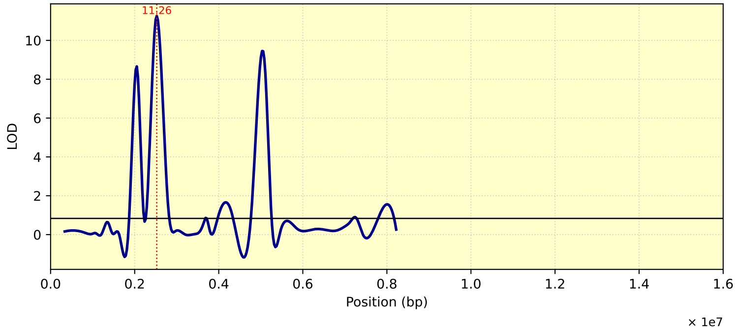
LOD Curve - chr07 - Tc25
