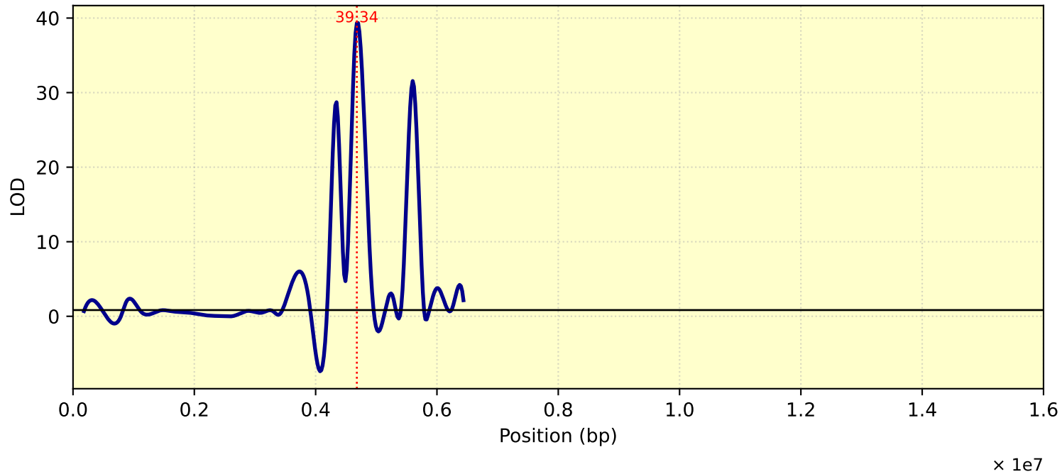
LOD Curve - chr15 - Tc25
