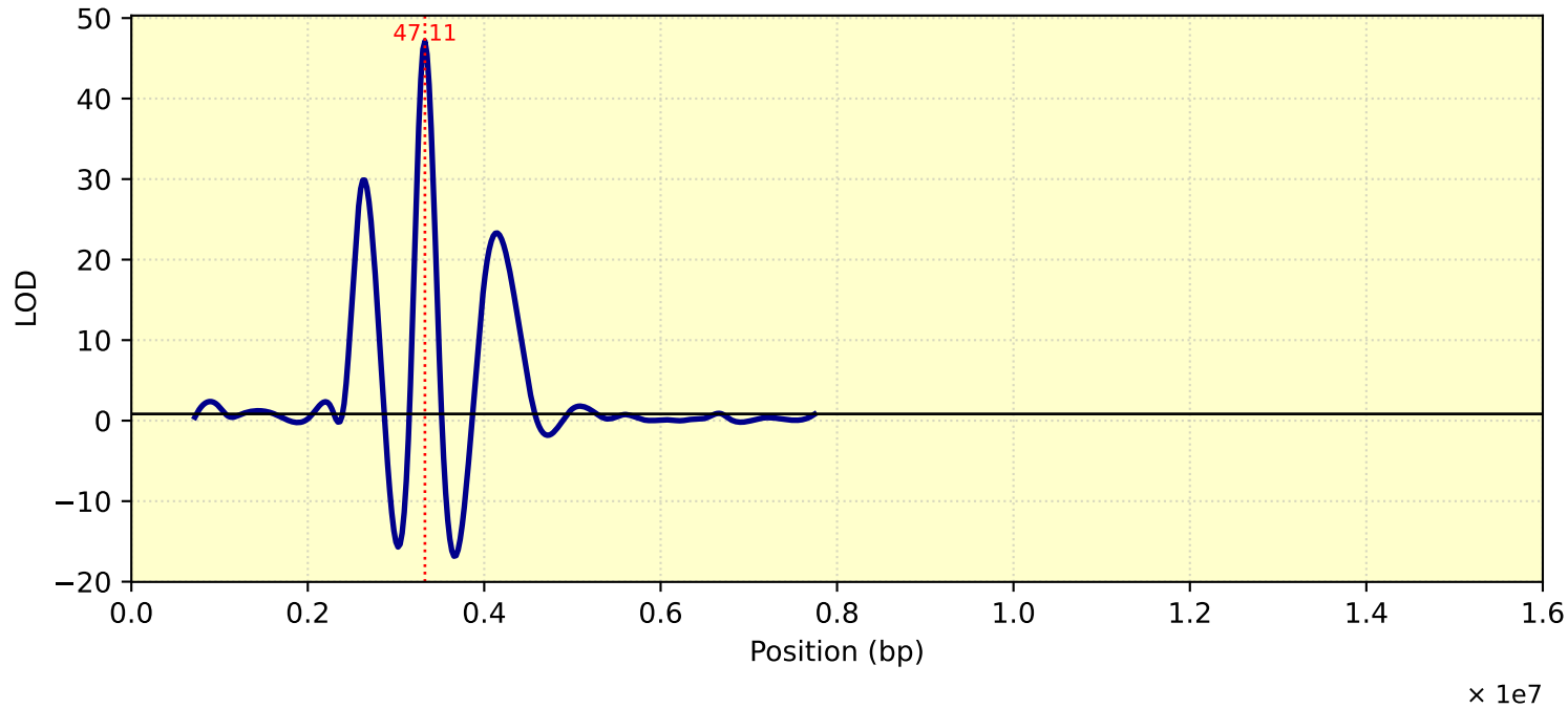
LOD Curve - chr08 - Tc25
