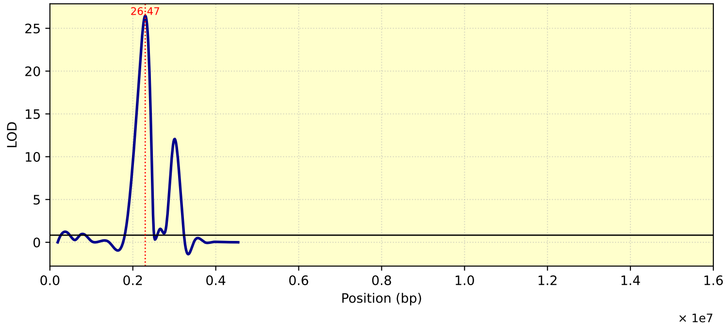
LOD Curve - chr19 - Tc25
