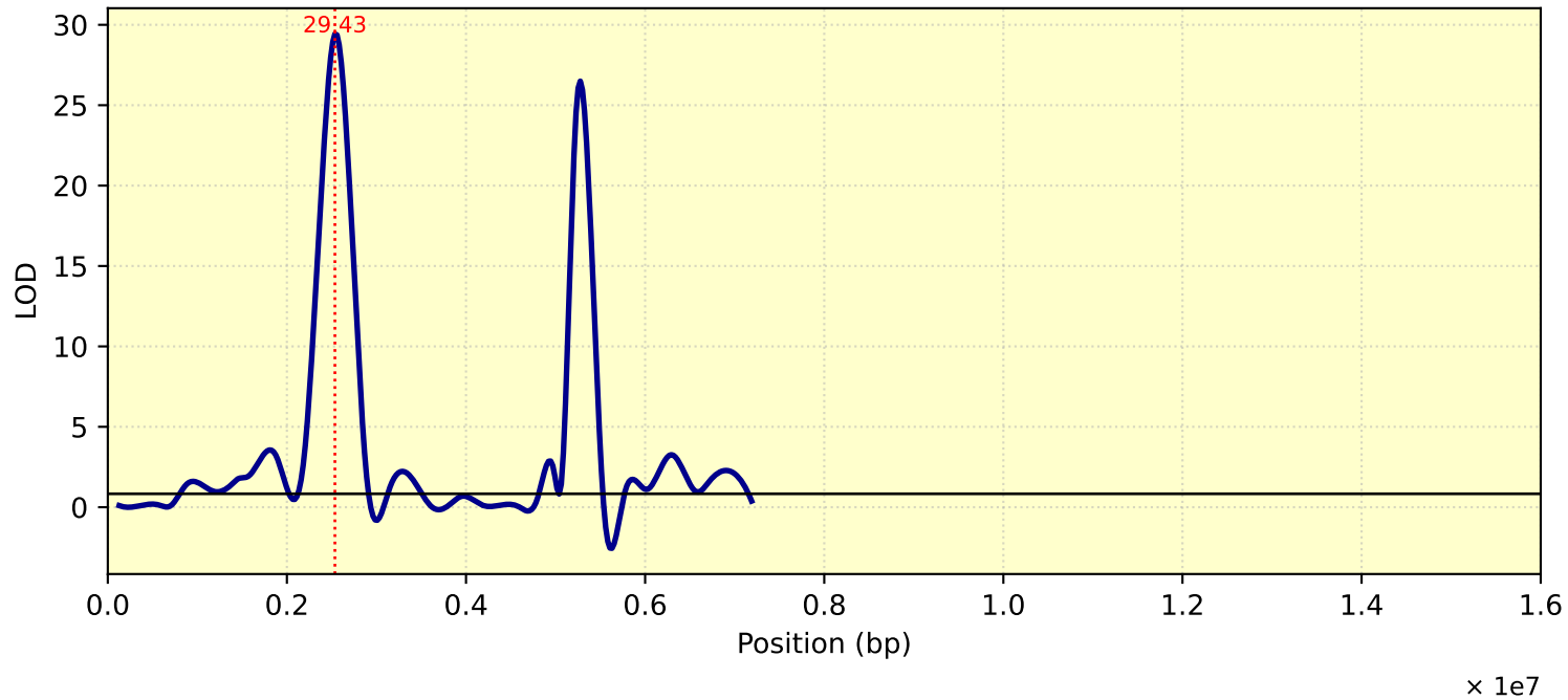
LOD Curve - chr10 - Tc25
