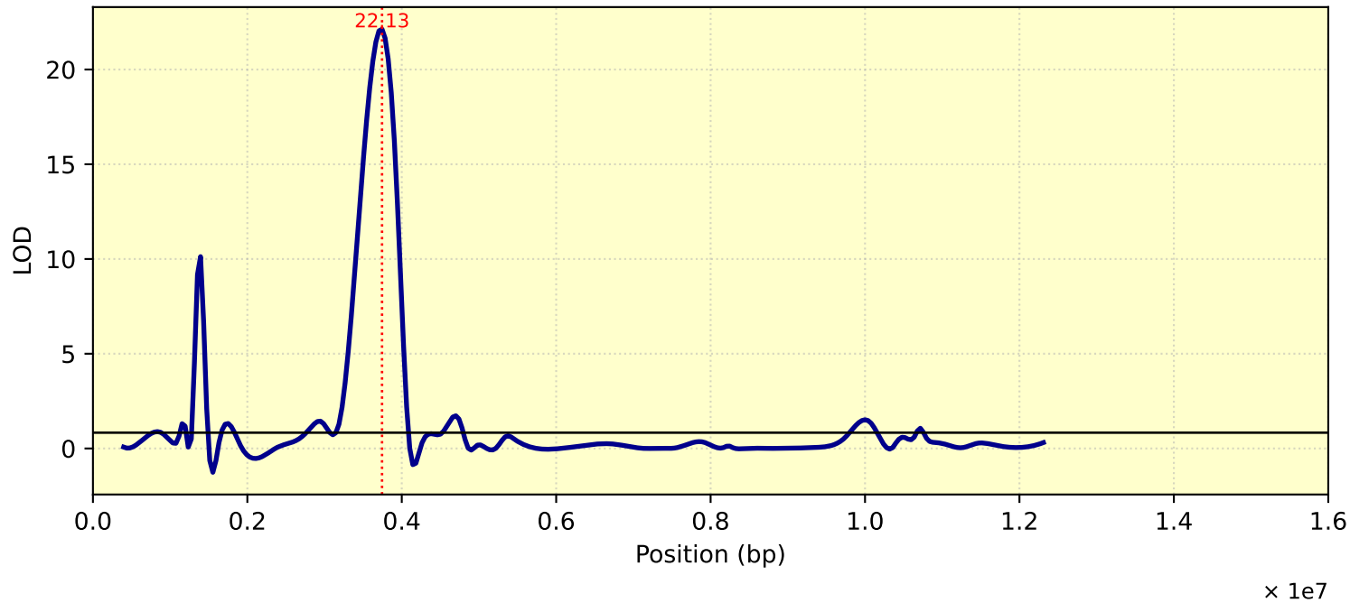
LOD Curve - chr02 - Tc25
