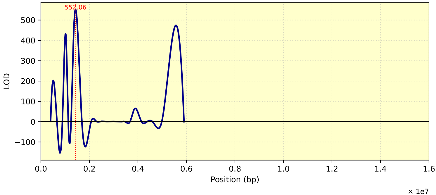
LOD Curve - chr14 - Tc26Me10T1
