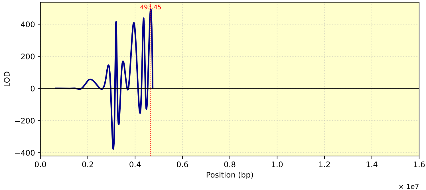
LOD Curve - chr21 - Tc26Me10T1
