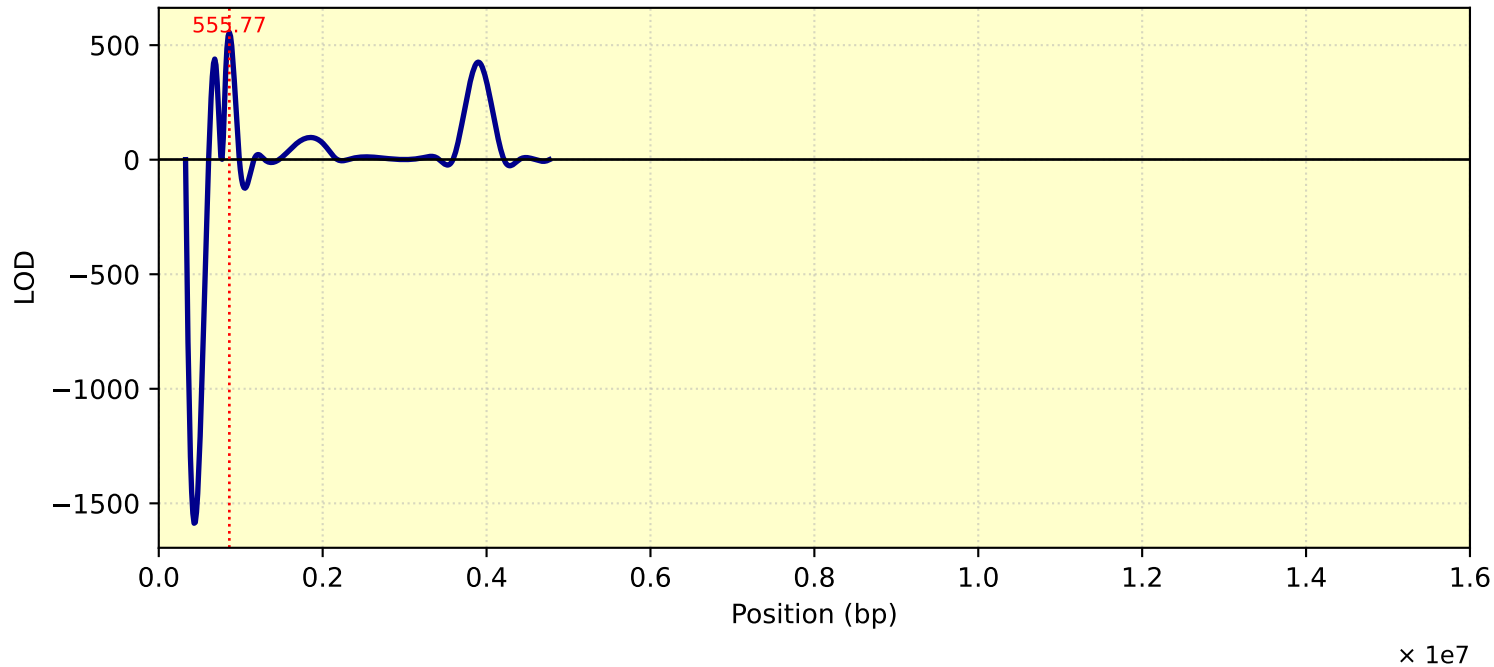
LOD Curve - chr17 - Tc26Me10T1
