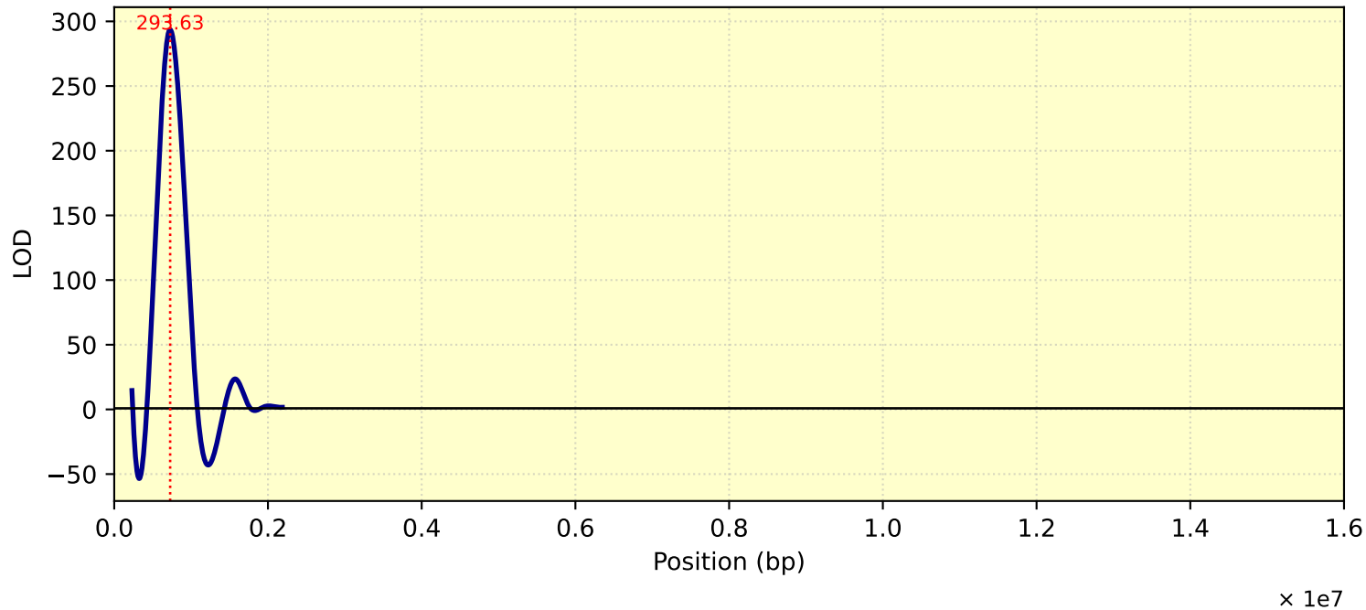
LOD Curve - chr23 - Tc26Me10T1
