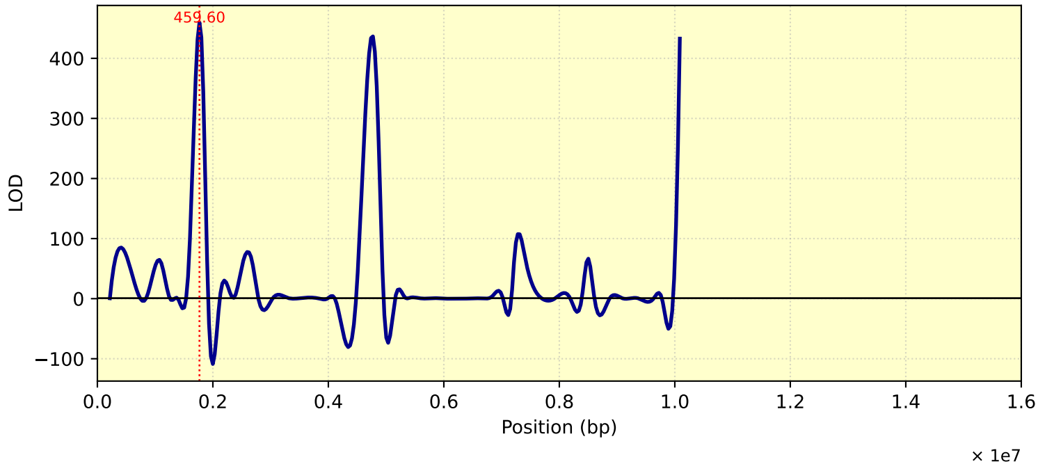
LOD Curve - chr04 - Tc26Me10T1
