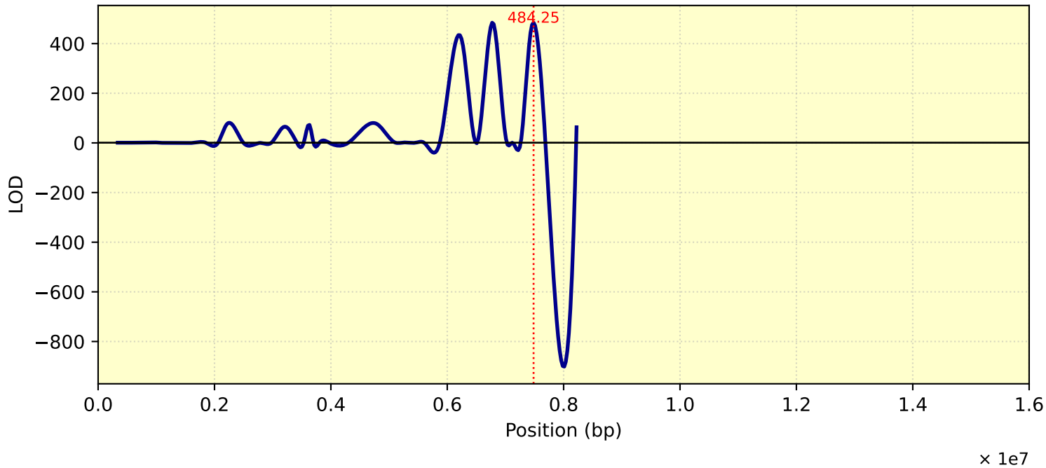
LOD Curve - chr07 - Tc26Me10T1
