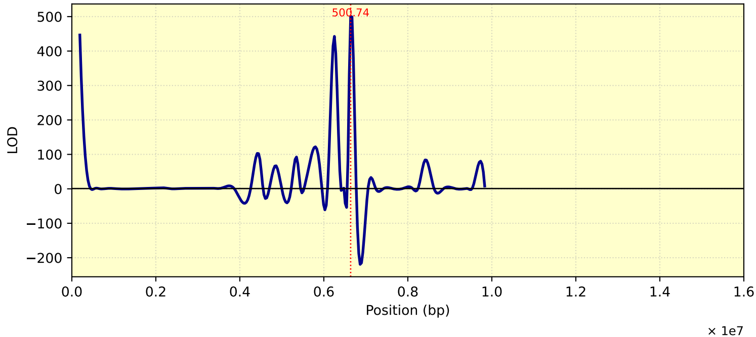
LOD Curve - chr06 - Tc26Me10T1
