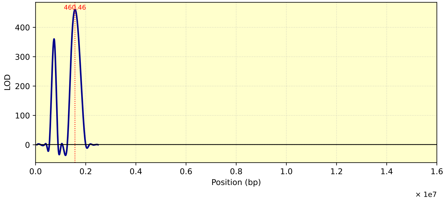
LOD Curve - chr25 - Tc26Me10T1
