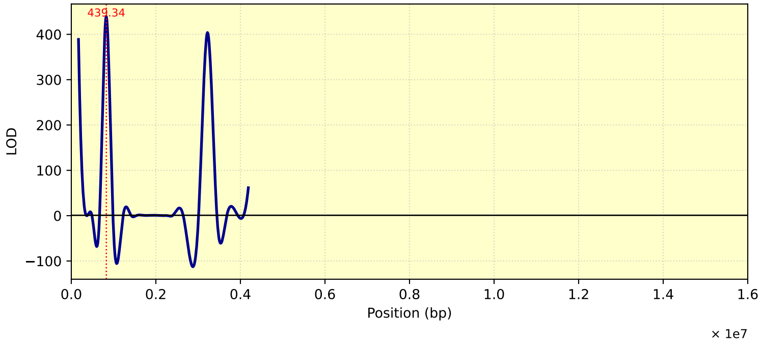
LOD Curve - chr16 - Tc26Me10T1
