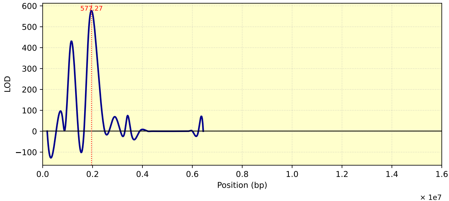
LOD Curve - chr15 - Tc26Me10T1
