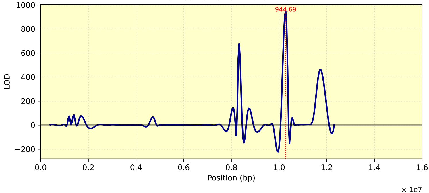
LOD Curve - chr02 - Tc26Me10T1
