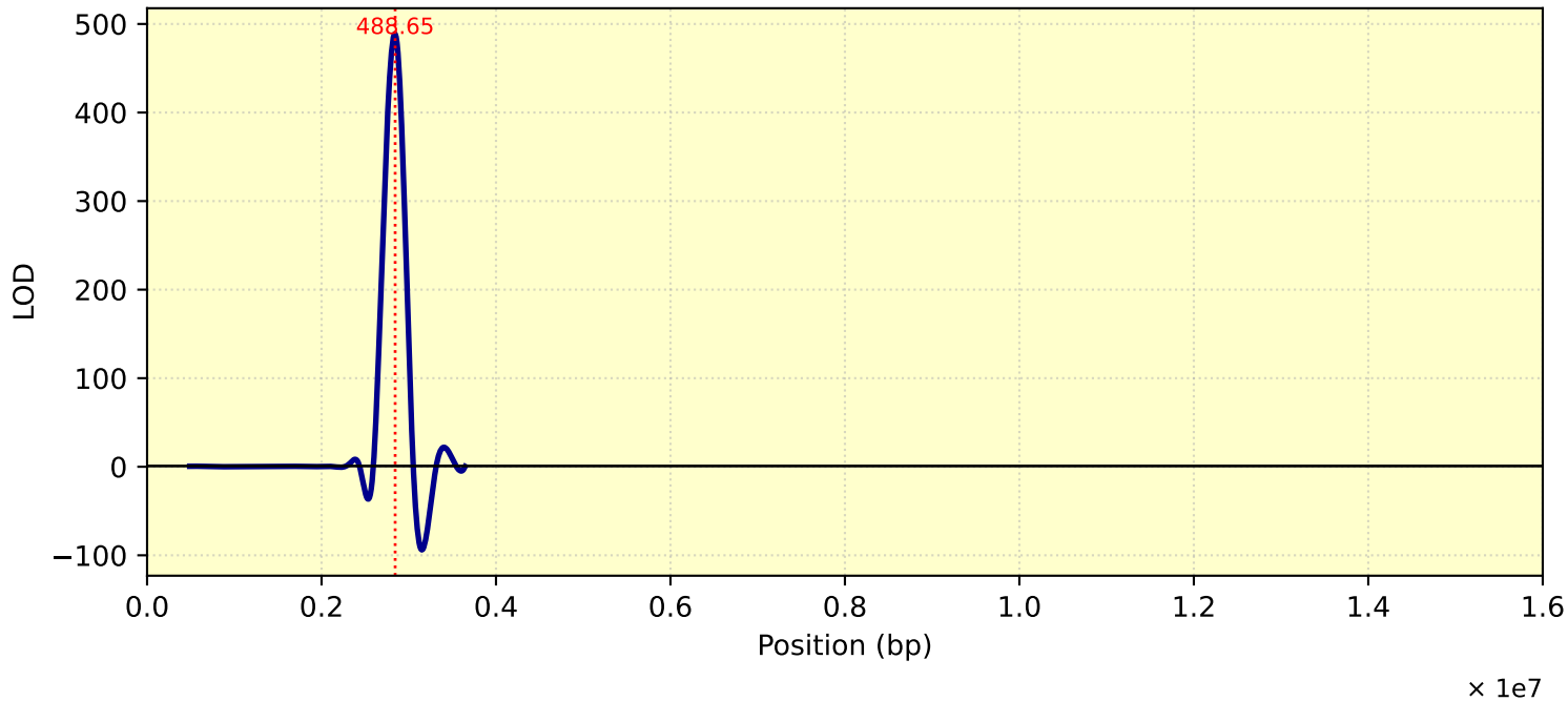
LOD Curve - chr24 - Tc26Me10T1
