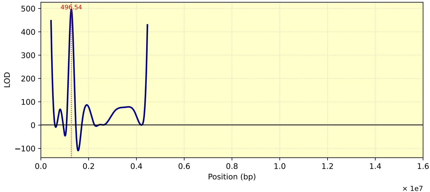
LOD Curve - chr22 - Tc26Me10T1
