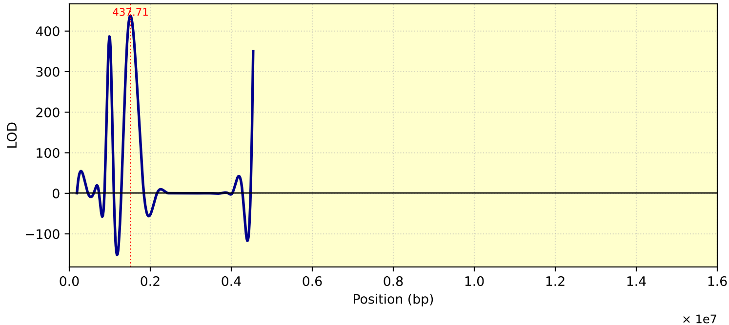
LOD Curve - chr19 - Tc26Me10T1
