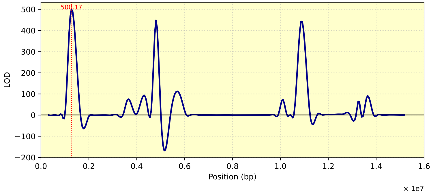
LOD Curve - chr01 - Tc26Me10T1
