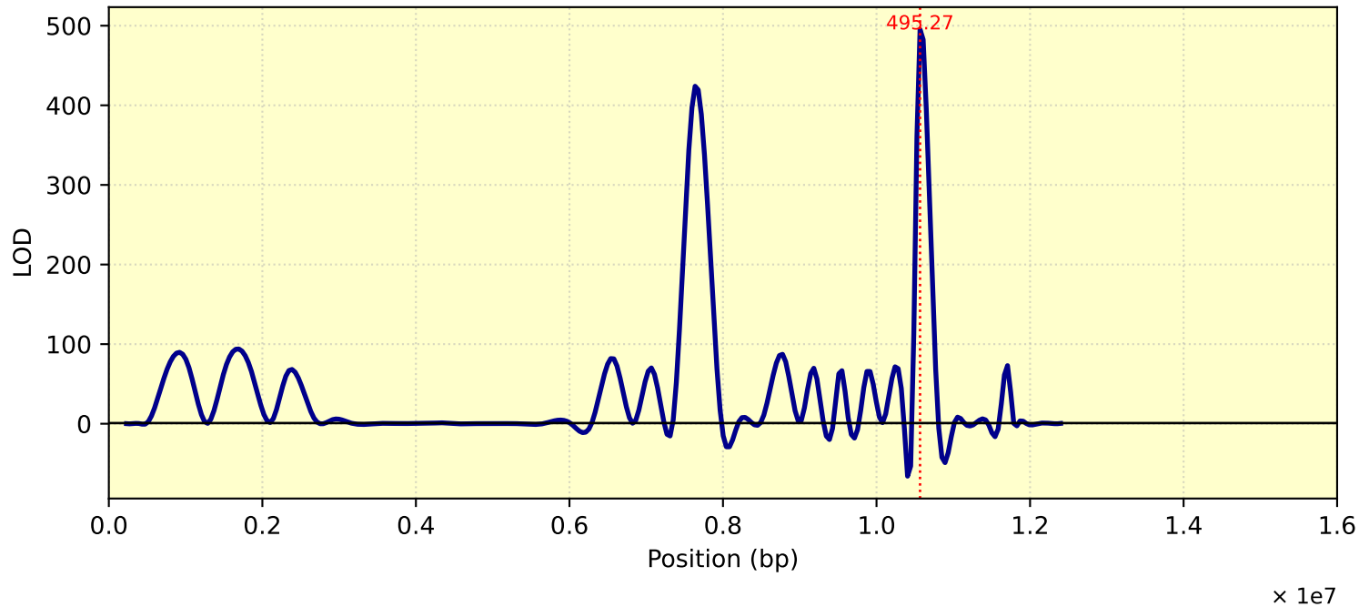
LOD Curve - chr03 - Tc26Me10T1
