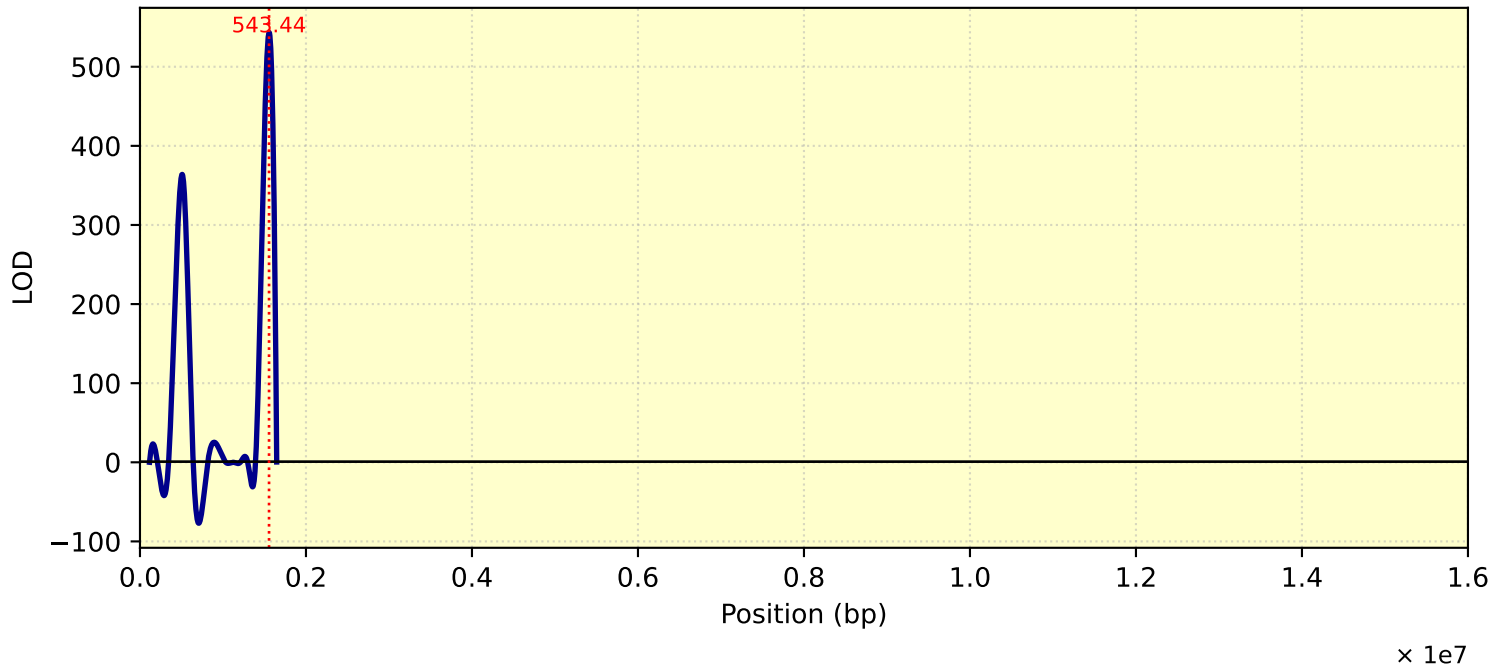
LOD Curve - chr26 - Tc26Me10T1
