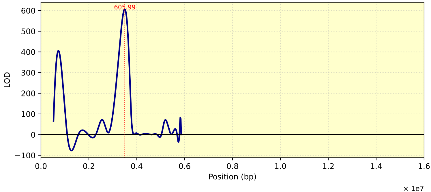
LOD Curve - chr18 - Tc26Me10T1
