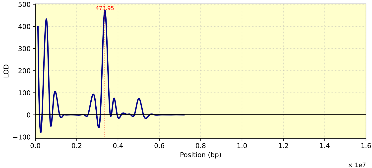
LOD Curve - chr10 - Tc26Me10T1
