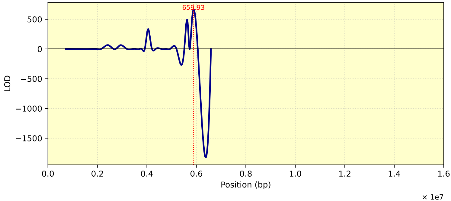
LOD Curve - chr13 - Tc26Me10T1
