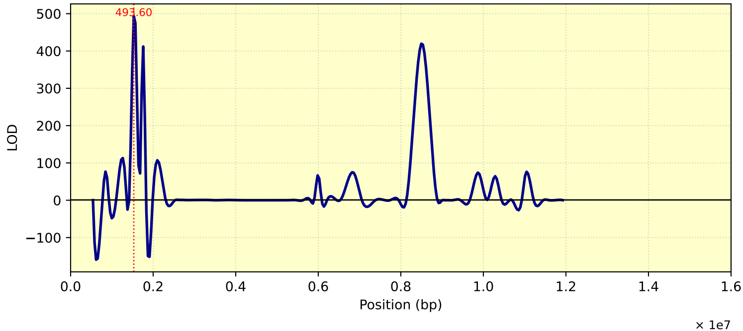
LOD Curve - chr05 - Tc26Me10T1
