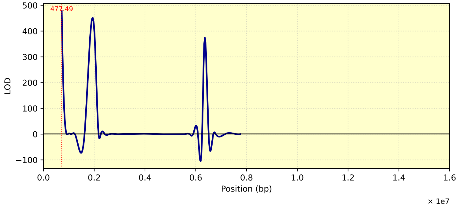
LOD Curve - chr08 - Tc26Me10T1
