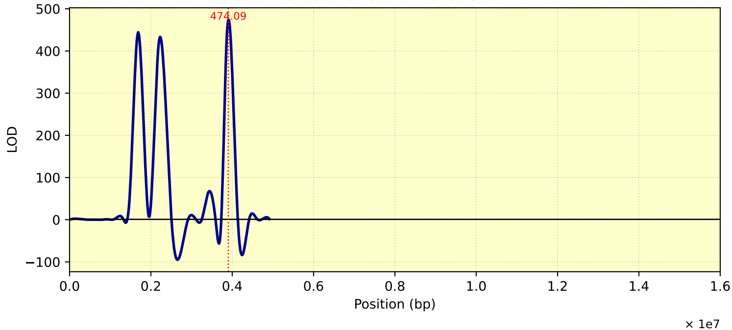
LOD Curve - chr12 - Tc26Me10T1
