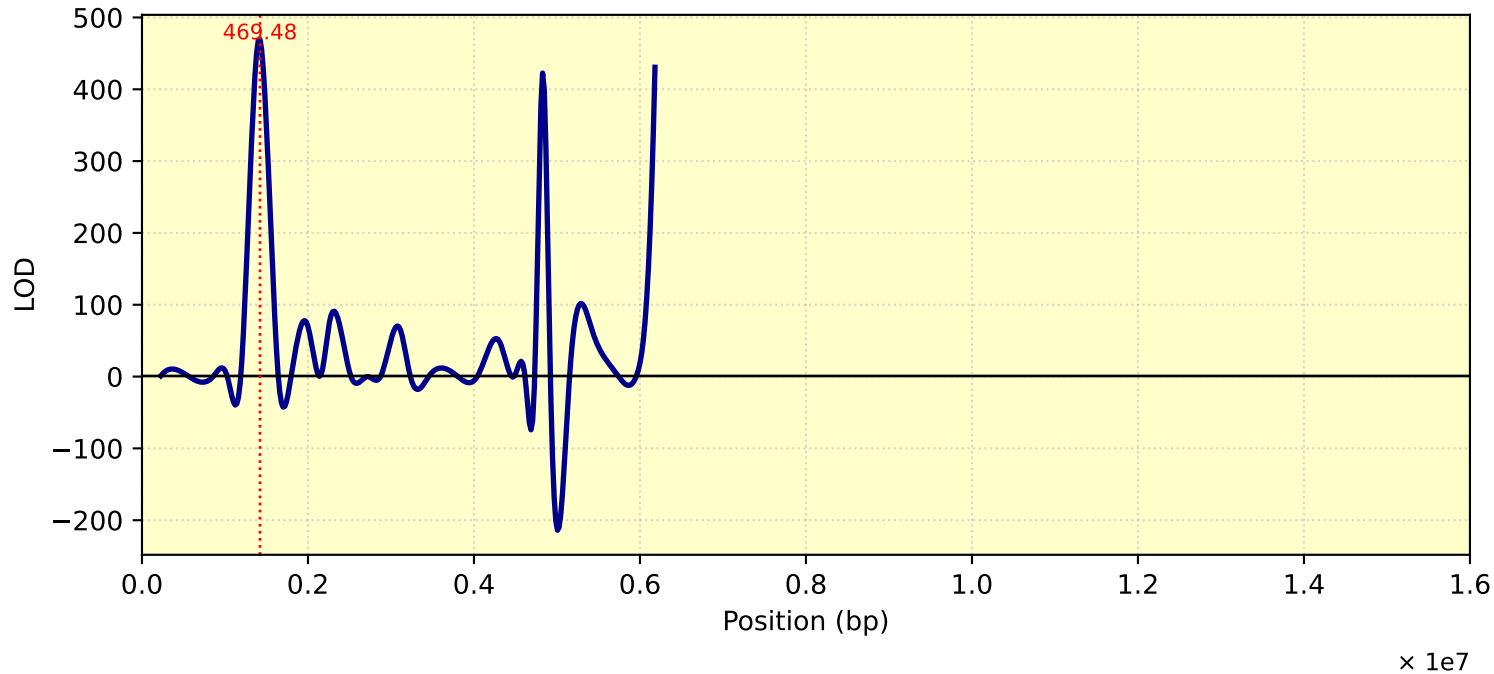
LOD Curve - chr11 - Tc26Me10T1
