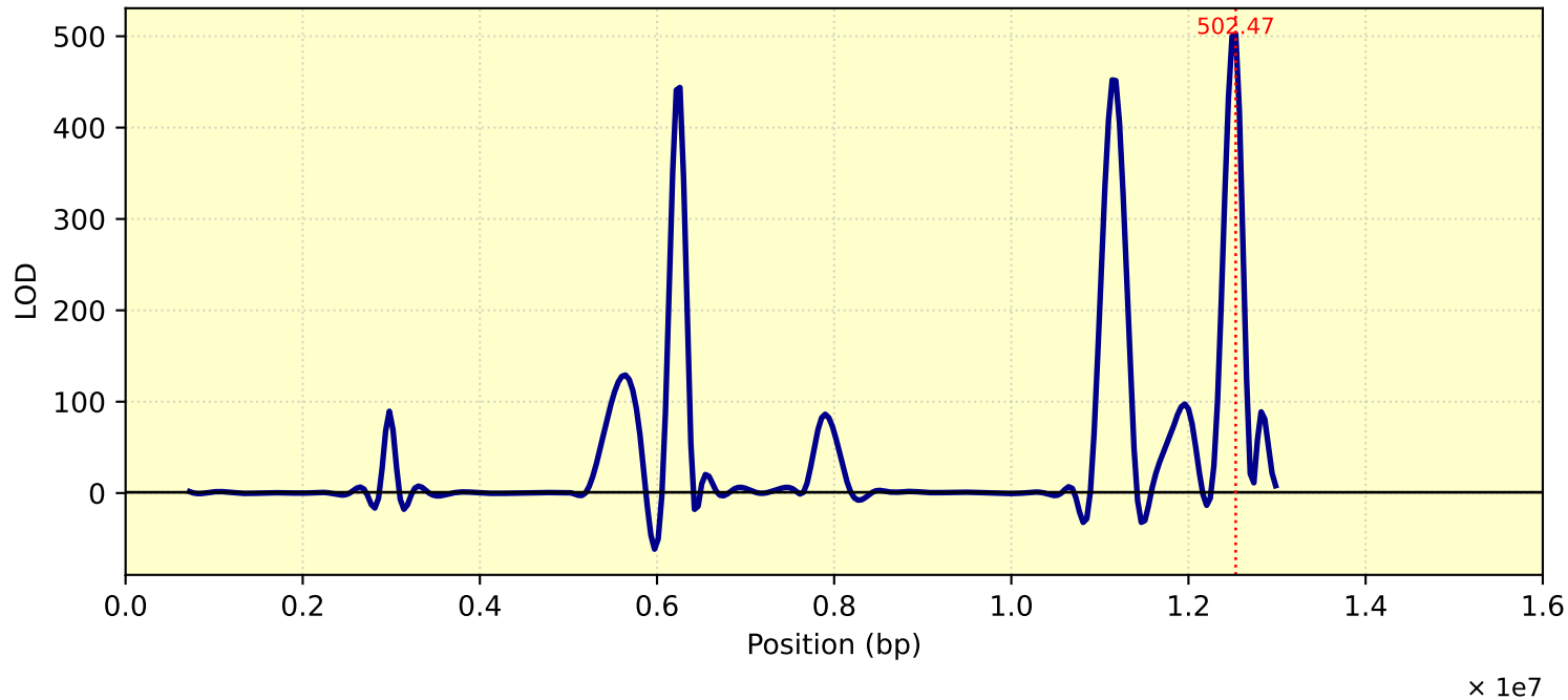
LOD Curve - chr09 - Tc26Me10T1
