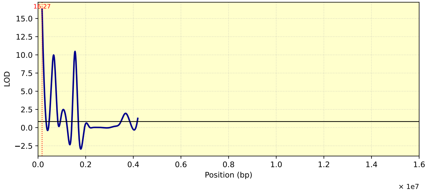
LOD Curve - chr16 - Tc27M11-13D
