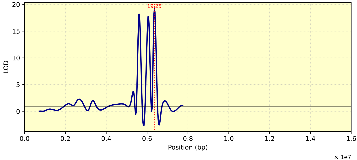
LOD Curve - chr08 - Tc27M11-13D
