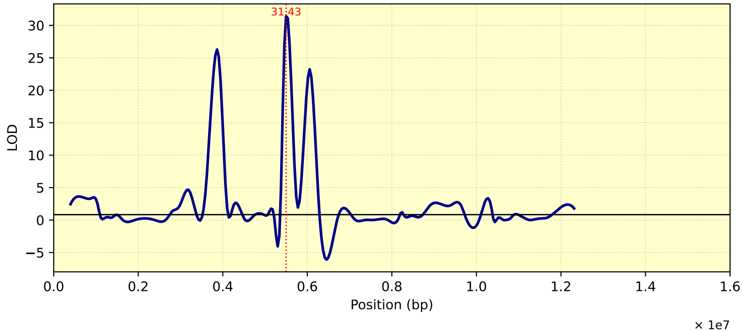
LOD Curve - chr02 - Tc27di11me15
