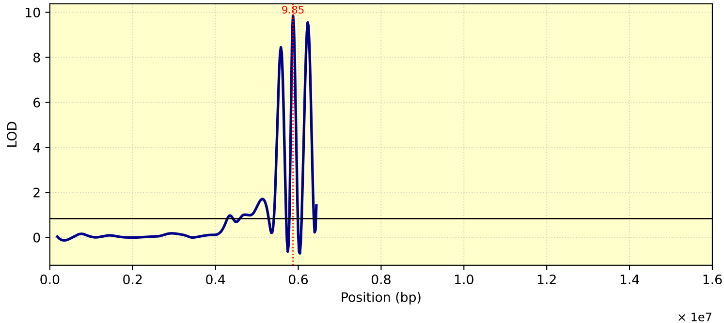
LOD Curve - chr15 - Tc27di11me15
