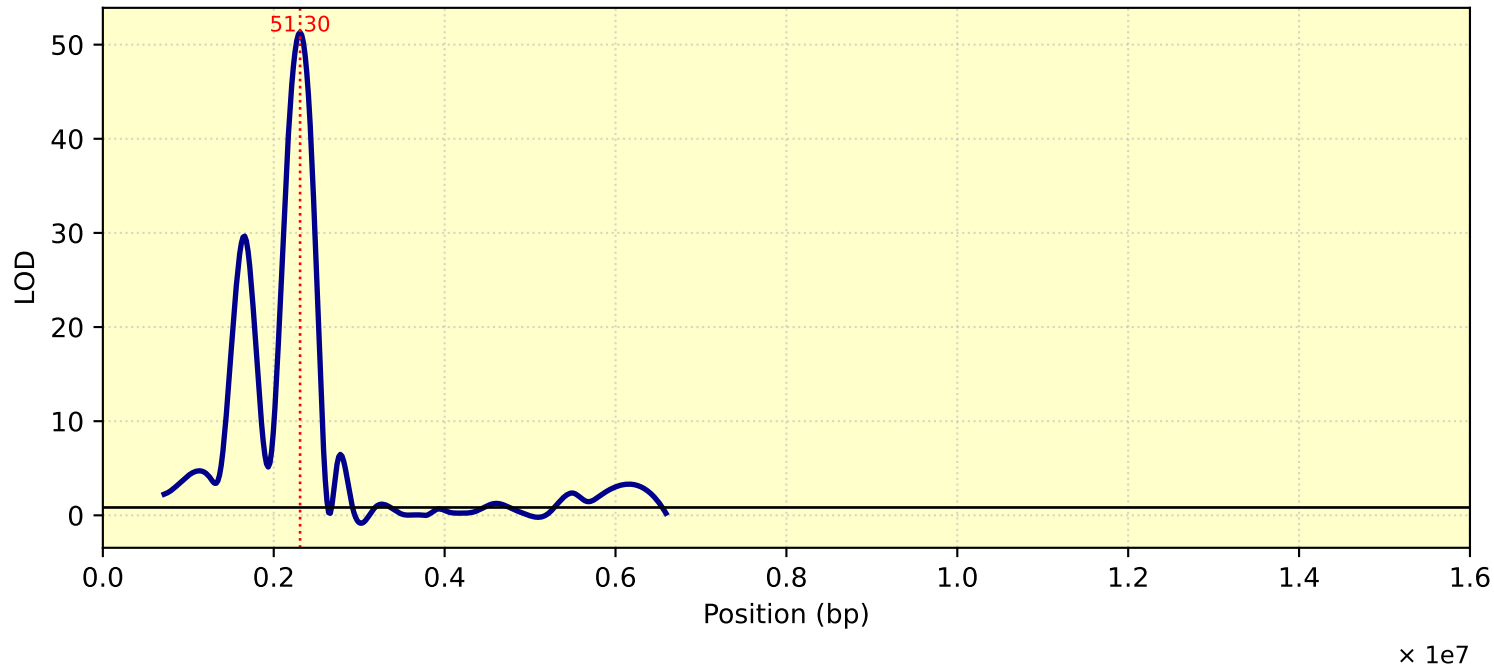
LOD Curve - chr13 - Tc27di11me15
