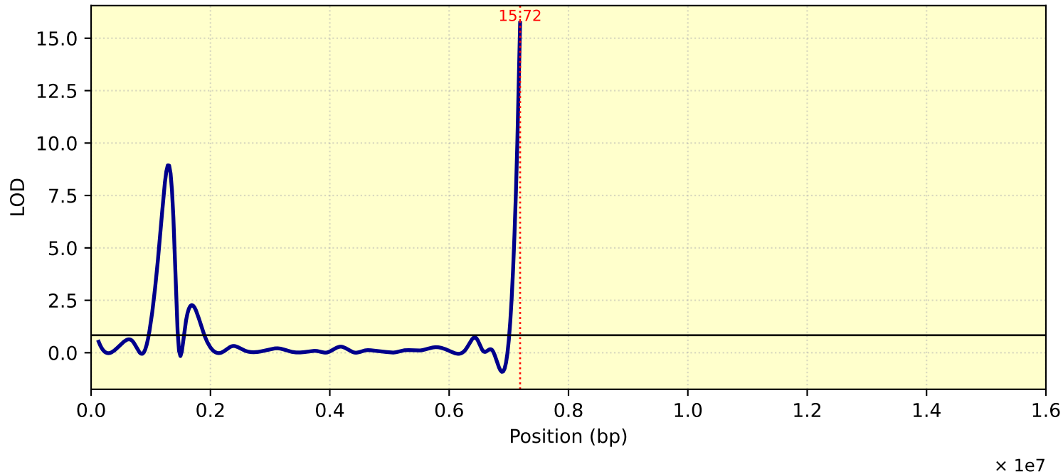
LOD Curve - chr10 - Tc27di11me15
