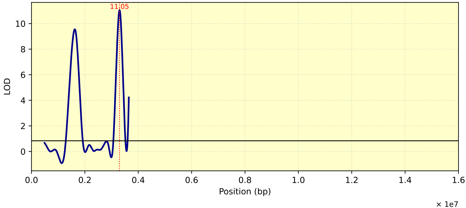
LOD Curve - chr24 - Tc27di11me15
