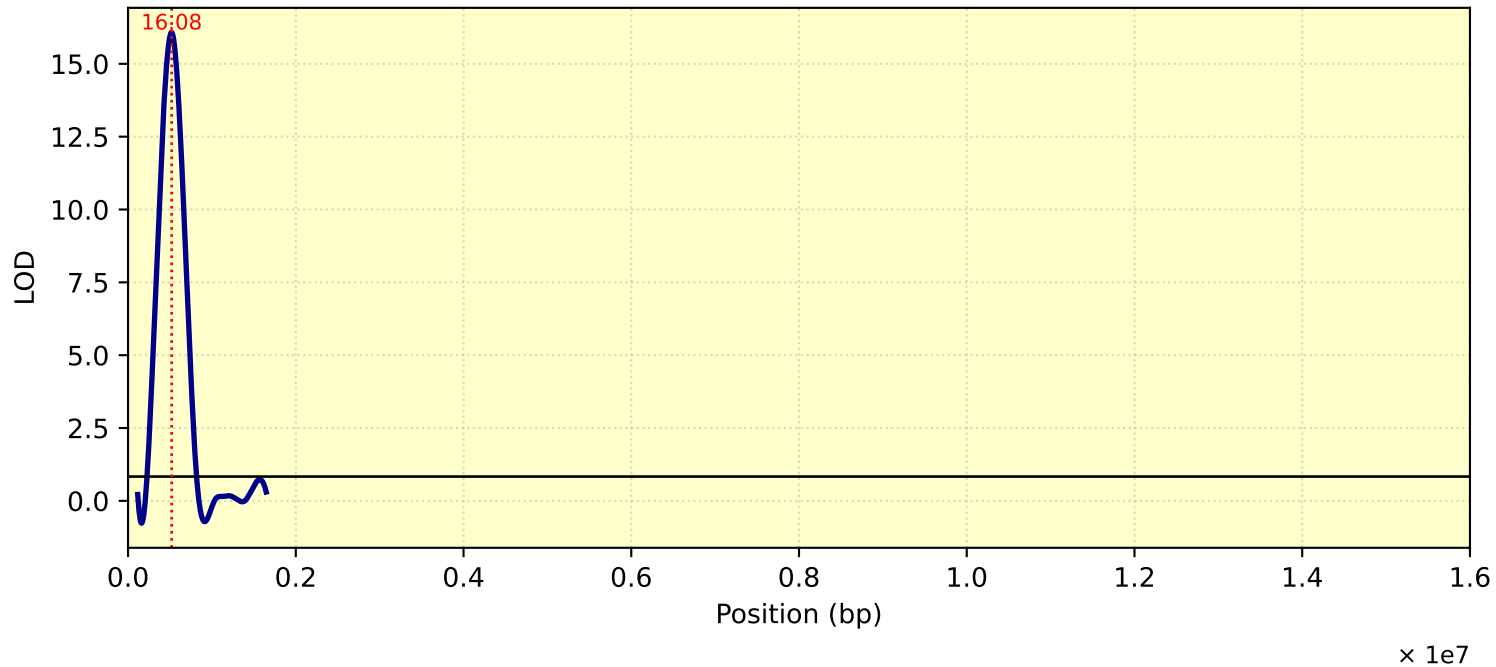
LOD Curve - chr26 - Tc27di11me15
