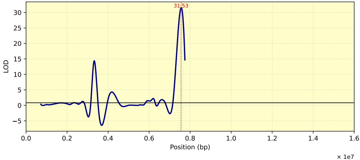
LOD Curve - chr08 - Tc27di11me15
