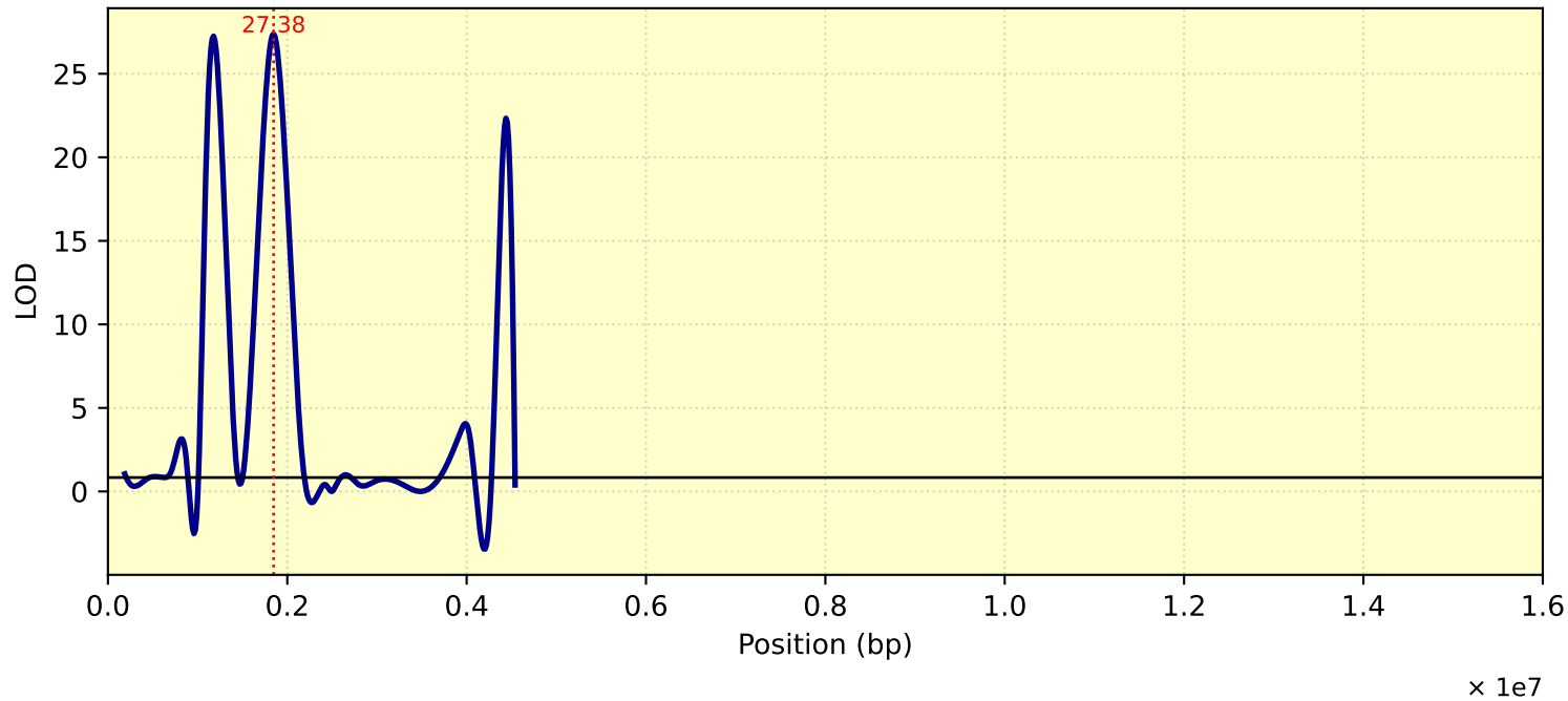
LOD Curve - chr19 - Tc27di11me15
