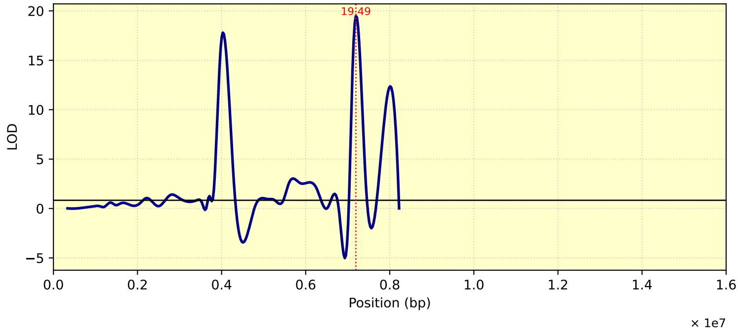
LOD Curve - chr07 - Tc28D1T
