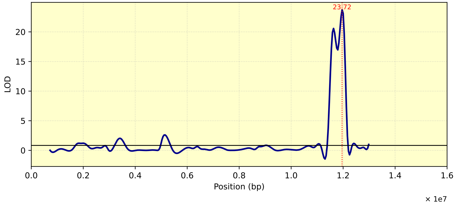
LOD Curve - chr09 - Tc28D1T
