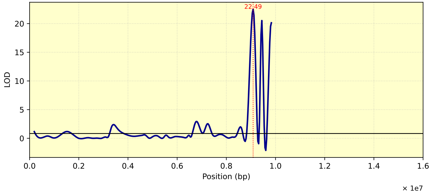
LOD Curve - chr06 - Tc28D1T
