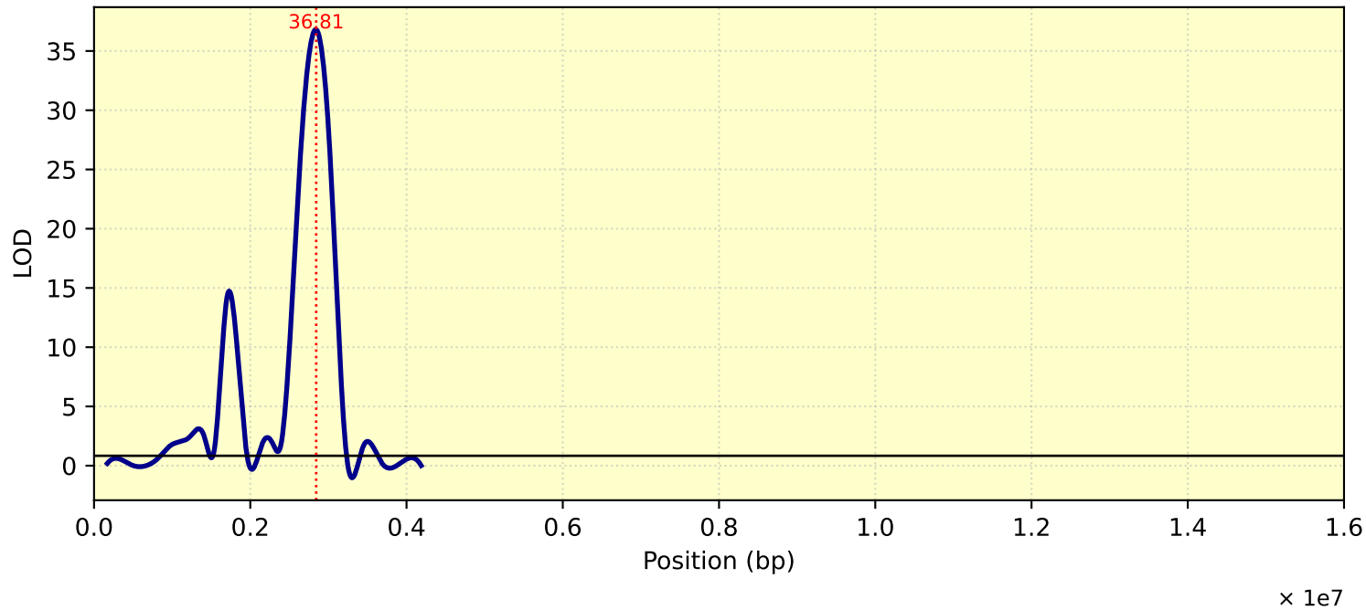
LOD Curve - chr16 - Tc28D1T
