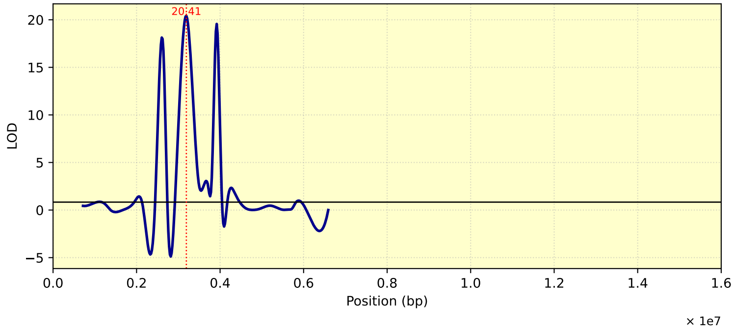
LOD Curve - chr13 - Tc28D1T
