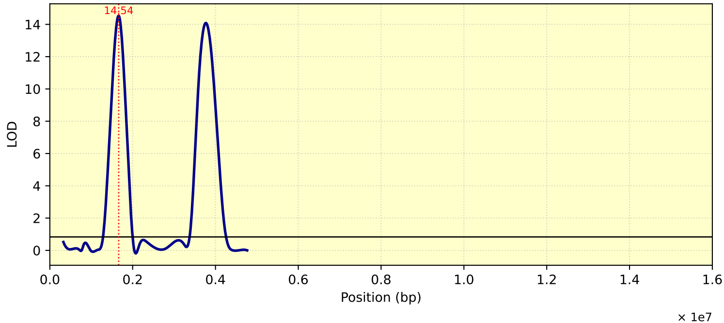
LOD Curve - chr17 - Tc28D1T
