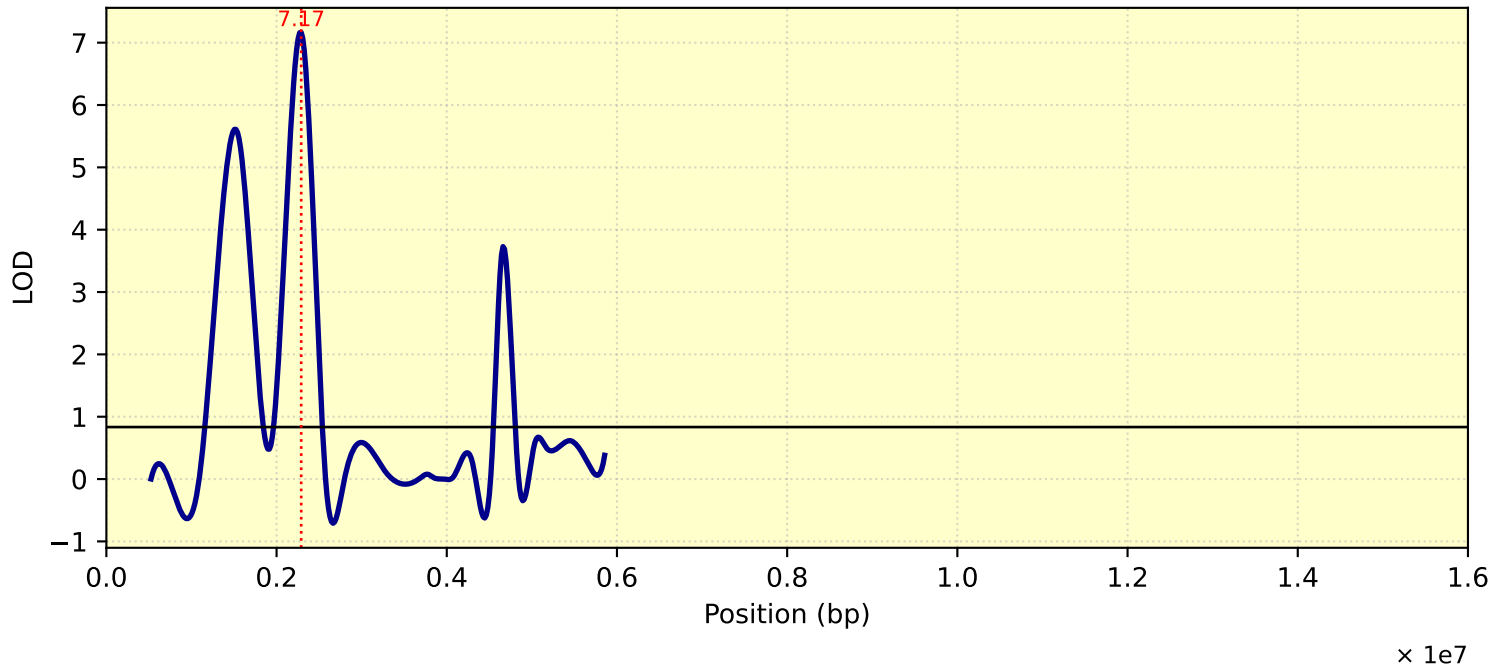
LOD Curve - chr18 - Tc28D1T
