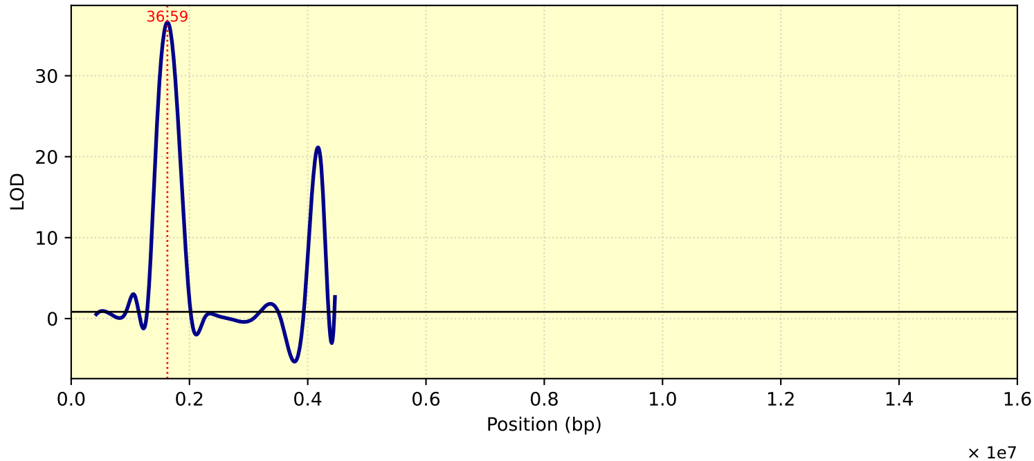
LOD Curve - chr22 - Tc28D1T
