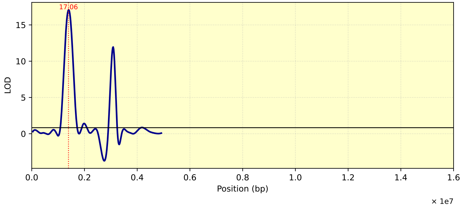
LOD Curve - chr12 - Tc28D1T
