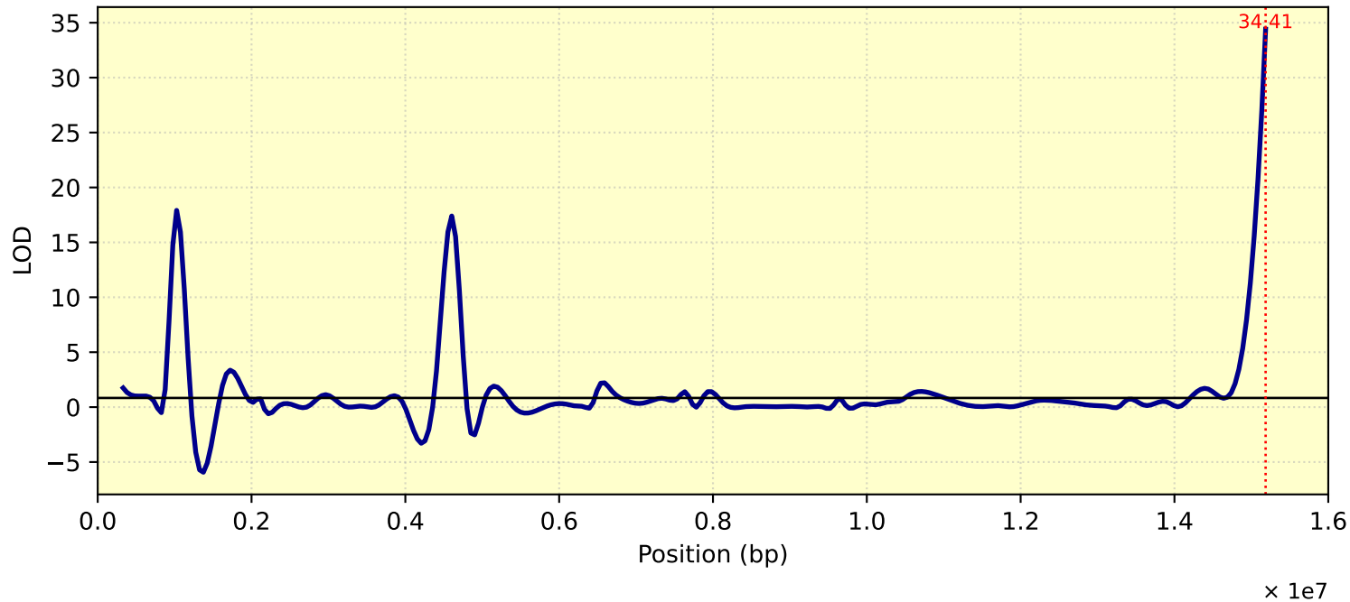
LOD Curve - chr01 - Tc28D1T
