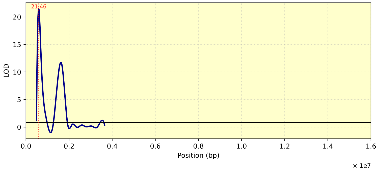
LOD Curve - chr24 - Tc28D1T
