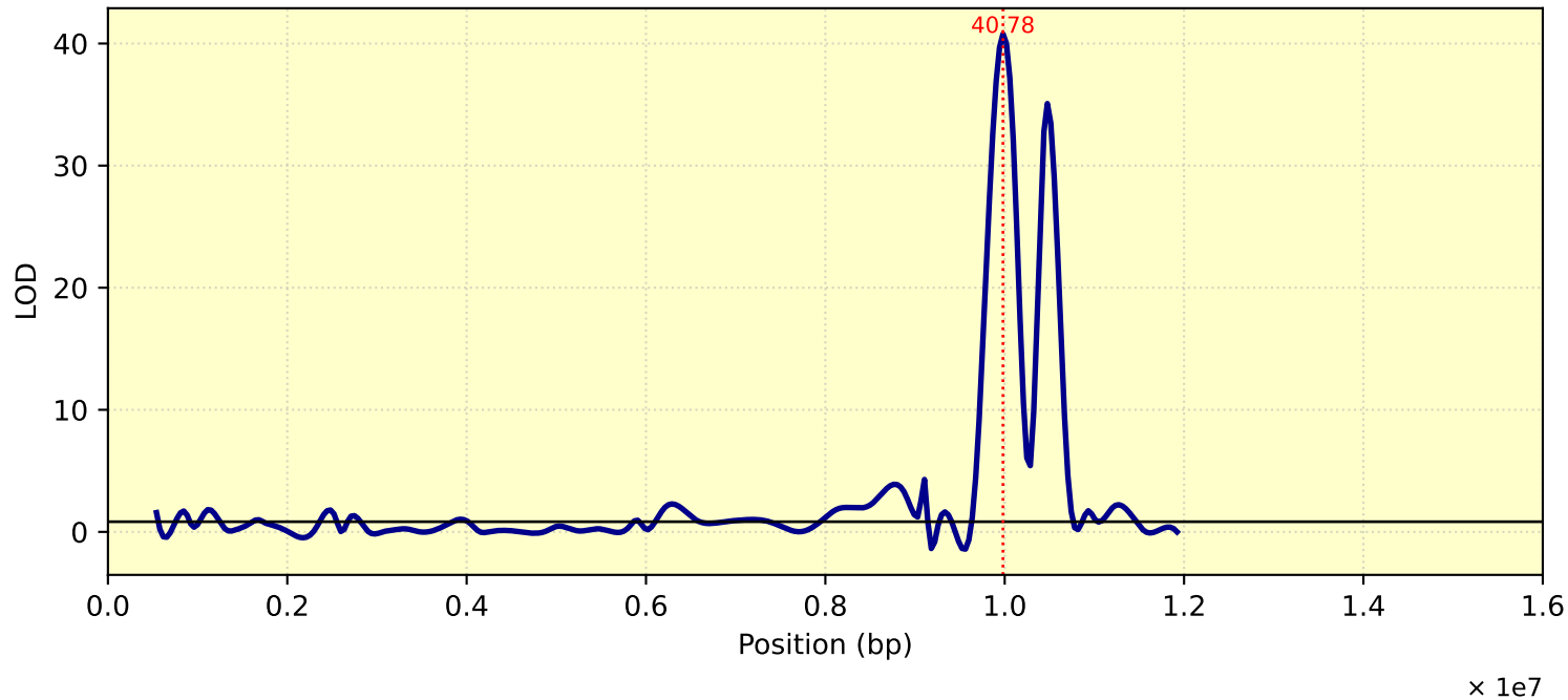
LOD Curve - chr05 - Tc28D1T
