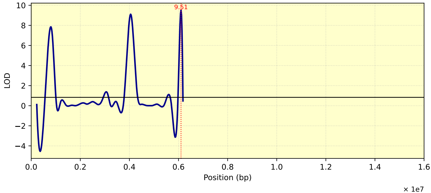
LOD Curve - chr11 - Tc28D1T
