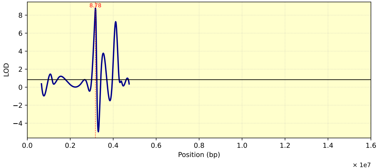
LOD Curve - chr21 - Tc28D1T
