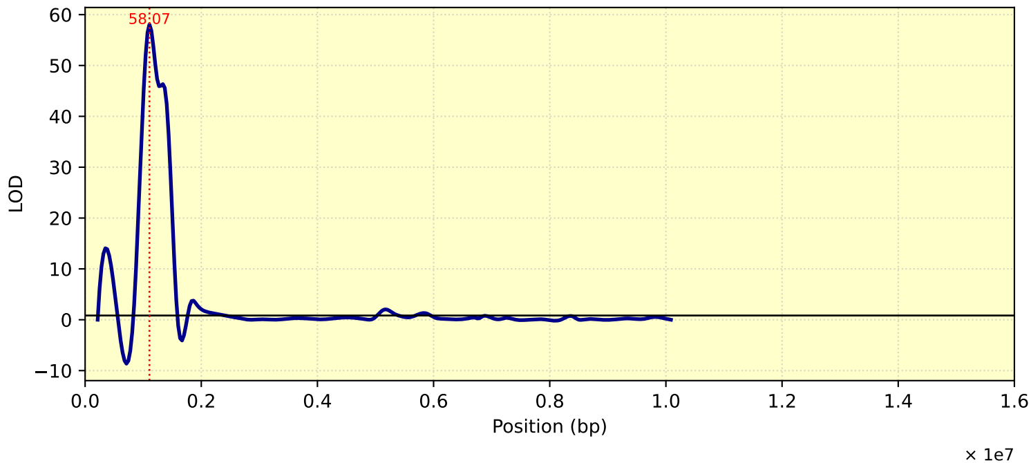
LOD Curve - chr04 - Tc28D1T
