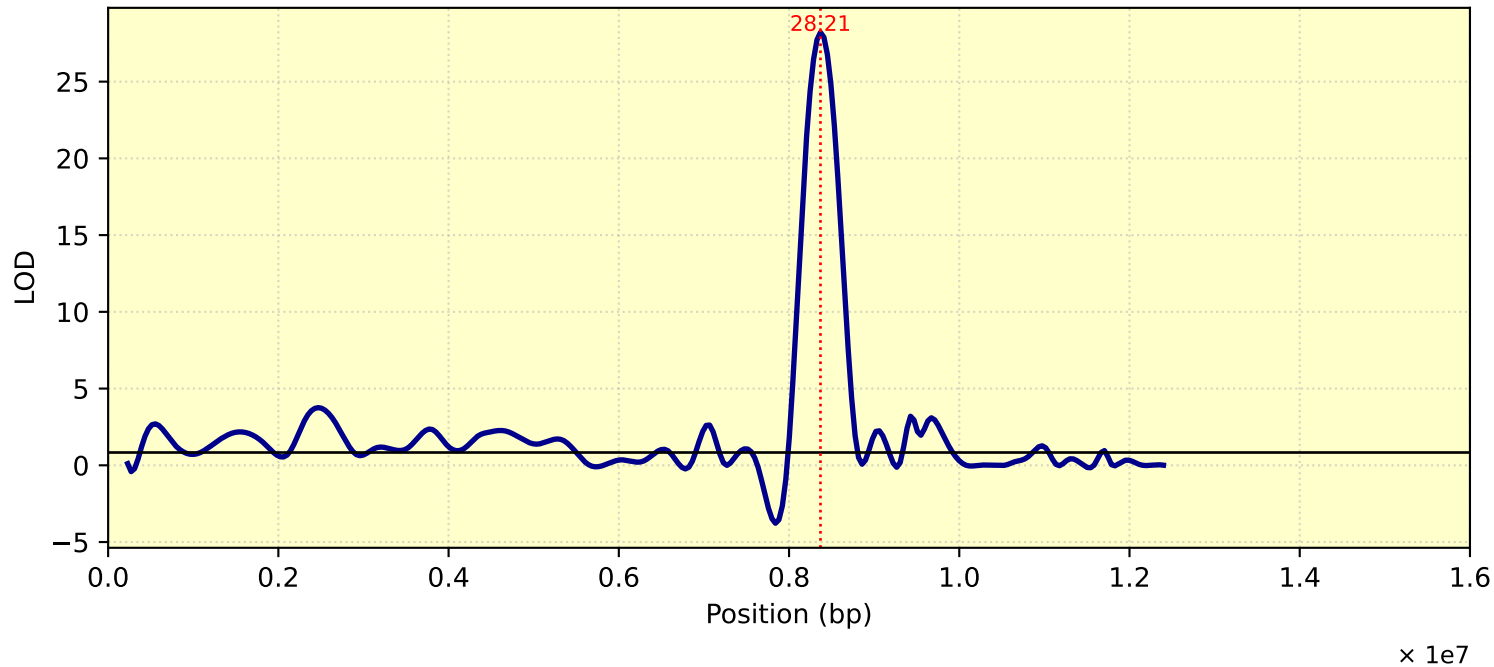
LOD Curve - chr03 - Tc28D1T
