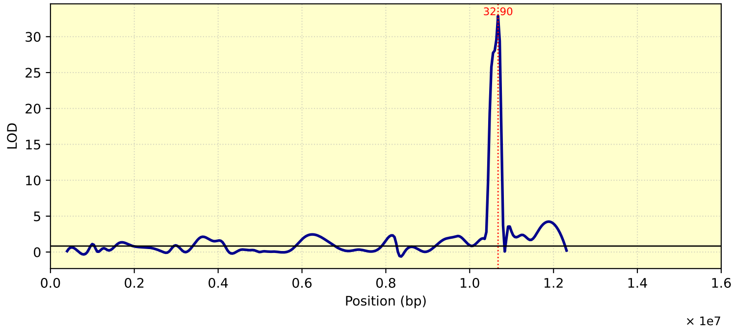
LOD Curve - chr02 - Tc28D1T
