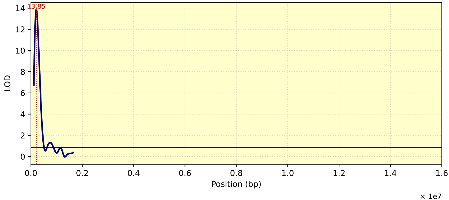
LOD Curve - chr26 - Tc28D1T
