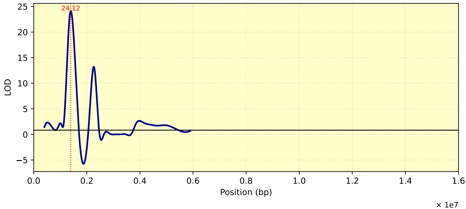
LOD Curve - chr14 - Tc28D1T
