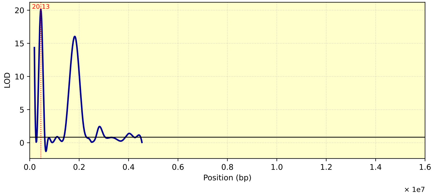
LOD Curve - chr19 - Tc28D1T
