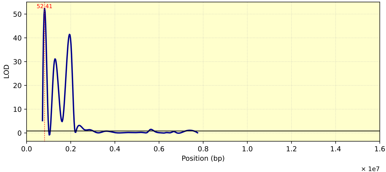
LOD Curve - chr08 - Tc28D1T
