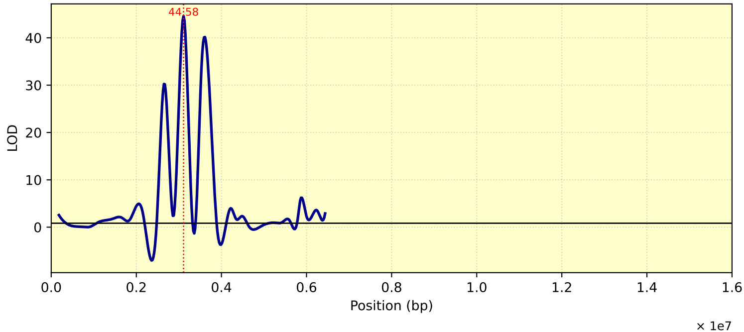
LOD Curve - chr15 - Tc28D1T
