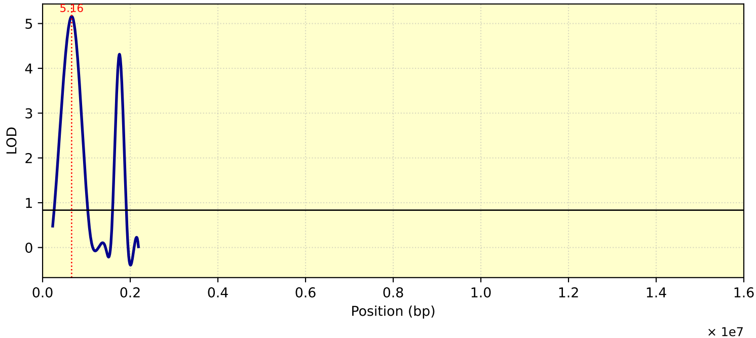
LOD Curve - chr23 - Tc28D1T
