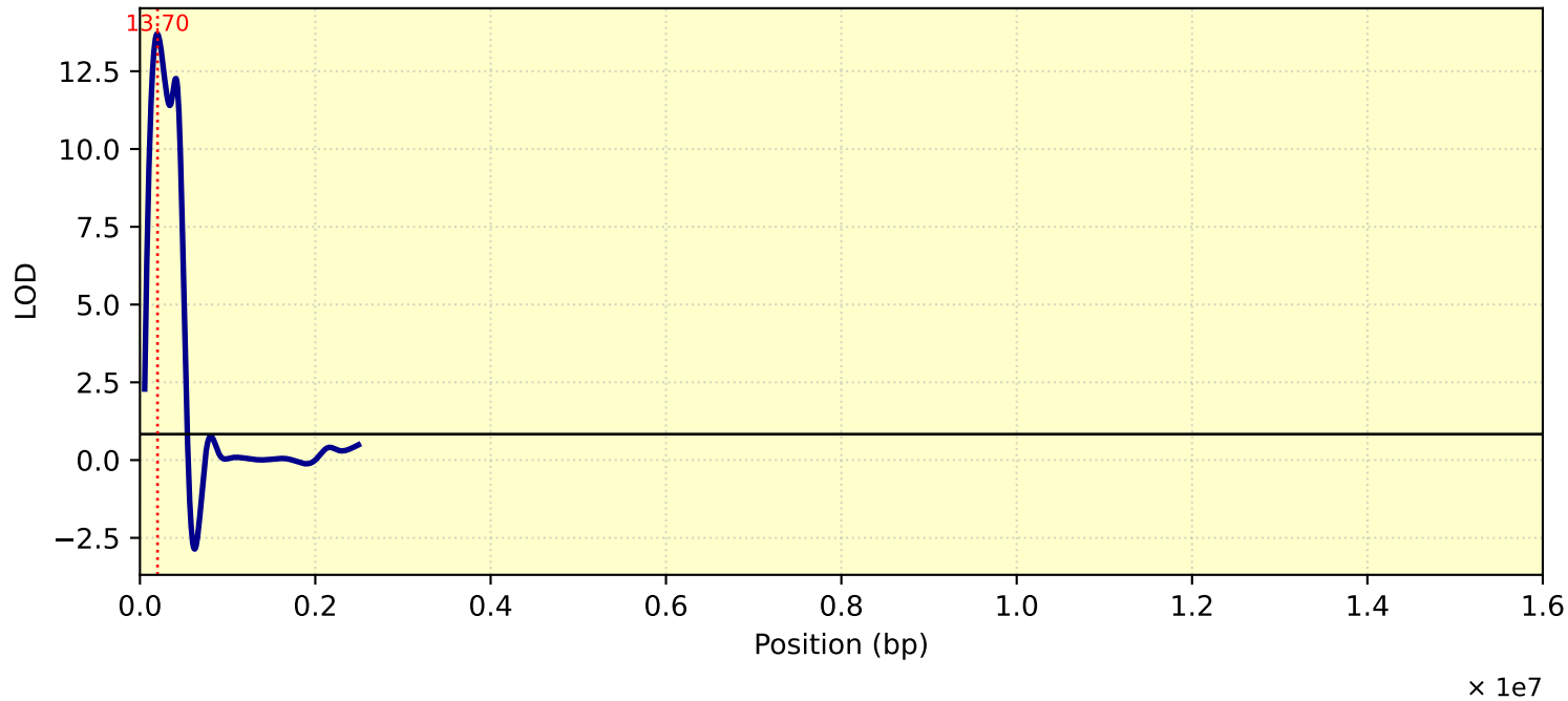
LOD Curve - chr25 - Tc28D1T
