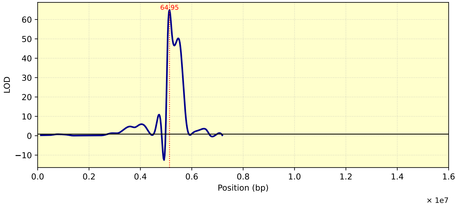
LOD Curve - chr10 - Tc28D1T
