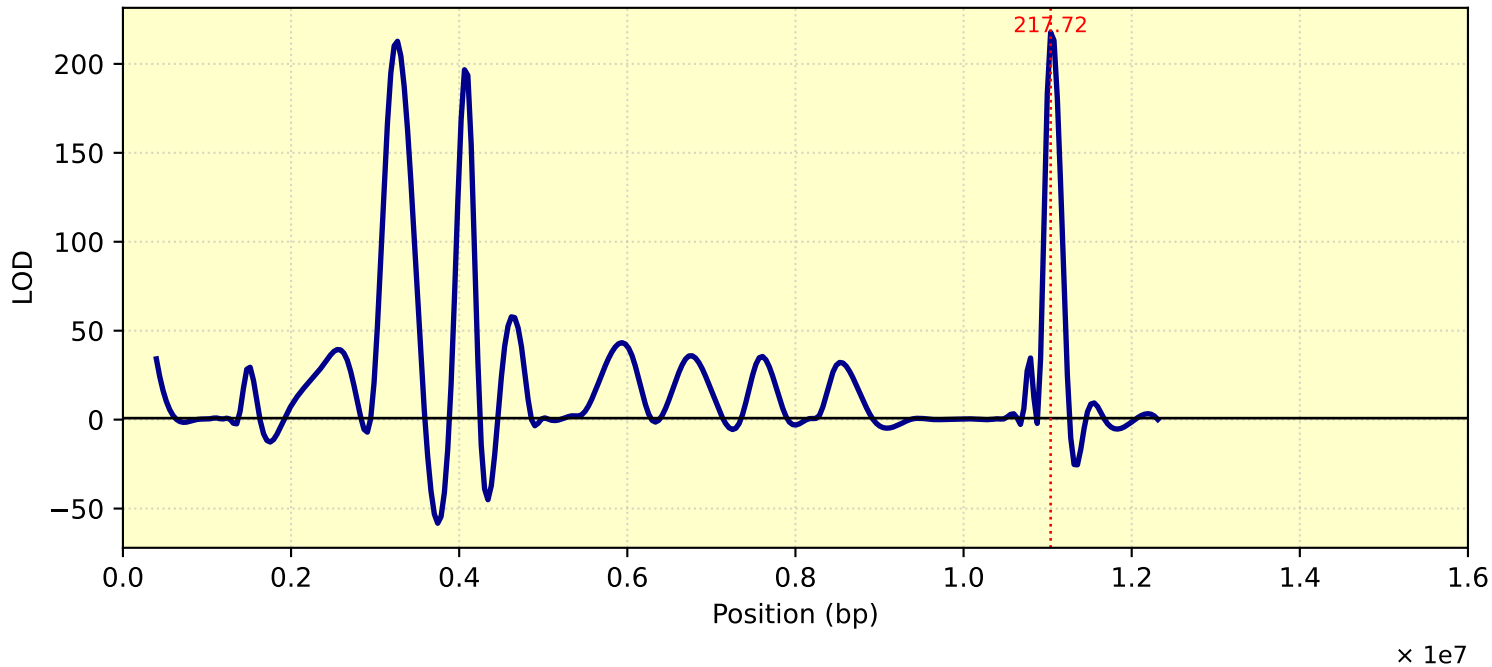
LOD Curve - chr02 - Tc28Me2T1
