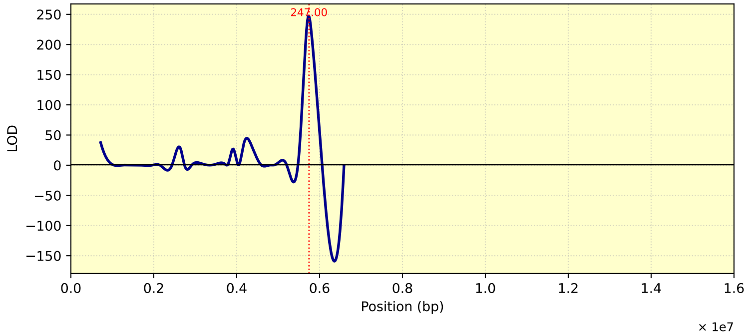
LOD Curve - chr13 - Tc28Me2T1
