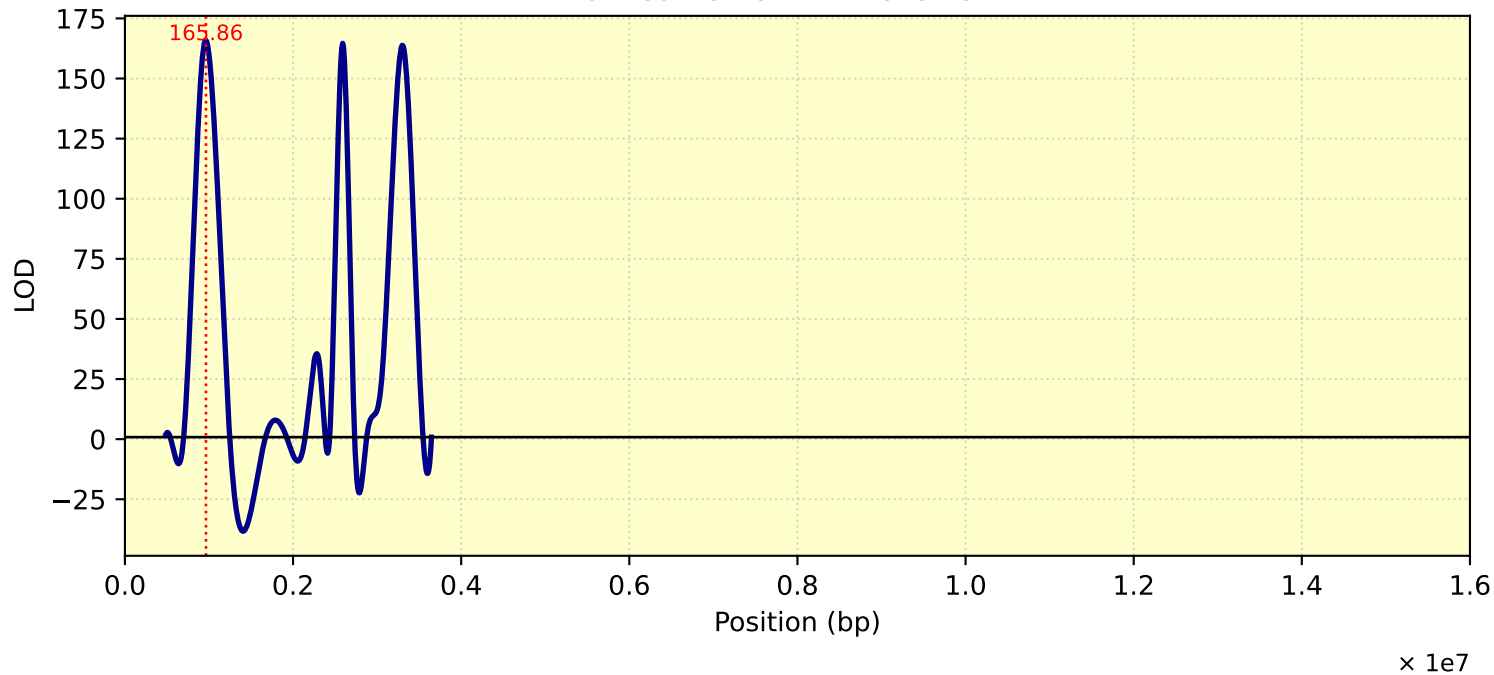
LOD Curve - chr24 - Tc28Me2T1
