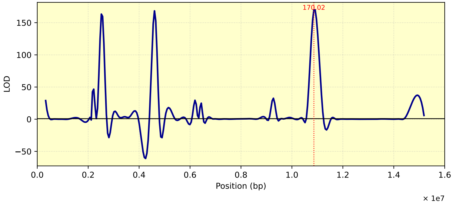
LOD Curve - chr01 - Tc28Me2T1
