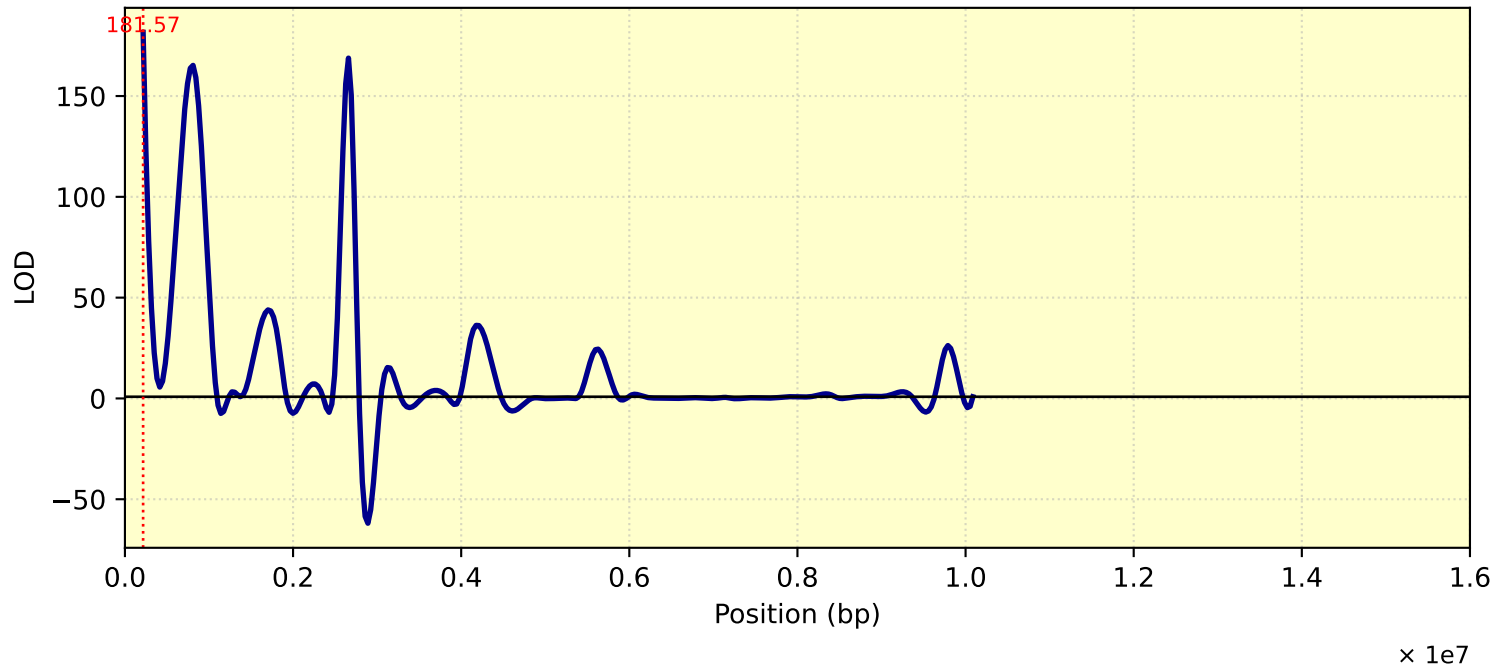
LOD Curve - chr04 - Tc28Me2T1
