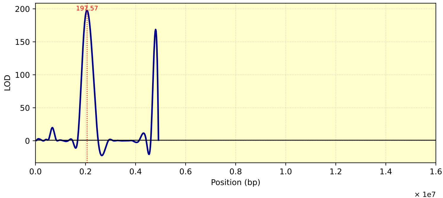
LOD Curve - chr12 - Tc28Me2T1
