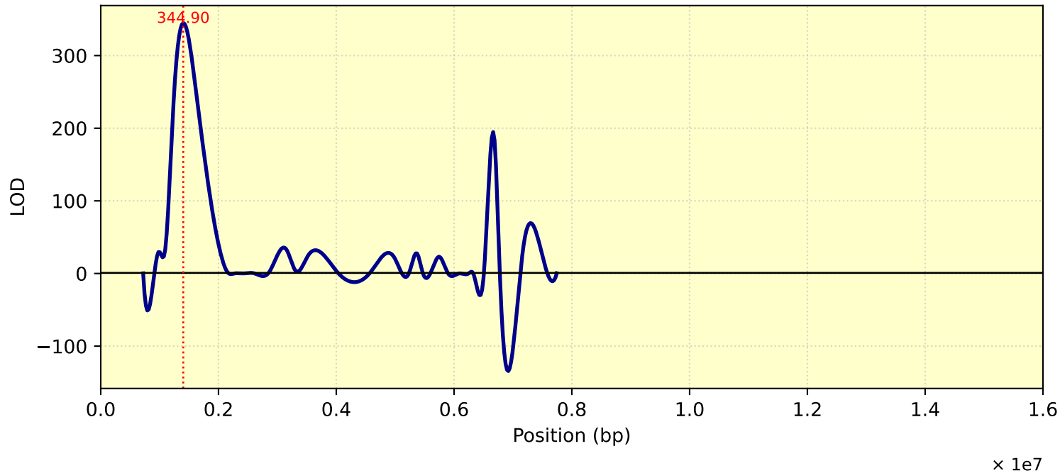
LOD Curve - chr08 - Tc28Me2T1
