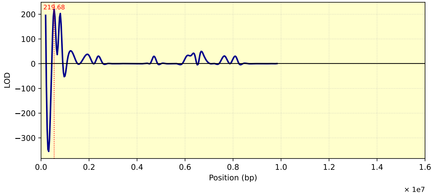
LOD Curve - chr06 - Tc28Me2T1
