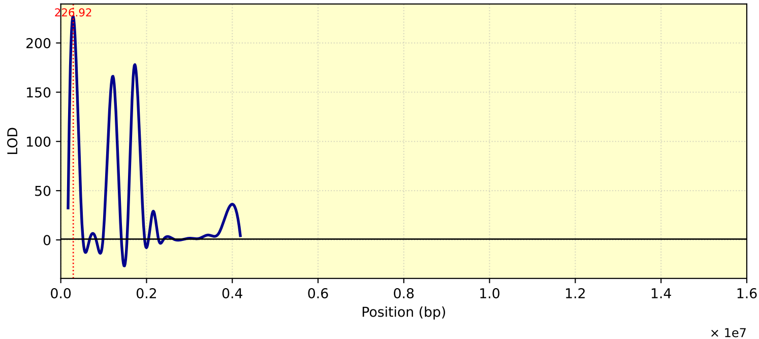
LOD Curve - chr16 - Tc28Me2T1
