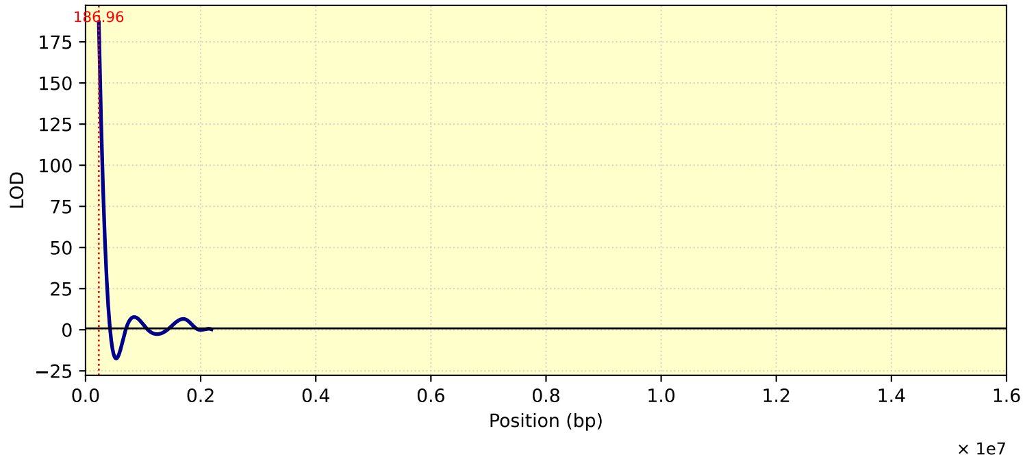
LOD Curve - chr23 - Tc28Me2T1
