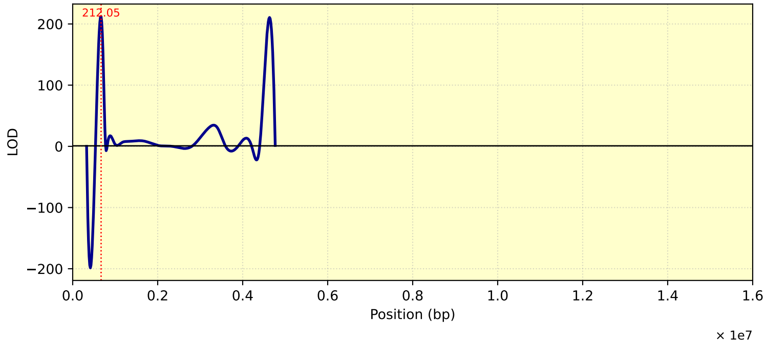
LOD Curve - chr17 - Tc28Me2T1
