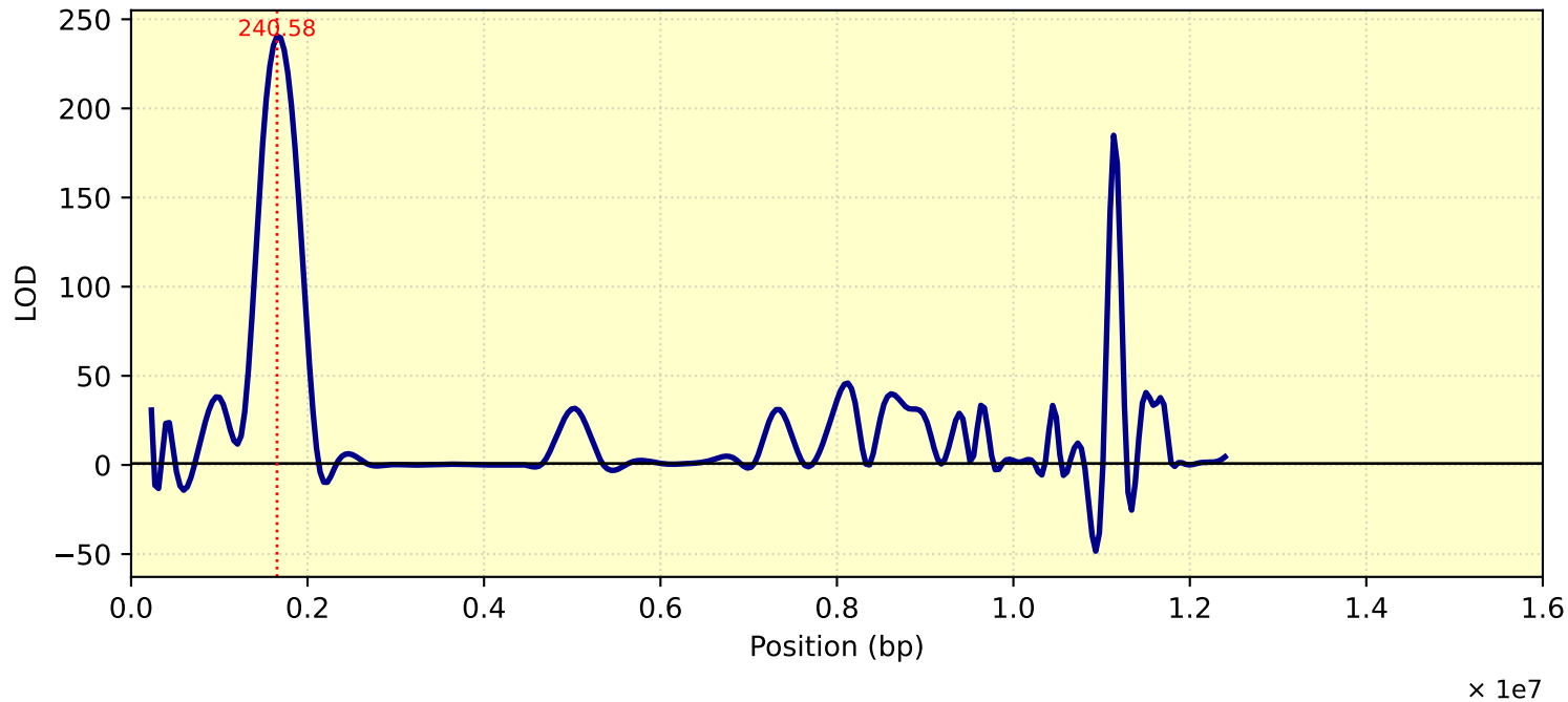
LOD Curve - chr03 - Tc28Me2T1
