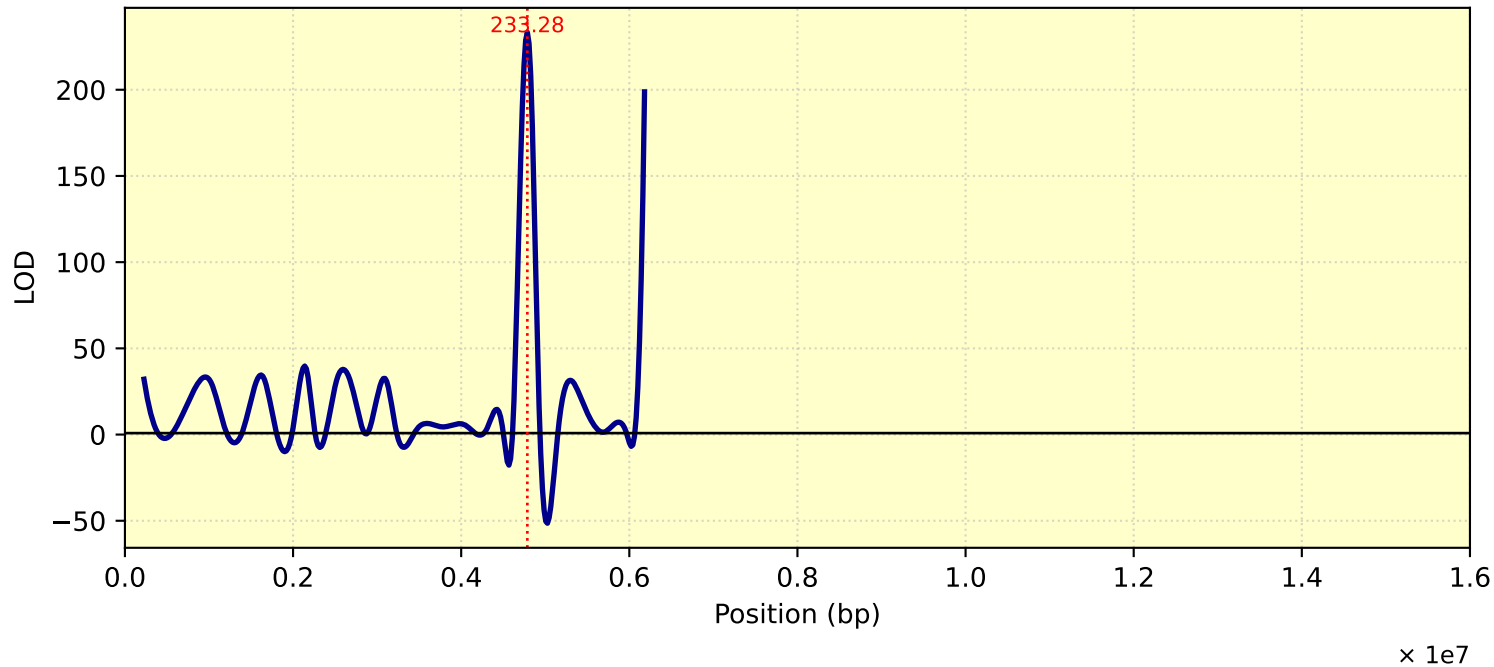
LOD Curve - chr11 - Tc28Me2T1
