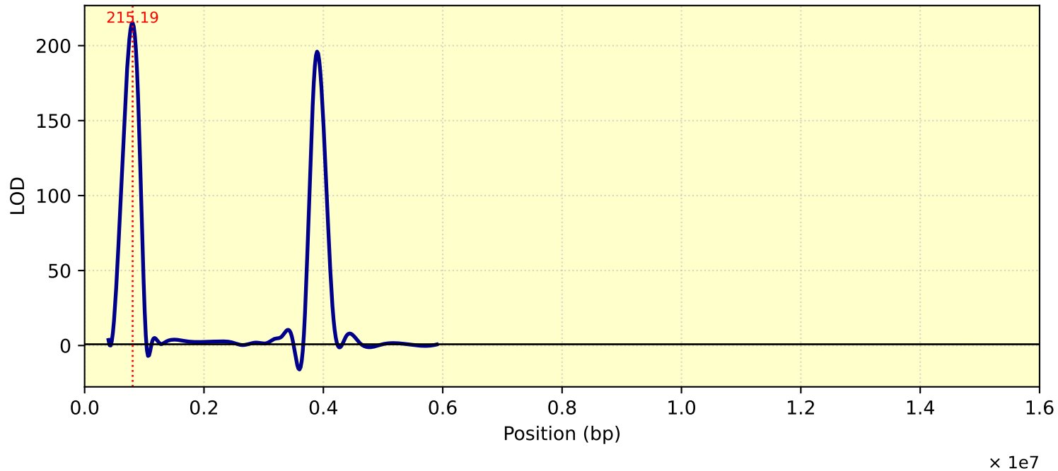
LOD Curve - chr14 - Tc28Me2T1
