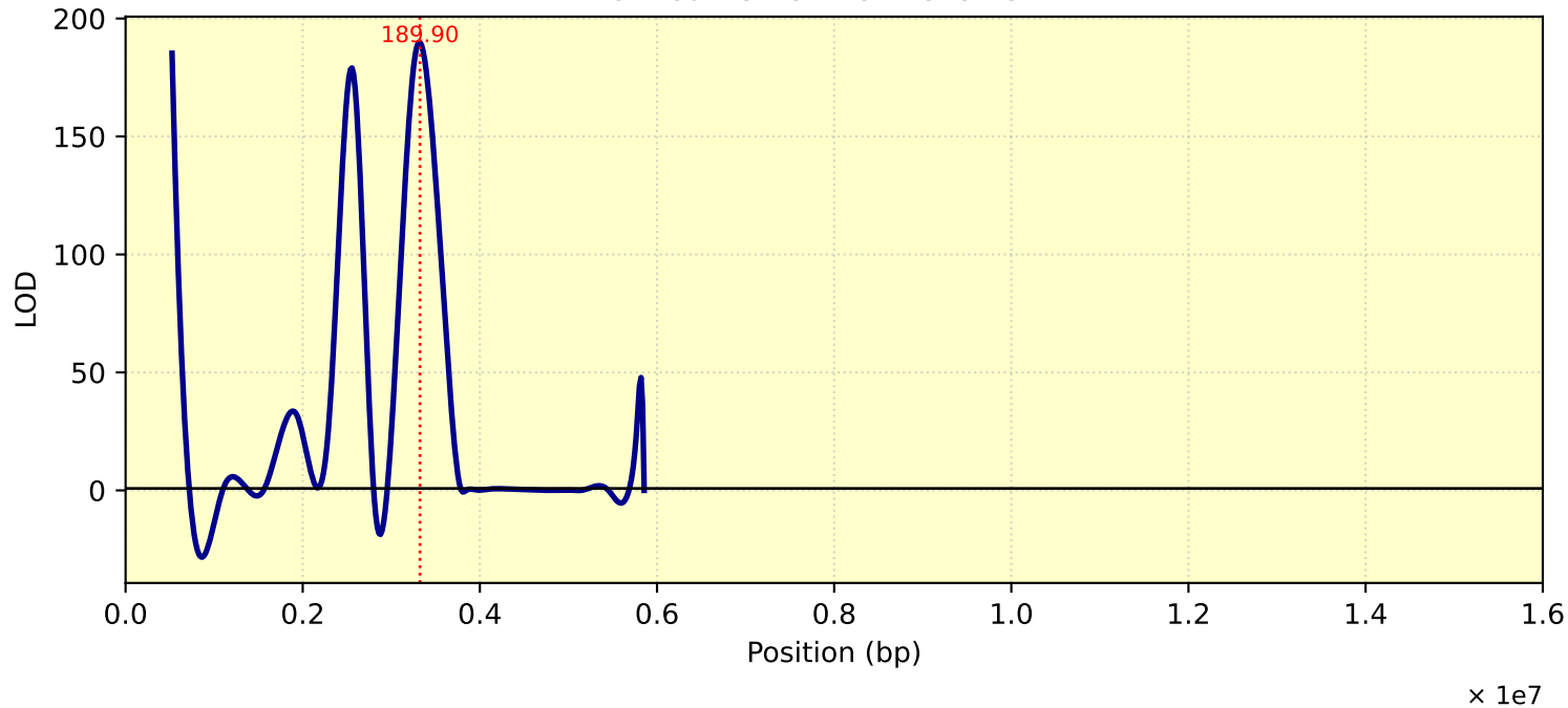
LOD Curve - chr18 - Tc28Me2T1
