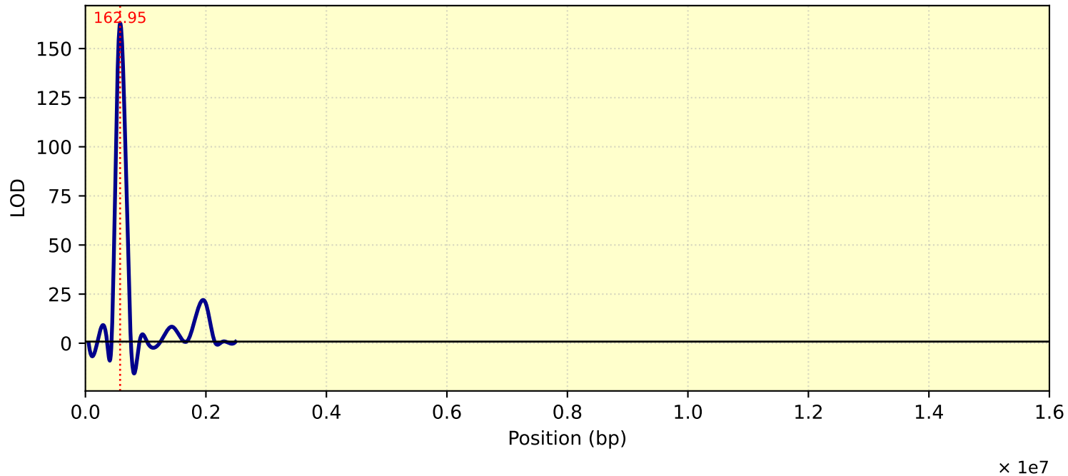
LOD Curve - chr25 - Tc28Me2T1
