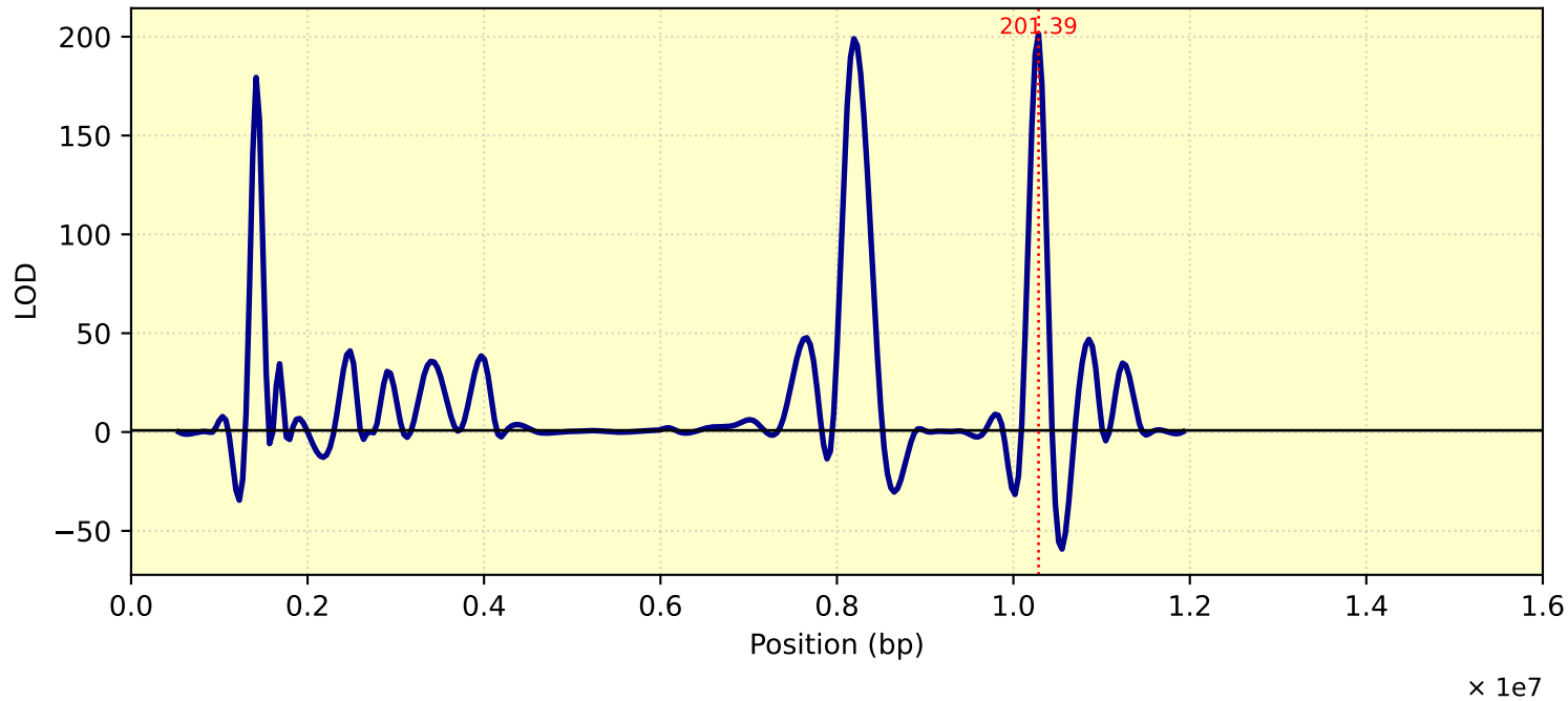
LOD Curve - chr05 - Tc28Me2T1
