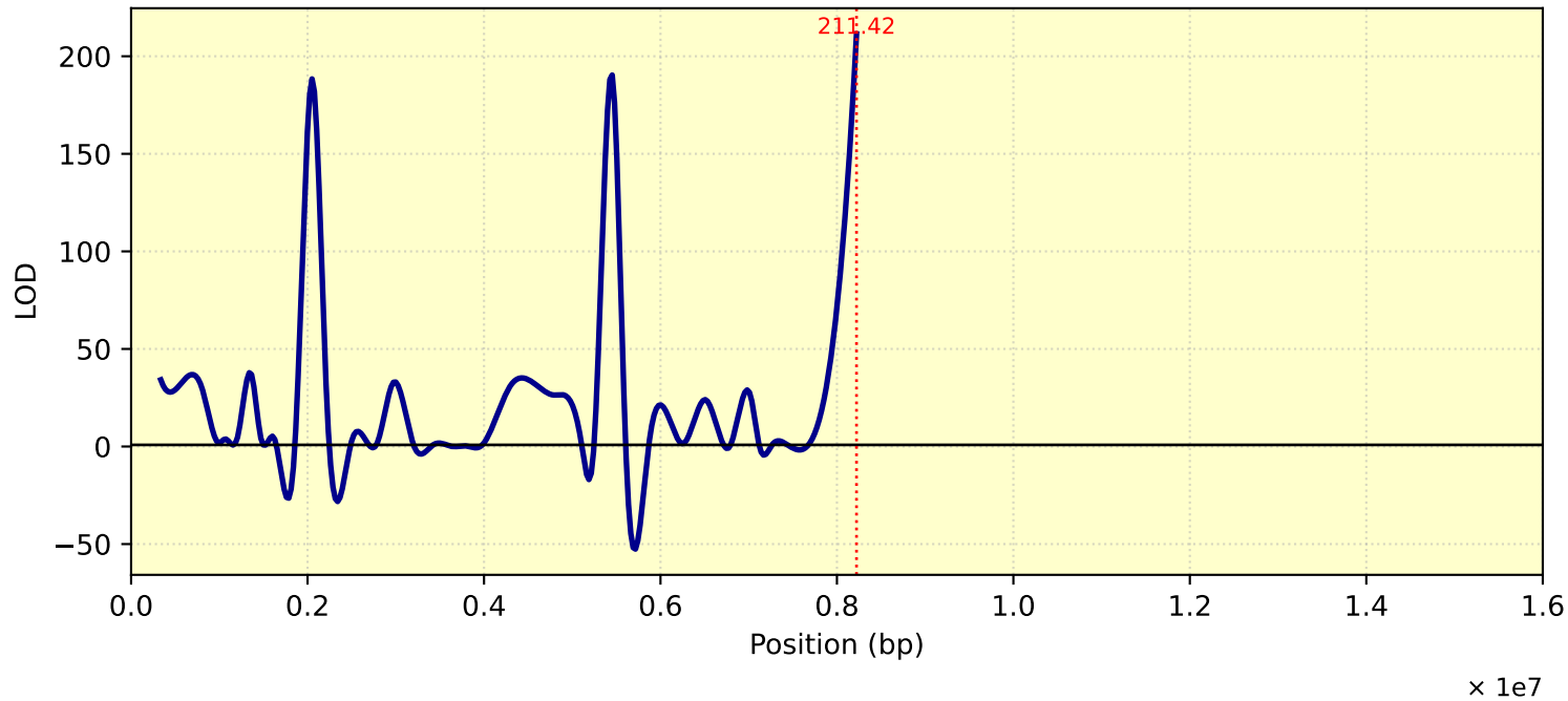
LOD Curve - chr07 - Tc28Me2T1
