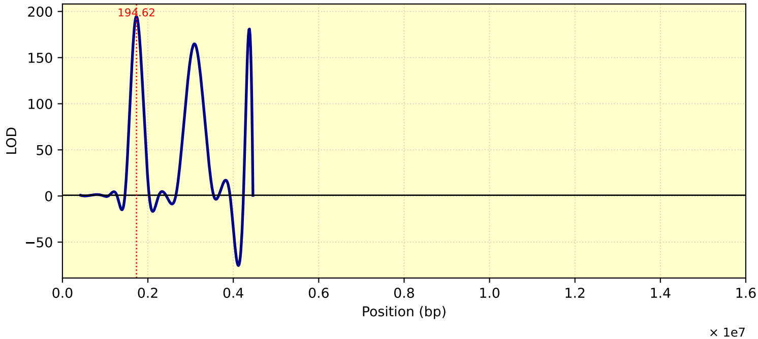
LOD Curve - chr22 - Tc28Me2T1
