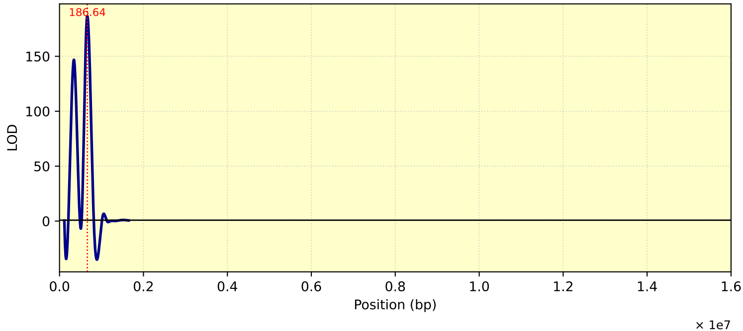
LOD Curve - chr26 - Tc28Me2T1
