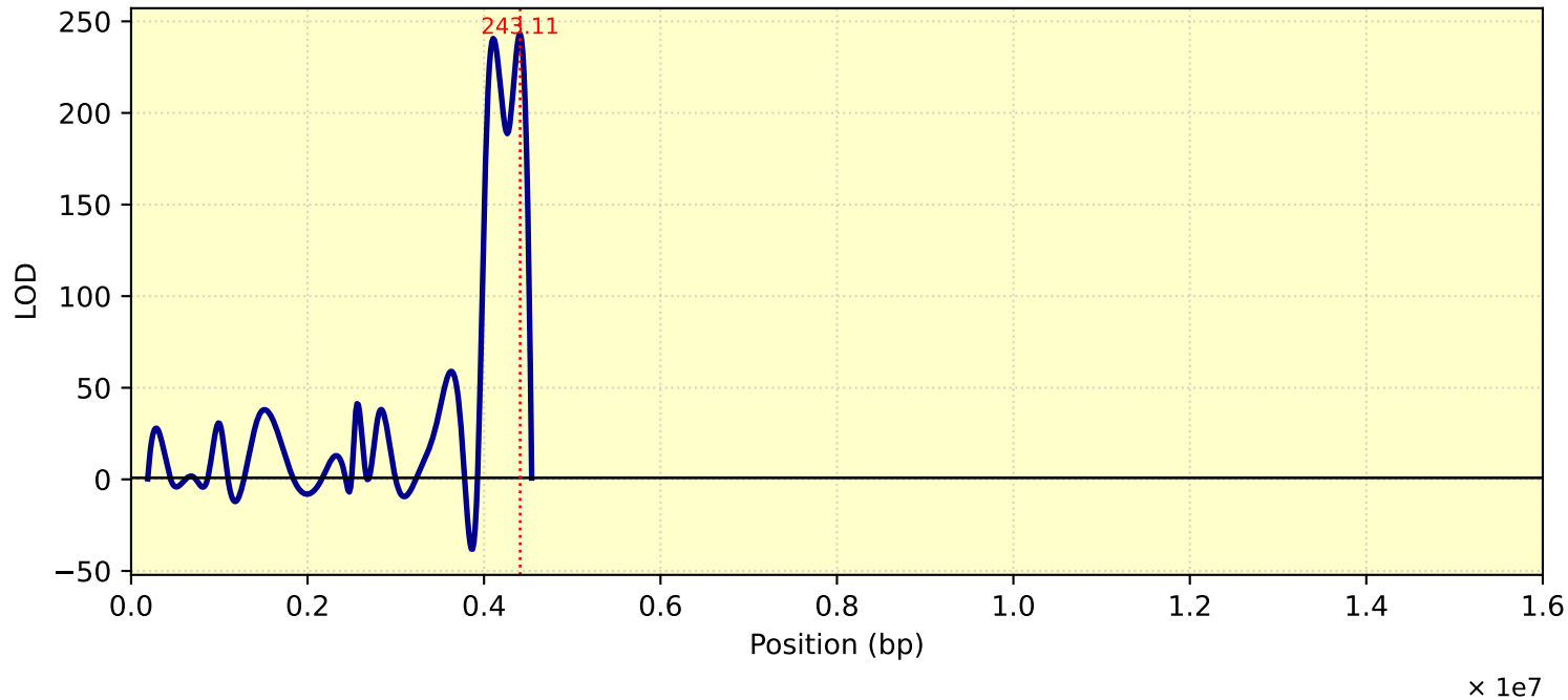
LOD Curve - chr19 - Tc28Me2T1
