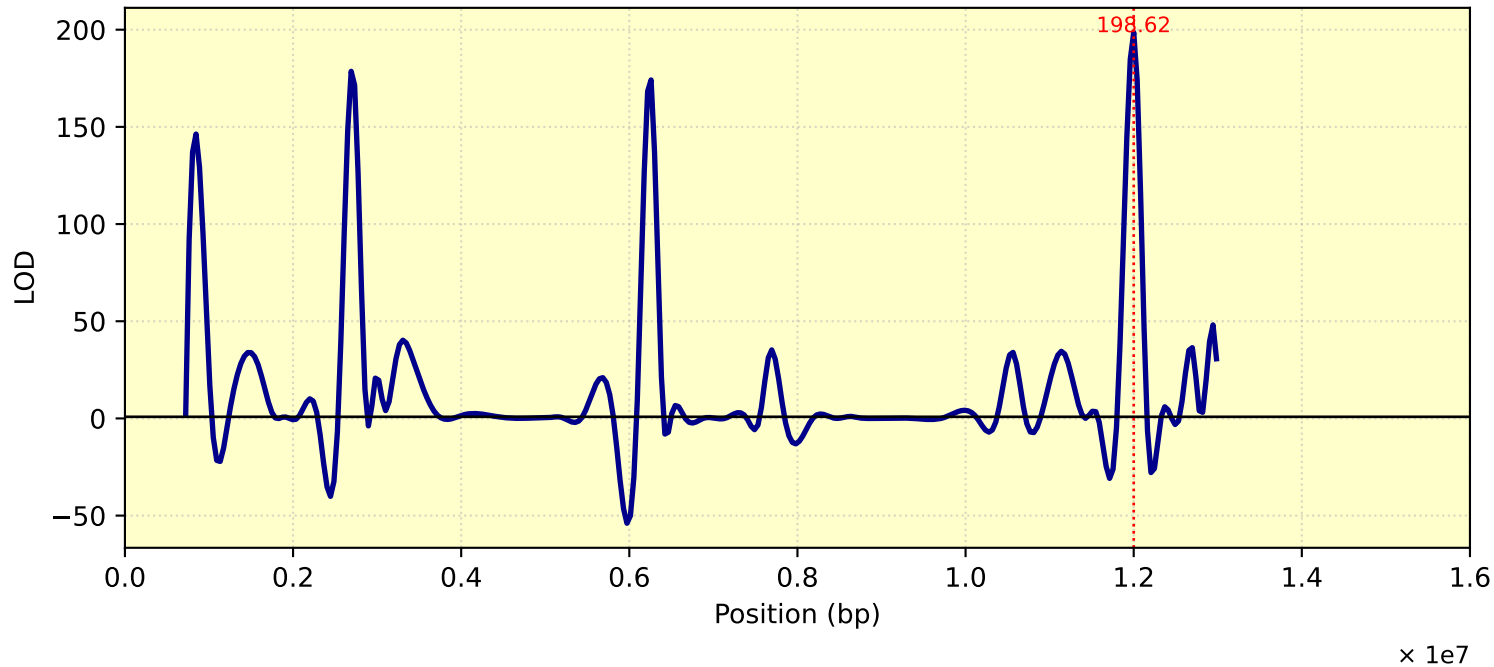
LOD Curve - chr09 - Tc28Me2T1
