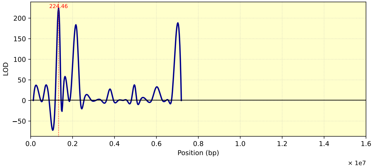
LOD Curve - chr10 - Tc28Me2T1
