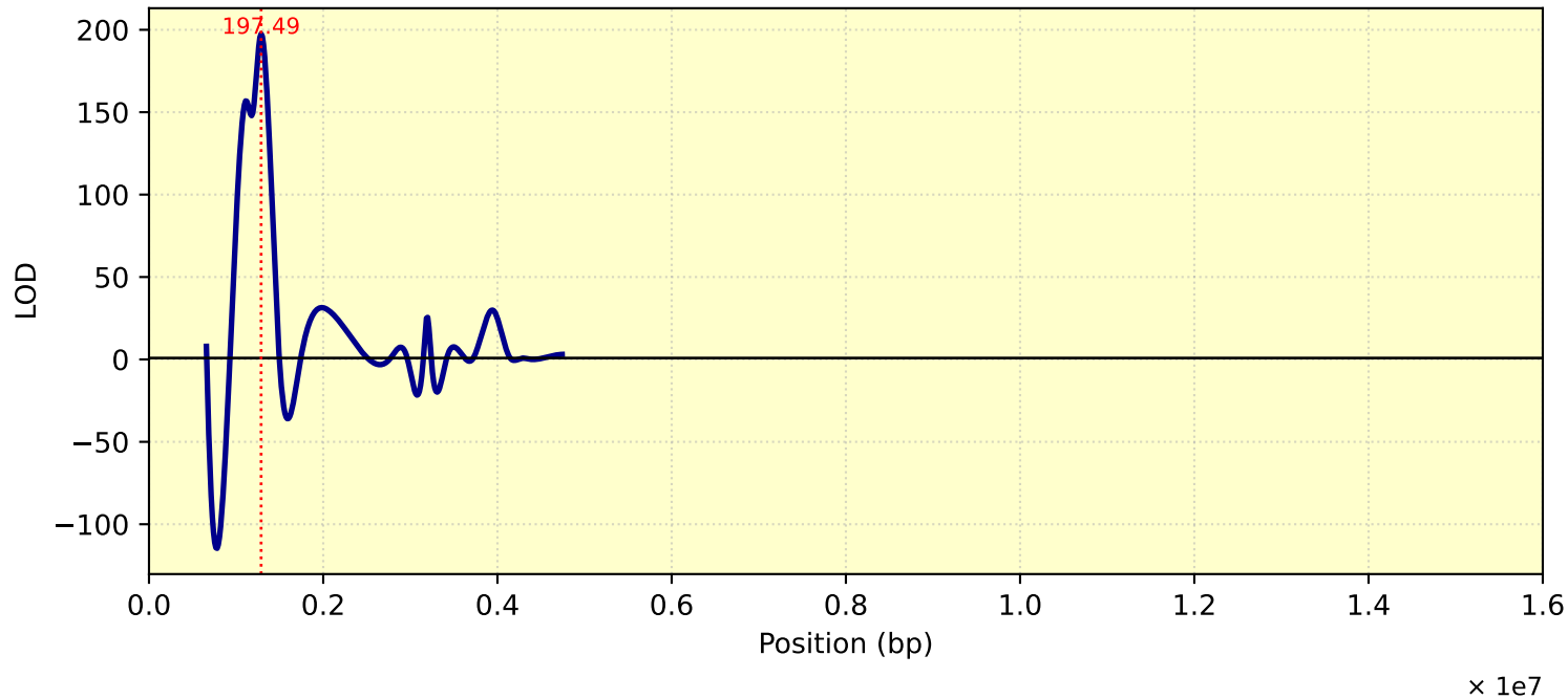
LOD Curve - chr21 - Tc28Me2T1
