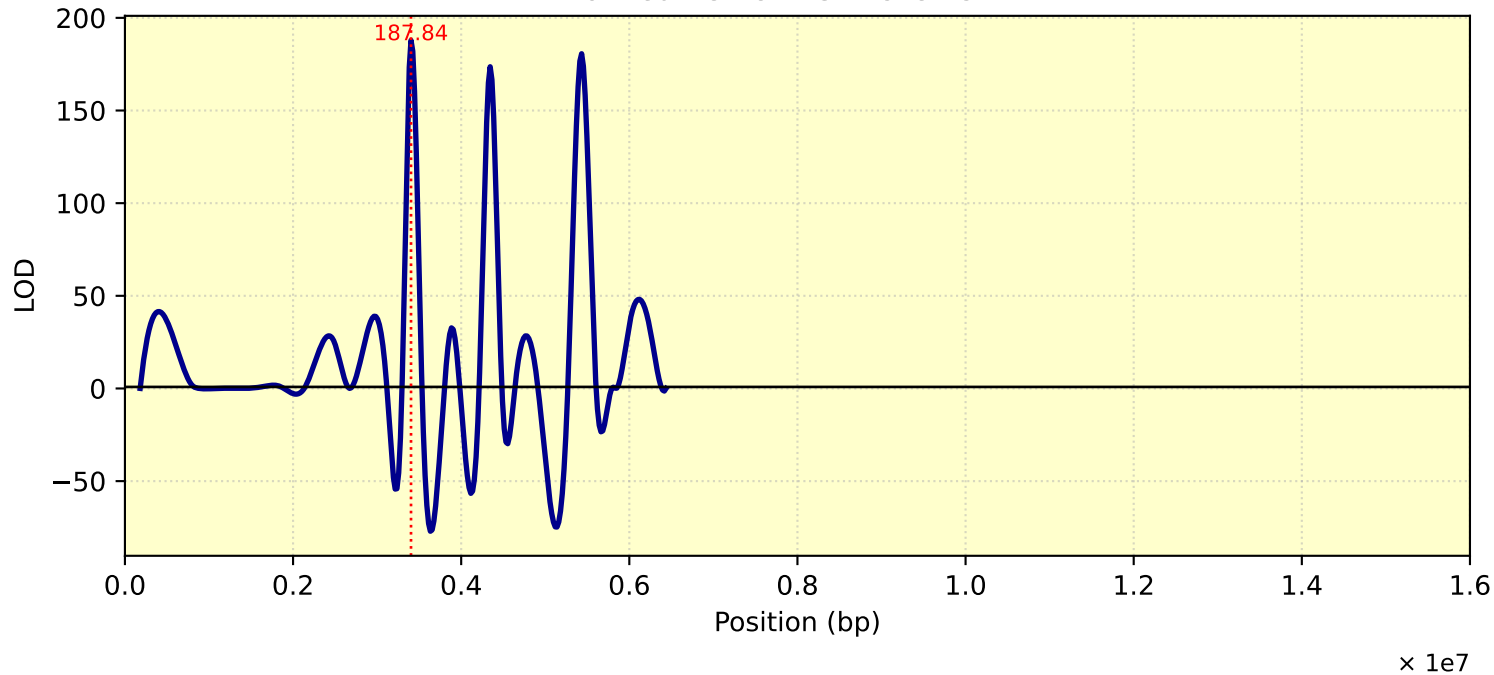
LOD Curve - chr15 - Tc28Me2T1
