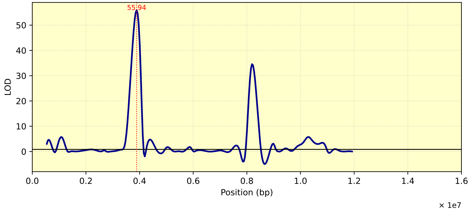
LOD Curve - chr05 - Tc29me3
