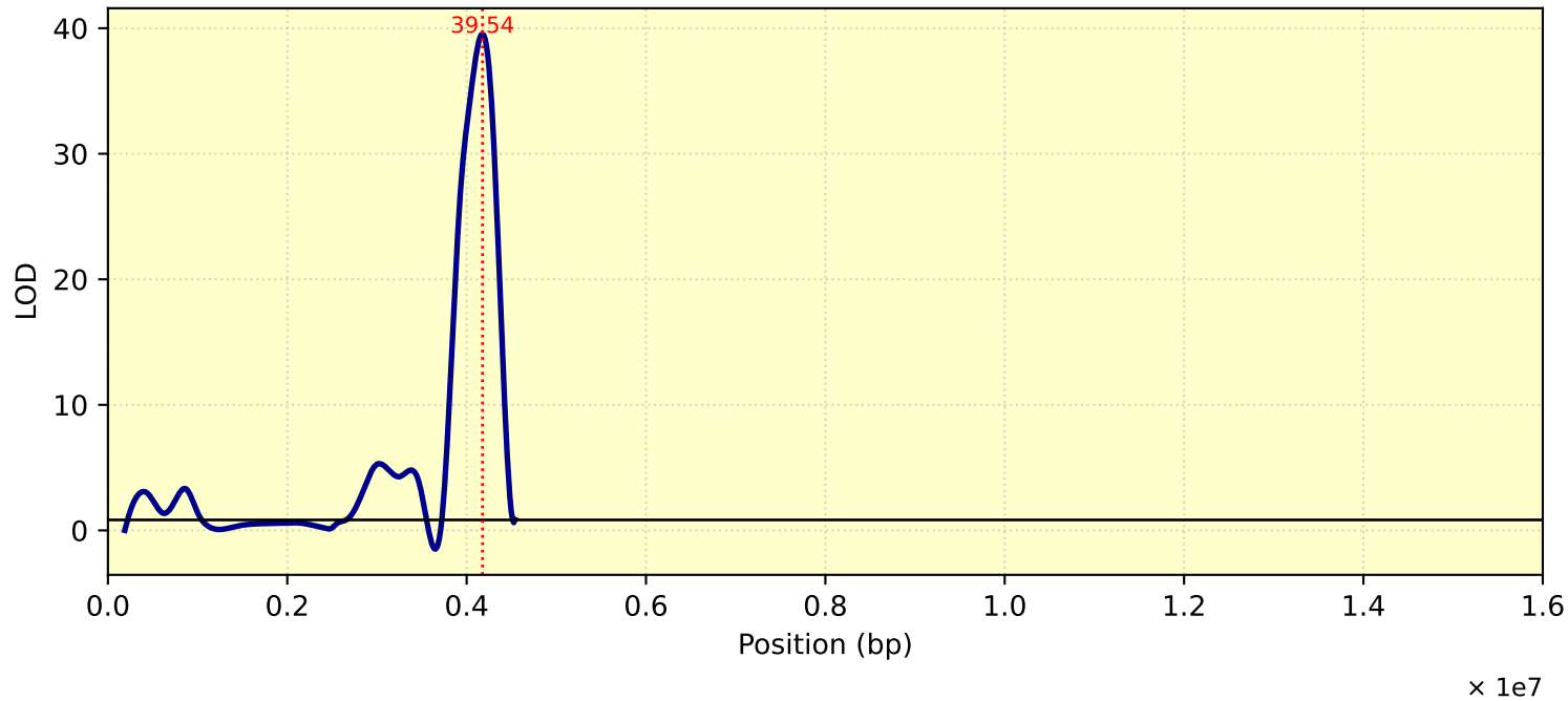
LOD Curve - chr19 - Tc29me3
