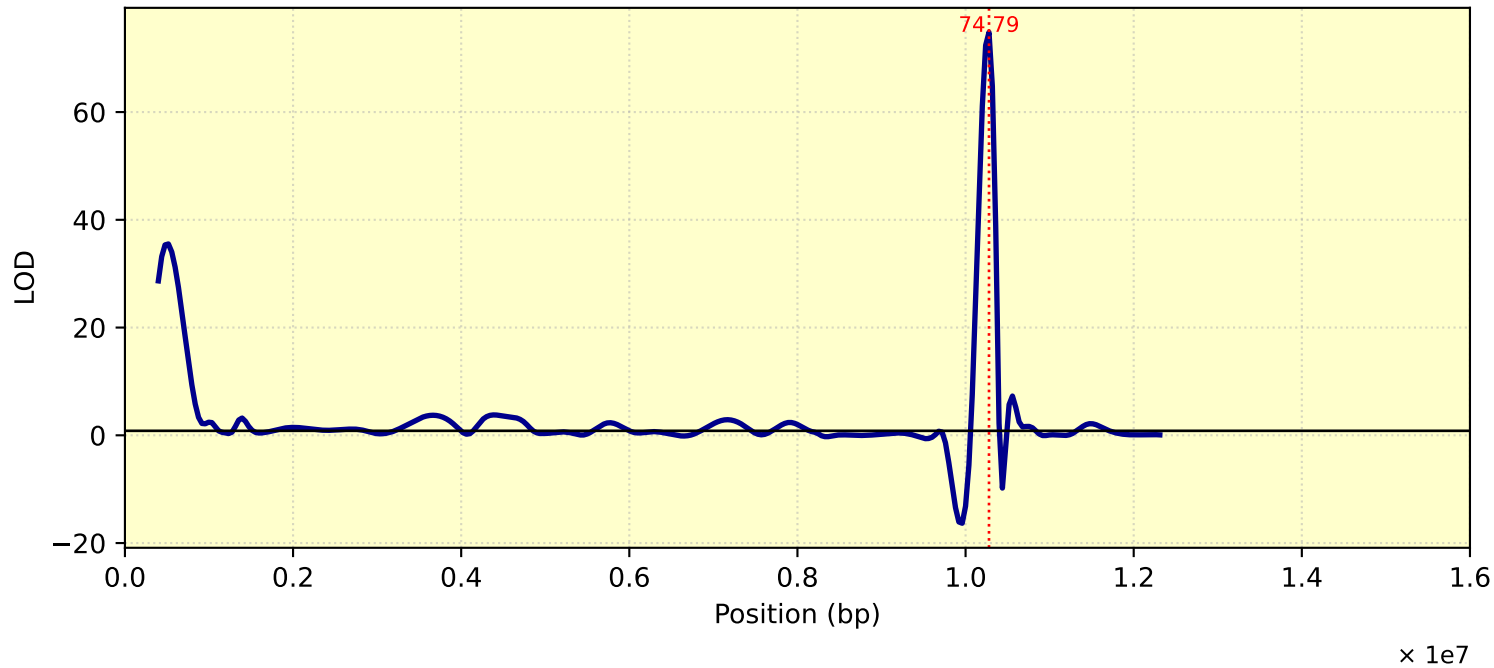
LOD Curve - chr02 - Tc29me3
