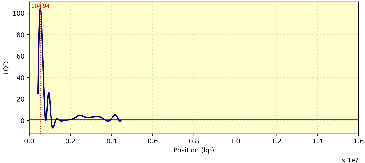
LOD Curve - chr22 - Tc29me3
