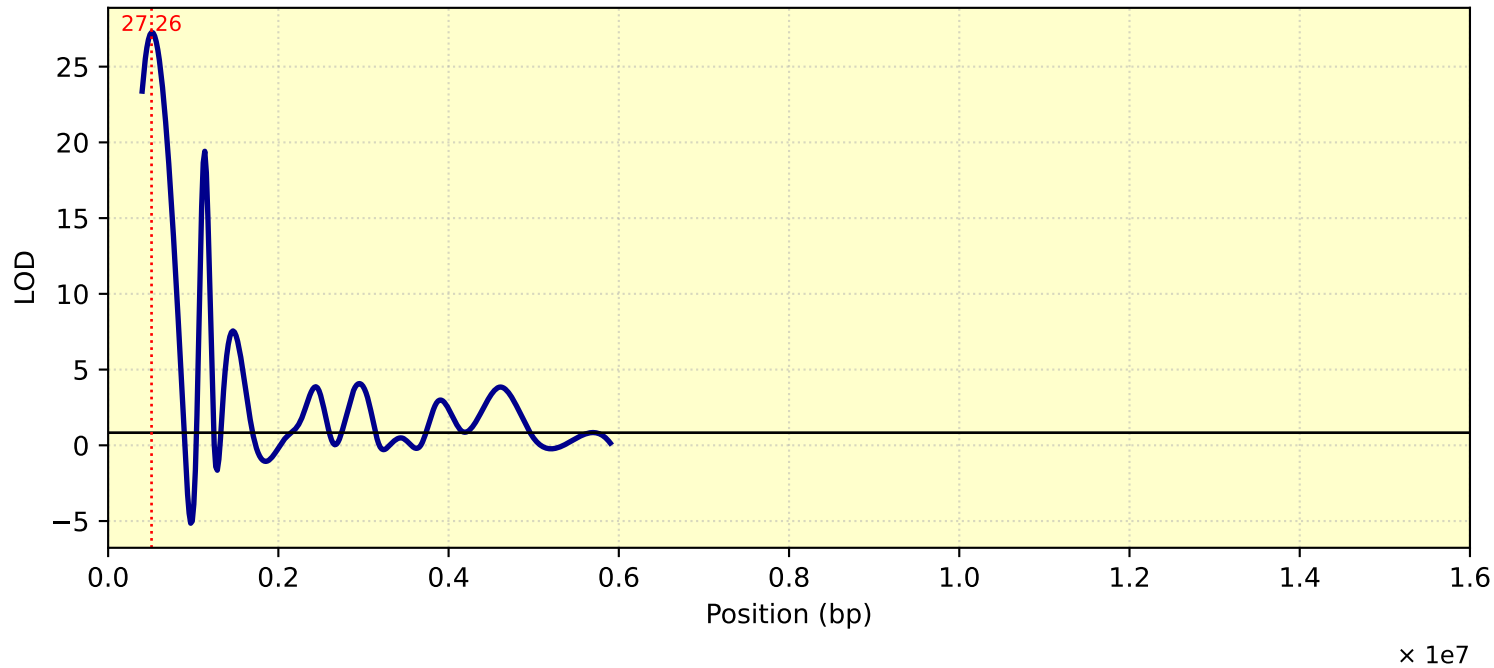
LOD Curve - chr14 - Tc29me3
