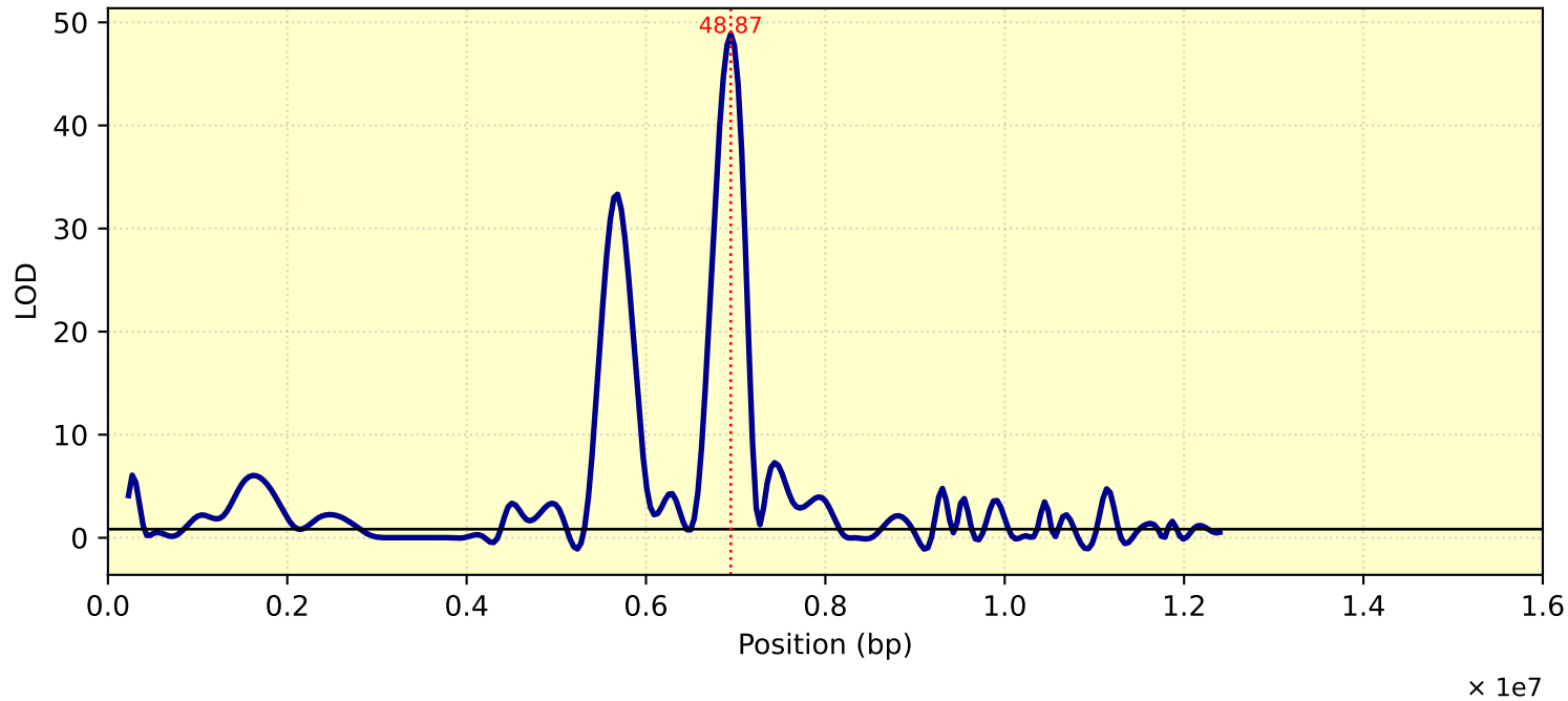
LOD Curve - chr03 - Tc29me3
