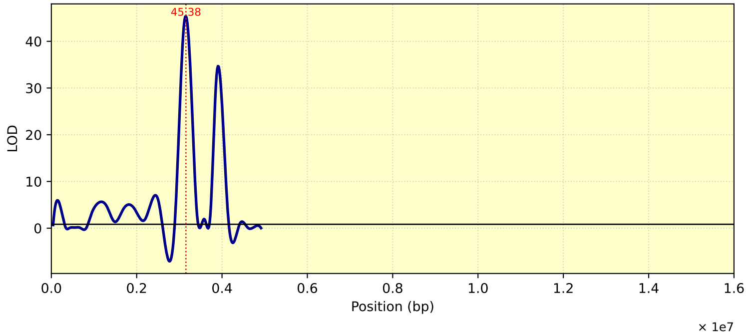
LOD Curve - chr12 - Tc29me3
