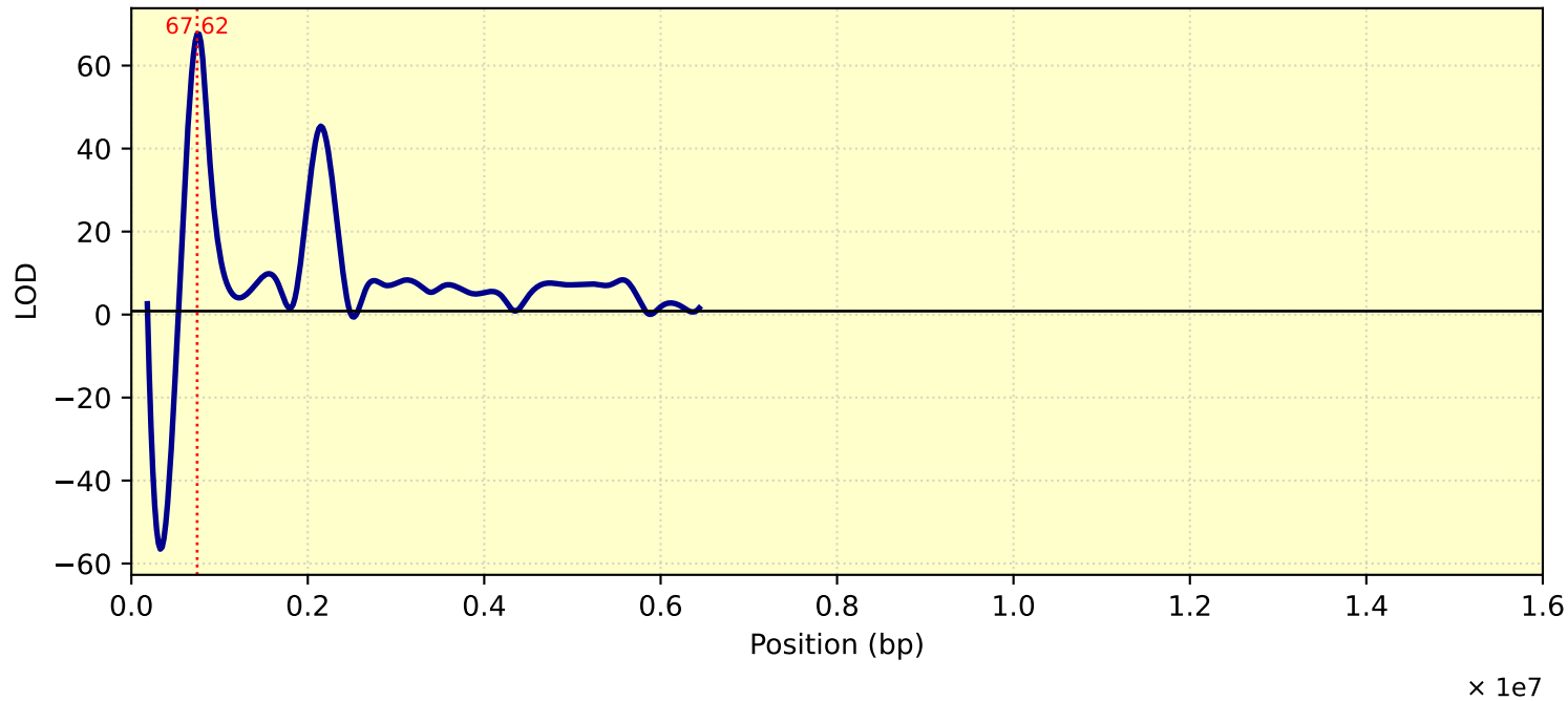
LOD Curve - chr15 - Tc29me3
