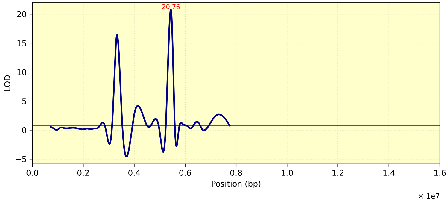
LOD Curve - chr08 - Tc29me3
