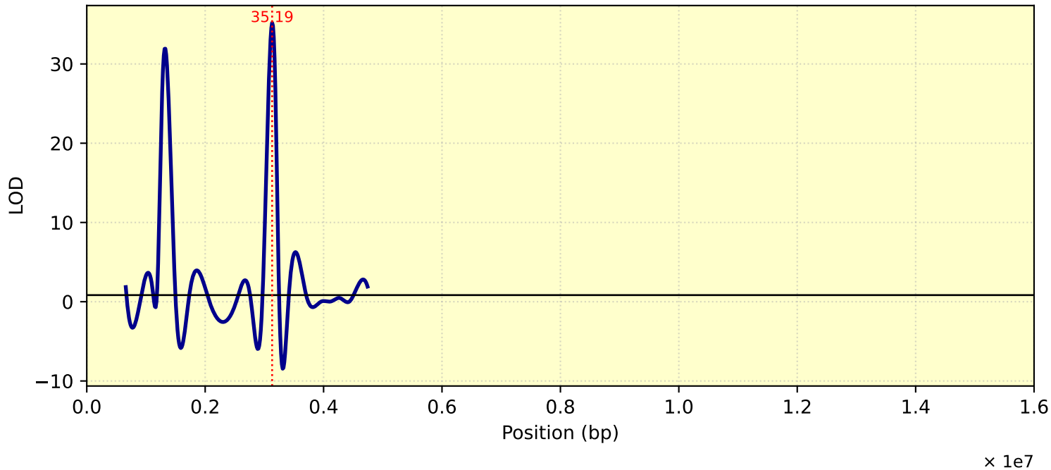
LOD Curve - chr21 - Tc29me3
