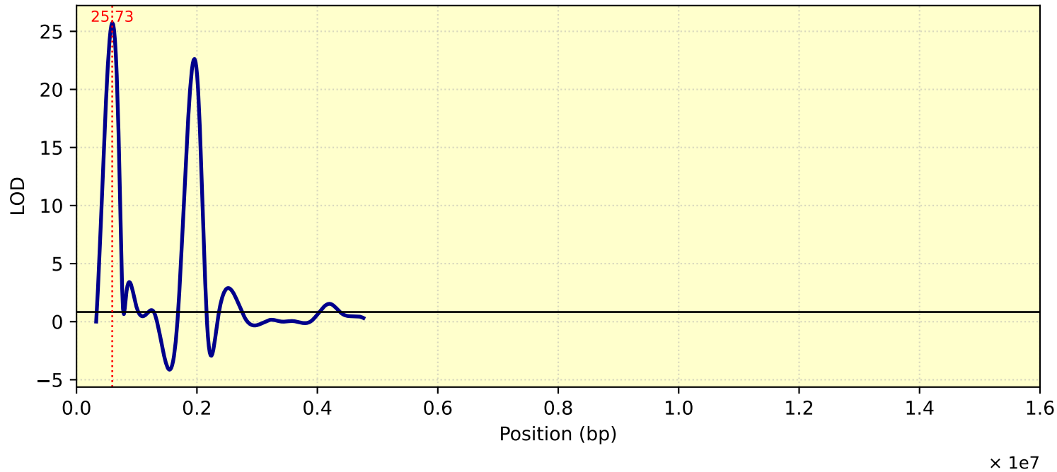
LOD Curve - chr17 - Tc29me3
