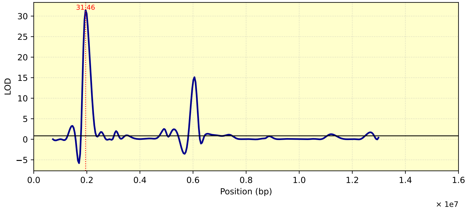
LOD Curve - chr09 - Tc29me3
