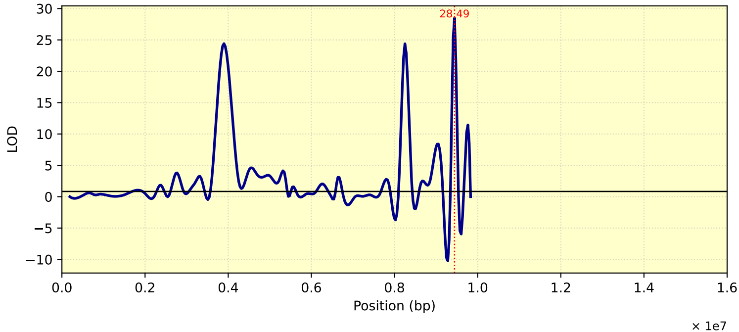
LOD Curve - chr06 - Tc29me3
