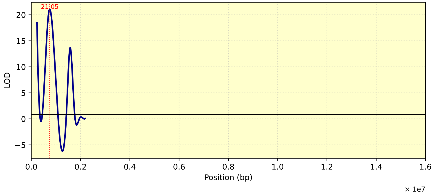
LOD Curve - chr23 - Tc29me3
