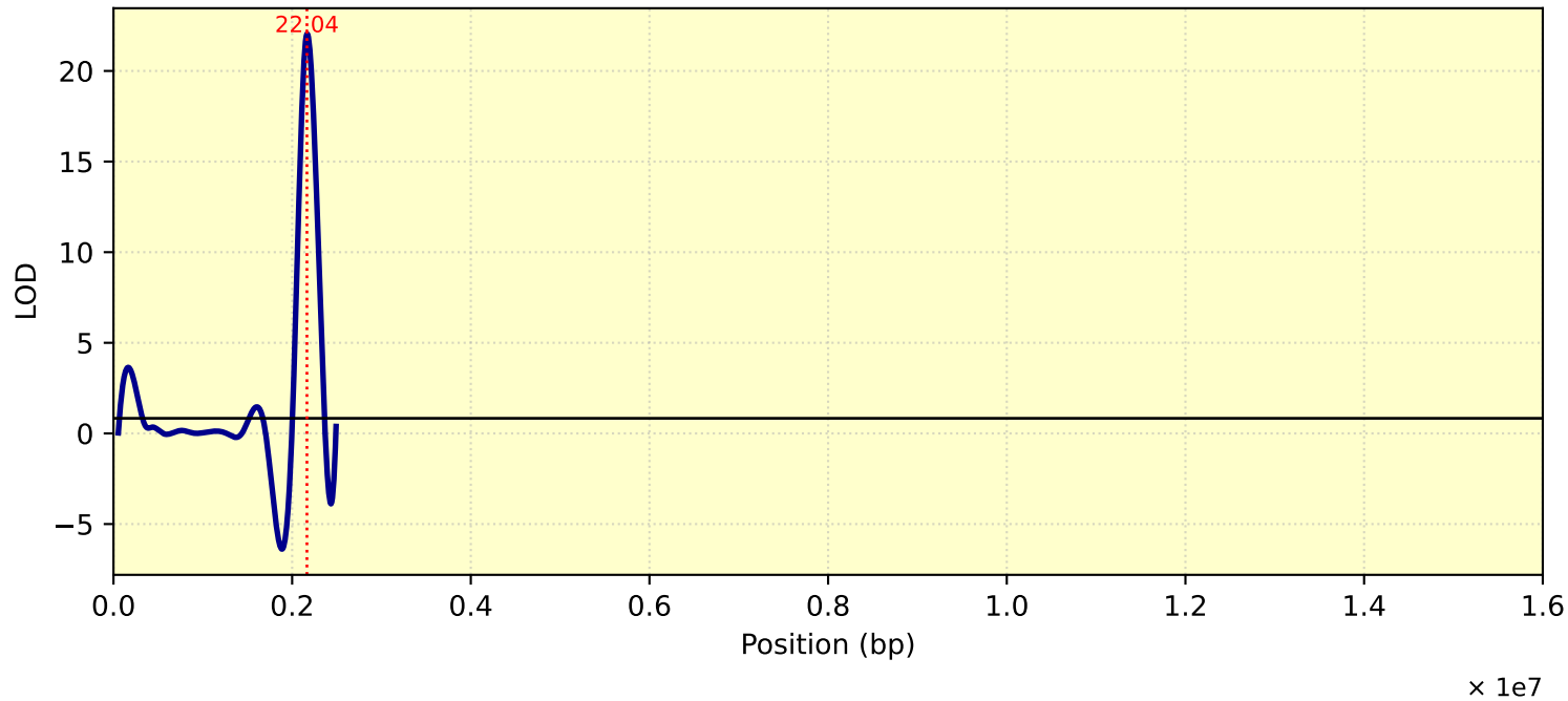
LOD Curve - chr25 - Tc29me3
