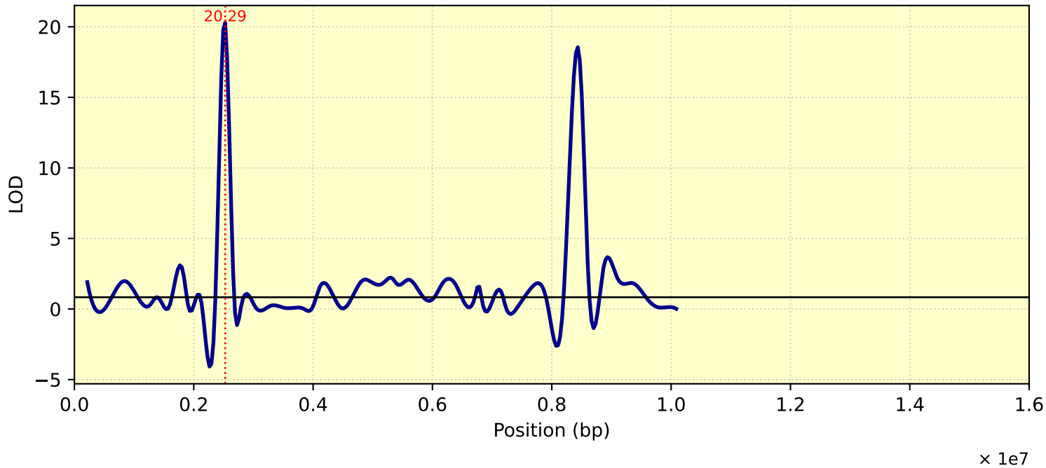
LOD Curve - chr04 - Tc29me3
