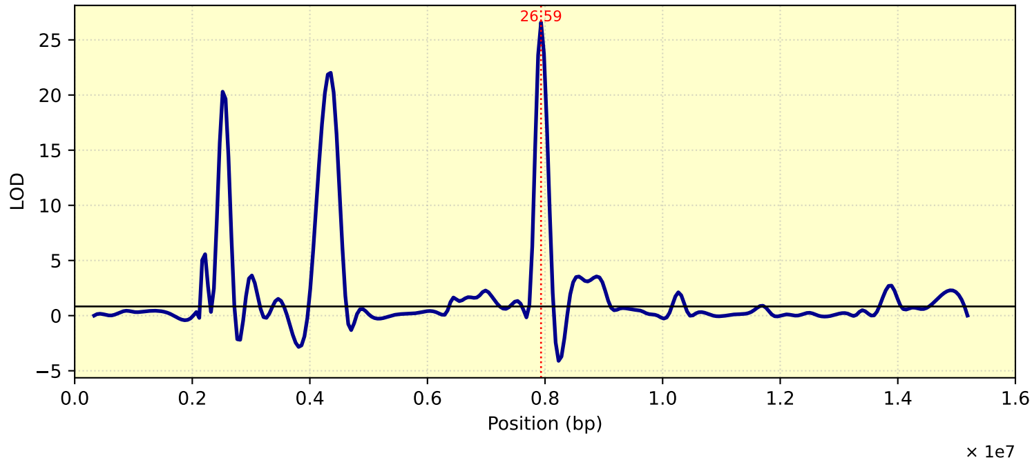
LOD Curve - chr01 - Tc29me3
