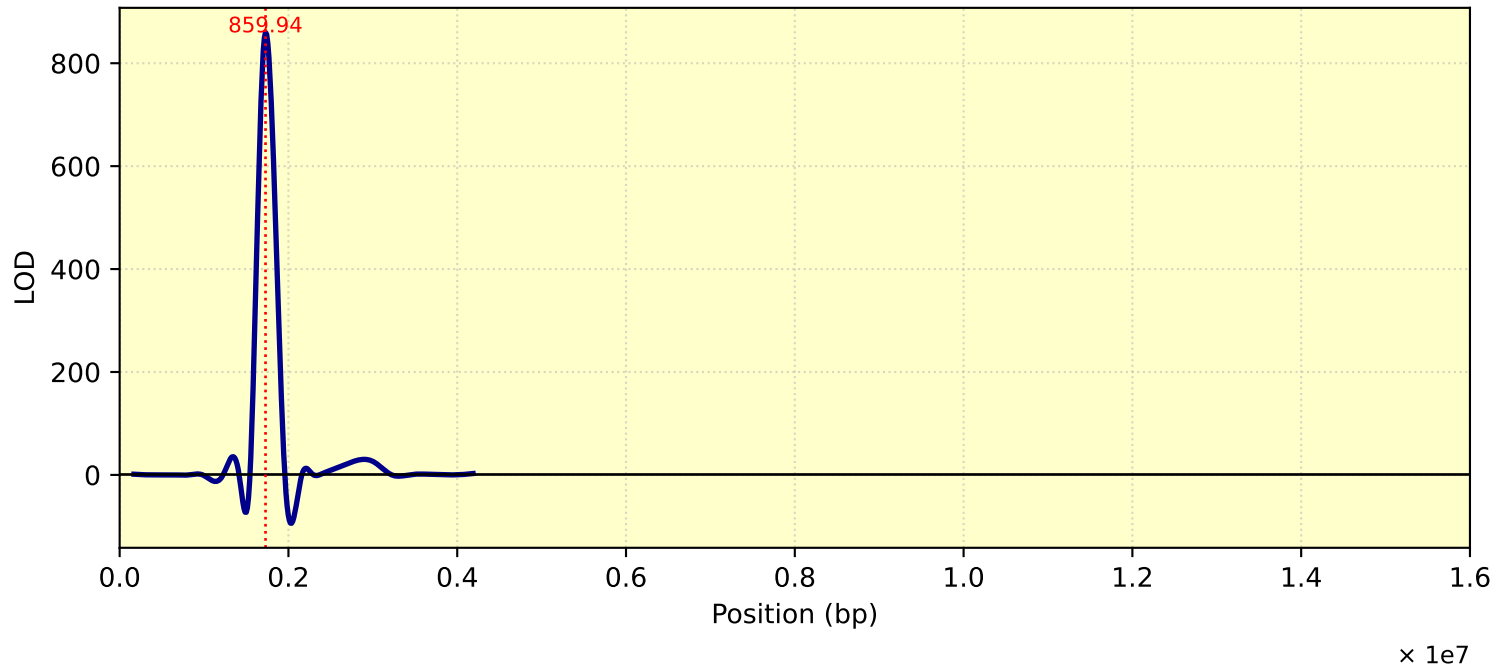
LOD Curve - chr16 - Tc29me3
