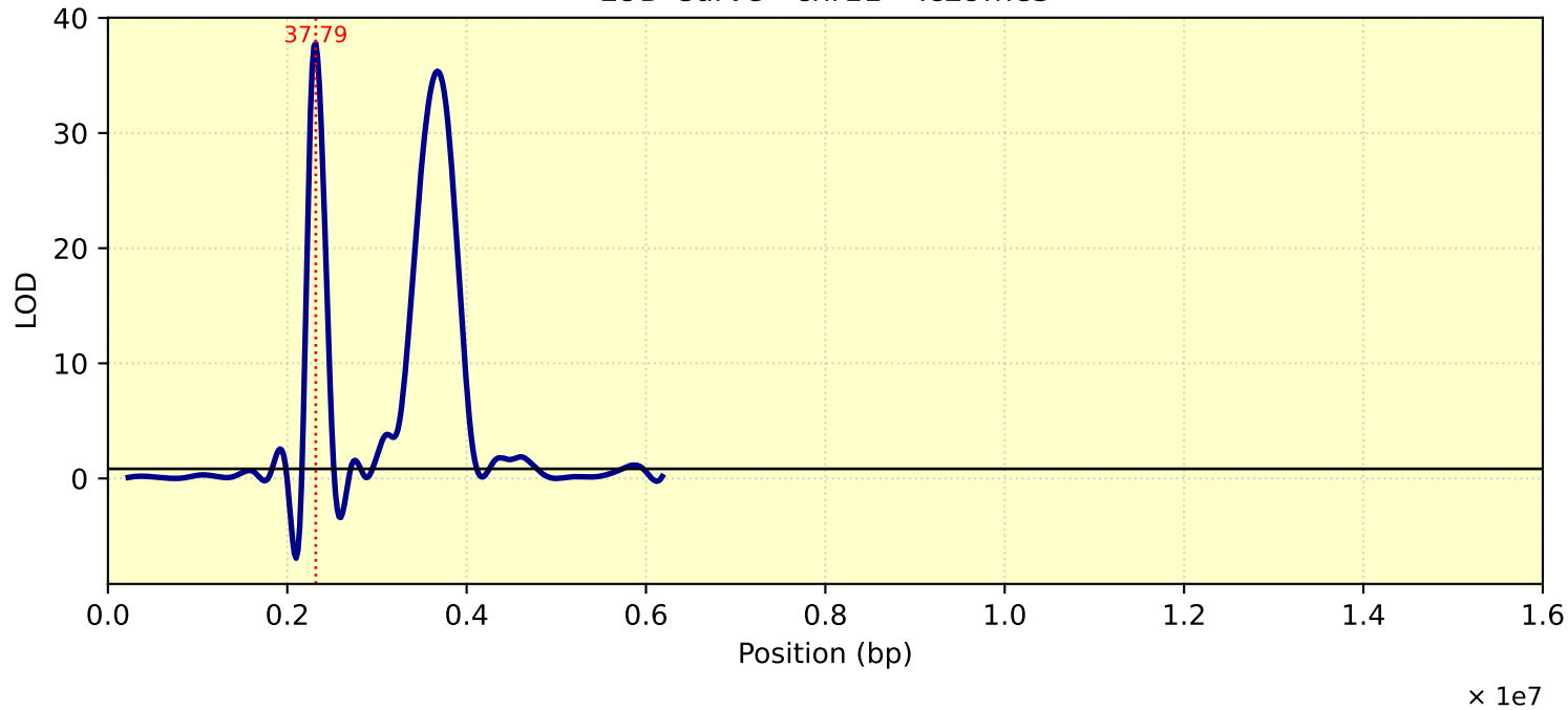
LOD Curve - chr11 - Tc29me3
