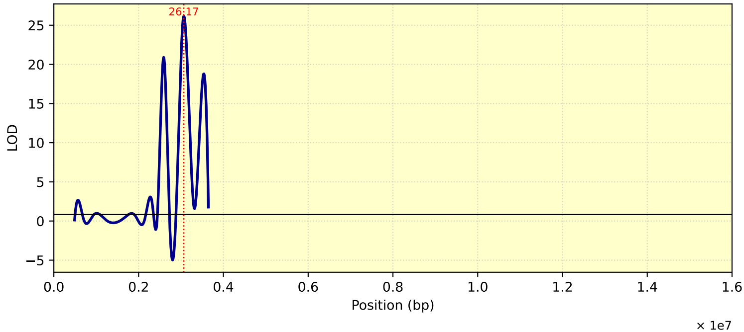
LOD Curve - chr24 - Tc29me3
