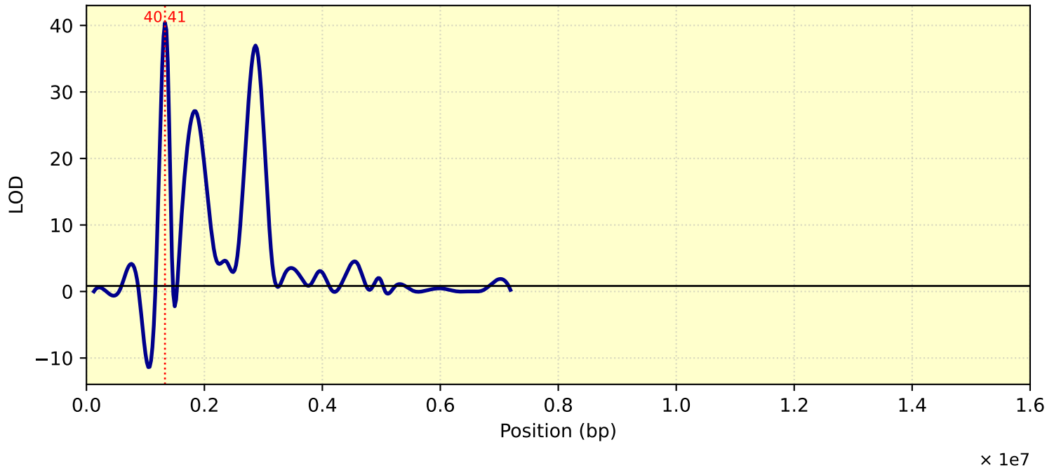
LOD Curve - chr10 - Tc29me3
