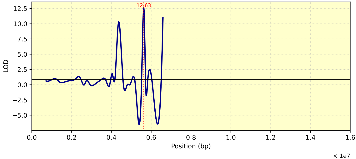
LOD Curve - chr13 - Tc29me3
