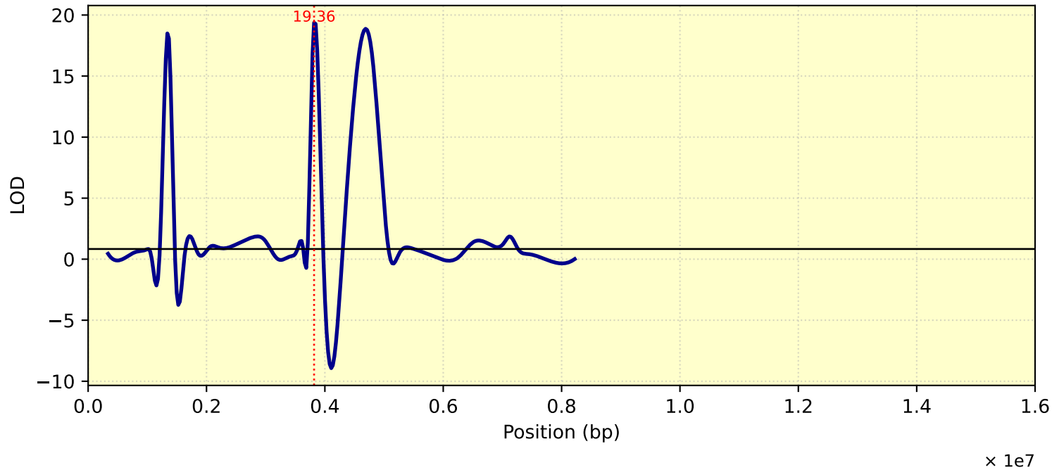
LOD Curve - chr07 - Tc29me3
