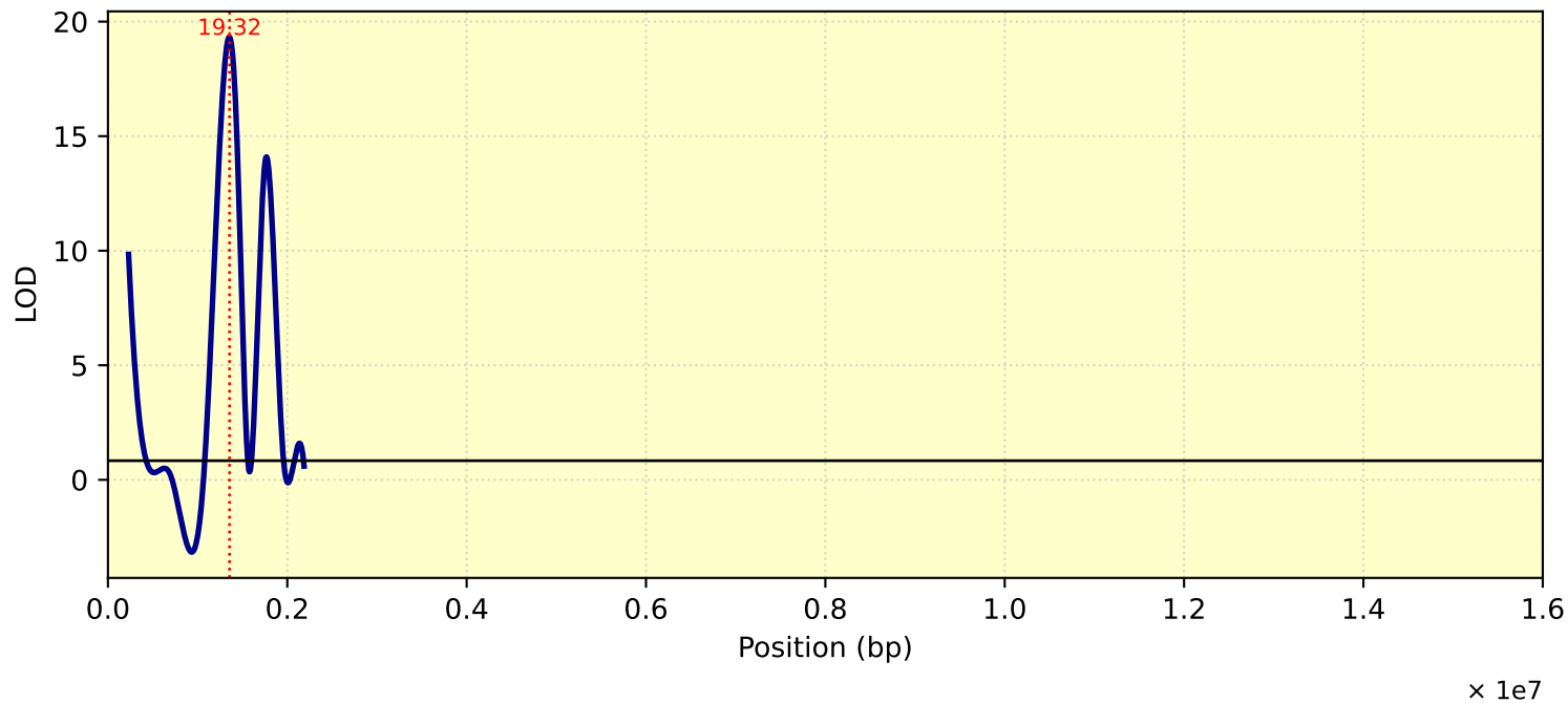
LOD Curve - chr23 - Tc31T
