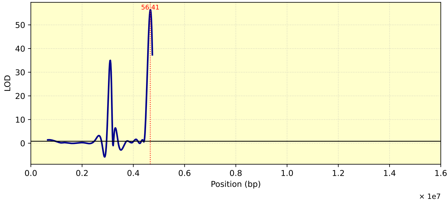
LOD Curve - chr21 - Tc31T
