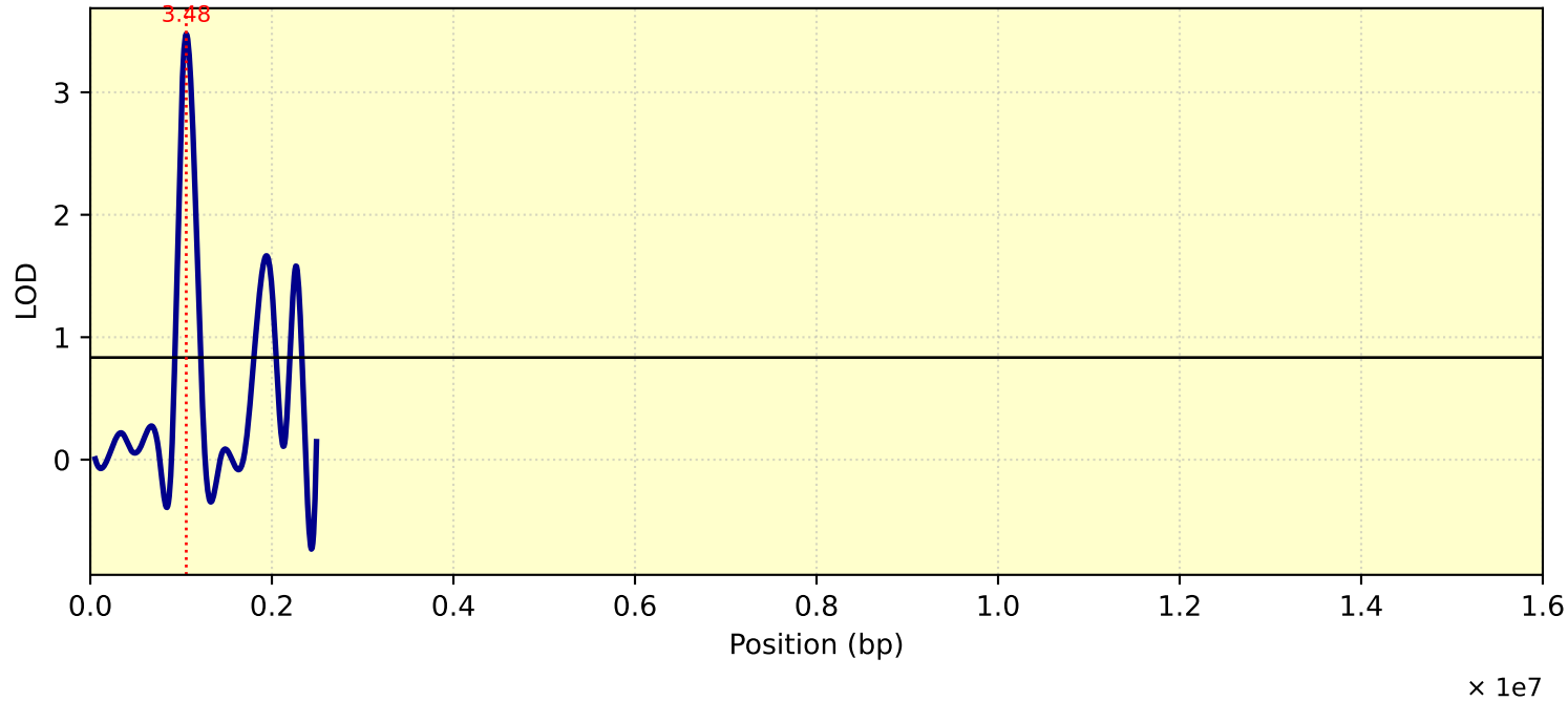
LOD Curve - chr25 - Tc31T
