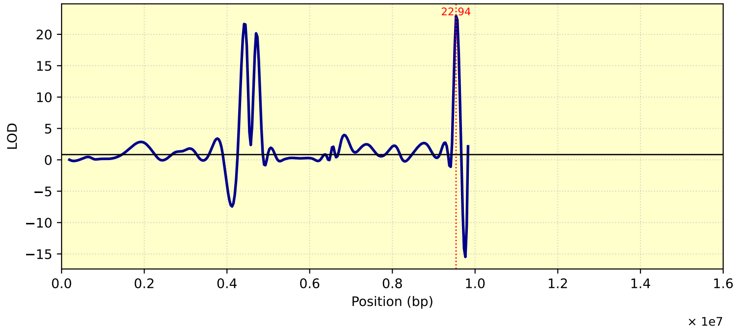
LOD Curve - chr06 - Tc31T
