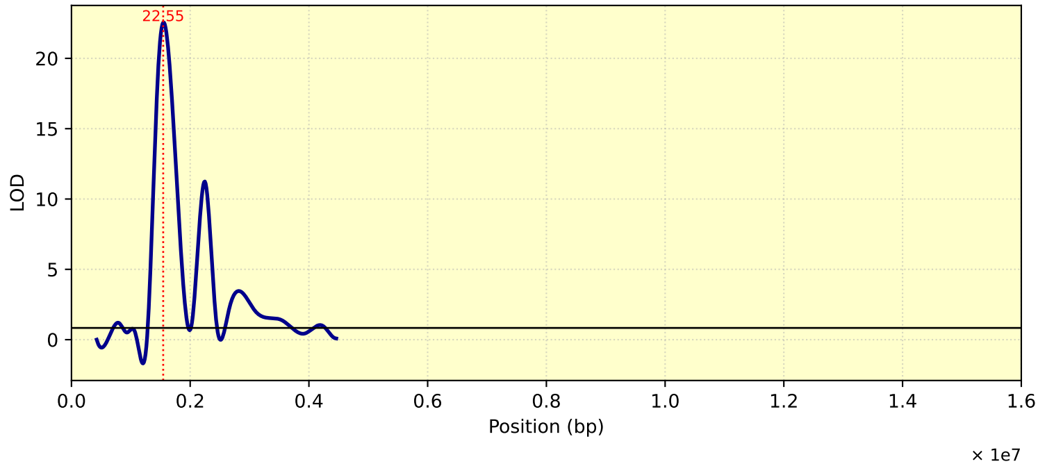
LOD Curve - chr22 - Tc31T
