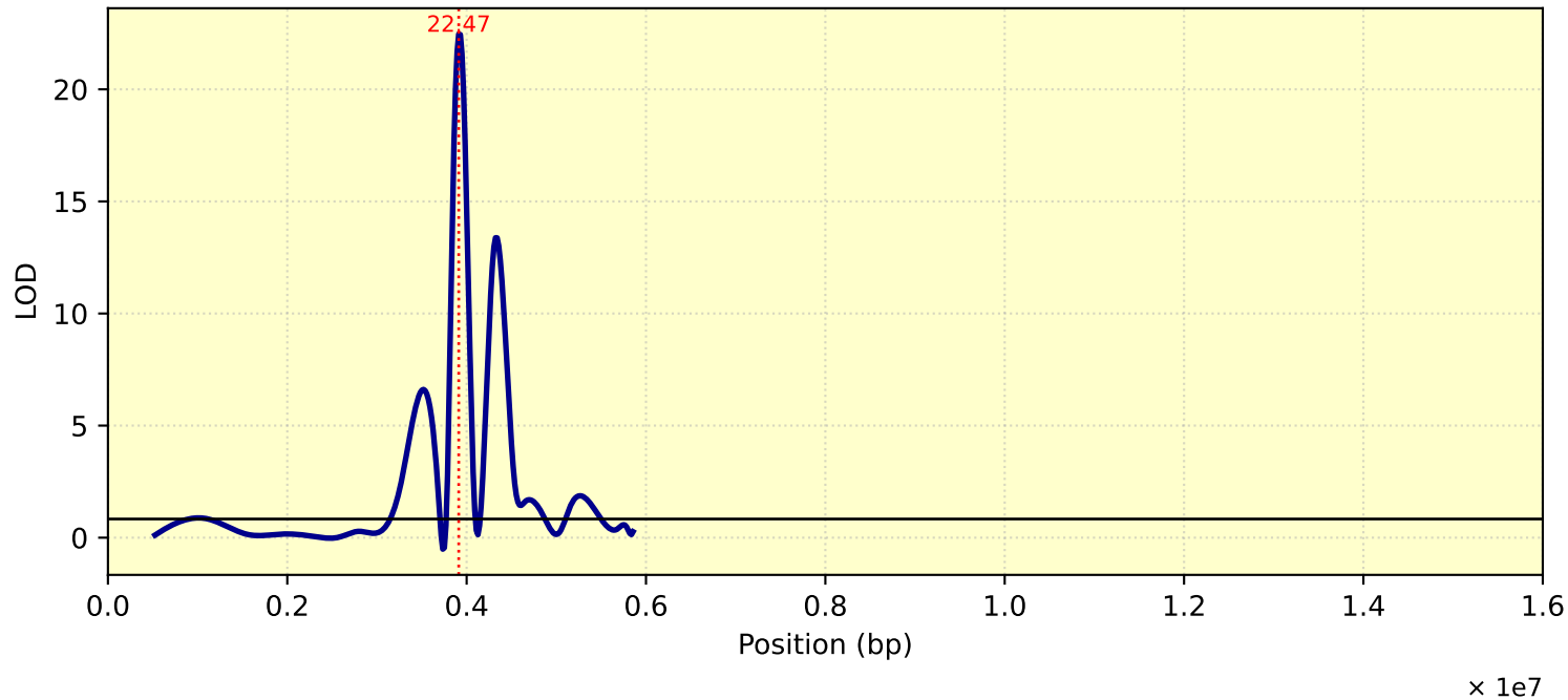
LOD Curve - chr18 - Tc31T
