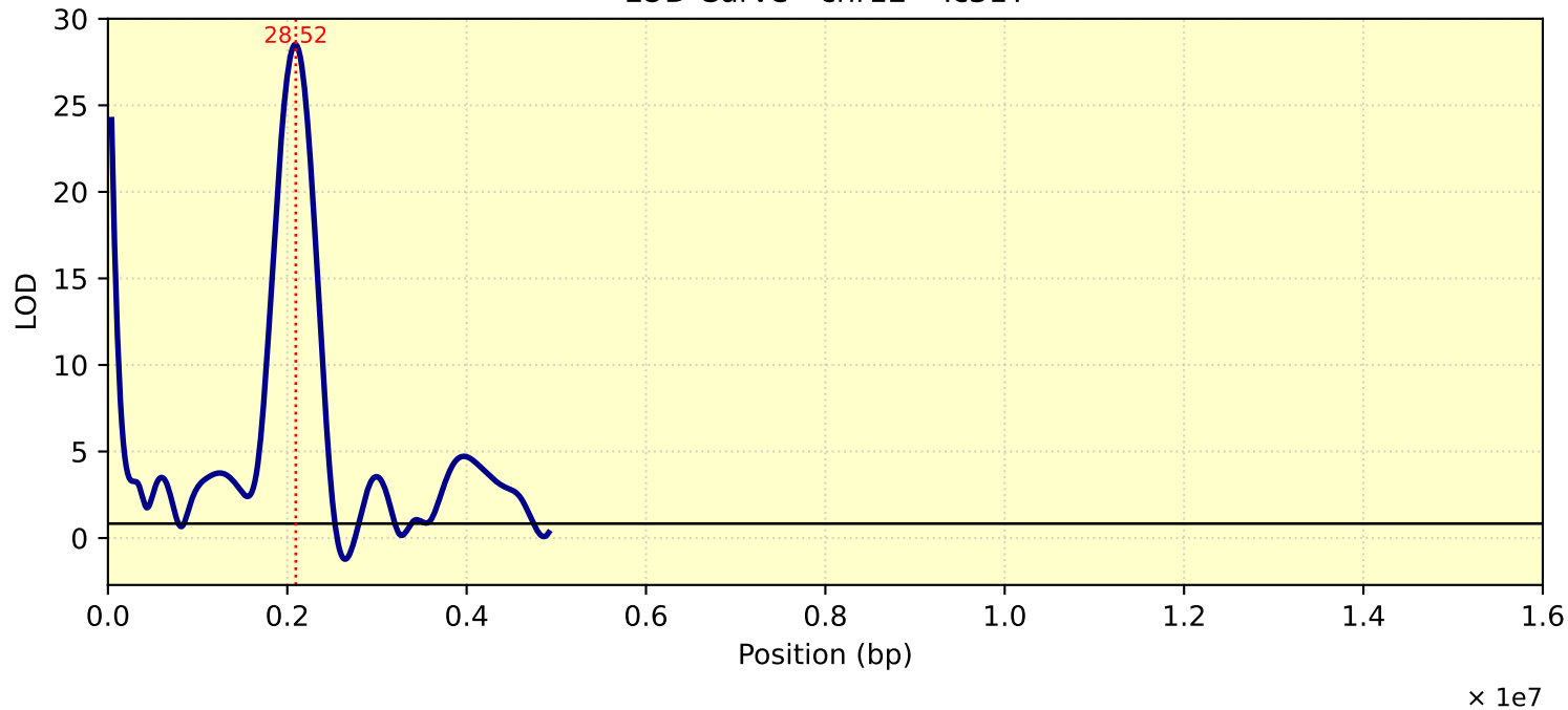
LOD Curve - chr12 - Tc31T
