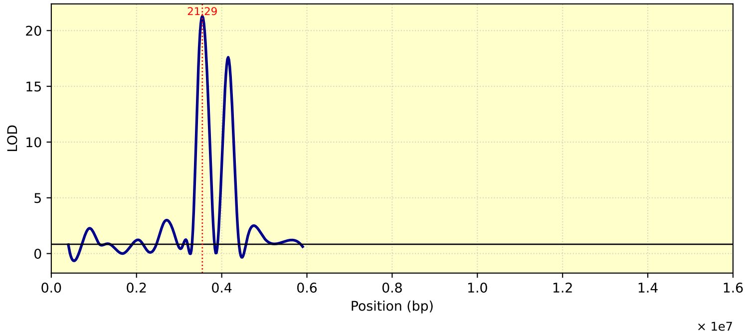
LOD Curve - chr14 - Tc31T
