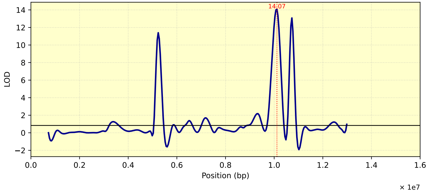
LOD Curve - chr09 - Tc31T
