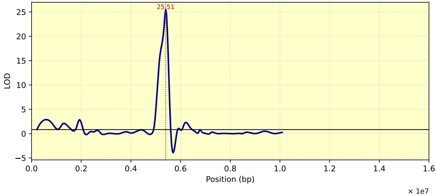
LOD Curve - chr04 - Tc31T
