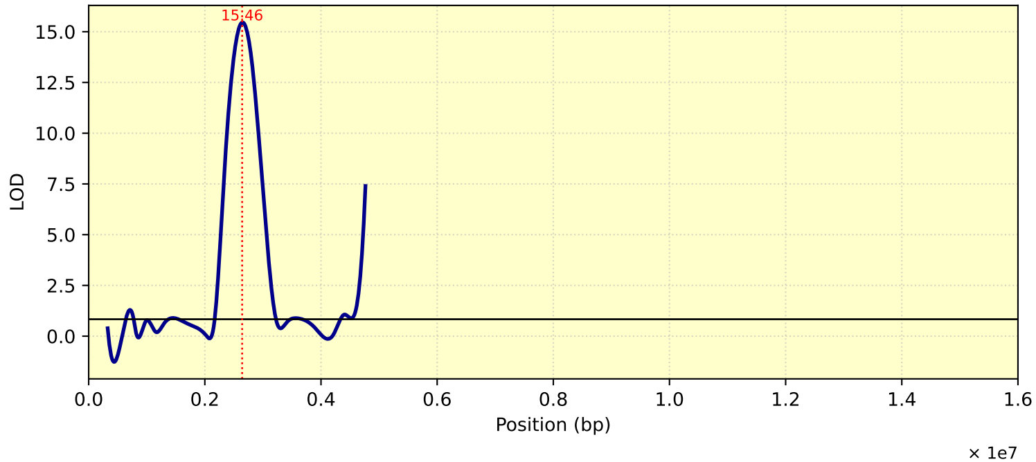
LOD Curve - chr17 - Tc31T
