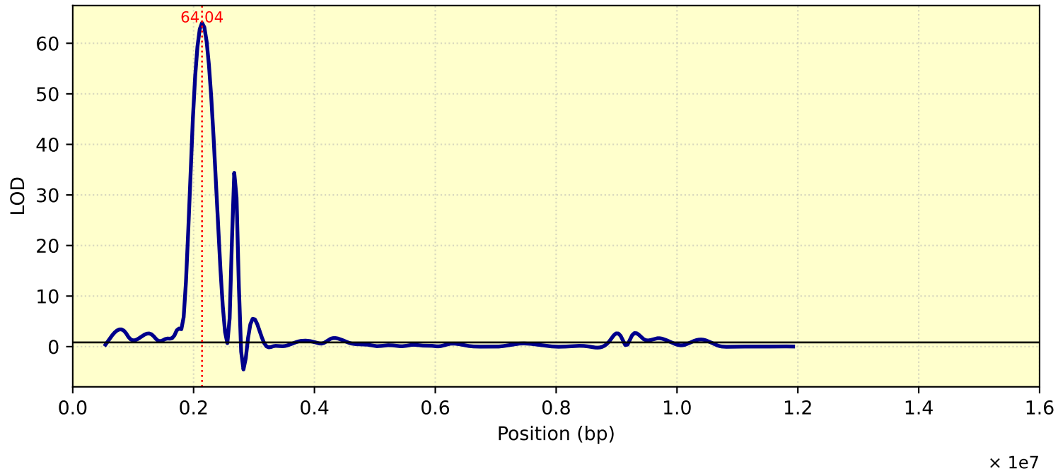
LOD Curve - chr05 - Tc31T
