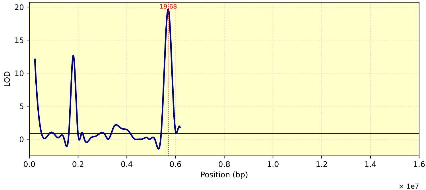
LOD Curve - chr11 - Tc31T
