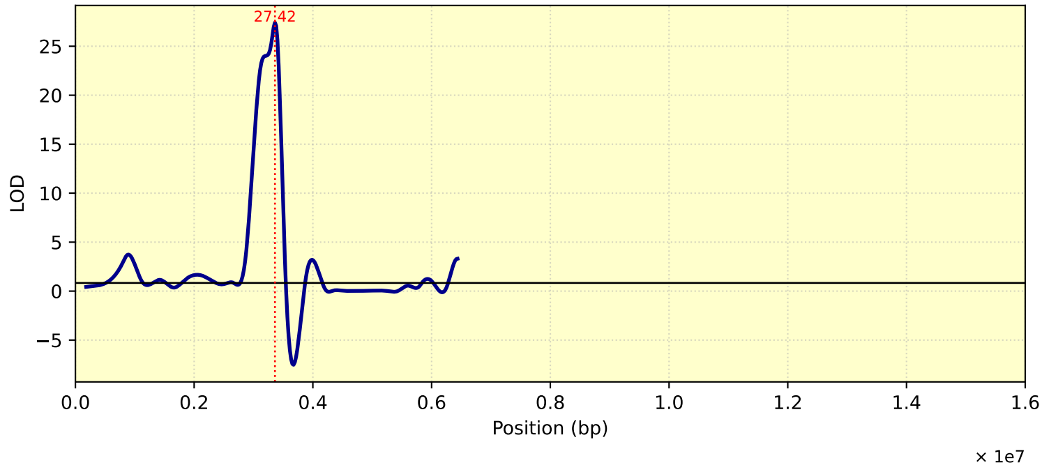
LOD Curve - chr15 - Tc31T
