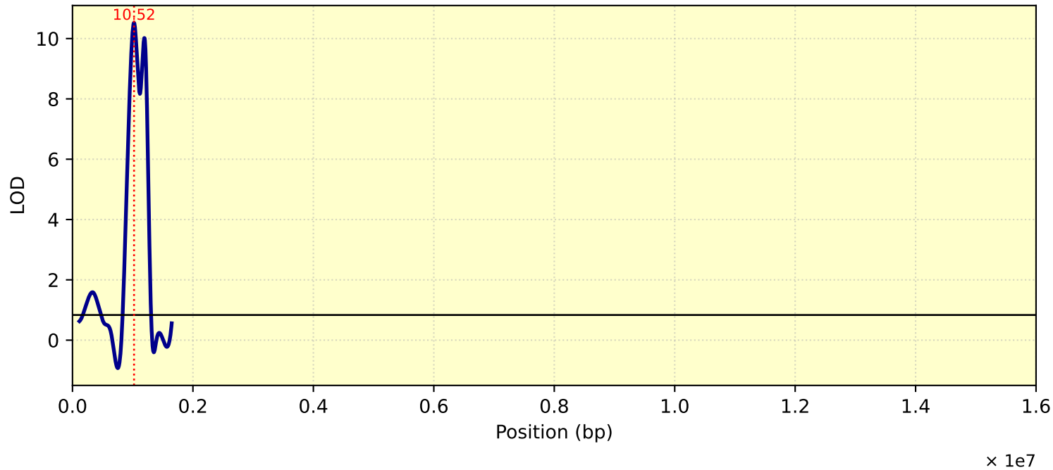
LOD Curve - chr26 - Tc31T
