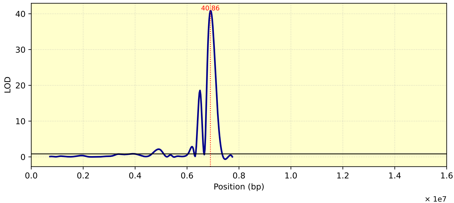
LOD Curve - chr08 - Tc31T
