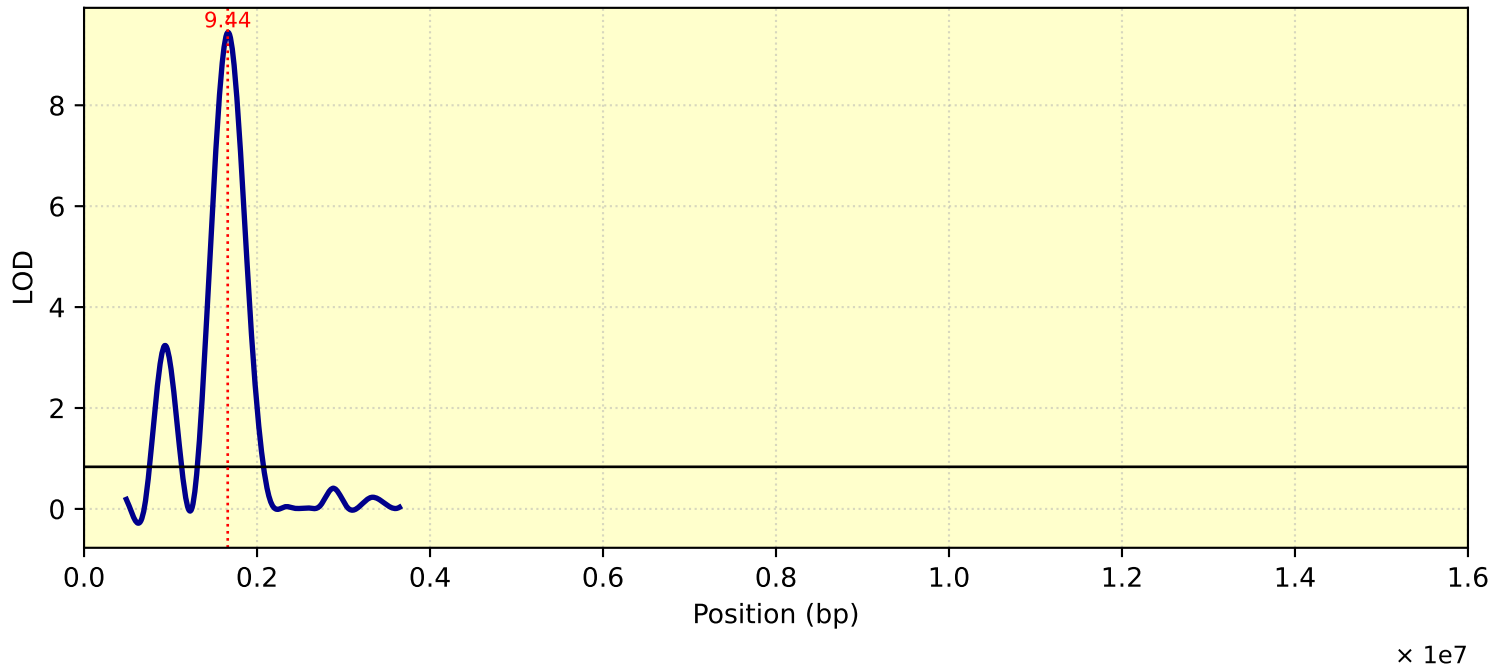
LOD Curve - chr24 - Tc31T
