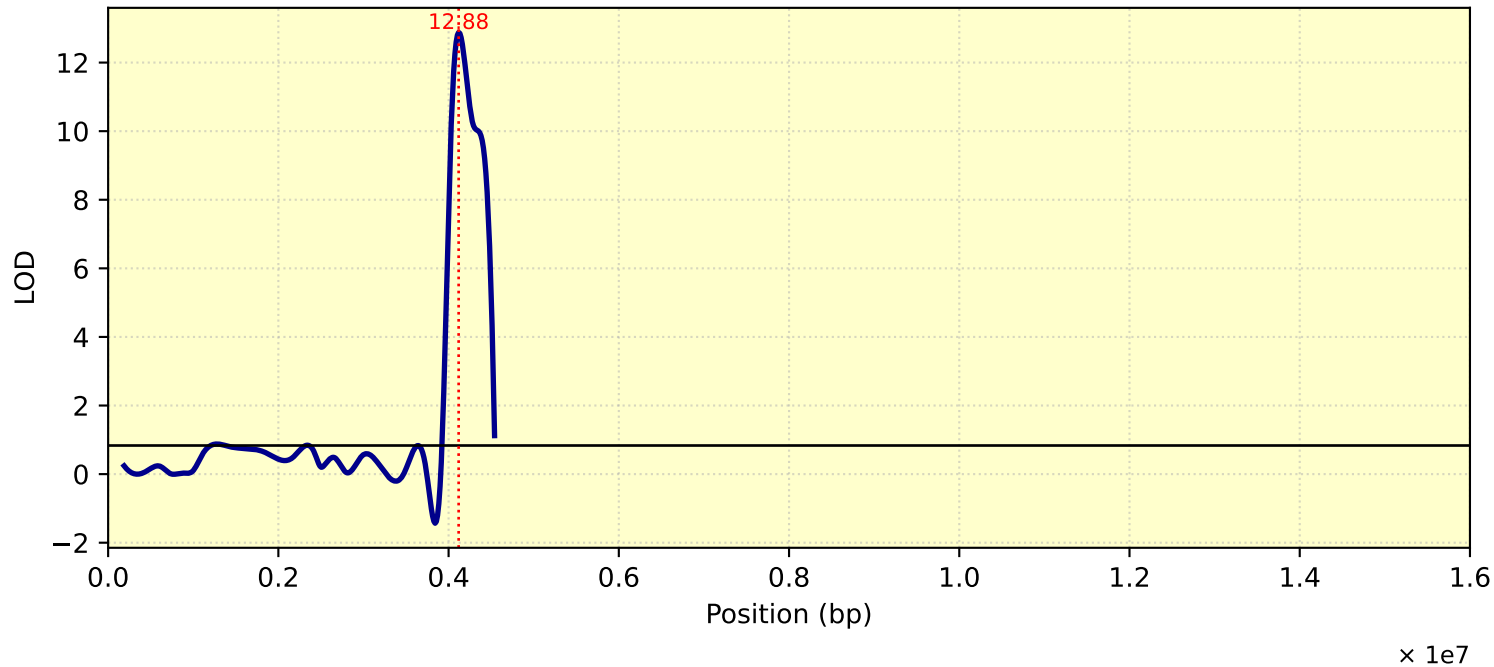
LOD Curve - chr19 - Tc31T
