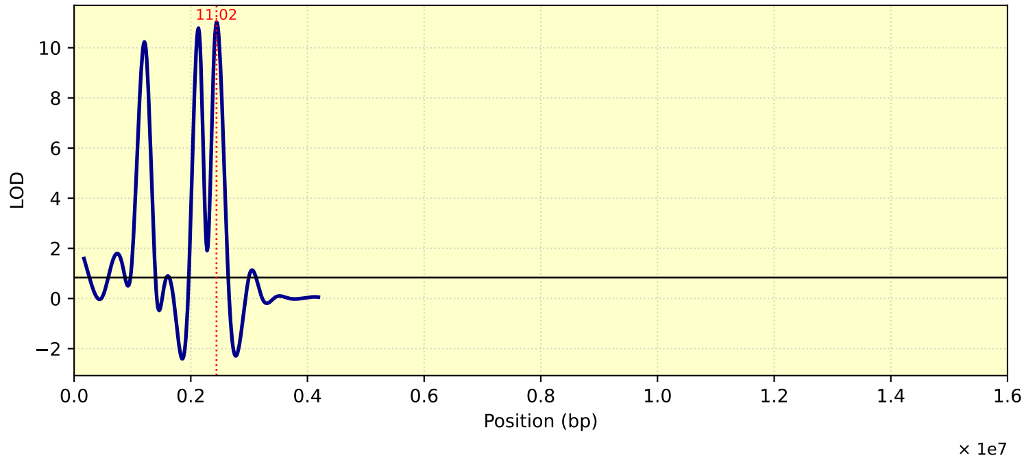
LOD Curve - chr16 - Tc31T
