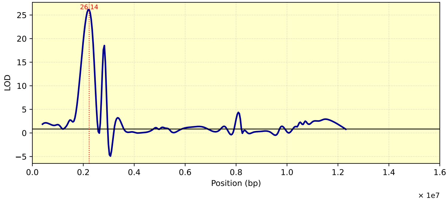
LOD Curve - chr02 - Tc31T
