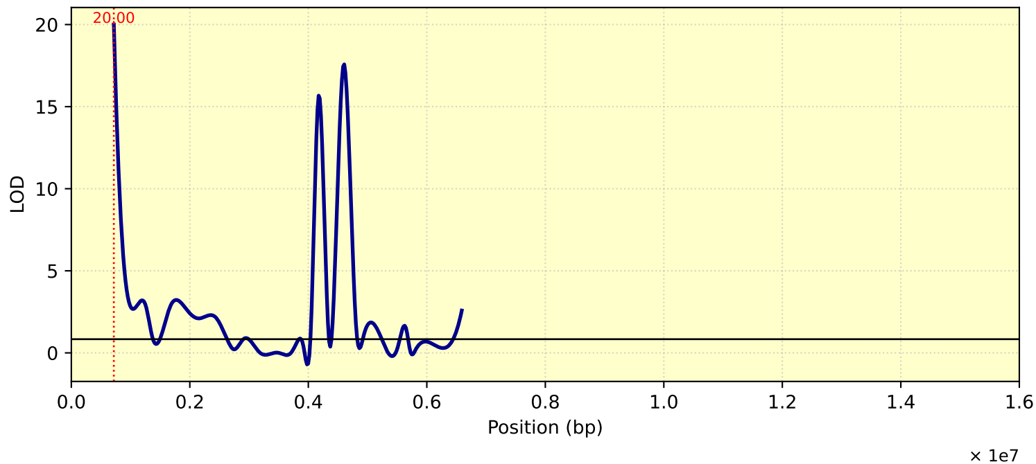
LOD Curve - chr13 - Tc31T
