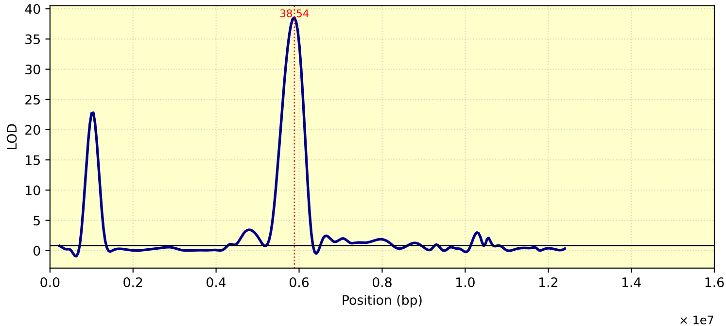
LOD Curve - chr03 - Tc31T
