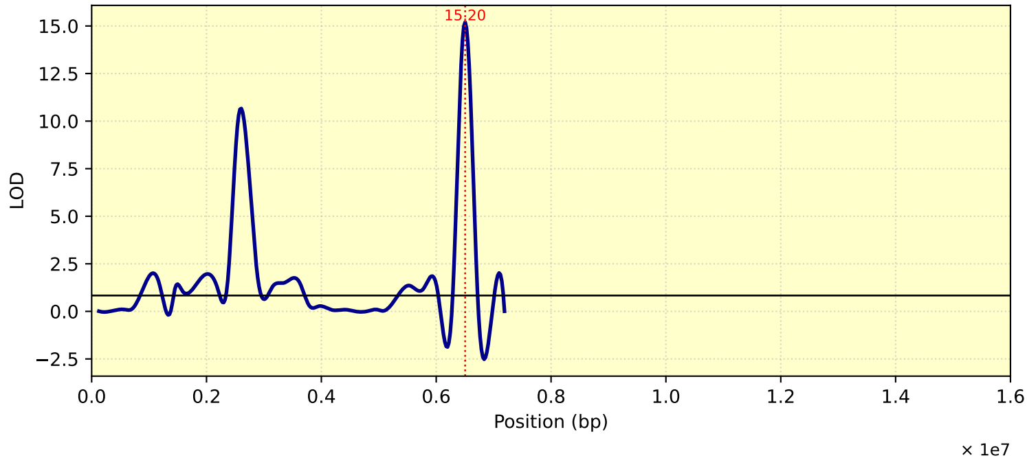
LOD Curve - chr10 - Tc31T
