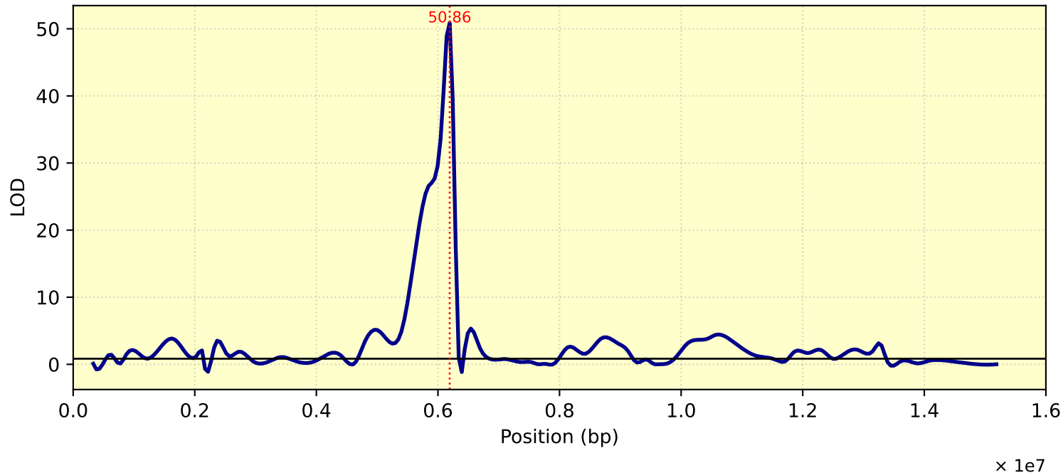
LOD Curve - chr01 - Tc31T
