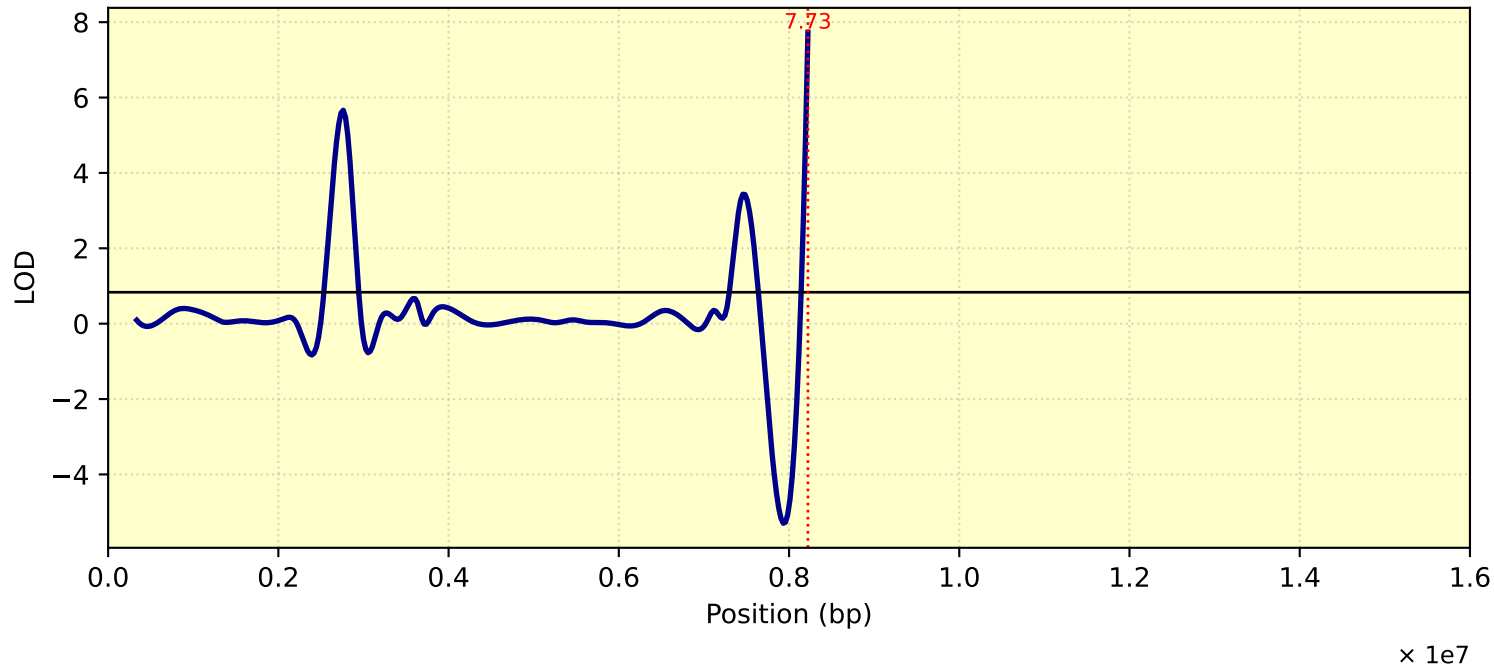
LOD Curve - chr07 - Tc31T
