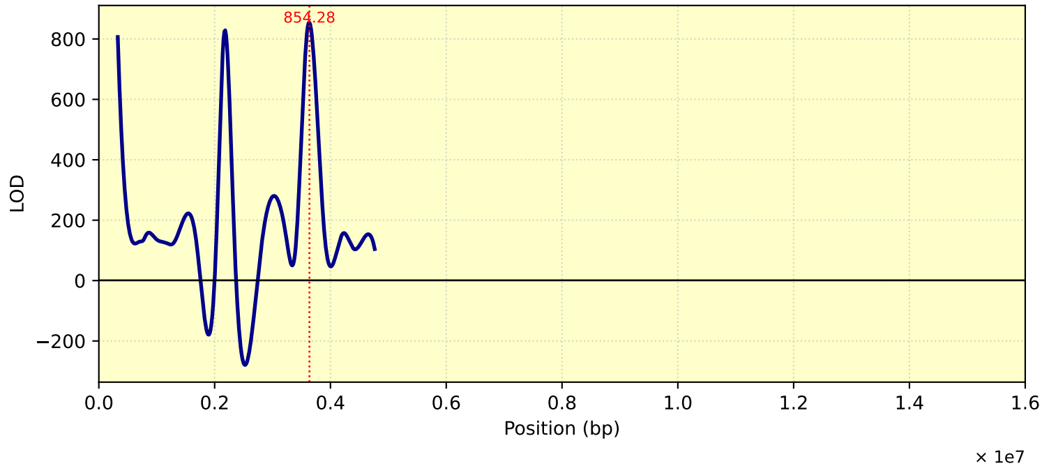
LOD Curve - chr17 - TotalD1T
