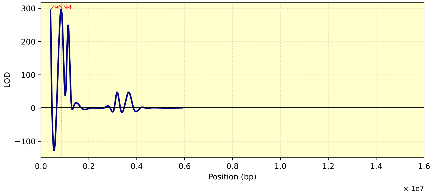
LOD Curve - chr14 - tc27d7m11T1
