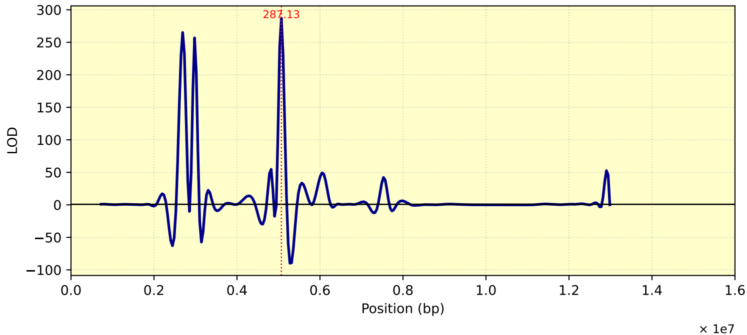
LOD Curve - chr09 - tc27d7m11T1
