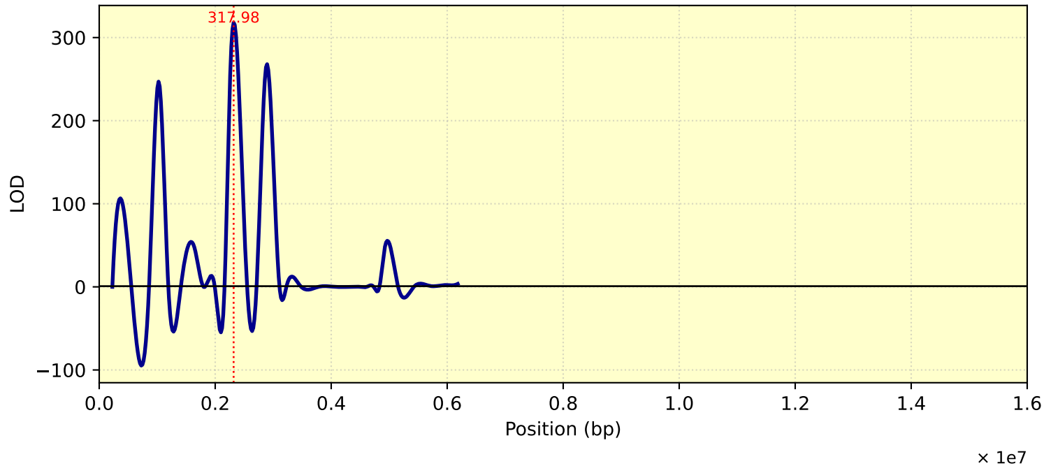
LOD Curve - chr11 - tc27d7m11T1
