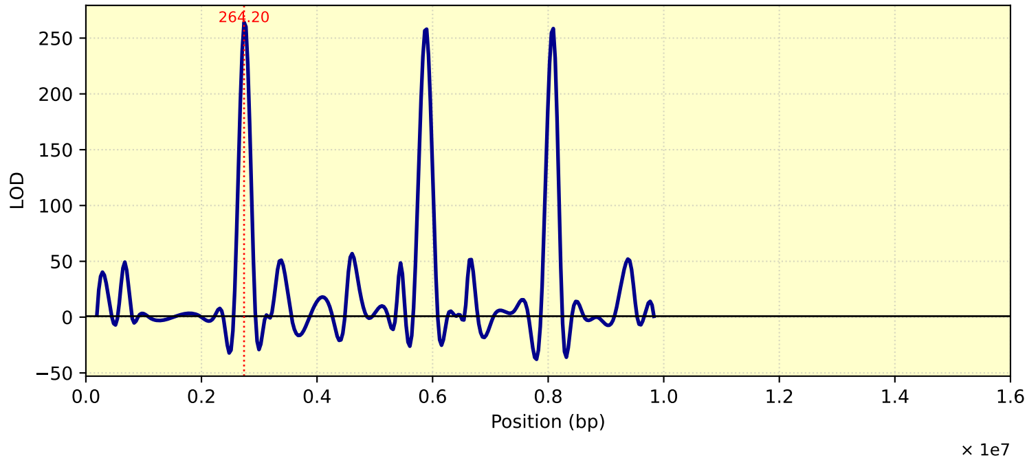
LOD Curve - chr06 - tc27d7m11T1
