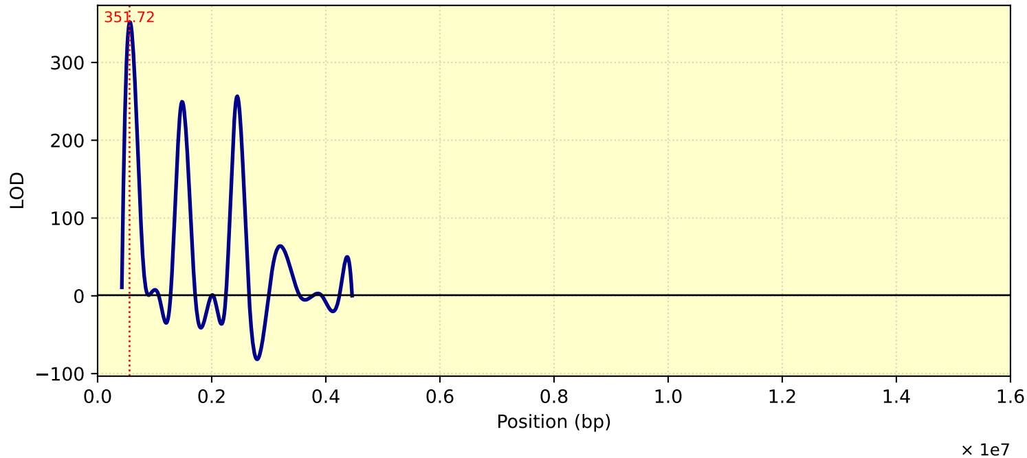
LOD Curve - chr22 - tc27d7m11T1
