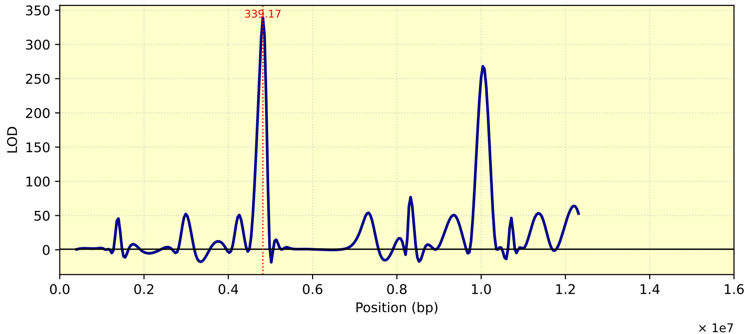
LOD Curve - chr02 - tc27d7m11T1
