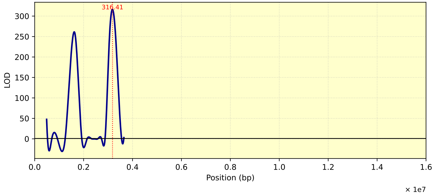
LOD Curve - chr24 - tc27d7m11T1
