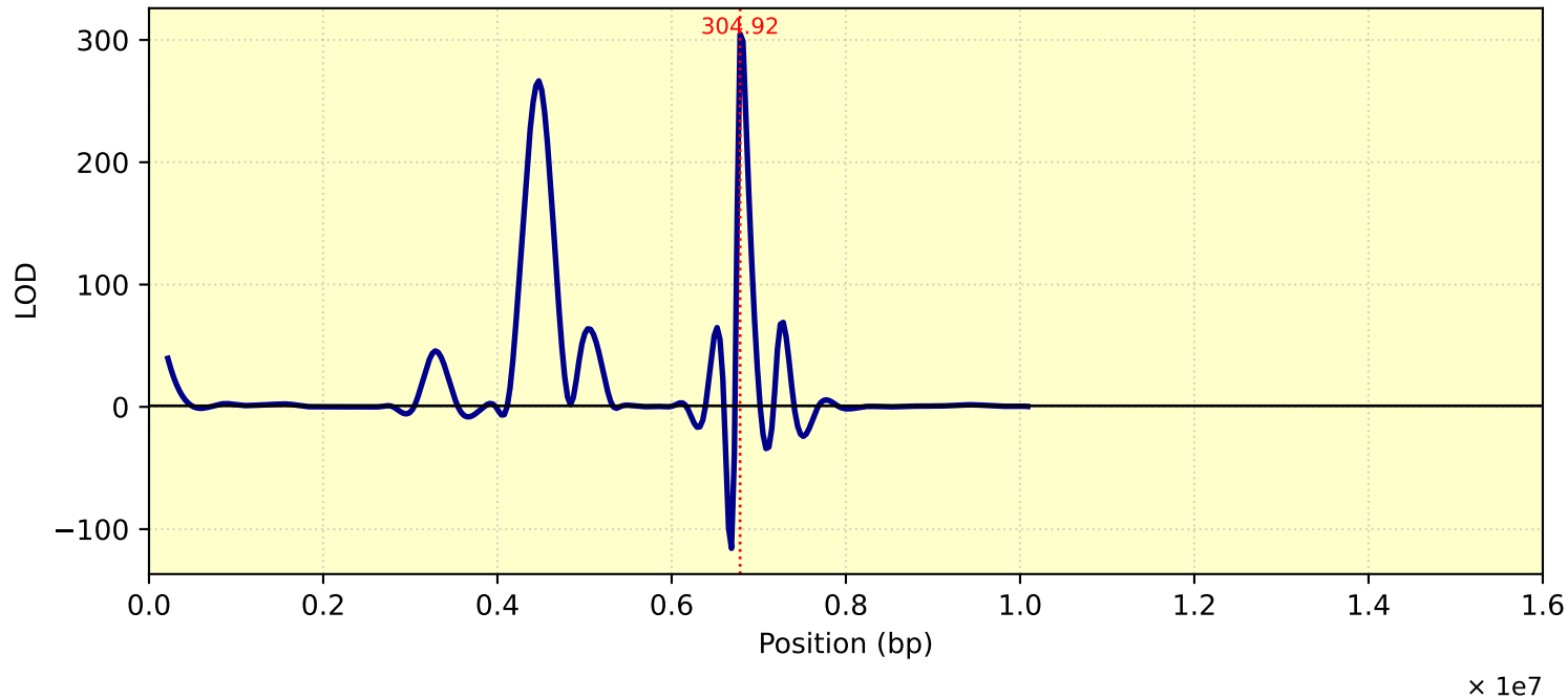
LOD Curve - chr04 - tc27d7m11T1
