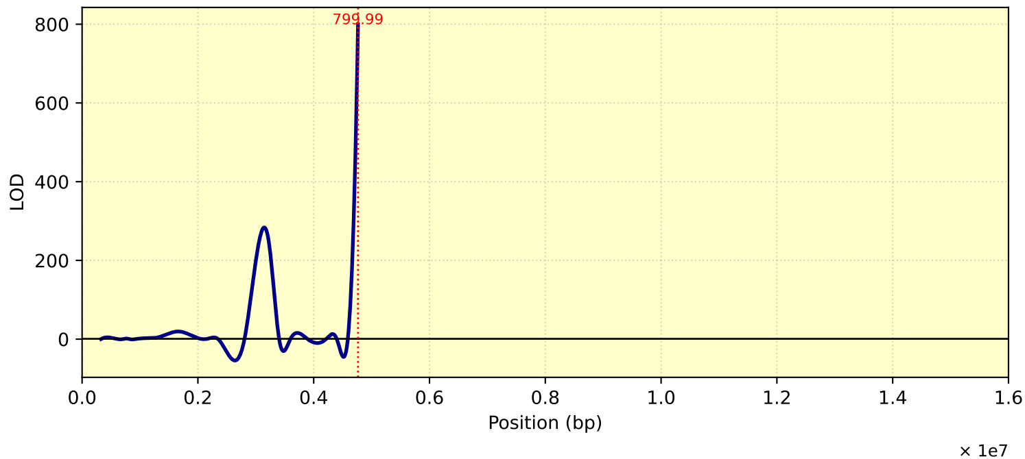
LOD Curve - chr17 - tc27d7m11T1
