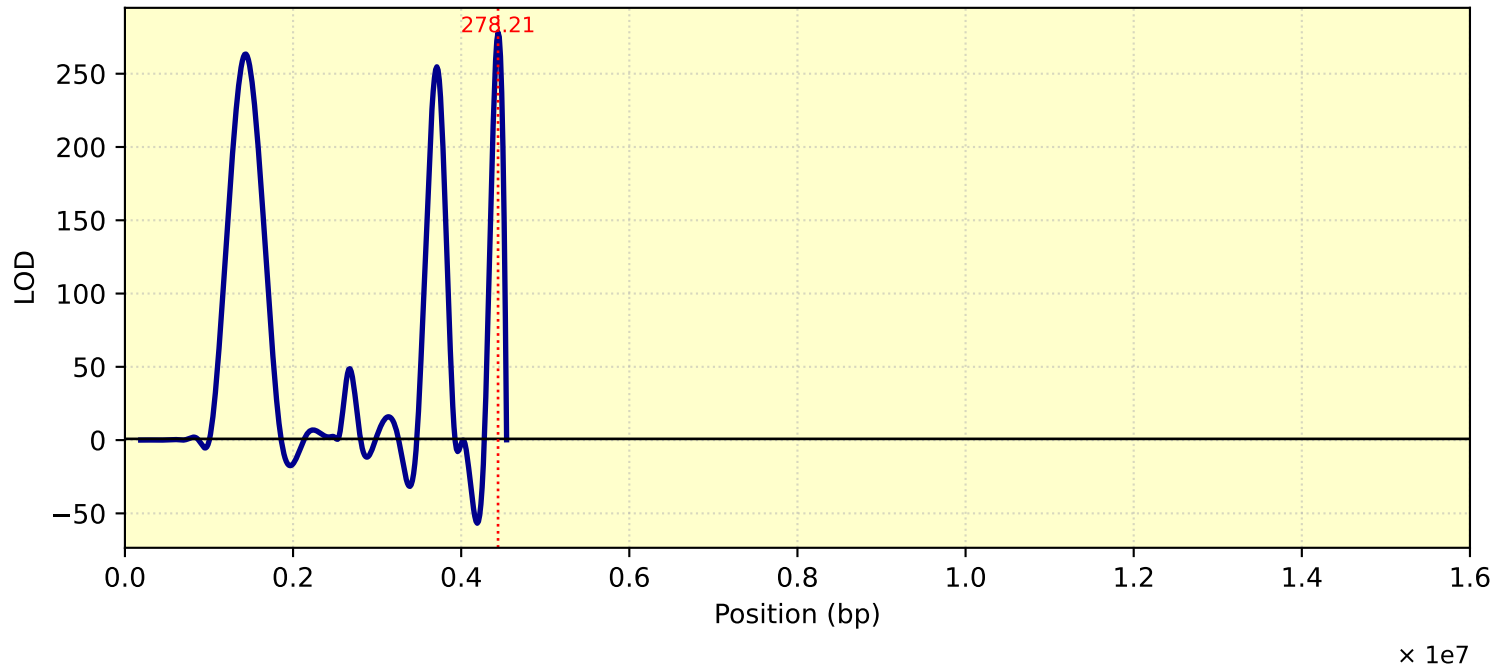
LOD Curve - chr19 - tc27d7m11T1
