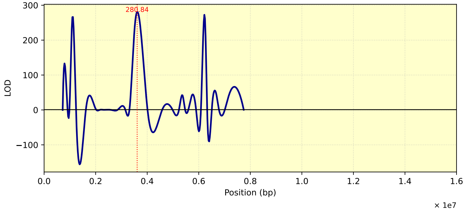
LOD Curve - chr08 - tc27d7m11T1
