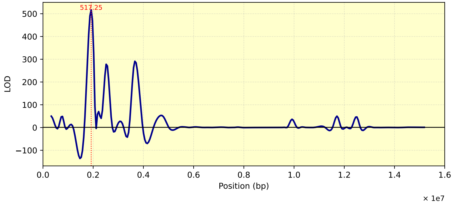
LOD Curve - chr01 - tc27d7m11T1
