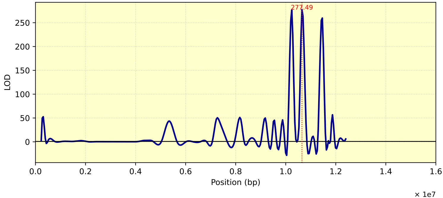
LOD Curve - chr03 - tc27d7m11T1
