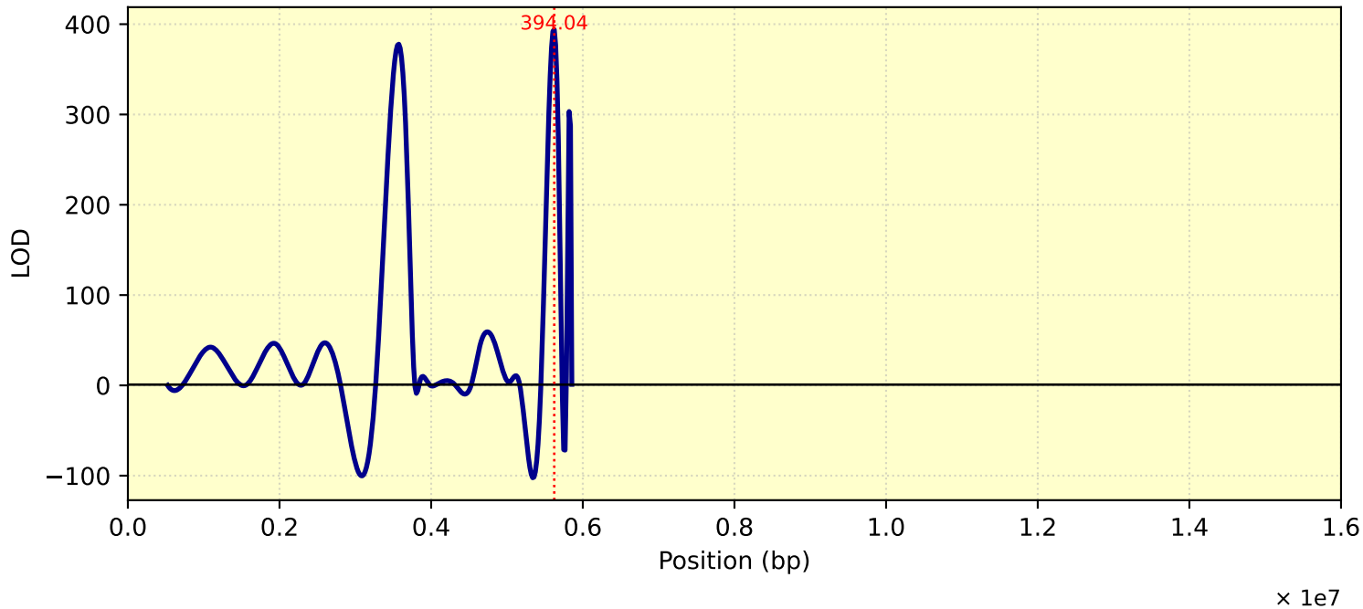
LOD Curve - chr18 - tc27d7m11T1
