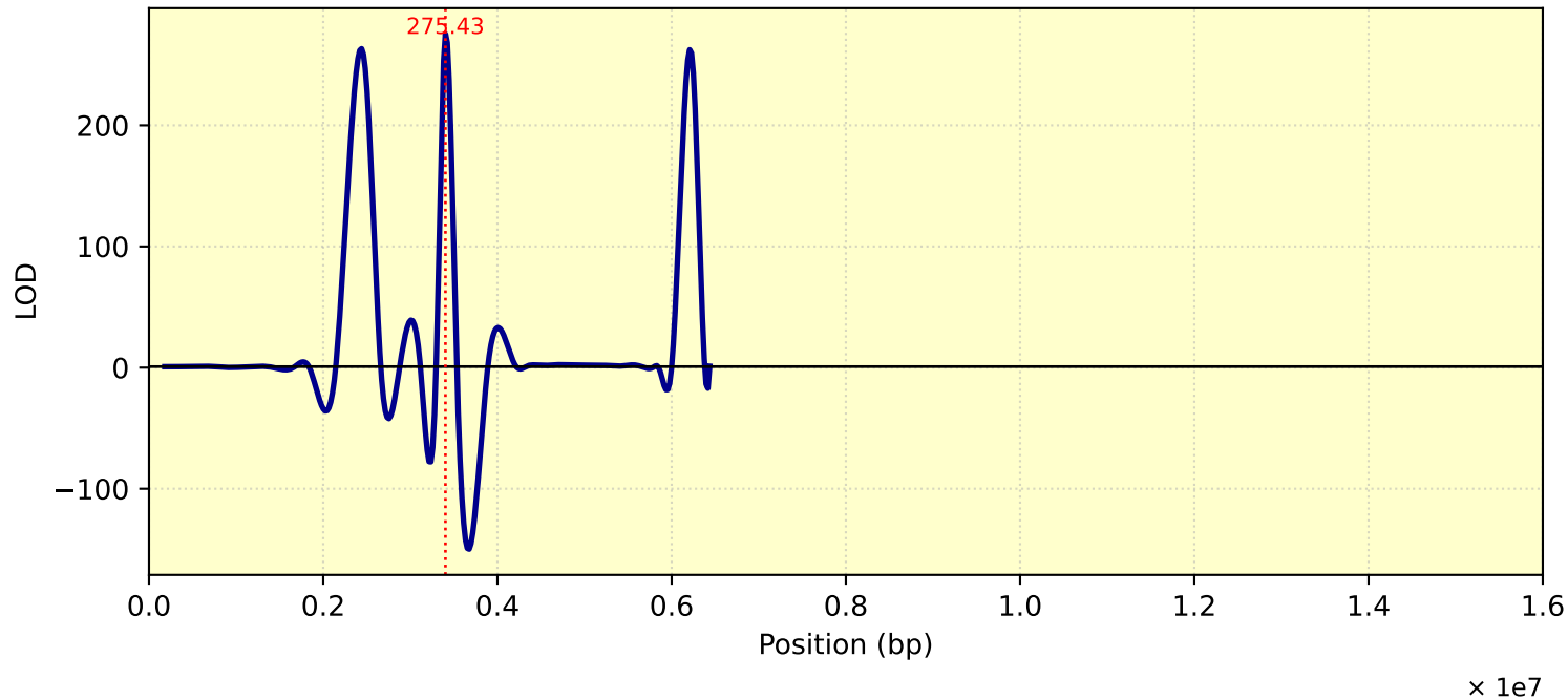
LOD Curve - chr15 - tc27d7m11T1
