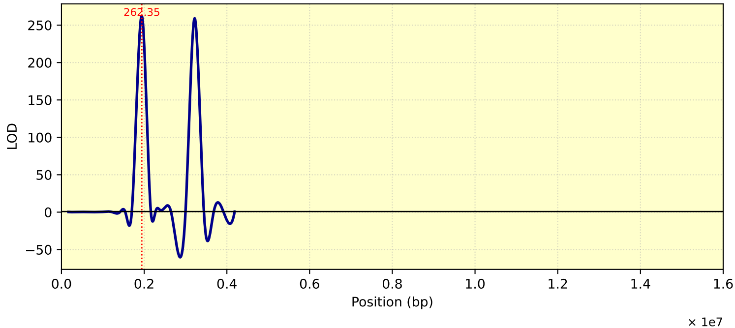
LOD Curve - chr16 - tc27d7m11T1
