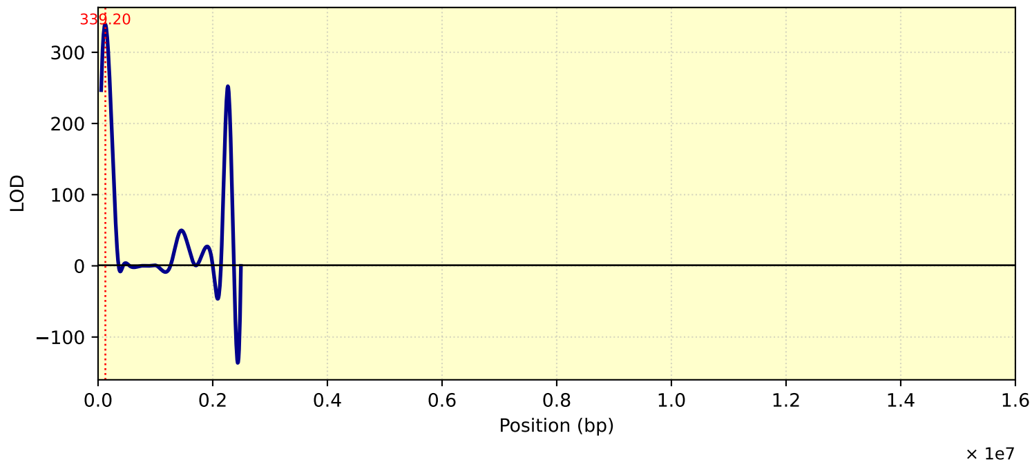
LOD Curve - chr25 - tc27d7m11T1
