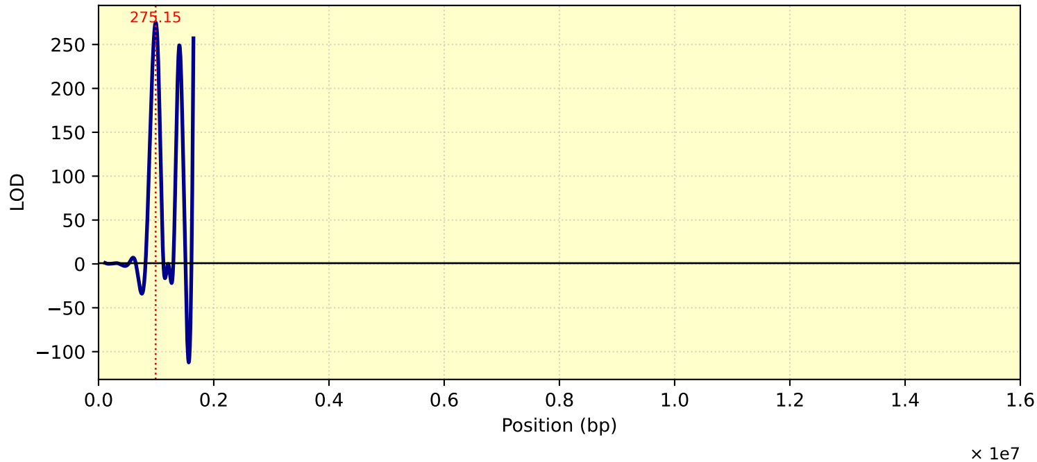
LOD Curve - chr26 - tc27d7m11T1
