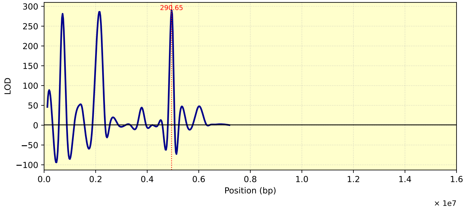
LOD Curve - chr10 - tc27d7m11T1
