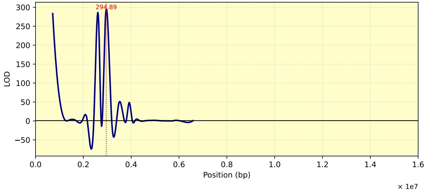
LOD Curve - chr13 - tc27d7m11T1
