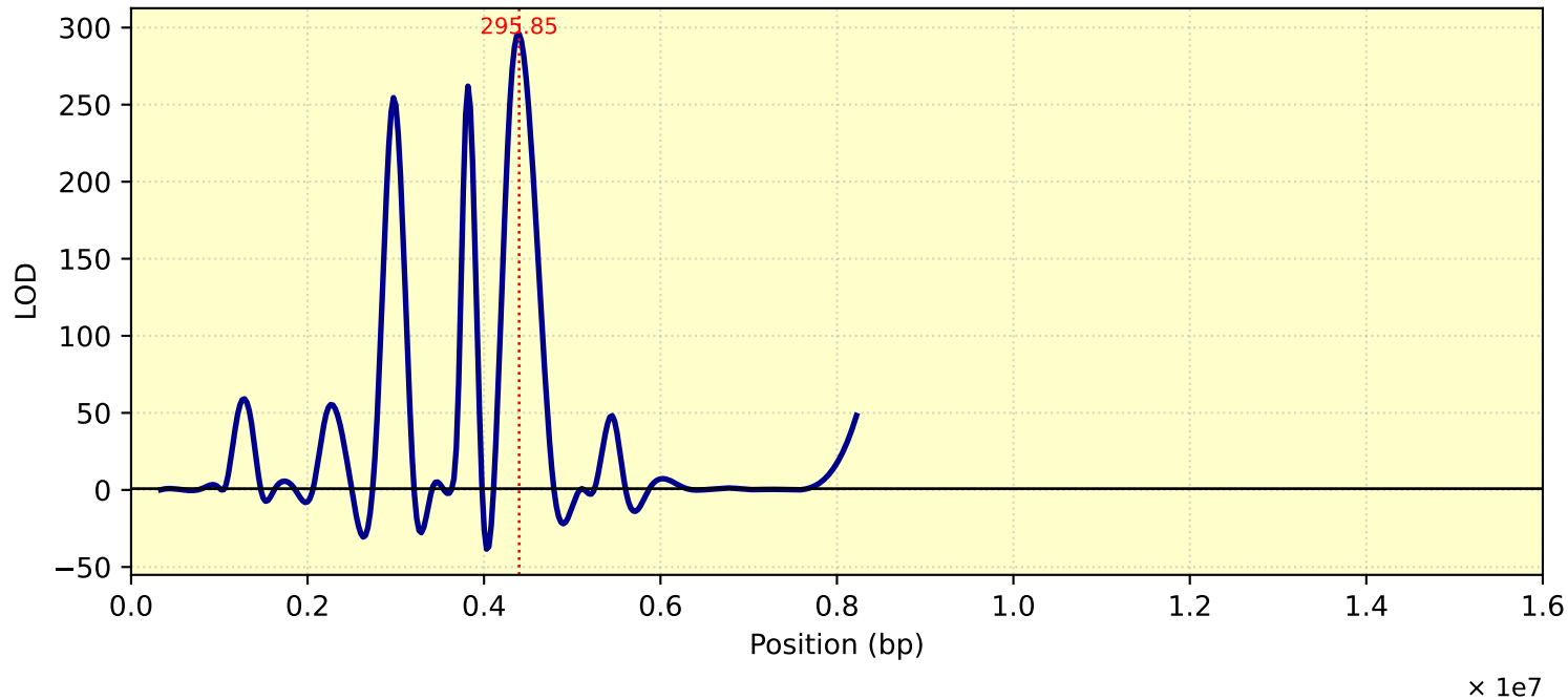
LOD Curve - chr07 - tc27d7m11T1
