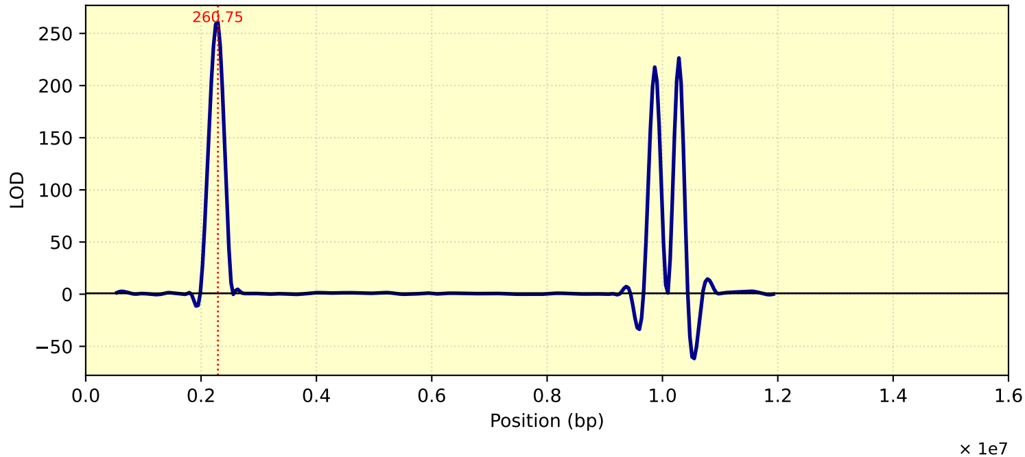
LOD Curve - chr05 - tc27d7m11T1
