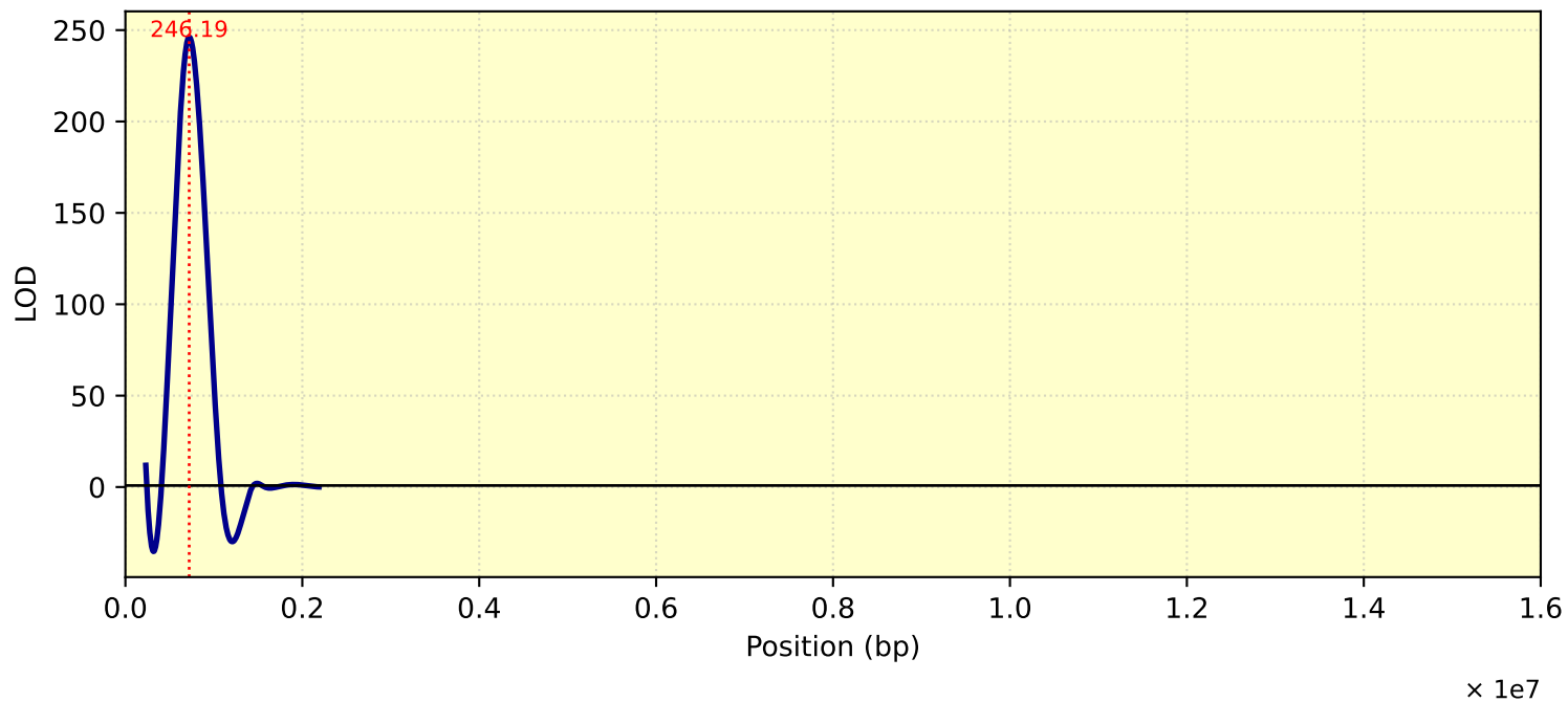
LOD Curve - chr23 - tc27d7m11T1
