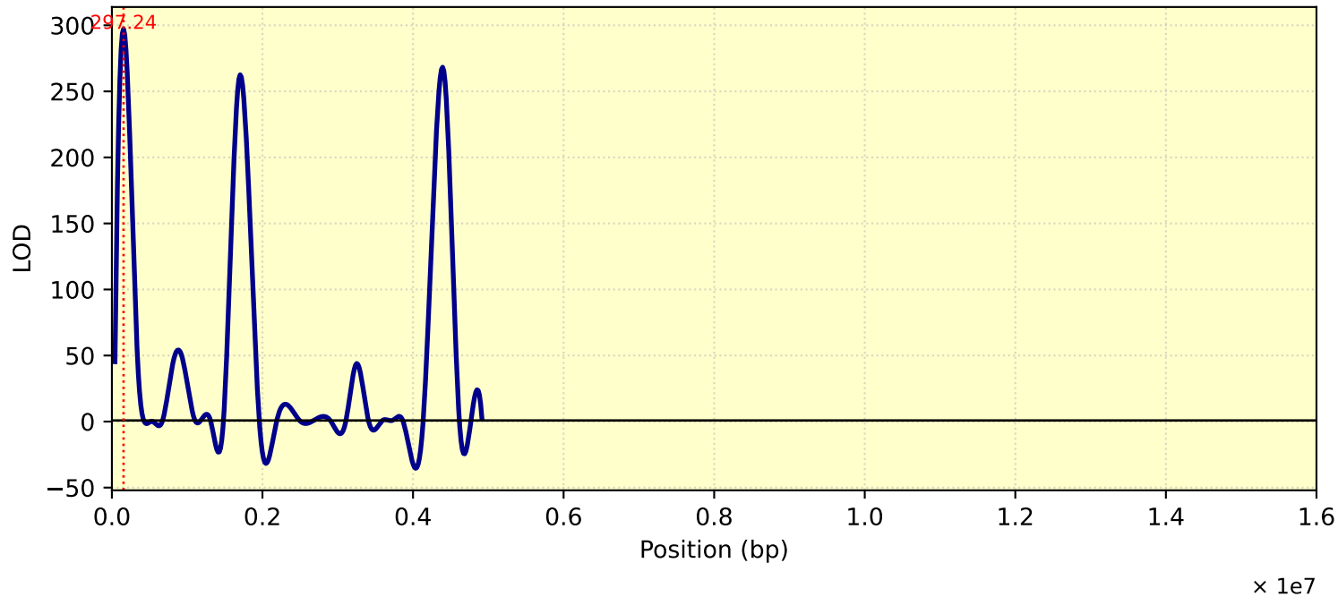
LOD Curve - chr12 - tc27d7m11T1
