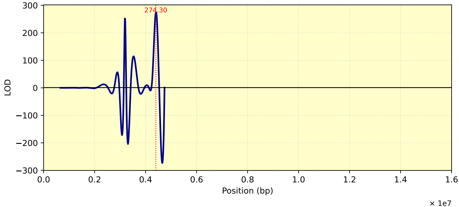
LOD Curve - chr21 - tc27d7m11T1
