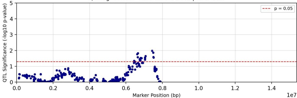
QTL Significance - Chromosome chr08 | Trait: TC29
