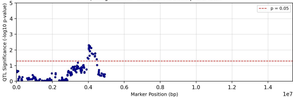
QTL Significance - Chromosome chr19 | Trait: TC29
