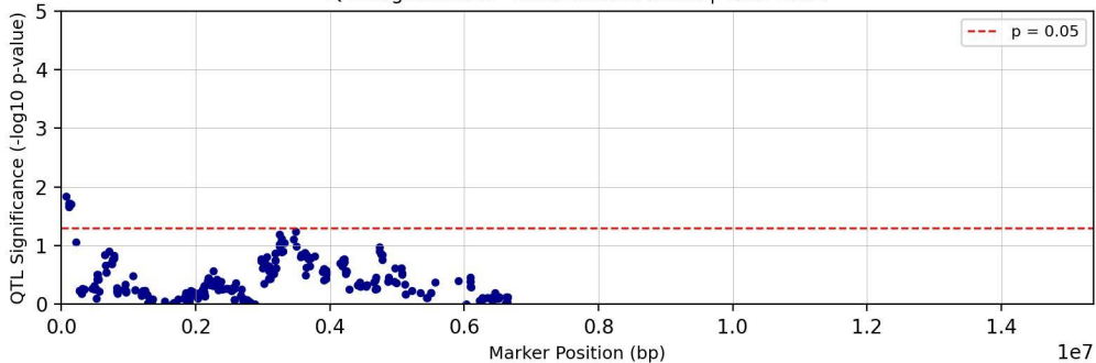
QTL Significance - Chromosome chr11 | Trait: TC29
