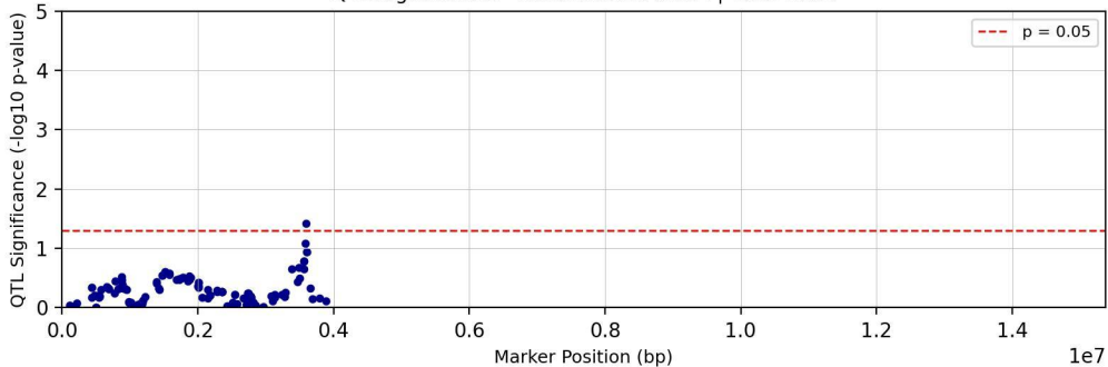
QTL Significance - Chromosome chr24 | Trait: TC29
