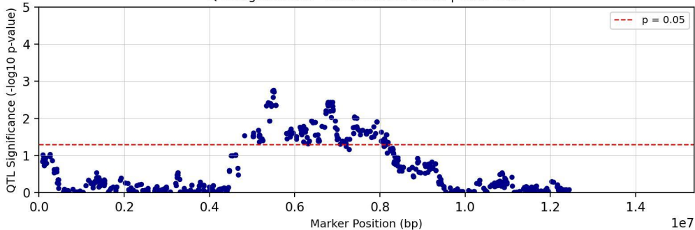
QTL Significance - Chromosome chr03 | Trait: TC29
