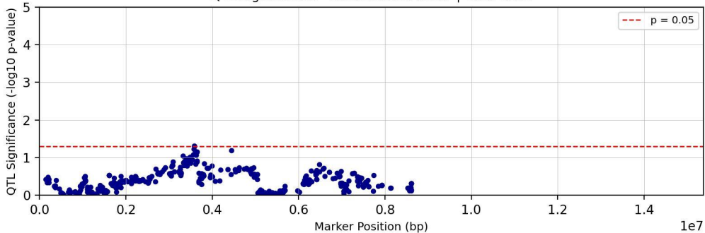
QTL Significance - Chromosome chr07 | Trait: TC29
