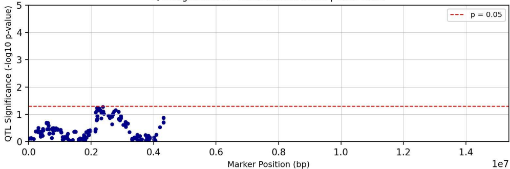
QTL Significance - Chromosome chr16 | Trait: TC29
