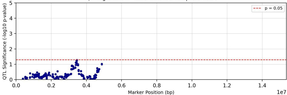
QTL Significance - Chromosome chr21 | Trait: TC29
