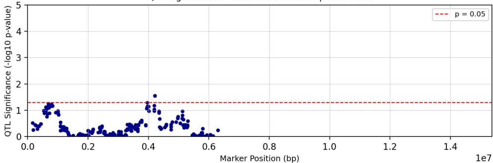
QTL Significance - Chromosome chr14 | Trait: TC29
