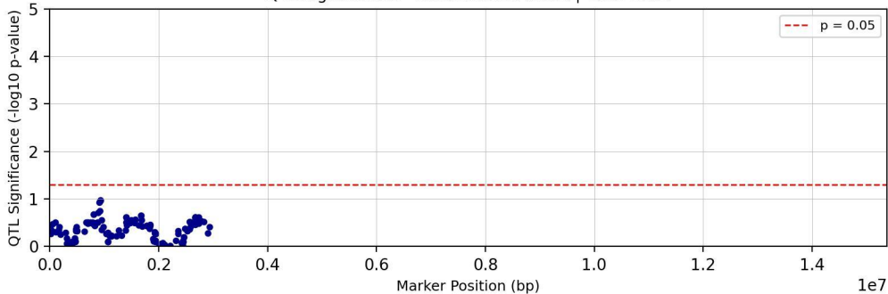
QTL Significance - Chromosome chr25 | Trait: TC29
