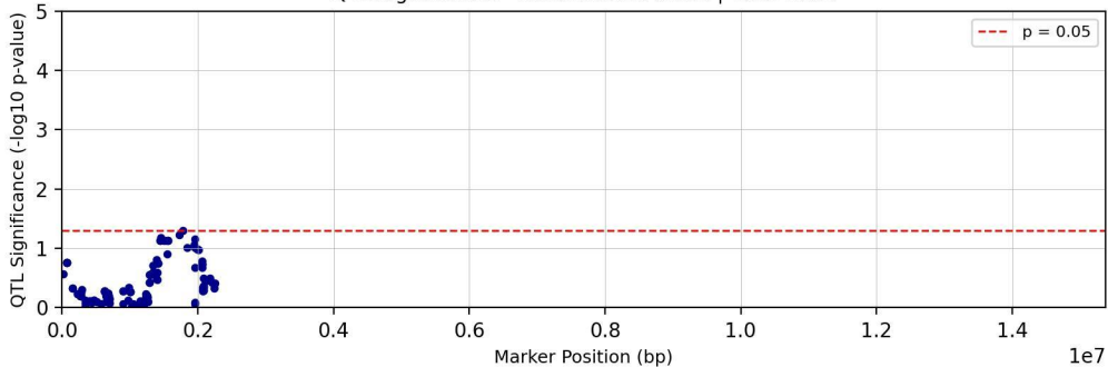
QTL Significance - Chromosome chr26 | Trait: TC29
