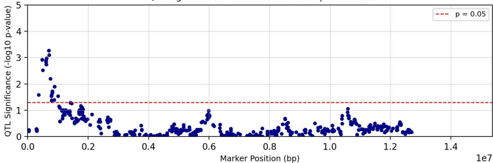
QTL Significance - Chromosome chr02 | Trait: TC29
