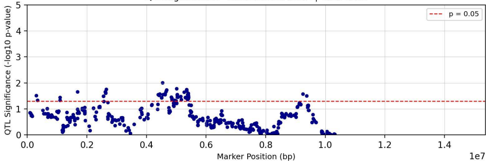
QTL Significance - Chromosome chr04 | Trait: TC29
