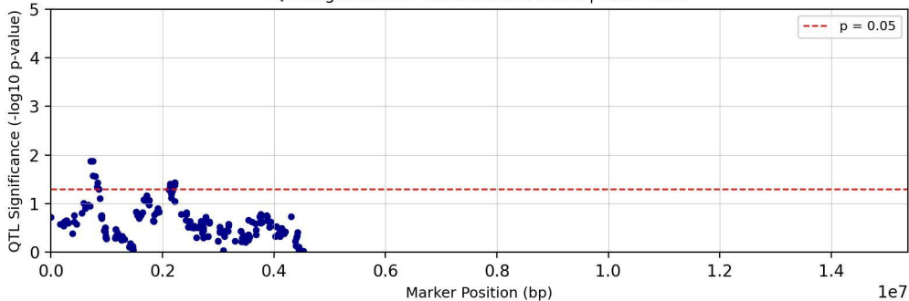
QTL Significance - Chromosome chr22 | Trait: TC29
