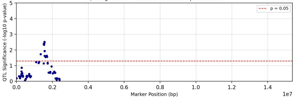
QTL Significance - Chromosome chr23 | Trait: TC29
