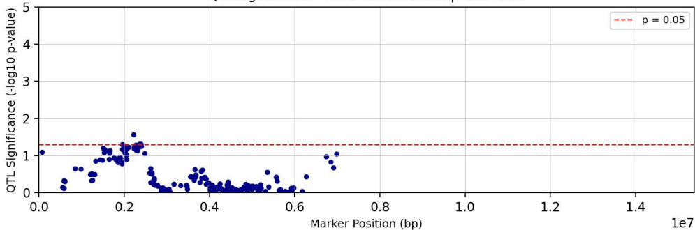
QTL Significance - Chromosome chr13 | Trait: TC29
