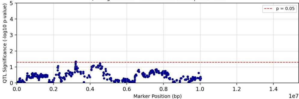
QTL Significance - Chromosome chr06 | Trait: TC29
