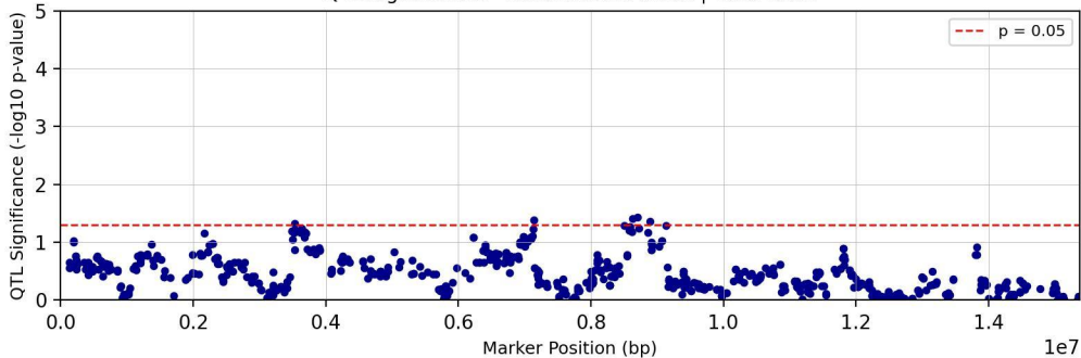
QTL Significance - Chromosome chr01 | Trait: TC29
