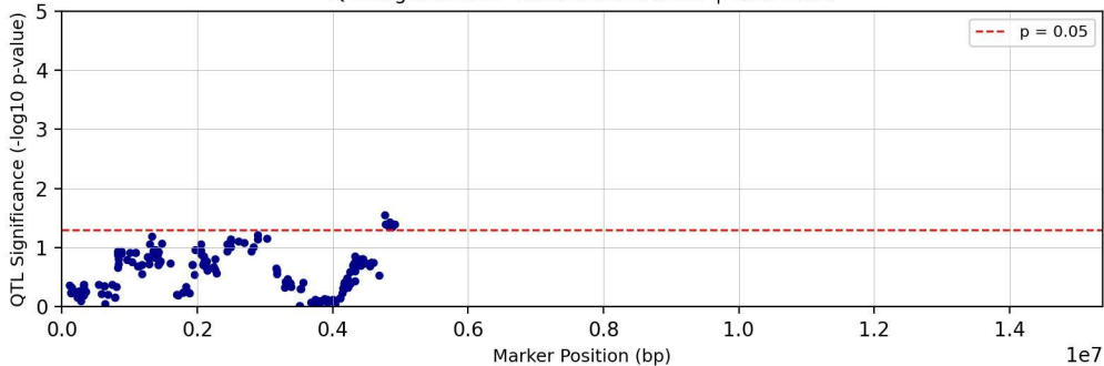
QTL Significance - Chromosome chr17 | Trait: TC29
