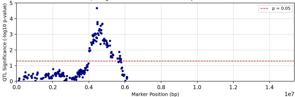
QTL Significance - Chromosome chr18 | Trait: TC29
