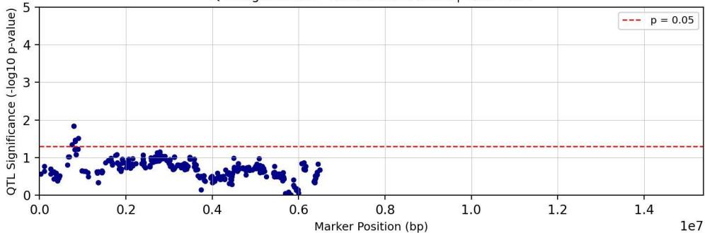
QTL Significance - Chromosome chr15 | Trait: TC29
