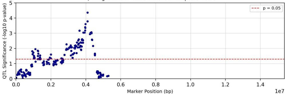
QTL Significance - Chromosome chr12 | Trait: TC29
