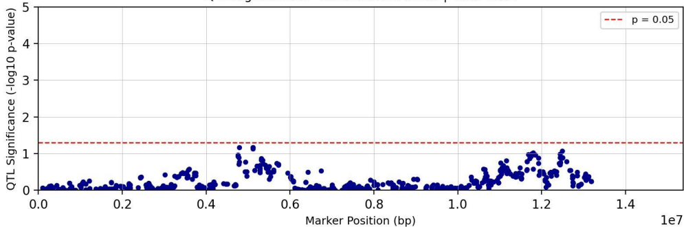
QTL Significance - Chromosome chr09 | Trait: TC29
