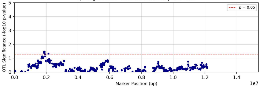
QTL Significance - Chromosome chr05 | Trait: TC29
