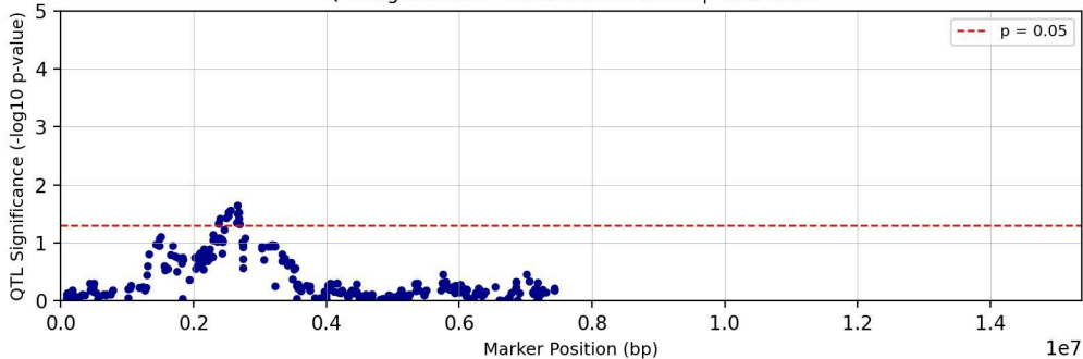
QTL Significance - Chromosome chr10 | Trait: TC29
