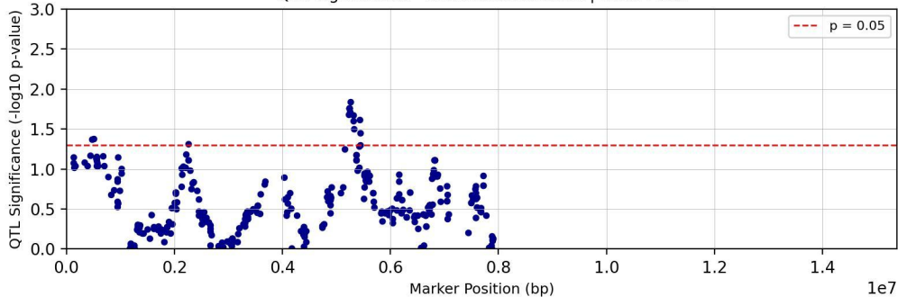
QTL Significance - Chromosome chr08 | Trait: TC30
