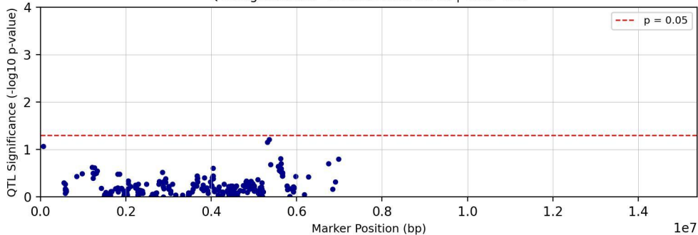
QTL Significance - Chromosome chr13 | Trait: Tc25
