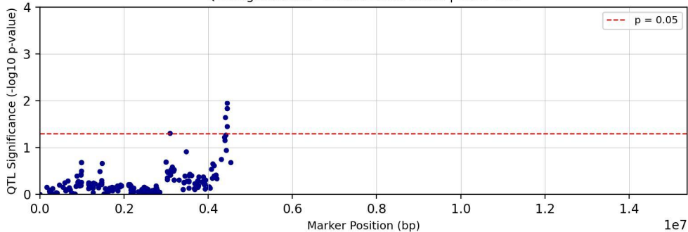
QTL Significance - Chromosome chr22 | Trait: Tc25
