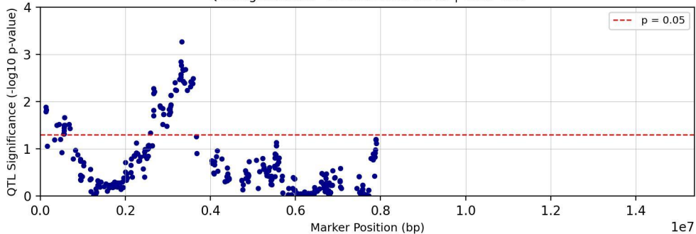
QTL Significance - Chromosome chr08 | Trait: Tc25
