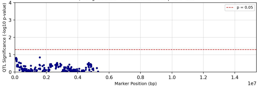
QTL Significance - Chromosome chr12 | Trait: Tc25
