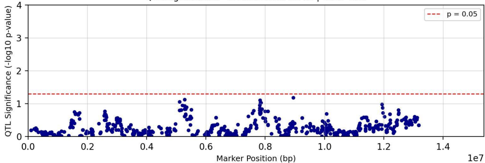
QTL Significance - Chromosome chr09 | Trait: Tc25
