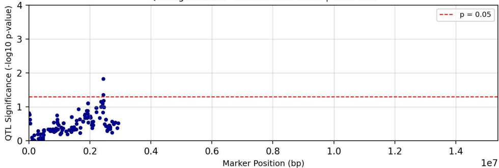
QTL Significance - Chromosome chr25 | Trait: Tc25
