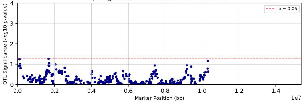
QTL Significance - Chromosome chr04 | Trait: Tc25
