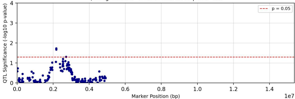
QTL Significance - Chromosome chr19 | Trait: Tc25
