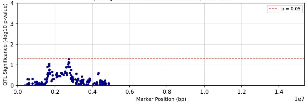
QTL Significance - Chromosome chr21 | Trait: Tc25
