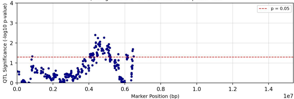
QTL Significance - Chromosome chr15 | Trait: Tc25
