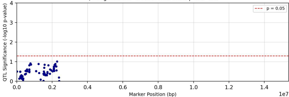
QTL Significance - Chromosome chr23 | Trait: Tc25
