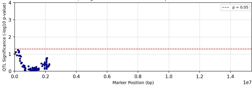
QTL Significance - Chromosome chr26 | Trait: Tc25
