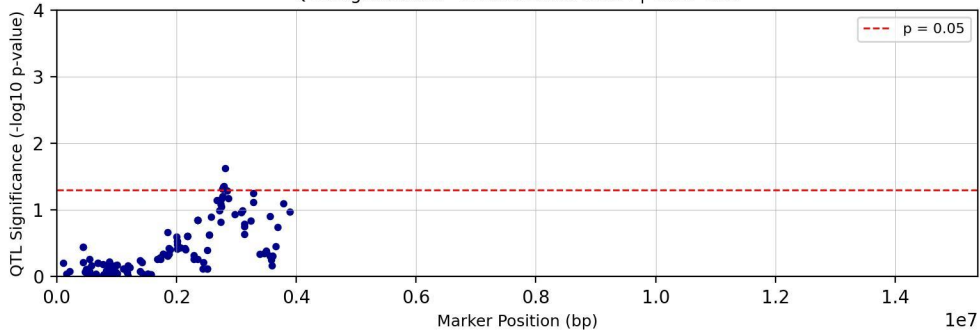
QTL Significance - Chromosome chr24 | Trait: Tc25
