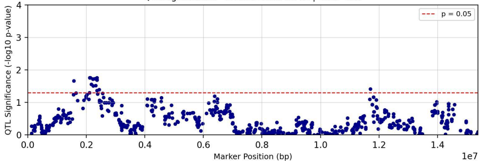
QTL Significance - Chromosome chr01 | Trait: Tc25
