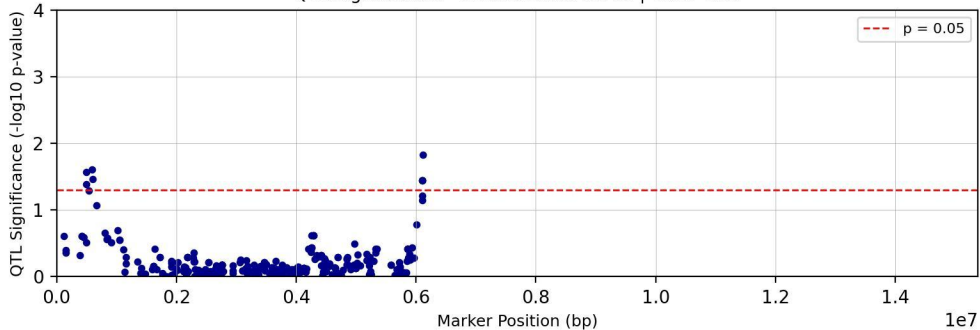
QTL Significance - Chromosome chr18 | Trait: Tc25
