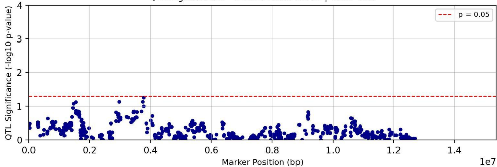
QTL Significance - Chromosome chr02 | Trait: Tc25
