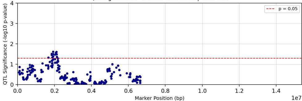
QTL Significance - Chromosome chr11 | Trait: Tc25
