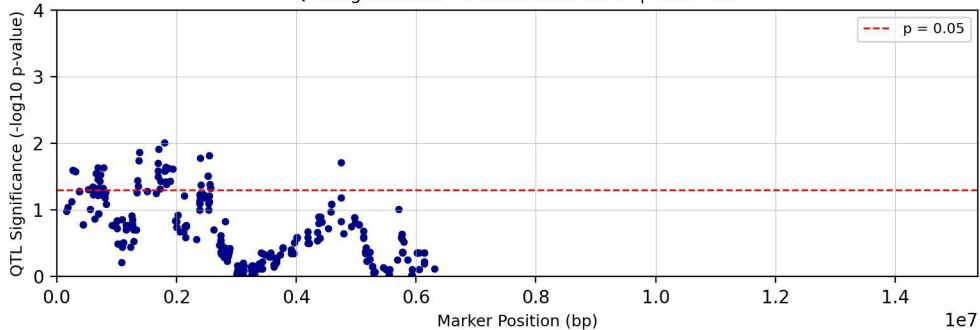
QTL Significance - Chromosome chr14 | Trait: Tc25
