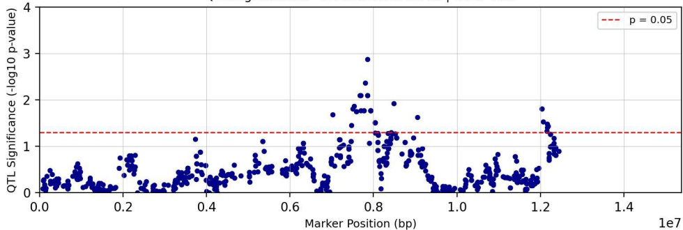
QTL Significance - Chromosome chr03 | Trait: Tc25
