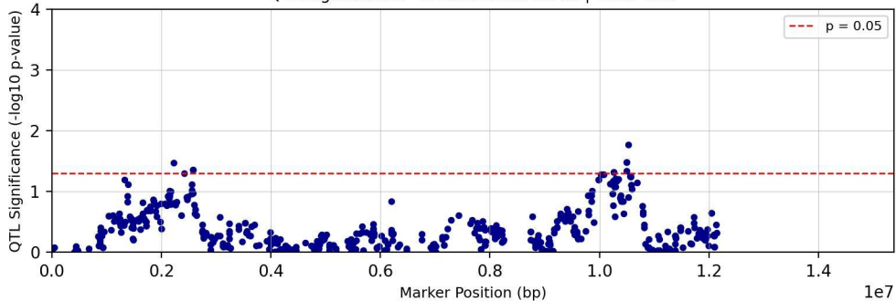
QTL Significance - Chromosome chr05 | Trait: Tc25
