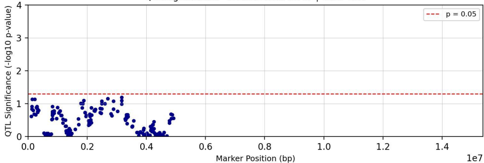
QTL Significance - Chromosome chr17 | Trait: Tc25
