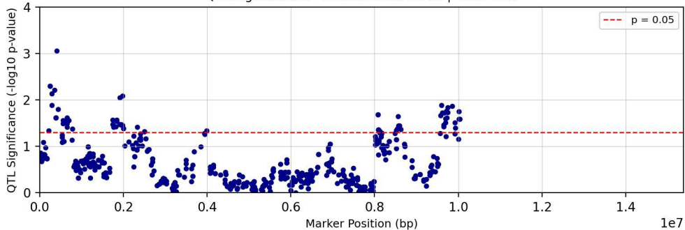
QTL Significance - Chromosome chr06 | Trait: Tc25
