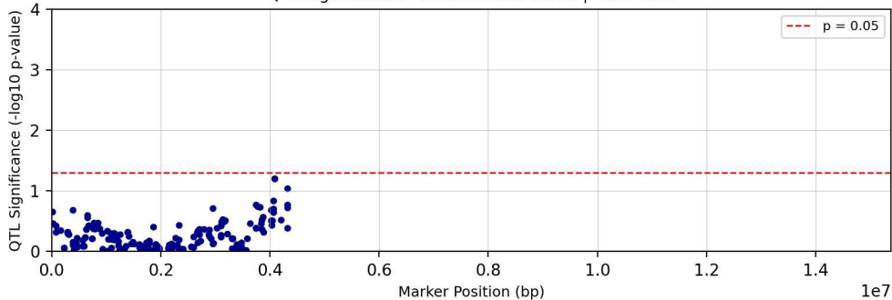
QTL Significance - Chromosome chr16 | Trait: Tc25
