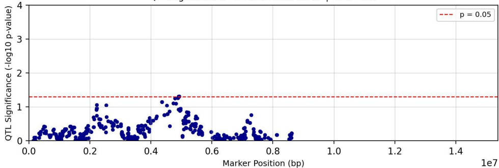
QTL Significance - Chromosome chr07 | Trait: Tc25
