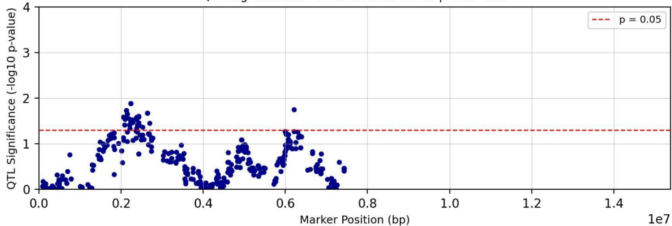
QTL Significance - Chromosome chr10 | Trait: Tc25
