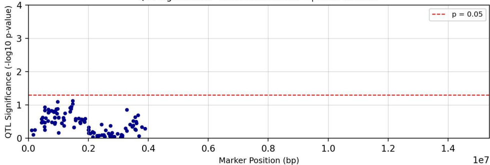
QTL Significance - Chromosome chr24 | Trait: Tc28D1T
