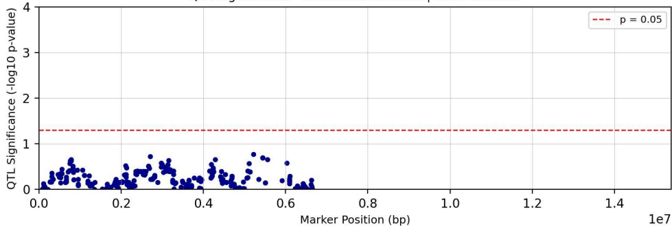
QTL Significance - Chromosome chr11 | Trait: Tc28D1T
