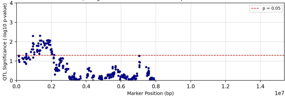
QTL Significance - Chromosome chr08 | Trait: Tc28D1T
