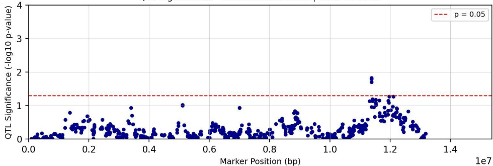
QTL Significance - Chromosome chr09 | Trait: Tc28D1T
