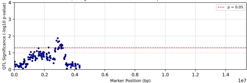
QTL Significance - Chromosome chr16 | Trait: Tc28D1T
