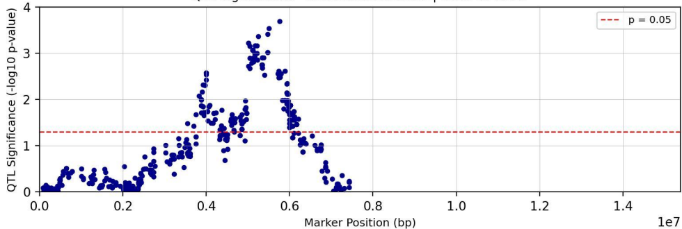
QTL Significance - Chromosome chr10 | Trait: Tc28D1T
