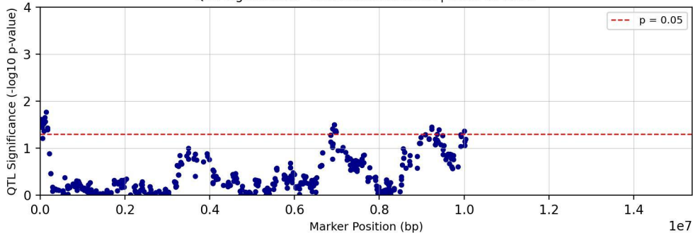
QTL Significance - Chromosome chr06 | Trait: Tc28D1T
