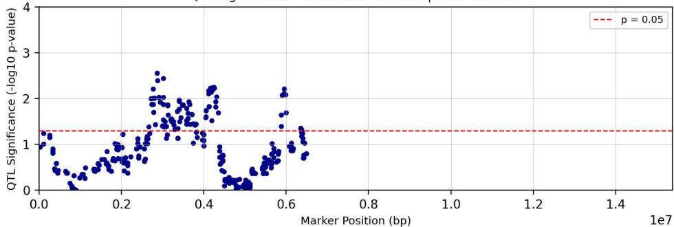
QTL Significance - Chromosome chr15 | Trait: Tc28D1T
