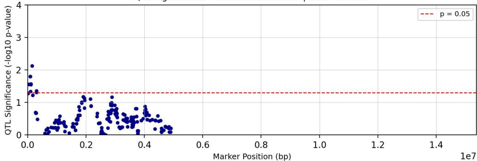
QTL Significance - Chromosome chr19 | Trait: Tc28D1T
