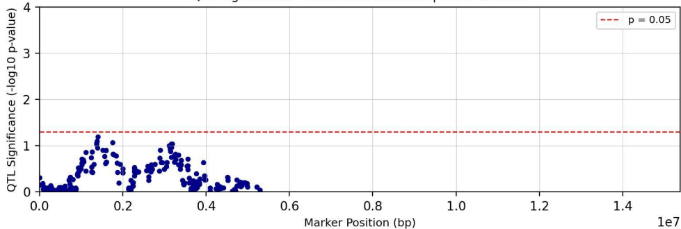
QTL Significance - Chromosome chr12 | Trait: Tc28D1T
