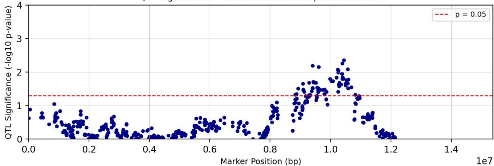
QTL Significance - Chromosome chr05 | Trait: Tc28D1T
