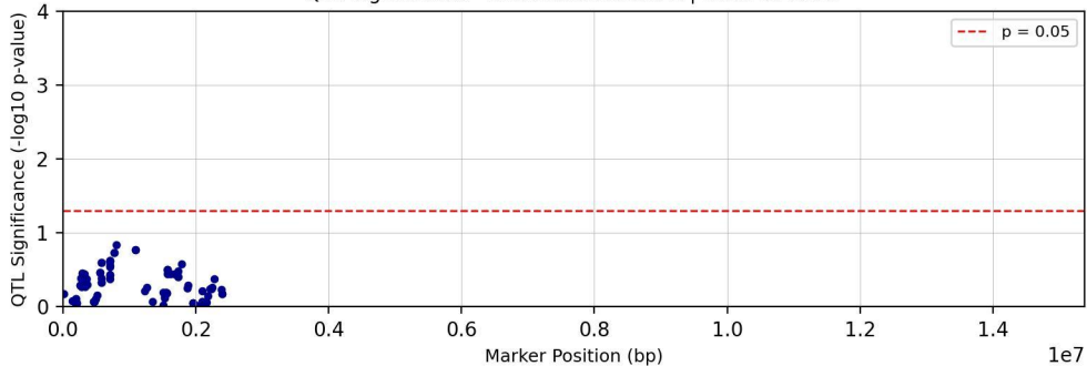
QTL Significance - Chromosome chr23 | Trait: Tc28D1T
