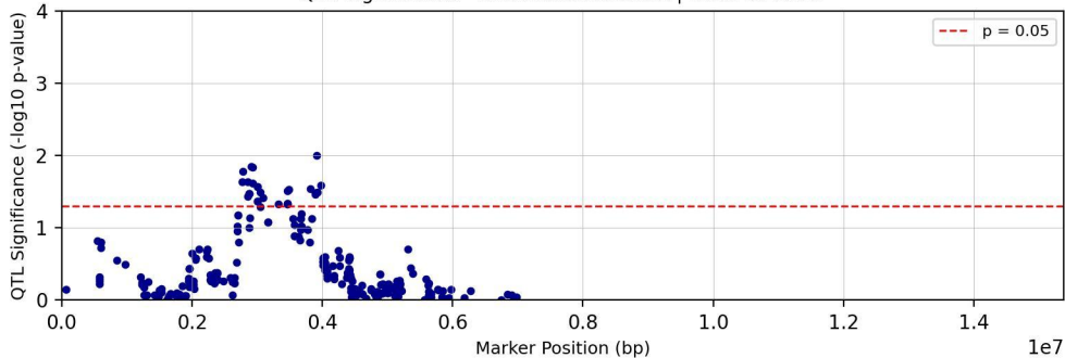
QTL Significance - Chromosome chr13 | Trait: Tc28D1T
