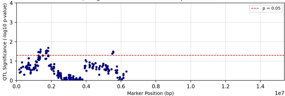
QTL Significance - Chromosome chr14 | Trait: Tc28D1T
