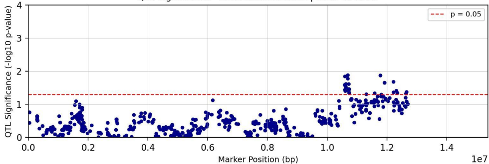
QTL Significance - Chromosome chr02 | Trait: Tc28D1T
