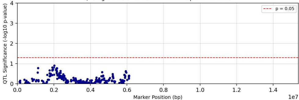
QTL Significance - Chromosome chr18 | Trait: Tc28D1T
