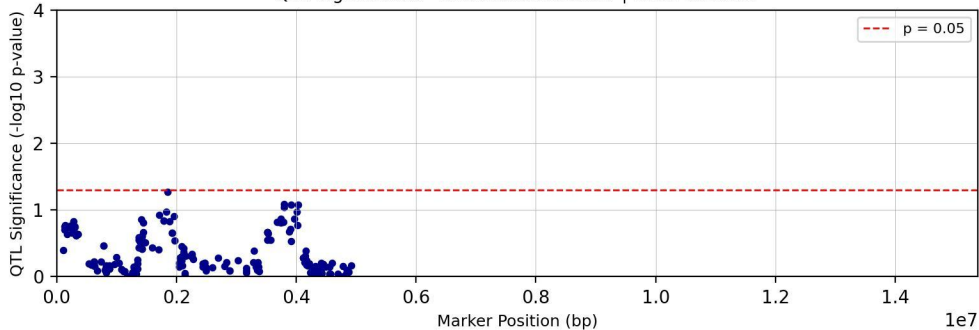
QTL Significance - Chromosome chr17 | Trait: Tc28D1T
