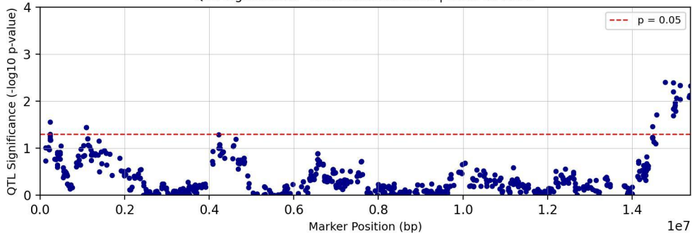
QTL Significance - Chromosome chr01 | Trait: Tc28D1T
