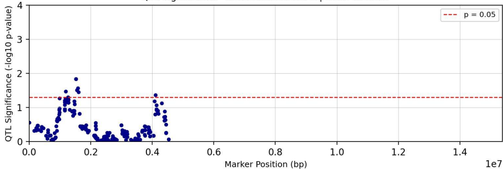
QTL Significance - Chromosome chr22 | Trait: Tc28D1T
