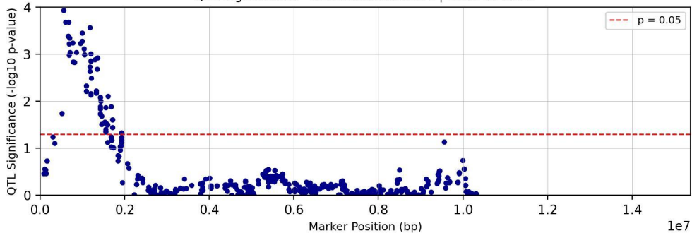
QTL Significance - Chromosome chr04 | Trait: Tc28D1T
