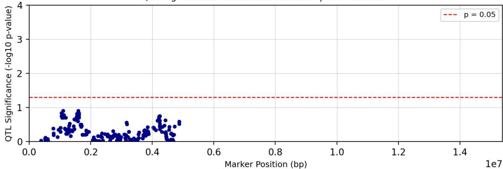
QTL Significance - Chromosome chr21 | Trait: Tc28D1T
