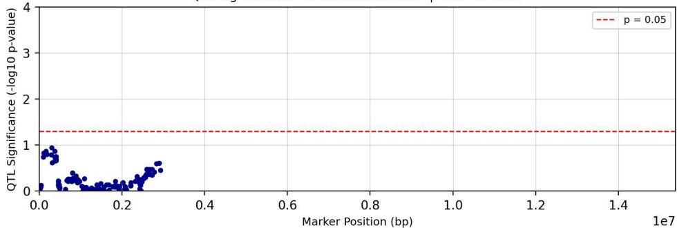
QTL Significance - Chromosome chr25 | Trait: Tc28D1T
