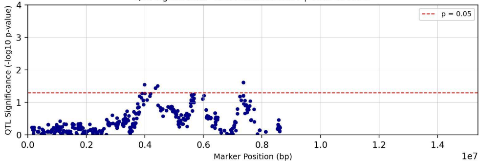
QTL Significance - Chromosome chr07 | Trait: Tc28D1T
