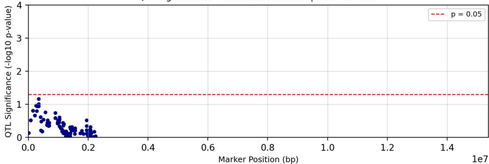
QTL Significance - Chromosome chr26 | Trait: Tc28D1T
