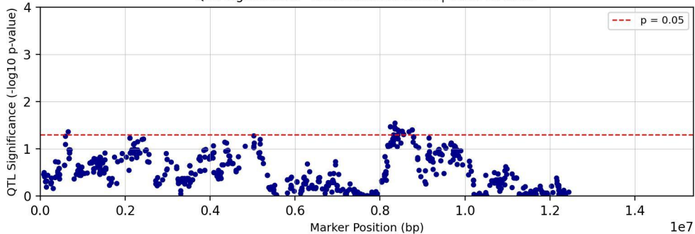
QTL Significance - Chromosome chr03 | Trait: Tc28D1T
