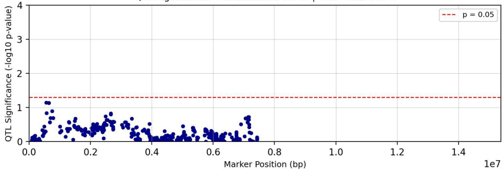
QTL Significance - Chromosome chr10 | Trait: Tc28Me2T1
