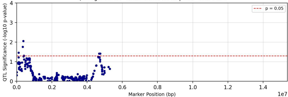
QTL Significance - Chromosome chr12 | Trait: Tc28Me2T1
