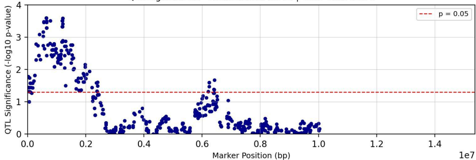
QTL Significance - Chromosome chr06 | Trait: Tc28Me2T1
