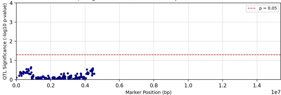
QTL Significance - Chromosome chr22 | Trait: Tc28Me2T1
