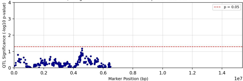
QTL Significance - Chromosome chr15 | Trait: Tc28Me2T1
