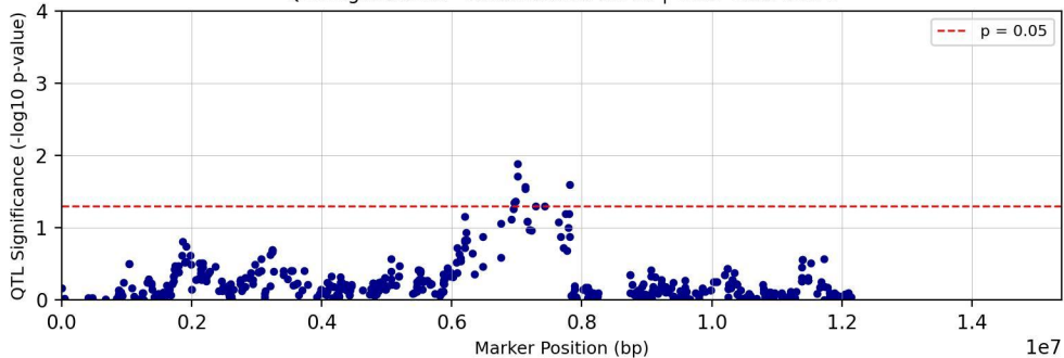
QTL Significance - Chromosome chr05 | Trait: Tc28Me2T1
