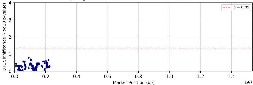
QTL Significance - Chromosome chr26 | Trait: Tc28Me2T1
