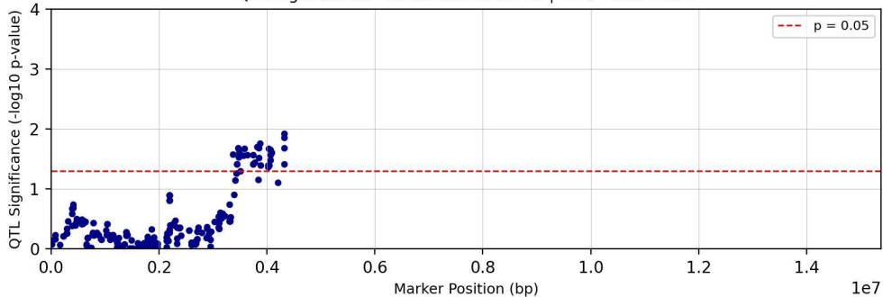
QTL Significance - Chromosome chr16 | Trait: Tc28Me2T1
