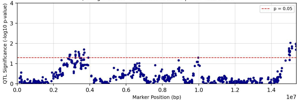
QTL Significance - Chromosome chr01 | Trait: Tc28Me2T1
