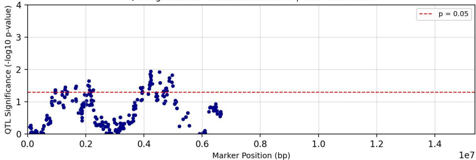
QTL Significance - Chromosome chr11 | Trait: Tc28Me2T1
