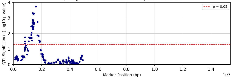
QTL Significance - Chromosome chr17 | Trait: Tc28Me2T1
