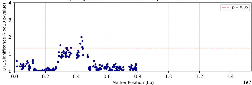
QTL Significance - Chromosome chr08 | Trait: Tc28Me2T1
