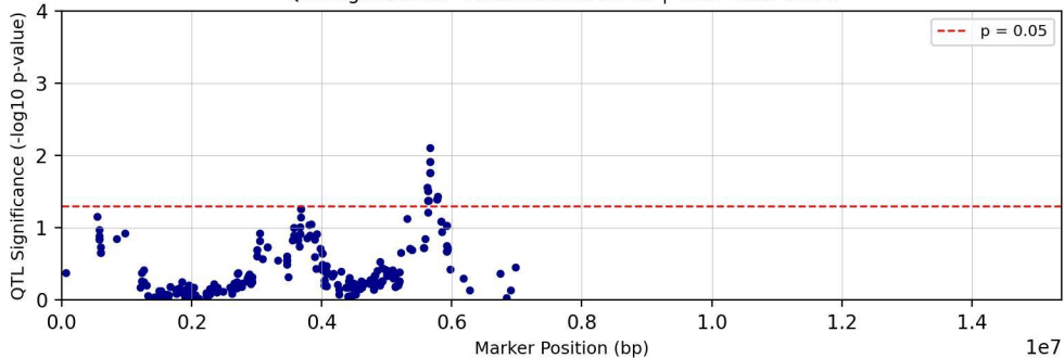
QTL Significance - Chromosome chr13 | Trait: Tc28Me2T1
