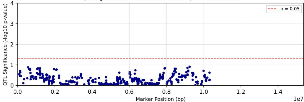
QTL Significance - Chromosome chr04 | Trait: Tc28Me2T1
