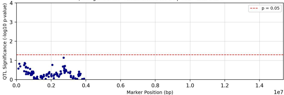
QTL Significance - Chromosome chr24 | Trait: Tc28Me2T1
