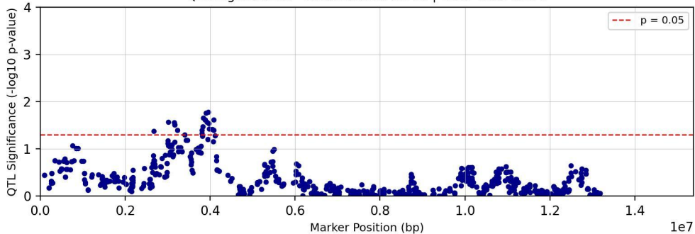
QTL Significance - Chromosome chr09 | Trait: Tc28Me2T1
