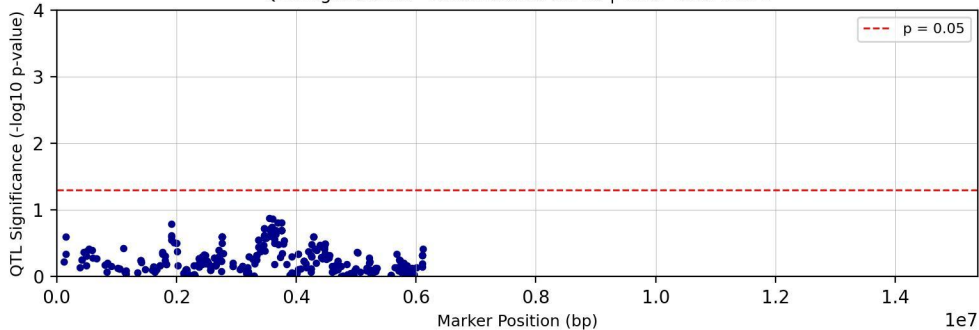
QTL Significance - Chromosome chr18 | Trait: Tc28Me2T1
