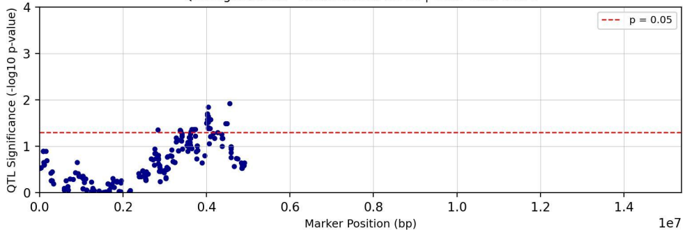
QTL Significance - Chromosome chr19 | Trait: Tc28Me2T1
