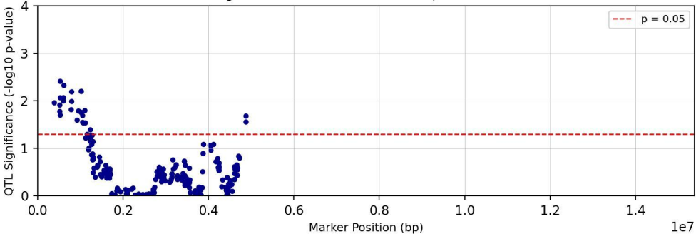
QTL Significance - Chromosome chr21 | Trait: Tc28Me2T1
