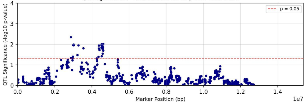
QTL Significance - Chromosome chr02 | Trait: Tc28Me2T1
