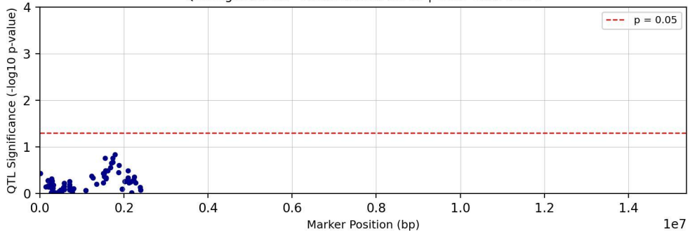
QTL Significance - Chromosome chr23 | Trait: Tc28Me2T1
