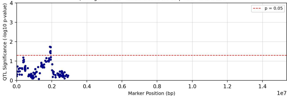
QTL Significance - Chromosome chr25 | Trait: Tc28Me2T1
