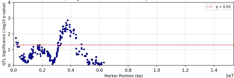
QTL Significance - Chromosome chr14 | Trait: Tc28Me2T1
