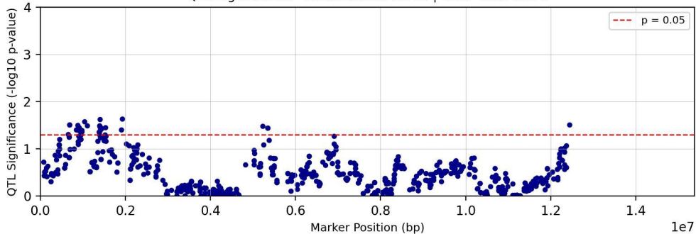
QTL Significance - Chromosome chr03 | Trait: Tc28Me2T1
