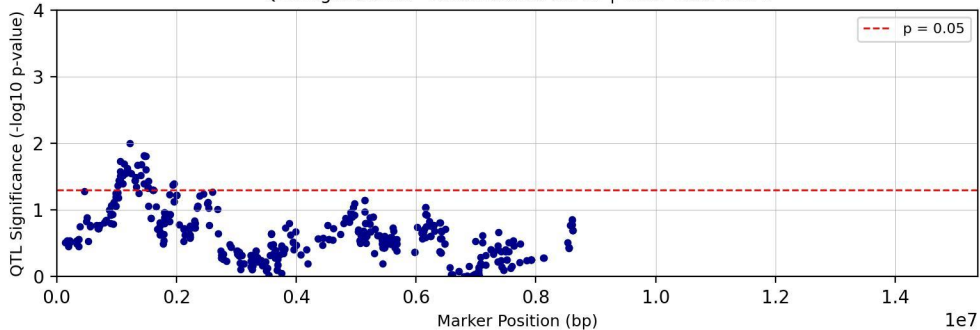
QTL Significance - Chromosome chr07 | Trait: Tc28Me2T1
