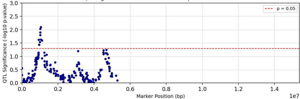
QTL Significance - Chromosome chr12 | Trait: Tc29tri711T
