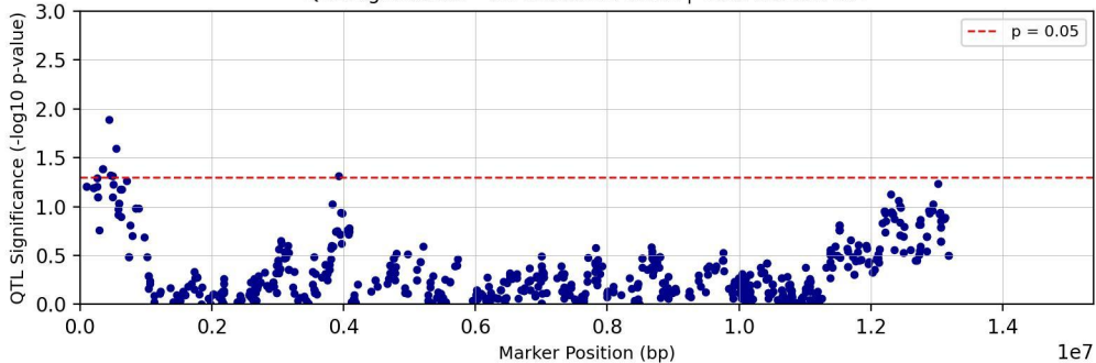
QTL Significance - Chromosome chr09 | Trait: Tc29tri711T
