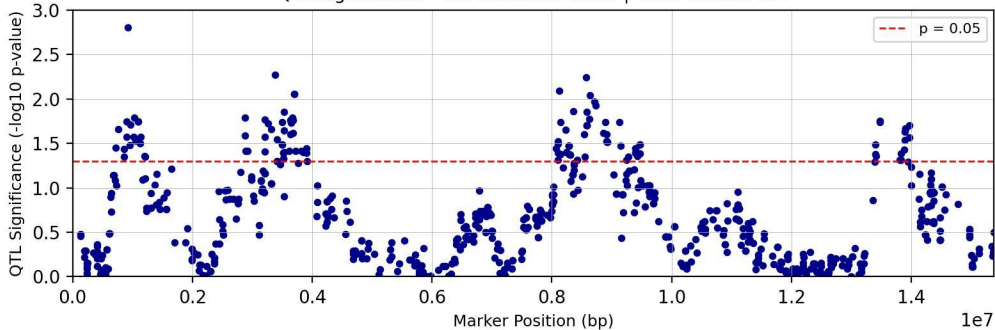
QTL Significance - Chromosome chr01 | Trait: Tc29tri711T
