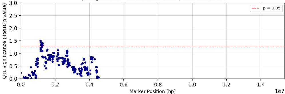
QTL Significance - Chromosome chr22 | Trait: Tc29tri711T
