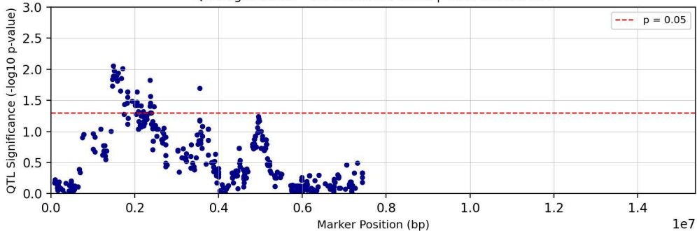
QTL Significance - Chromosome chr10 | Trait: Tc29tri711T
