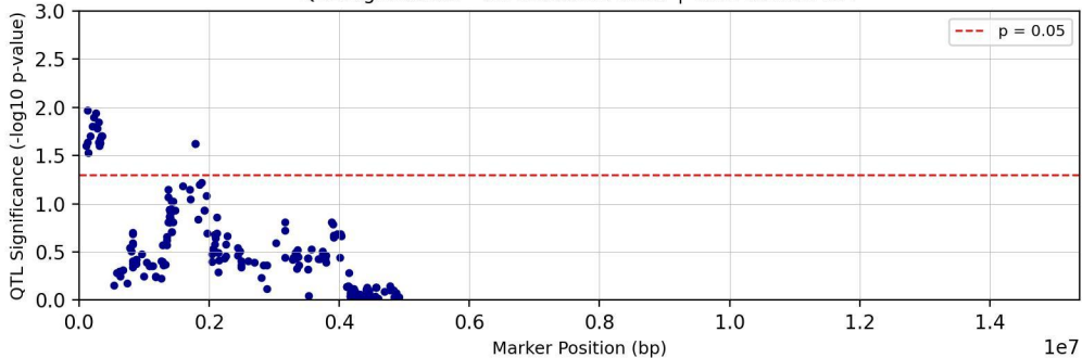
QTL Significance - Chromosome chr17 | Trait: Tc29tri711T
