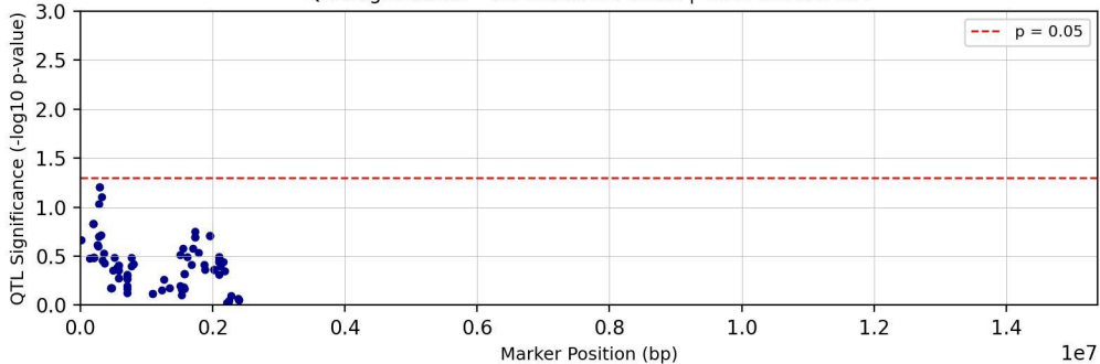
QTL Significance - Chromosome chr23 | Trait: Tc29tri711T
