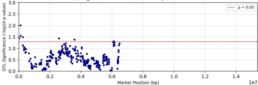
QTL Significance - Chromosome chr15 | Trait: Tc29tri711T
