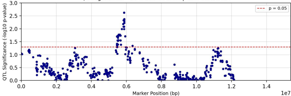
QTL Significance - Chromosome chr05 | Trait: Tc29tri711T
