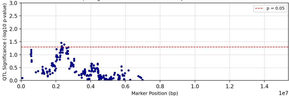
QTL Significance - Chromosome chr13 | Trait: Tc29tri711T
