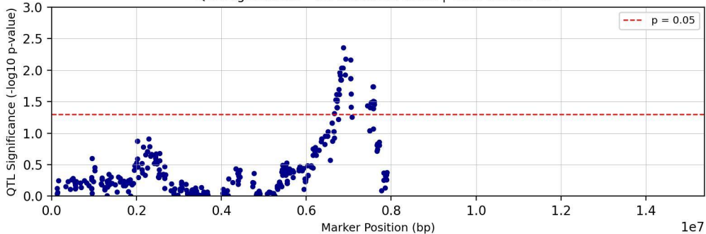
QTL Significance - Chromosome chr08 | Trait: Tc29tri711T
