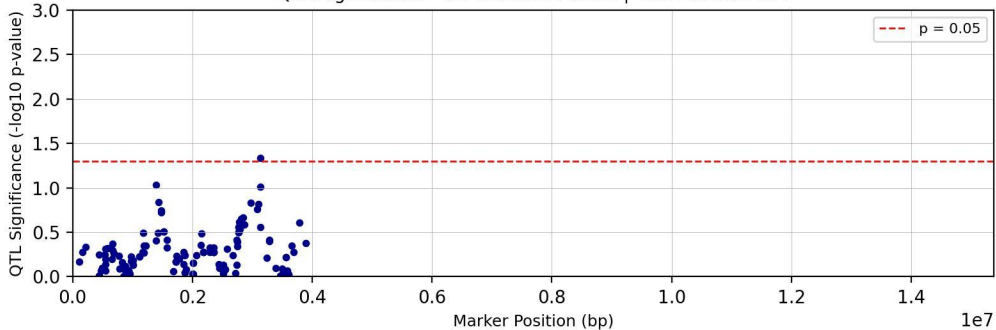
QTL Significance - Chromosome chr24 | Trait: Tc29tri711T
