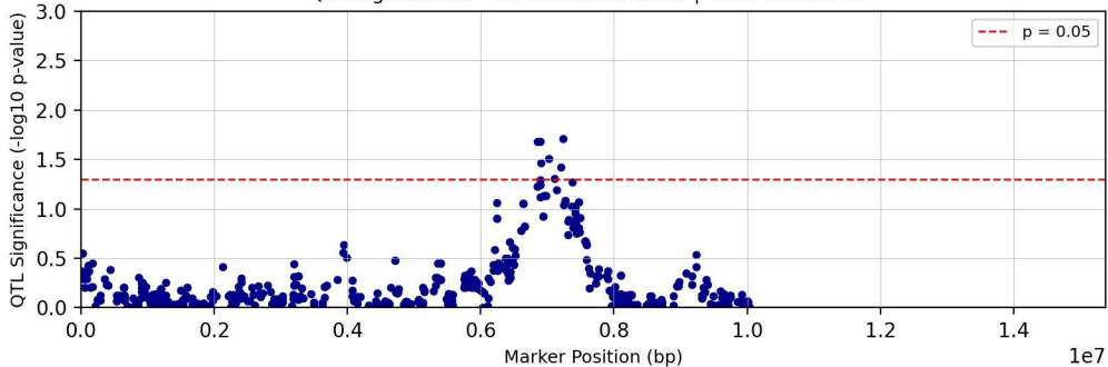
QTL Significance - Chromosome chr06 | Trait: Tc29tri711T
