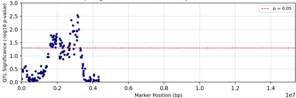
QTL Significance - Chromosome chr16 | Trait: Tc29tri711T
