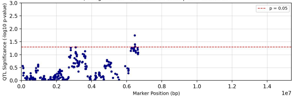
QTL Significance - Chromosome chr11 | Trait: Tc29tri711T
