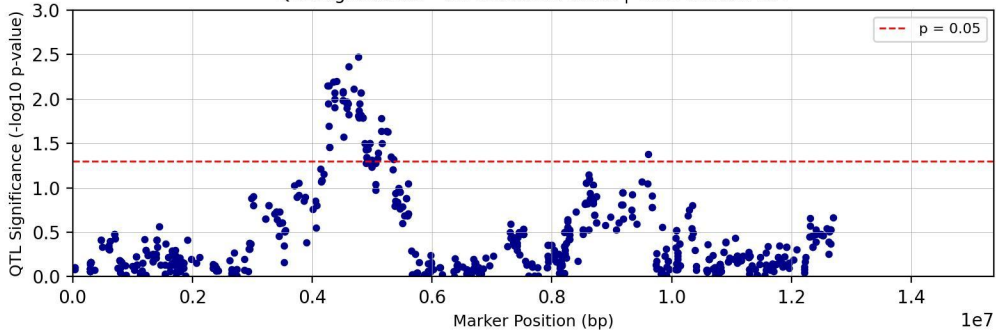
QTL Significance - Chromosome chr02 | Trait: Tc29tri711T
