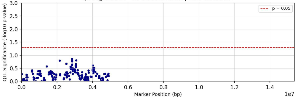
QTL Significance - Chromosome chr19 | Trait: Tc29tri711T
