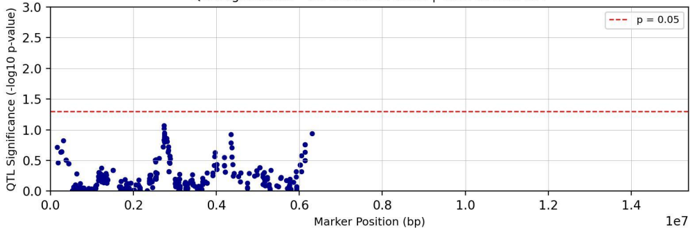
QTL Significance - Chromosome chr14 | Trait: Tc29tri711T
