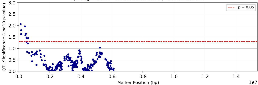
QTL Significance - Chromosome chr18 | Trait: Tc29tri711T
