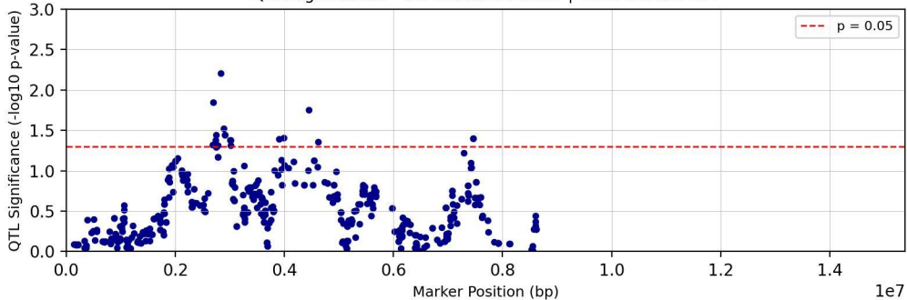
QTL Significance - Chromosome chr07 | Trait: Tc29tri711T
