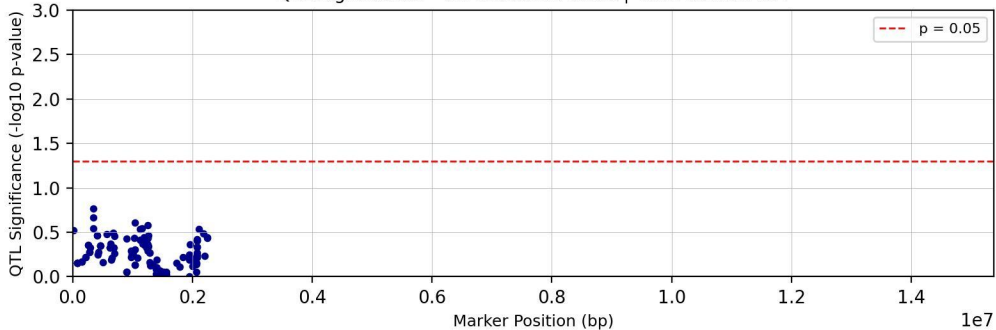
QTL Significance - Chromosome chr26 | Trait: Tc29tri711T
