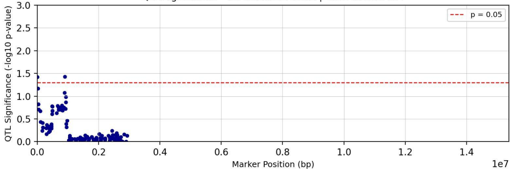
QTL Significance - Chromosome chr25 | Trait: Tc29tri711T
