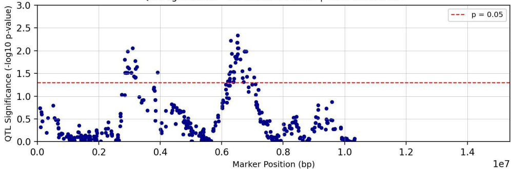
QTL Significance - Chromosome chr04 | Trait: Tc29tri711T
