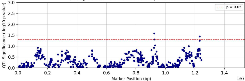
QTL Significance - Chromosome chr03 | Trait: Tc29tri711T
