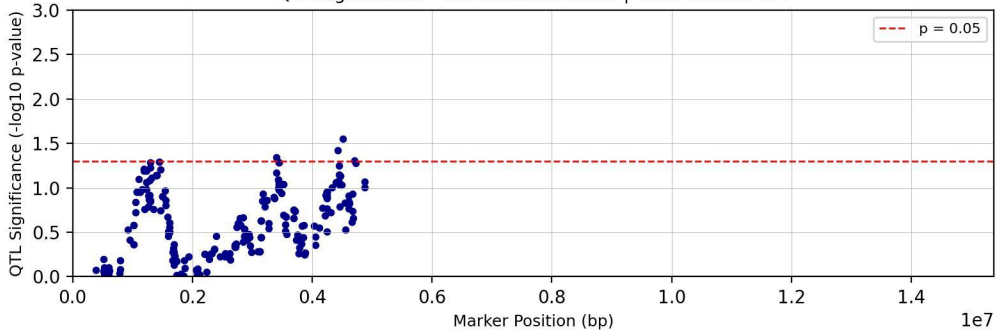
QTL Significance - Chromosome chr21 | Trait: Tc29tri711T
