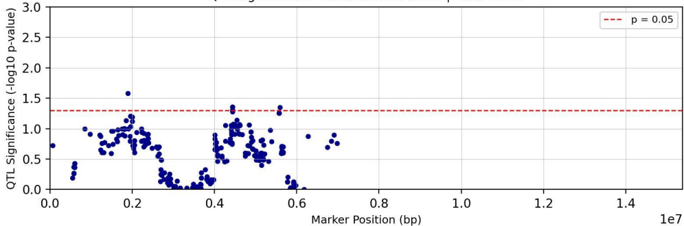
QTL Significance - Chromosome chr13 | Trait: Tc31T
