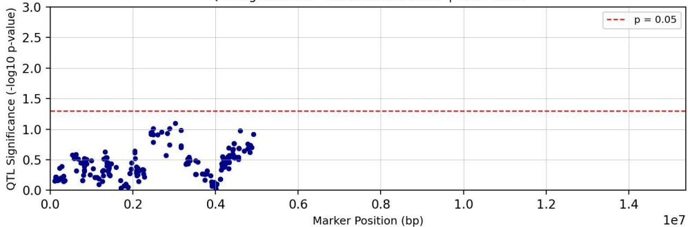
QTL Significance - Chromosome chr17 | Trait: Tc31T
