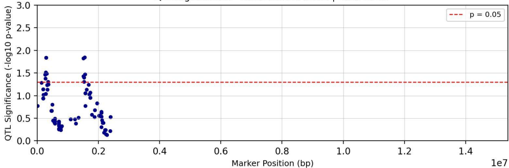
QTL Significance - Chromosome chr23 | Trait: Tc31T
