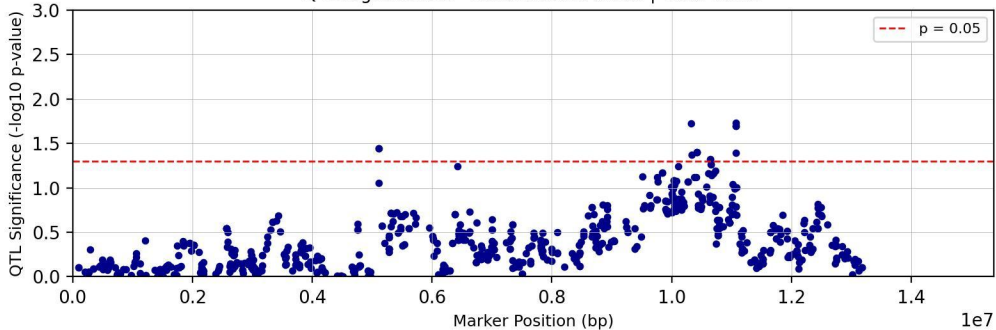
QTL Significance - Chromosome chr09 | Trait: Tc31T
