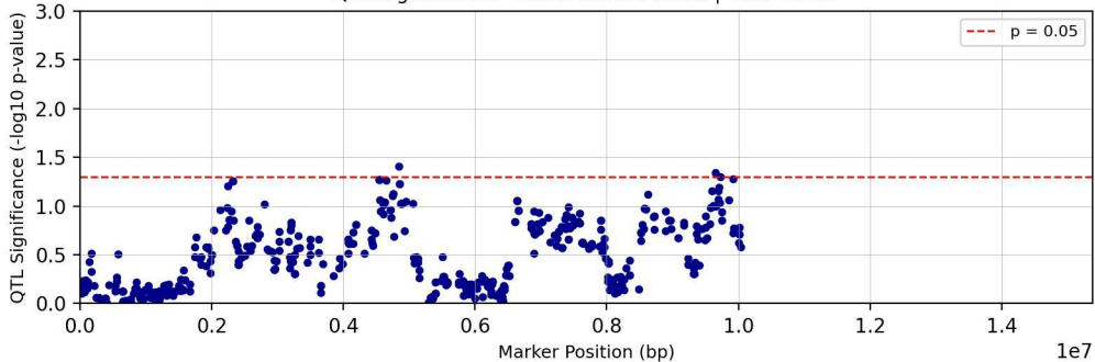
QTL Significance - Chromosome chr06 | Trait: Tc31T
