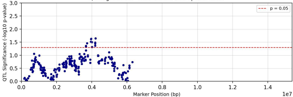
QTL Significance - Chromosome chr14 | Trait: Tc31T
