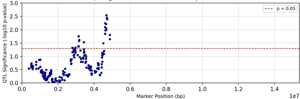
QTL Significance - Chromosome chr21 | Trait: Tc31T
