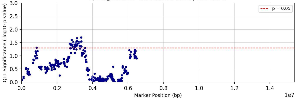
QTL Significance - Chromosome chr15 | Trait: Tc31T
