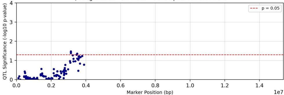
QTL Significance - Chromosome chr24 | Trait: tc27d7m11T1
