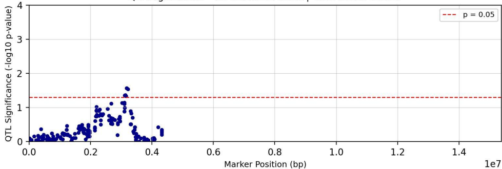
QTL Significance - Chromosome chr16 | Trait: tc27d7m11T1
