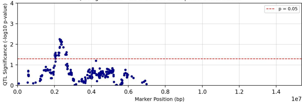
QTL Significance - Chromosome chr13 | Trait: tc27d7m11T1
