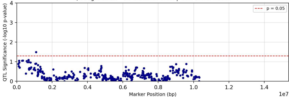
QTL Significance - Chromosome chr04 | Trait: tc27d7m11T1
