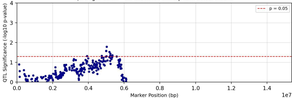
QTL Significance - Chromosome chr18 | Trait: tc27d7m11T1
