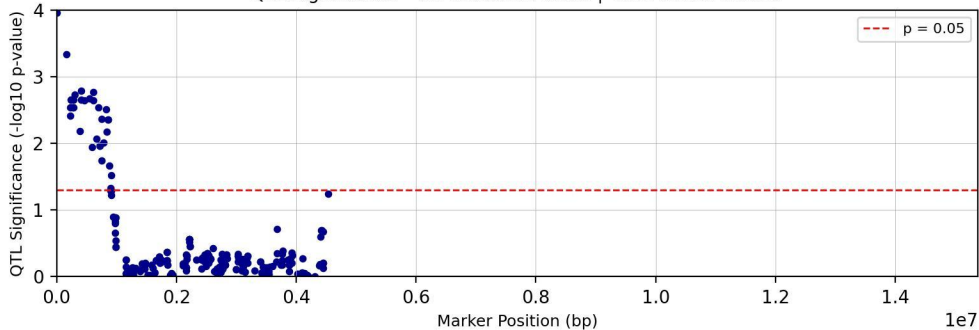
QTL Significance - Chromosome chr22 | Trait: tc27d7m11T1
