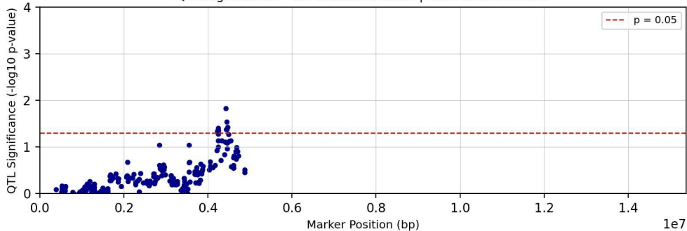
QTL Significance - Chromosome chr21 | Trait: tc27d7m11T1
