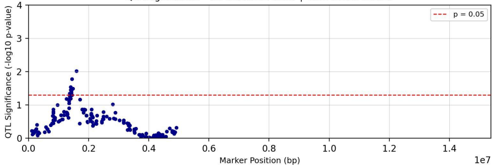
QTL Significance - Chromosome chr17 | Trait: tc27d7m11T1
