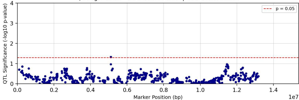
QTL Significance - Chromosome chr09 | Trait: tc27d7m11T1
