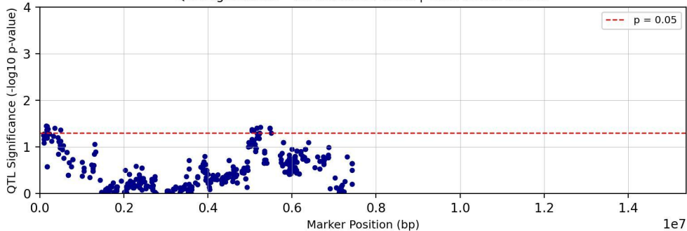
QTL Significance - Chromosome chr10 | Trait: tc27d7m11T1
