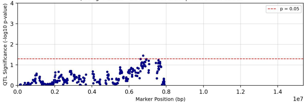
QTL Significance - Chromosome chr08 | Trait: tc27d7m11T1
