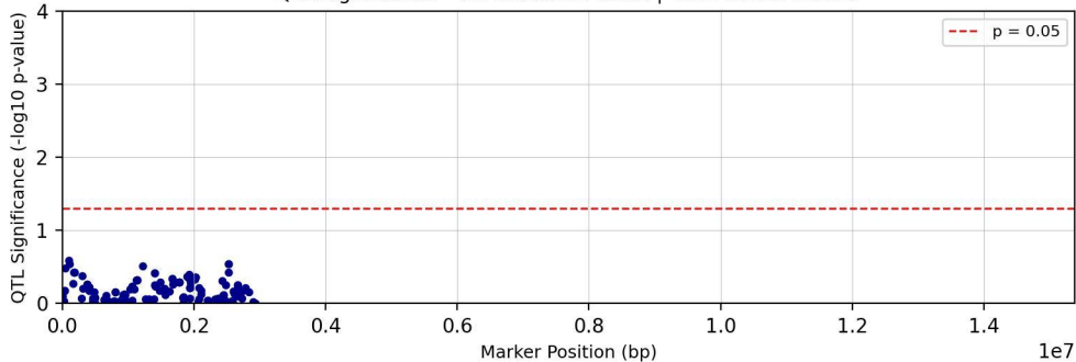
QTL Significance - Chromosome chr25 | Trait: tc27d7m11T1
