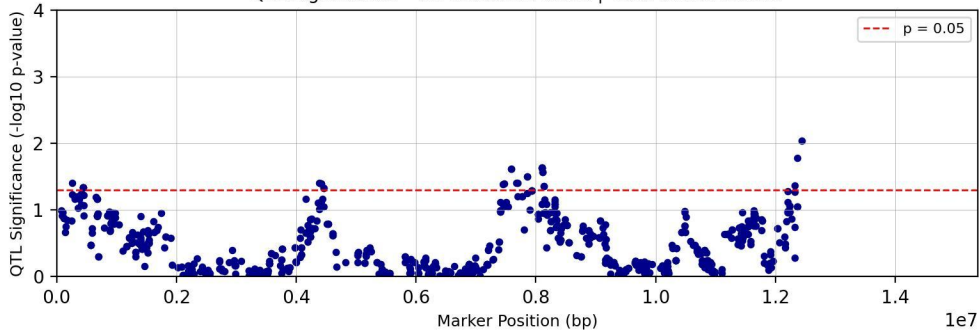
QTL Significance - Chromosome chr03 | Trait: tc27d7m11T1
