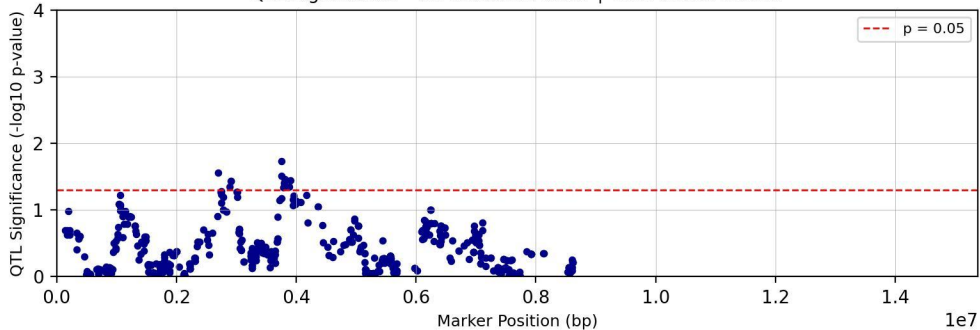
QTL Significance - Chromosome chr07 | Trait: tc27d7m11T1
