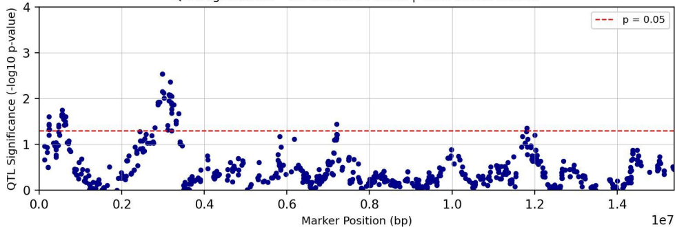
QTL Significance - Chromosome chr01 | Trait: tc27d7m11T1
