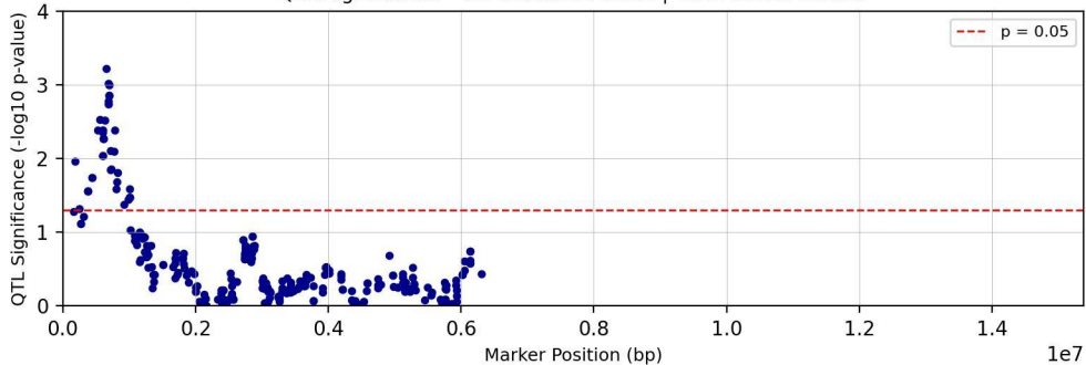
QTL Significance - Chromosome chr14 | Trait: tc27d7m11T1
