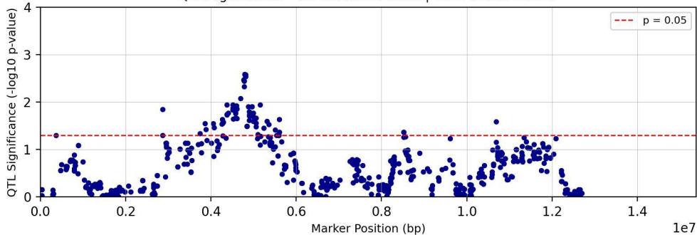
QTL Significance - Chromosome chr02 | Trait: tc27d7m11T1
