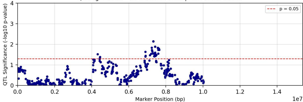
QTL Significance - Chromosome chr06 | Trait: tc27d7m11T1
