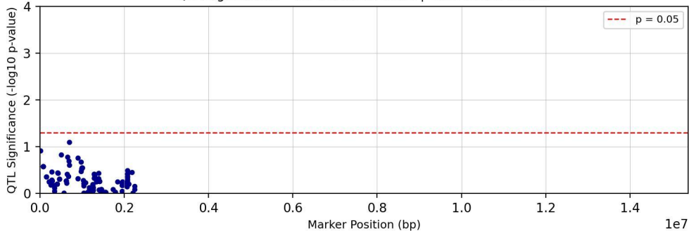
QTL Significance - Chromosome chr26 | Trait: tc27d7m11T1
