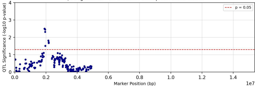
QTL Significance - Chromosome chr19 | Trait: tc27d7m11T1
