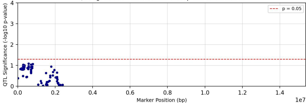
QTL Significance - Chromosome chr23 | Trait: tc27d7m11T1
