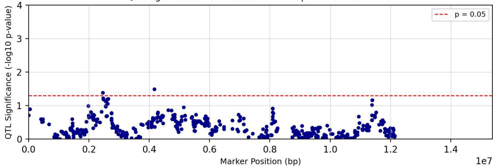
QTL Significance - Chromosome chr05 | Trait: tc27d7m11T1
