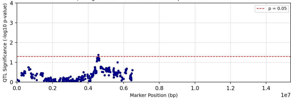
QTL Significance - Chromosome chr15 | Trait: tc27d7m11T1
