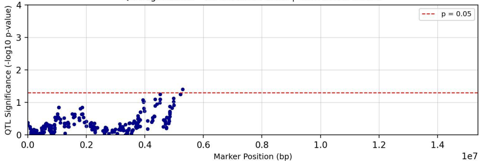
QTL Significance - Chromosome chr12 | Trait: tc27d7m11T1
