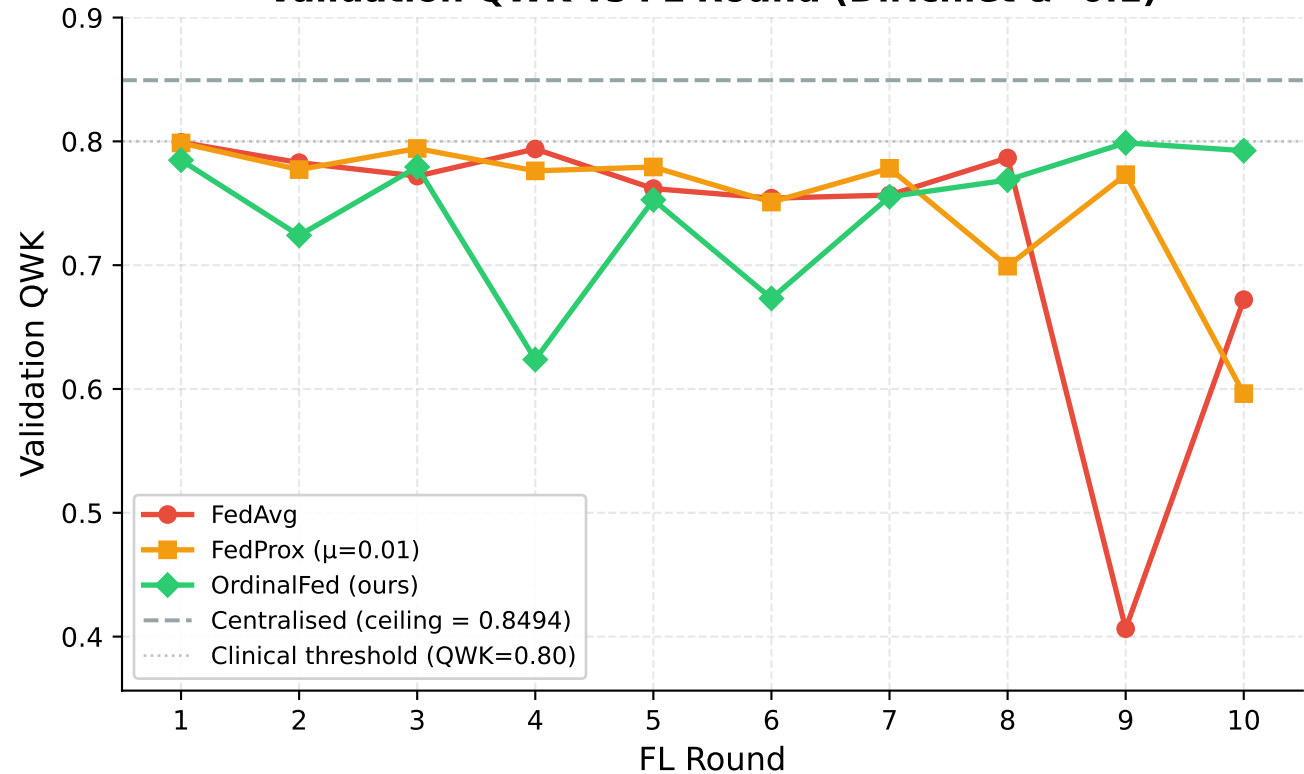
Validation QWK vs FL Round (Dirichlet \alpha=0.1 )
