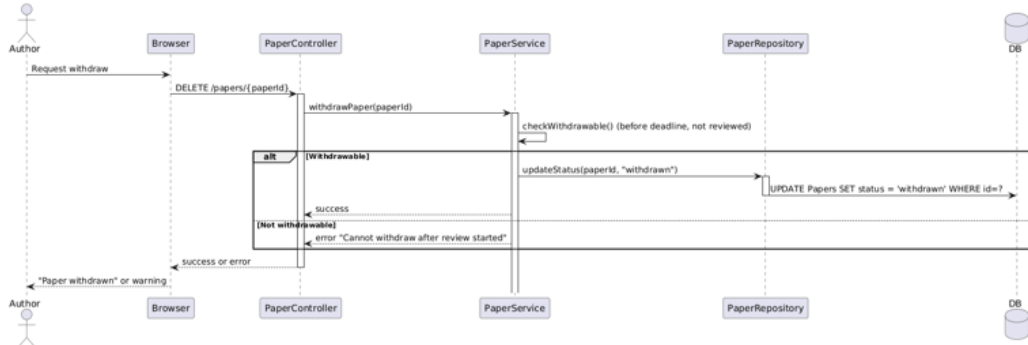
Sequence Diagram - Withdraw Paper
