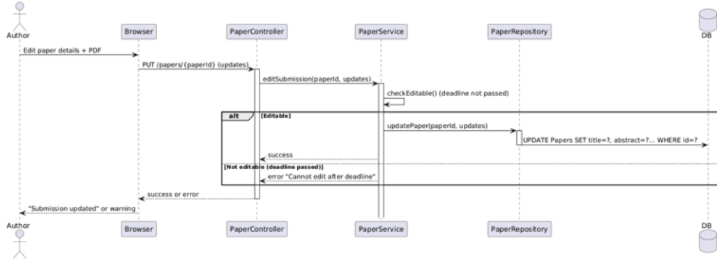
Sequence Diagram - Edit Submission
