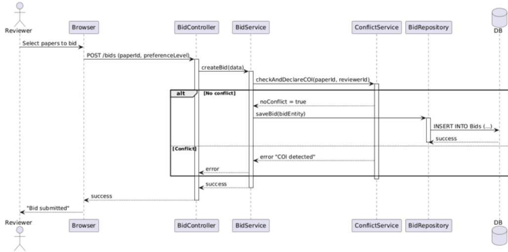
Sequence Diagram - Bid Papers & Declare COI
