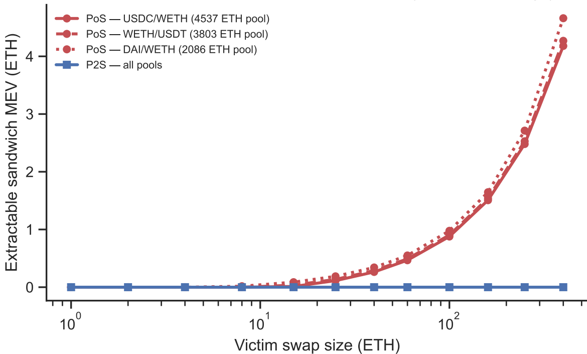
Measured sandwich MEV on real V2 reserves (1% victim slippage)
