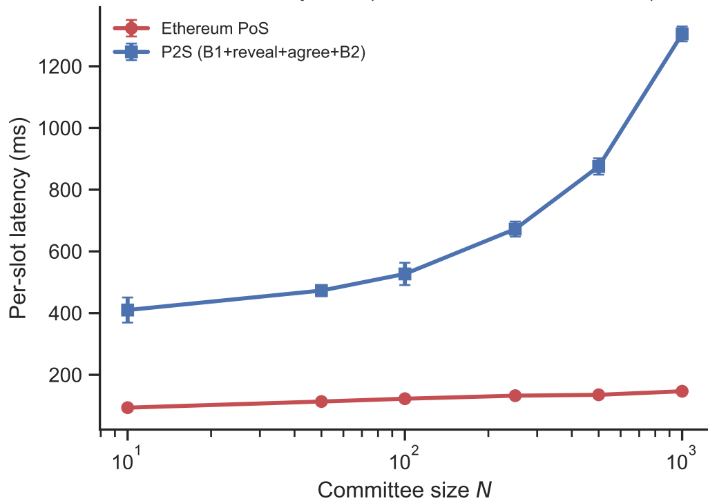
Network latency vs N (K=150 tx, 20 seeds, 95% CI)
