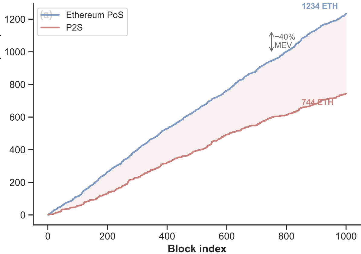
Cumulative MEV extracted (ETH)
