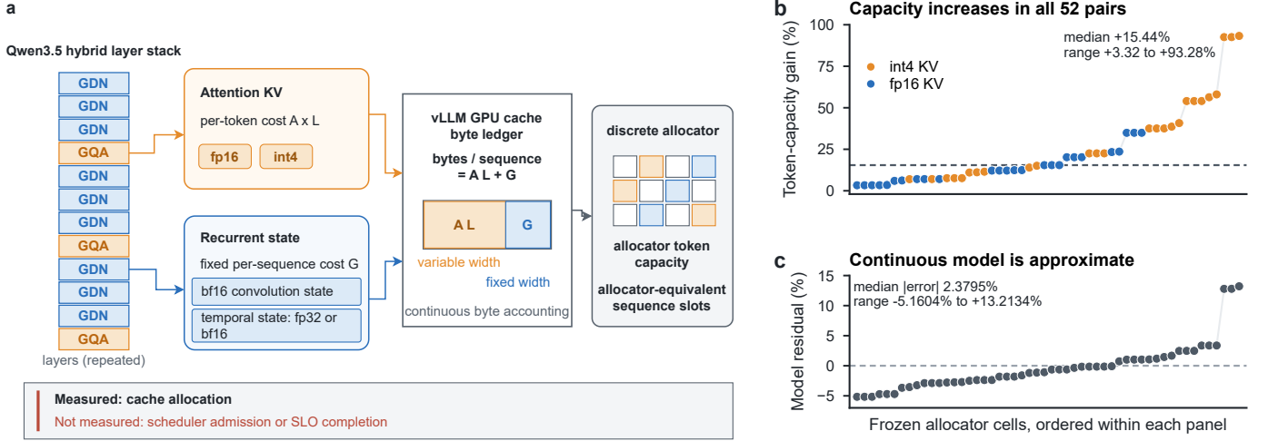
Fig. 2. From hybrid memory to measured allocator capacity. (a) GQA layers contribute per-token attention KV, while GDN layers contribute fixed recurrent state; both enter one GPU cache byte ledger before discrete allocation. The diagram explicitly separates measured cache allocation from unmeasured scheduler admission and SLO completion. (b) All 52 paired cells increase allocator token capacity under bf16 state. (c) The continuous model has mixed-sign approximation residuals and is neither a lower nor upper bound.
