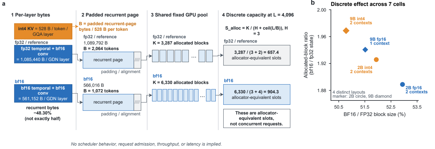
Fig. 1. Byte-to-page-to-block allocation. (a) Verified 2B/int4/4K worked example. The recurrent-page bytes and 528-byte int4 per-token cost determine attention block size; padding and integer block counts then determine allocator-equivalent slots. The 657.4 and 904.3 values are not concurrent requests. (b) Four distinct discrete layouts cover the seven fixed-utilization cells; marker area records whether one or two context lengths share the layout.
