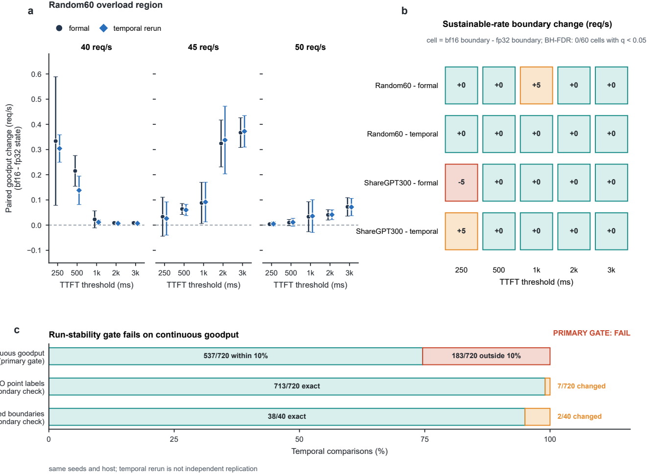
Fig. 5. Serving run-stability evidence. (a) Random60 paired goodput change in req/s for the formal run and temporal rerun. (b) Sustainable-rate boundary changes for Random60 and ShareGPT300. The rerun uses the same host, contracts, and seeds. None of 60 cellwise comparisons survives BH-FDR. (c) The four-configuration temporal audit fails its predeclared continuous- goodput gate: 183/720 comparisons exceed 10%. Exact binary SLO labels (713/720) do not override the failed primary endpoint.
