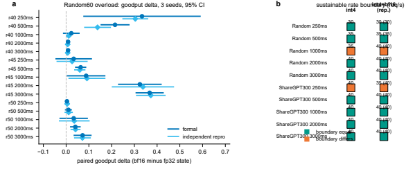
Figure 8. Serving, Random60 overload region . (a) Paired goodput delta (bf16 minus fp32 state) at rates 40–50 req/s, all thresholds, formal and second run, 3 seeds each, 95% CI. (b) Sustainable-rate boundary parity map (int4 vs. int4+bf16); orange cells differ between allocations, teal cells are equal, with the second-run value in parentheses.
