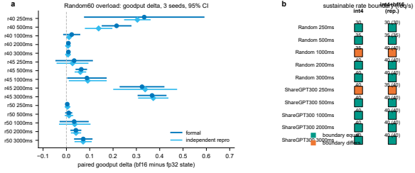
Figure 8. Serving, Random60 overload region . (a) Paired goodput delta (bf16 minus fp32 state) at rates 40–50 req/s, all thresholds, formal and independent reproduction, 3 seeds each, 95% CI. (b) Sustainable-rate boundary parity map (int4 vs. int4+bf16); orange cells differ between allocations, teal cells are equal, with the reproduction value in parentheses.
