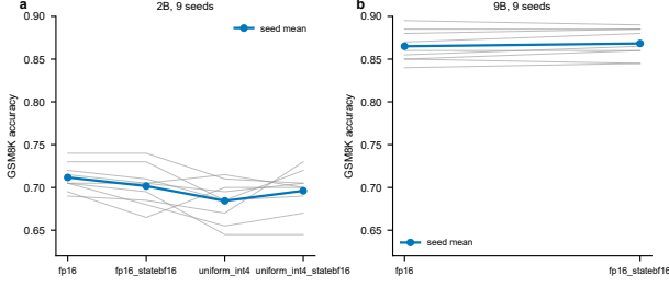
Figure 6. GSM8K per-seed paired accuracy . 200 seeded items, greedy, no chain-of-thought, 9 dataset seeds. Thin lines connect the same seed across allocations; the blue line and markers are seed means. (a) 2B across four allocations; (b) 9B across two.
