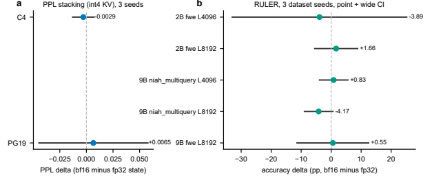
Figure 4. Perplexity stacking and RULER. (a) PPL marginal change of bf16 state under int4 KV (C4/PG19, 3 seeds). (b) RULER deltas (bf16 minus fp32 state) for the five previously nonzero cells; 3 dataset seeds, wide CIs, no detectable difference.
