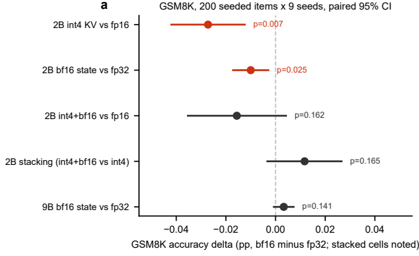
Figure 3. GSM8K paired deltas. 200 seeded items, greedy, no chain-of-thought, 9 dataset seeds; points and 95% paired CIs. Red intervals exclude zero. The 2B state and int4 regressions are significant; the 2B state effect is below the pre-registered MDE (1.16 pp) with 67.5% power.
