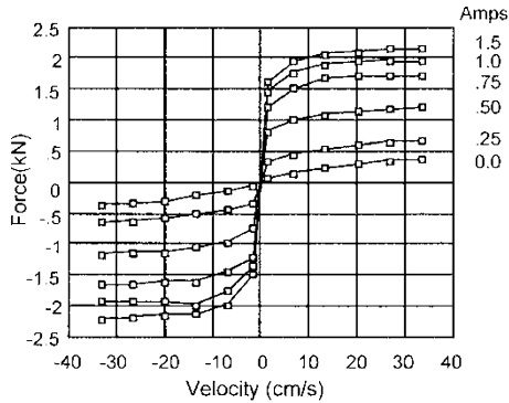
Figure 12-3. Performance curves for the linear MR damper 2
