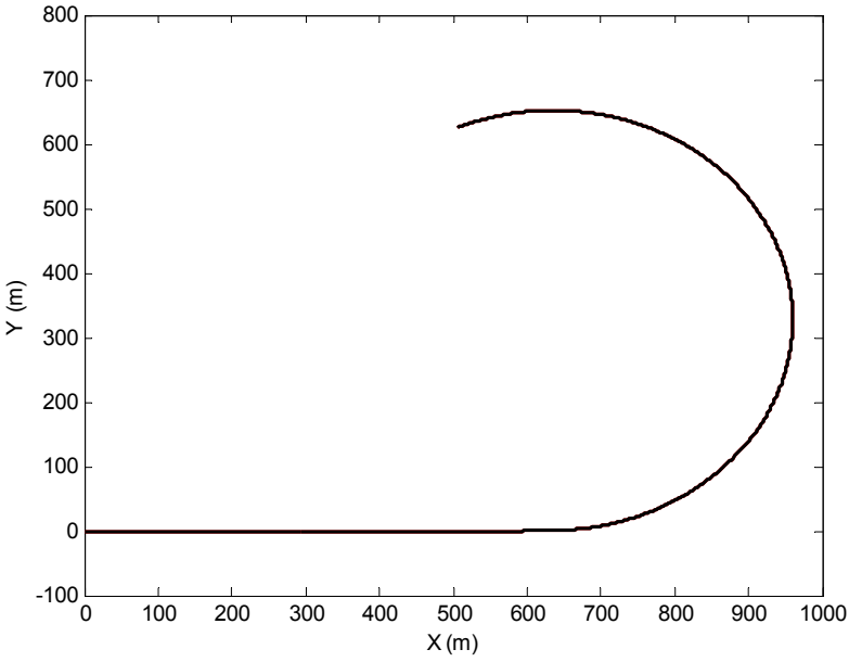
Figure 8-7. Vehicle trajectory for a step steering input
