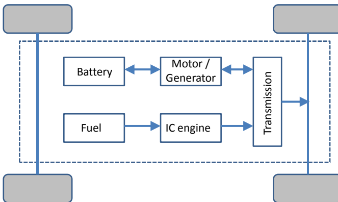
Figure 16-1. Schematic of powertrain for a parallel hybrid vehicle
