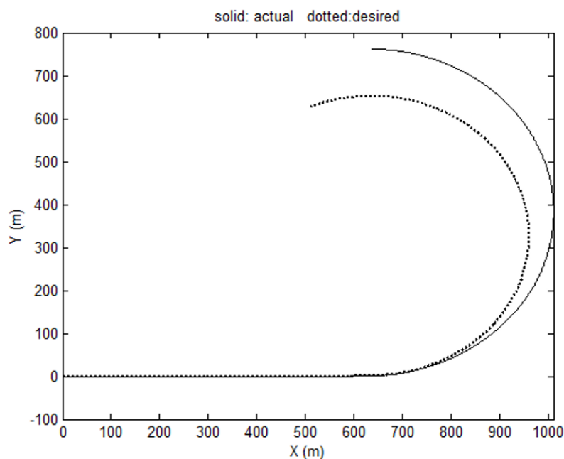
Figure 8-11. Trajectory with friction coefficient 0.6 and yaw rate + slip angle control
