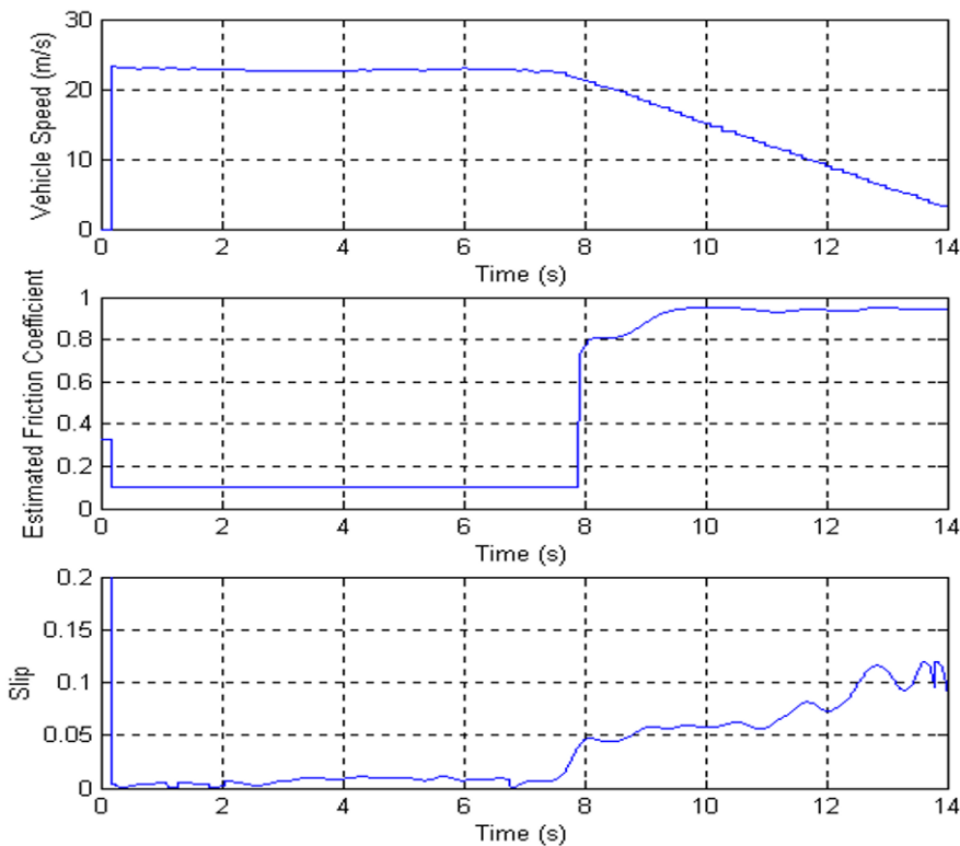
Figure 14-13. Test results for hard braking
