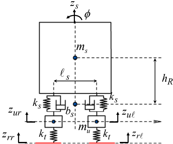
Figure 15-9. Four degree-of-freedom roll dynamics model
