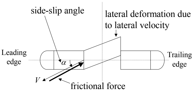
Figure 13-9. Lateral tire deflection and force generation
