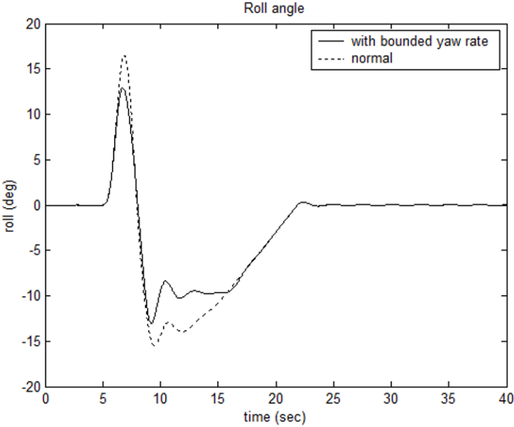
Figure 15-17. Roll angle – nominal and bounded yaw rate
