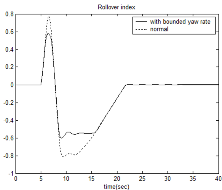
Figure 15-16. Rollover index – nominal and bounded yaw rate
