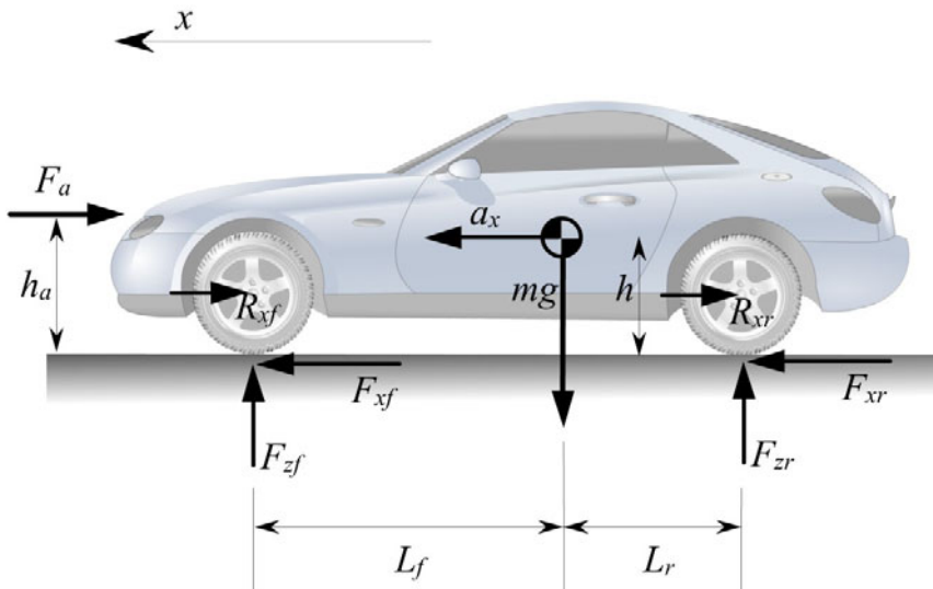
Figure 14-1. Vehicle longitudinal dynamics schematic diagram
