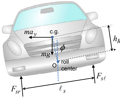
(b) Free body diagram for 1 dof roll model
