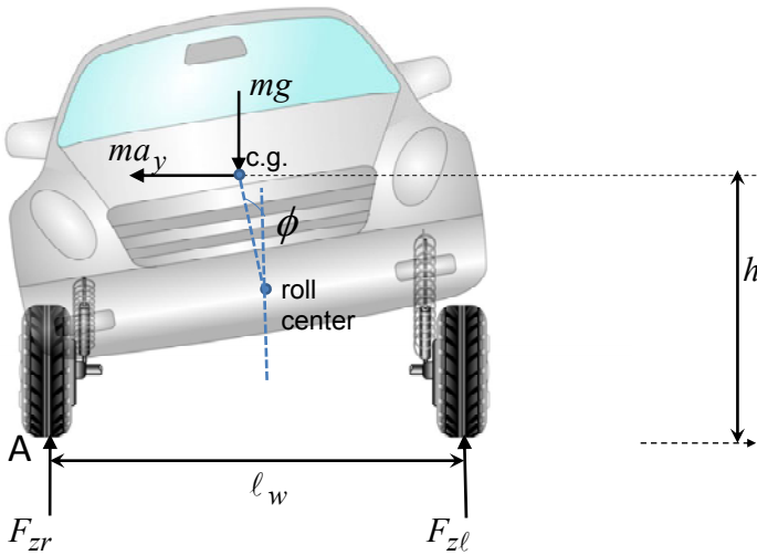
Figure 15-2. Roll moment balance in steady state cornering
