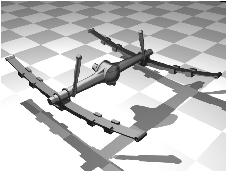
Figure 10-4. Solid-axle leaf-spring rear suspension 1
