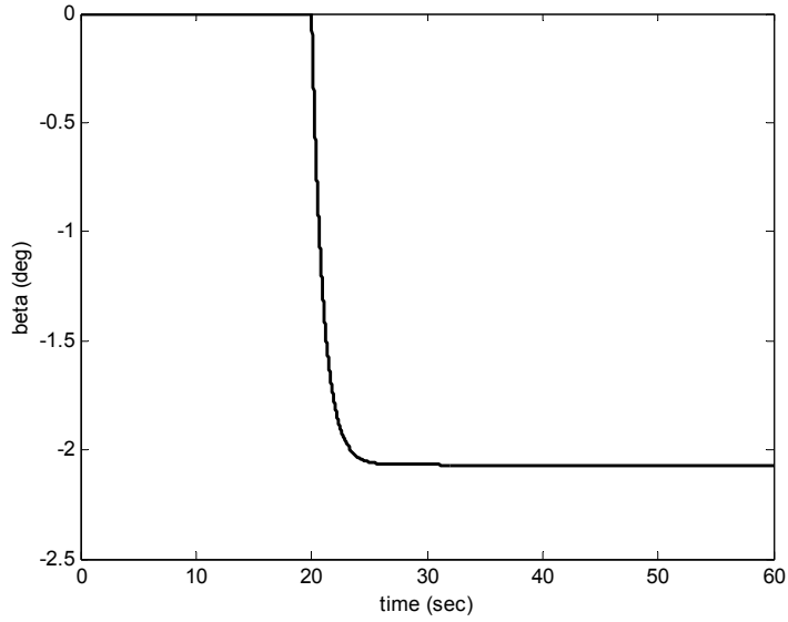
Figure 8-8. Slip angle on a dry road with a friction coefficient of 1.0
