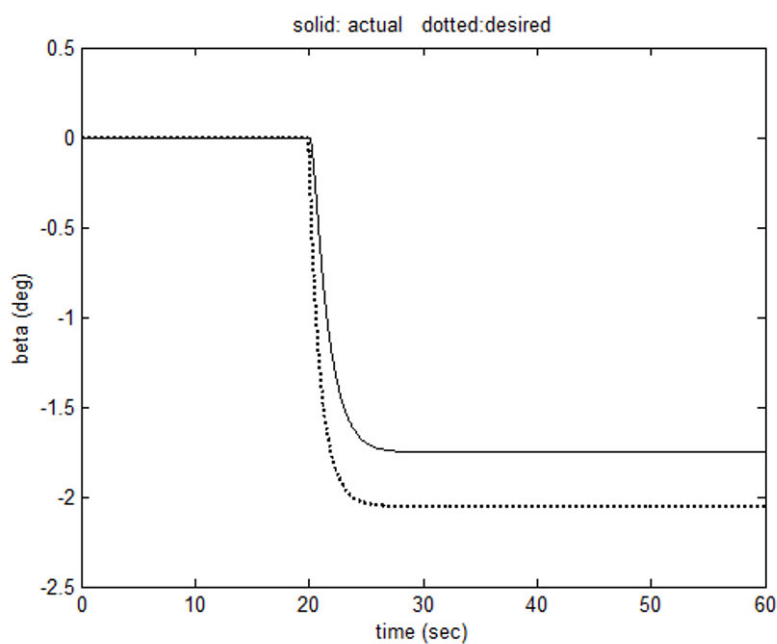
Figure 8-14. Slip angle with controller 1
