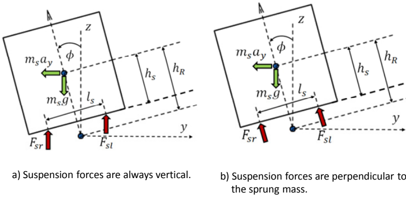
Figure 15-7. Different directions for suspension forces
