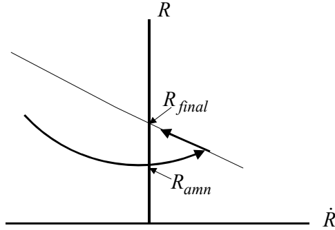
Figure 6-13. Parabolic trajectory during constant deceleration
