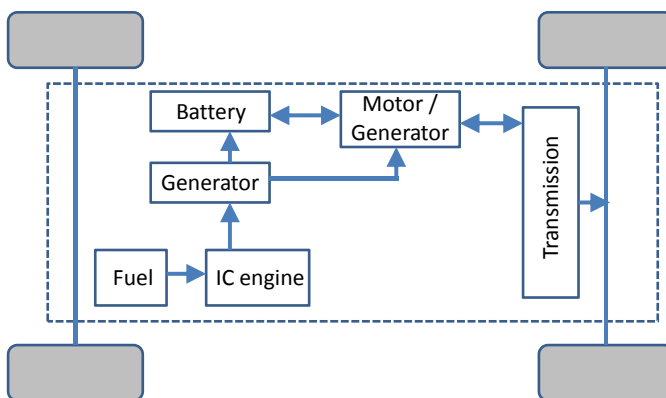
Figure 16-2. Schematic of powertrain for a series hybrid vehicle
