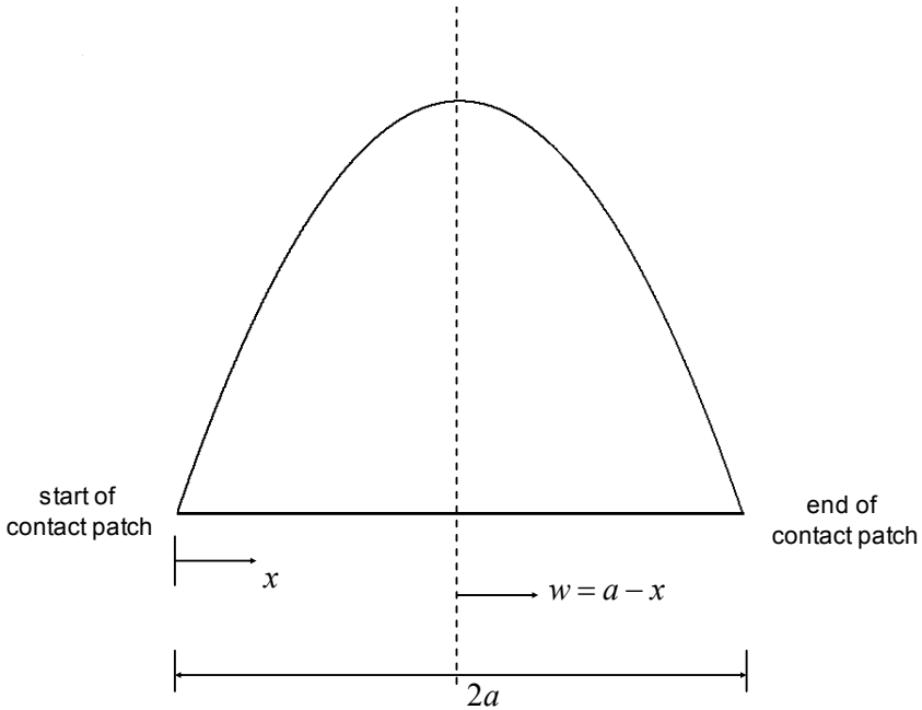
Figure 13-14. Parabolic normal pressure distribution on contact patch
