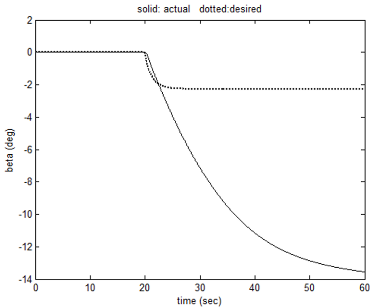
Figure 8-10. Slip angle with yaw rate control only
