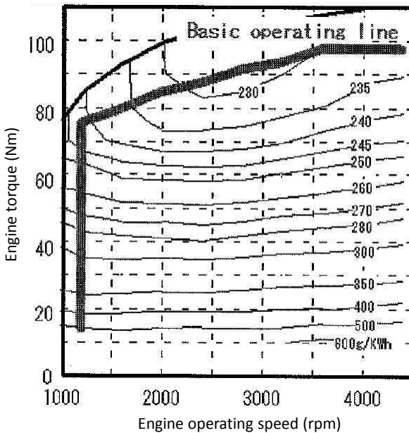
Figure 16-5. Engine map for the 1.5L engine in the THS-II powertrain system (Meisel, 2006) 1
