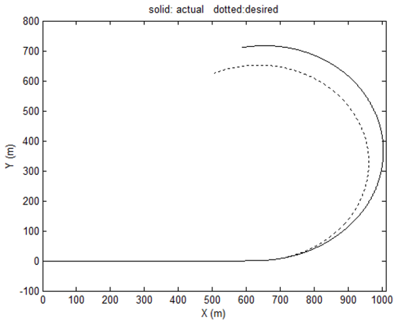
Figure 8-9. Vehicle trajectory on a road with friction coefficient of 0.6 and yaw rate control
