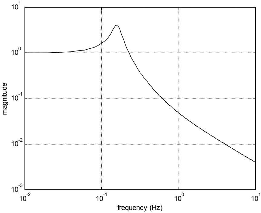
Figure 7-4. Magnitude of G(s) from Eqn. (7.32)
