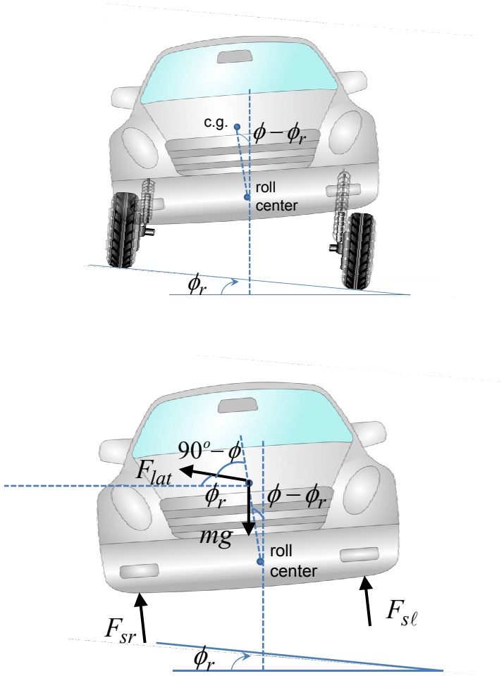
Figure 15-8. Roll dynamics and free body diagram
