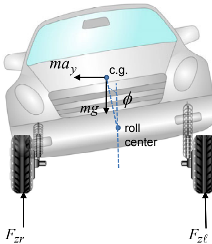
Figure 15-11. Rollover index using lateral load transfer
