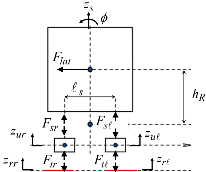
Figure 15-10. Four degree-of-freedom model with suspension and tire dynamic forces
