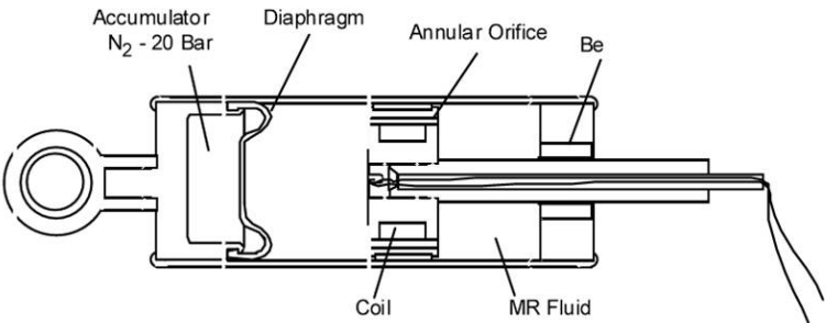
Figure 12-2. Commercial Linear MR Fluid-based Damper 1
