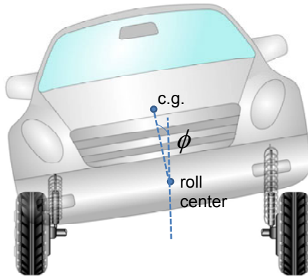
(a) Schematic for vehicle roll dynamics, 1 dof model
