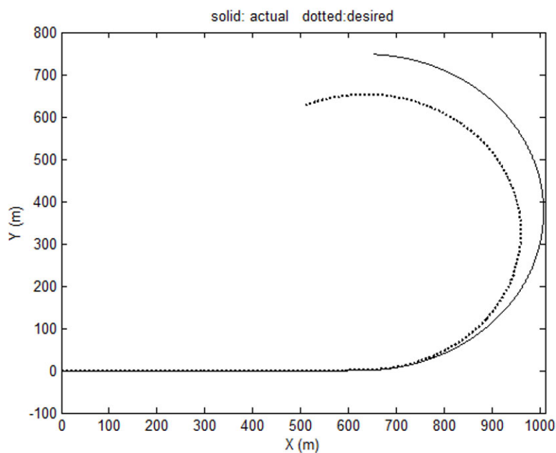
Figure 8-13. Vehicle trajectory with controller 1 on a road with friction coefficient 0.8
