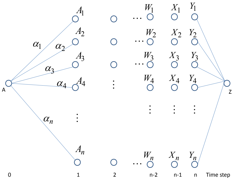
Figure 16-7. Dynamic programming for hybrid vehicle control system design
