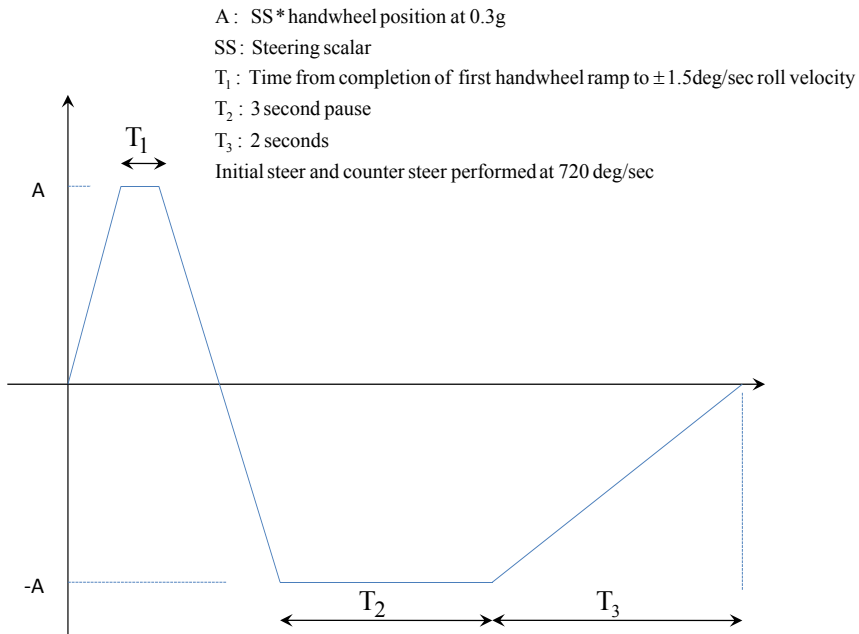
Figure 15-4. NHSTA fishhook maneuver
