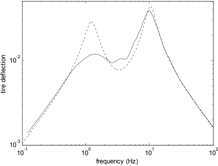
Figure 12-13. Tire deflection transfer functions for a performance index with moderate weights
