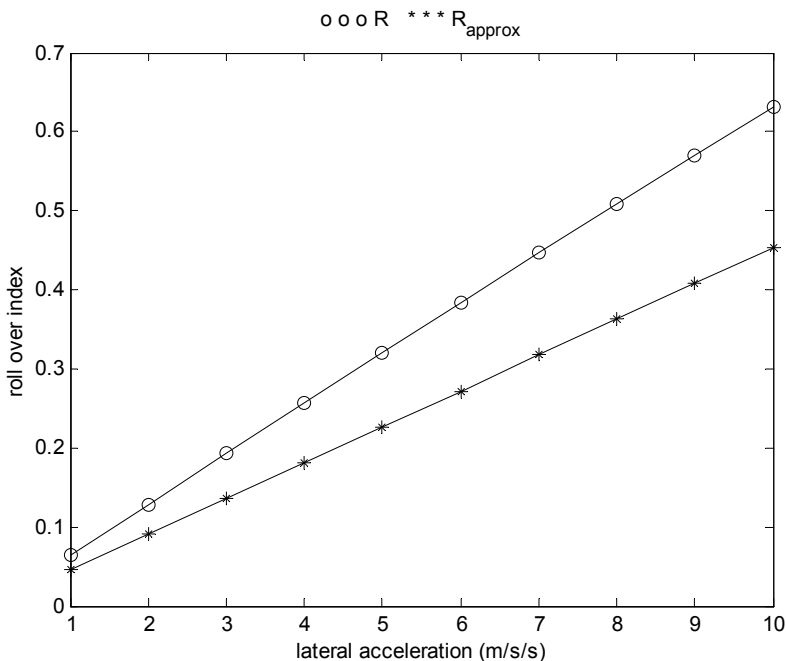
Figure 15-12. Rollover indices R and R_{approx} as a function of lateral acceleration
