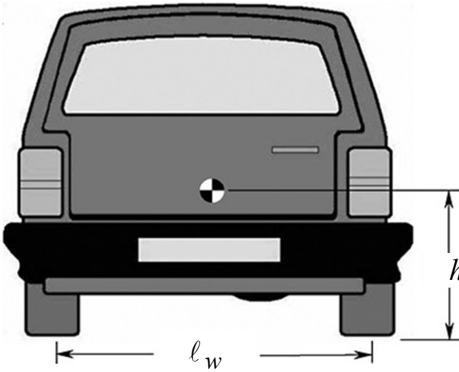
Figure 15-1. Parameters for vehicle static stability factor (TRB, 2002)
