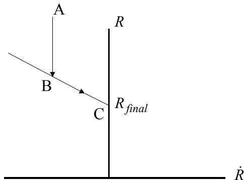
Figure 6-12. Switching line for spacing control
