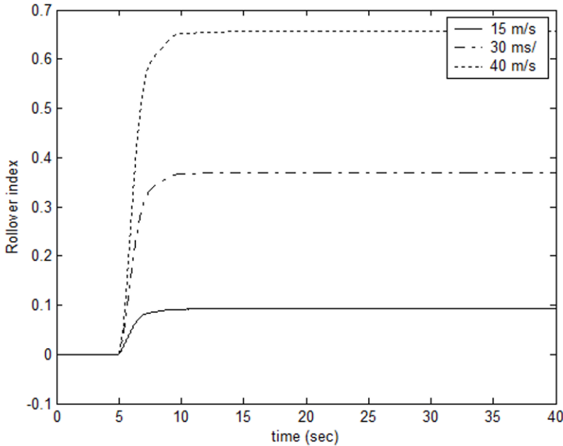
Figure 15-14. Rollover index at different speeds
