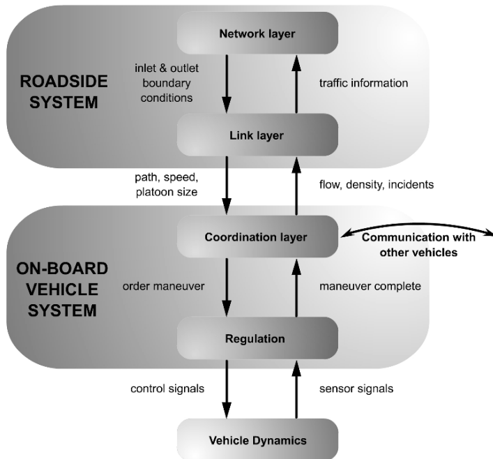
Figure 7-1. Control Architecture
