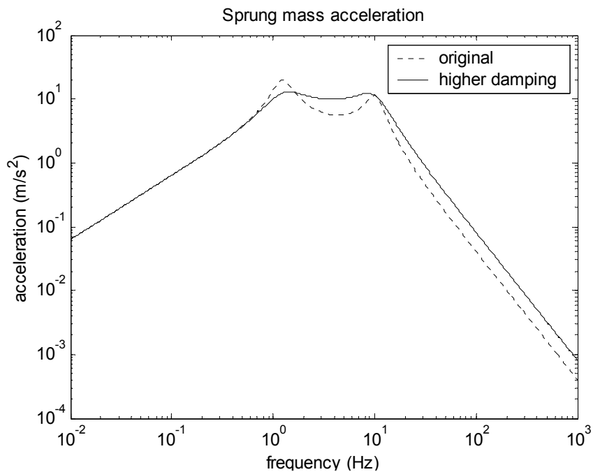
Figure 10-13. |H_A(j\omega)| with increased suspension damping
