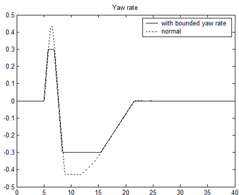
Figure 15-15. Yaw rate – nominal and bounded
