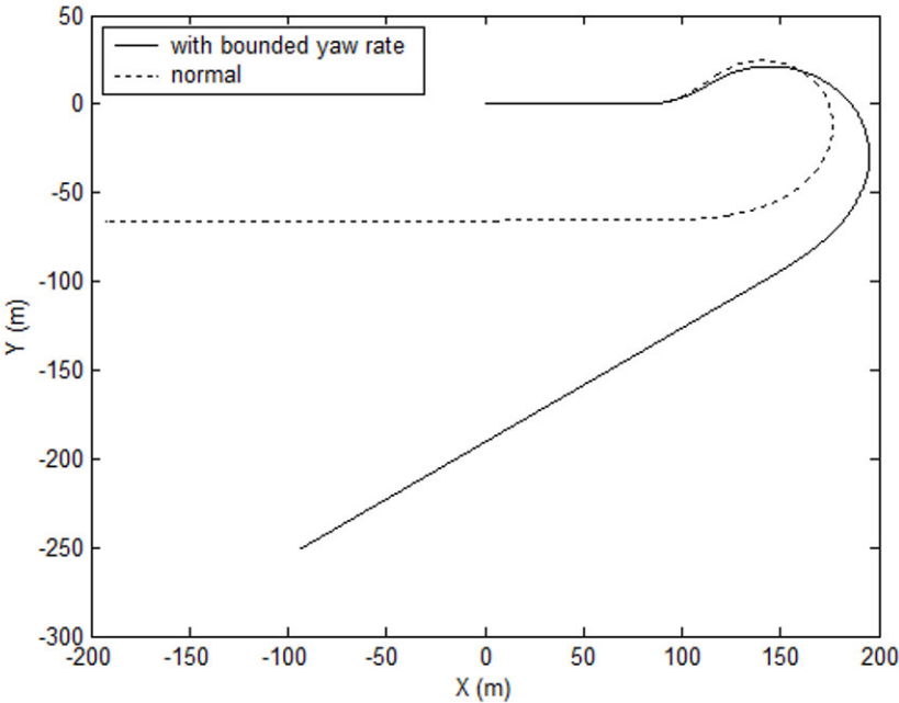
Figure 15-18. Vehicle trajectory - nominal and bounded yaw rate
