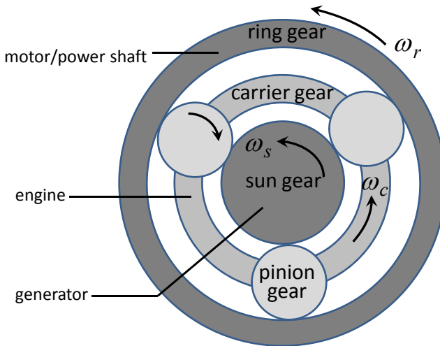
Figure 16-4. Planetary gear based power split system
