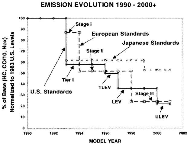
Figure 1-3. European, Japanese and US emission requirements 1
