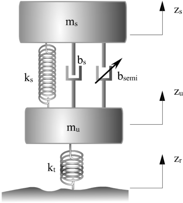
Figure 12-4. Quarter car semi-active automotive suspension
