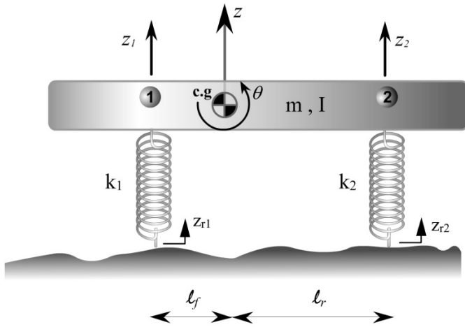
Figure 10-19. Two-degree of freedom half car model
