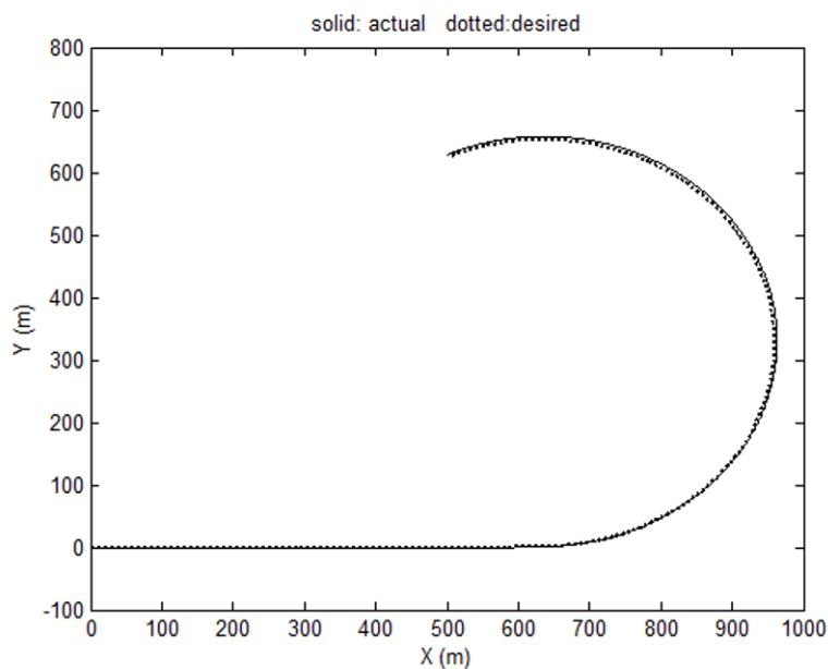
Figure 8-15. Vehicle trajectory with controller 2 on a road with friction coefficient 0.8
