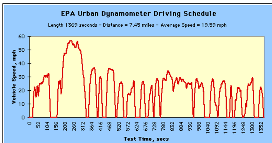
Figure 16-8. EPA Urban Driving Cycle (EPA, 2011)
