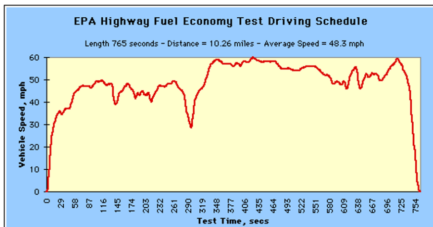
Figure 16-9. EPA Highway Driving Cycle (EPA, 2011)
