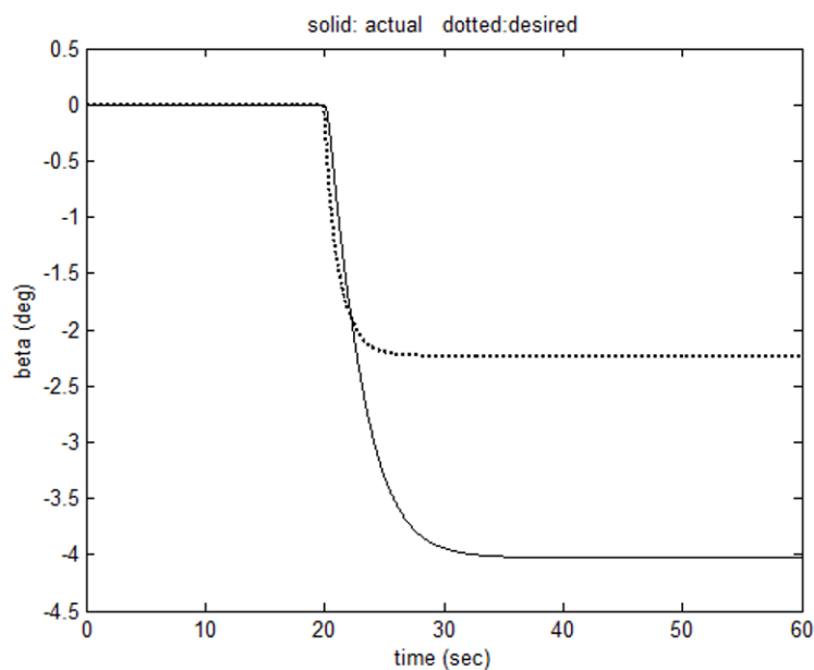
Figure 8-12. Slip angle with friction coefficient 0.6 and yaw rate + slip angle control
