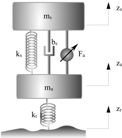
Figure 10-3. Quarter-car active automotive suspension
