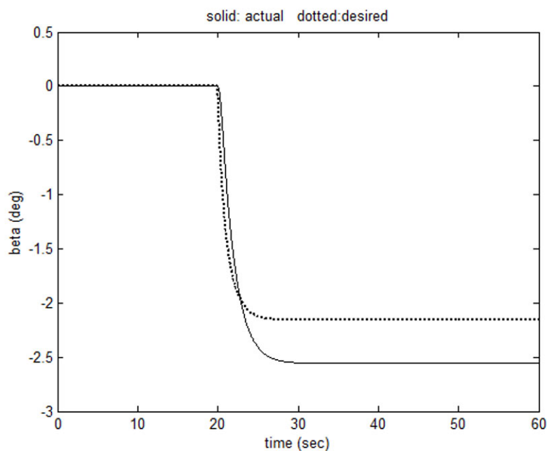
Figure 8-16. Slip angle with controller 2
