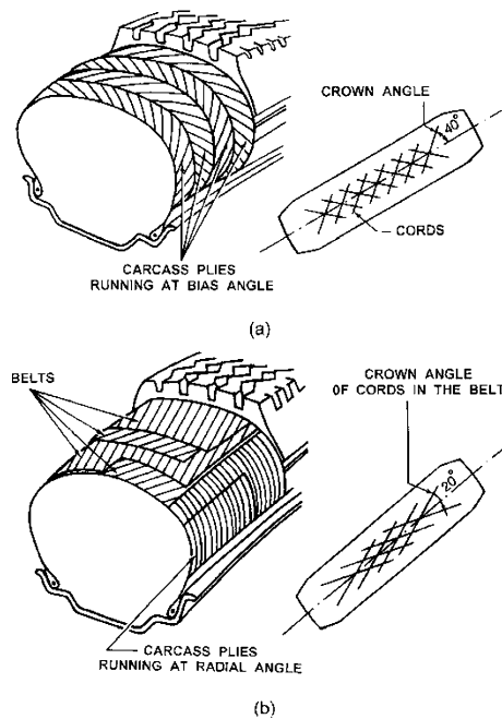
Figure 13-4. Tire construction: a) Bias-ply tire and b) Radial-ply tire 1
