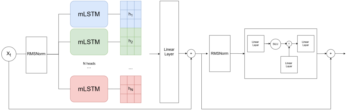
Figure 3: mLSTM Block
