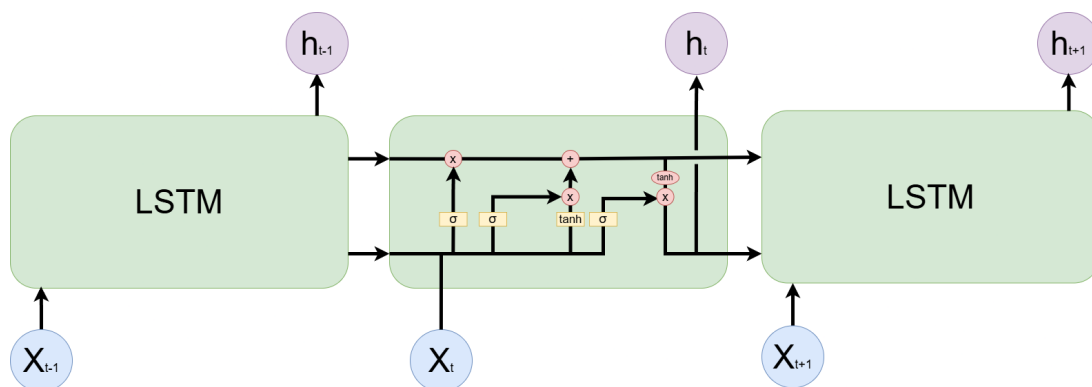
Figure 2: The LSTM cell, figure inspired by [19]
