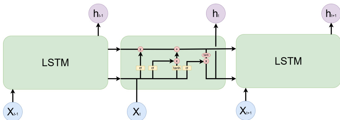
Figure 2: The LSTM cell, figure inspired by [19]
