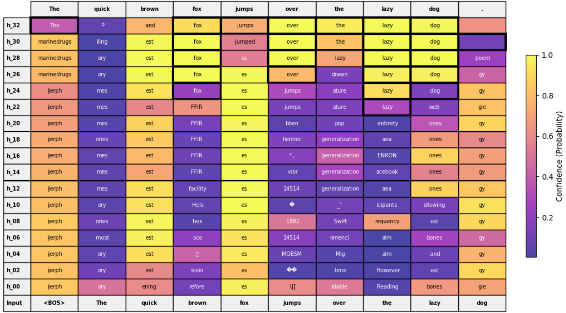
Figure 5: Top token prediction per hidden state
