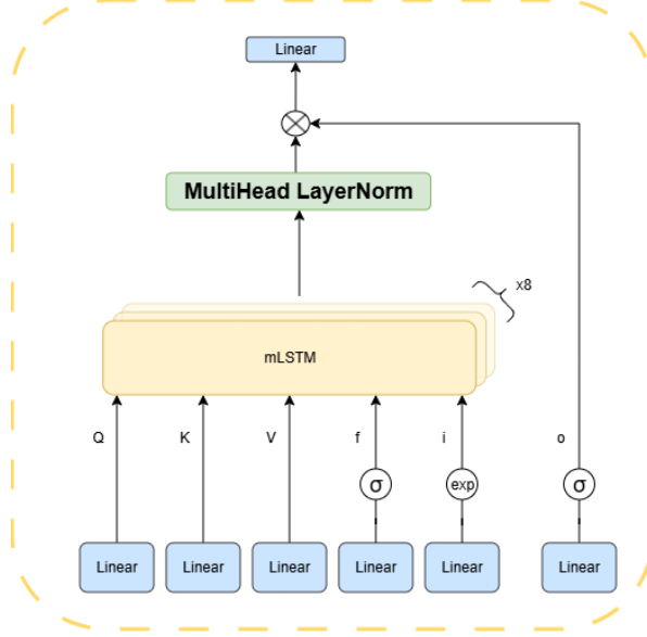
Figure 3: mLSTM layer - used in the xLSTM model. Adaptation after [26]
