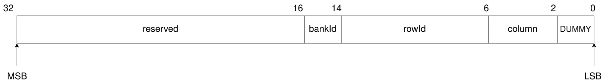
Address Translation
