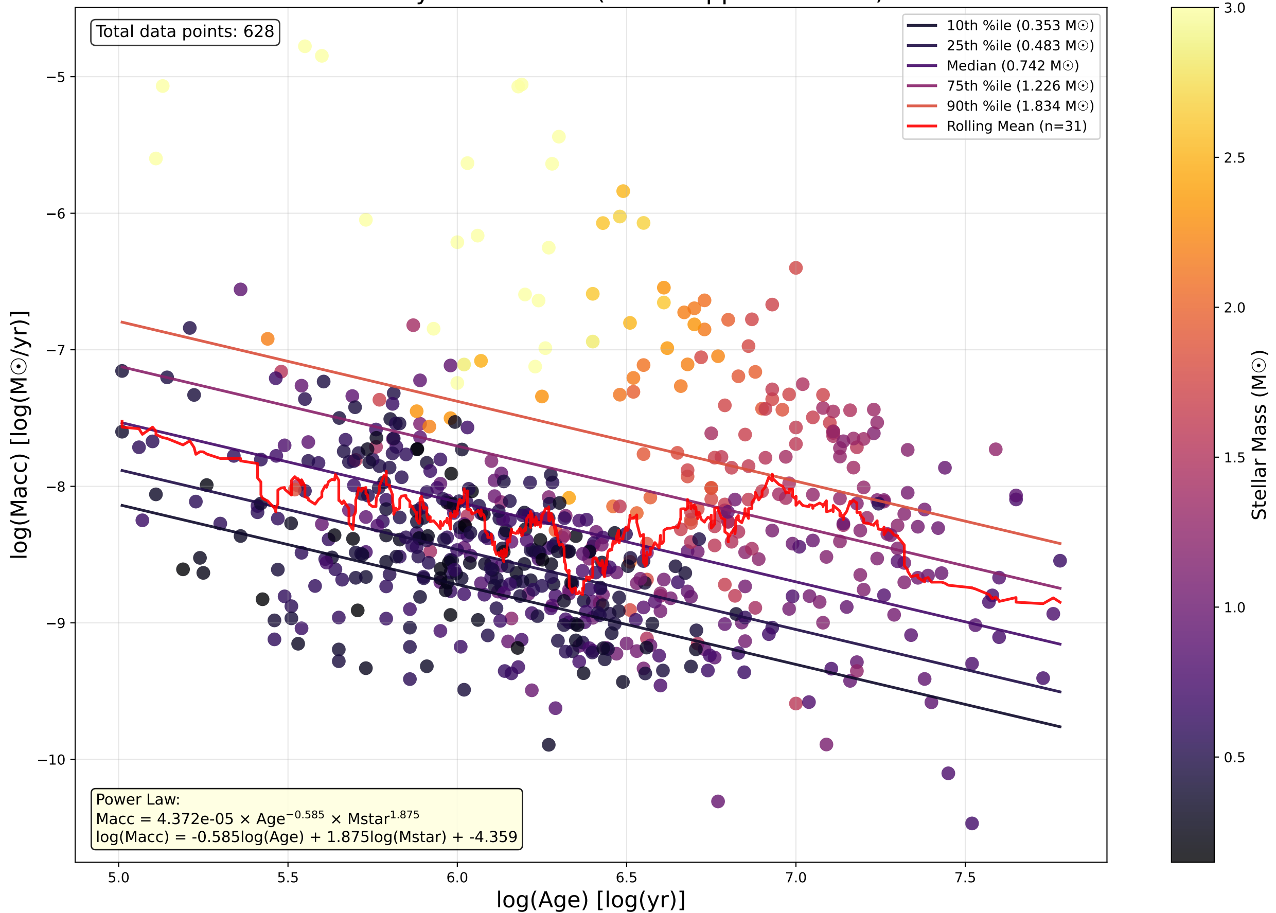
Mass Accretion Rate vs Age: Triple Power Law Fit Colored by Stellar Mass (scale capped at 3 M \odot )
