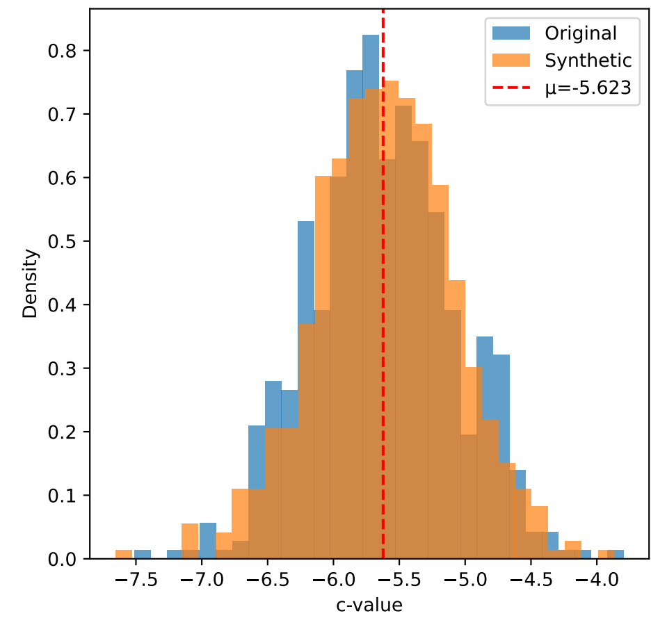
c-value Distribution
