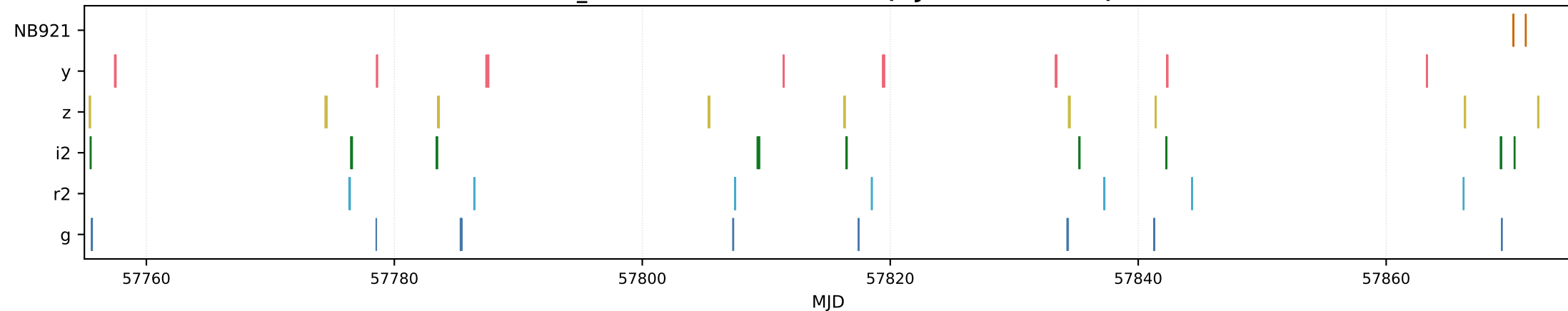
cid_42 — 2017 dense season (MJD 57755-57875)
