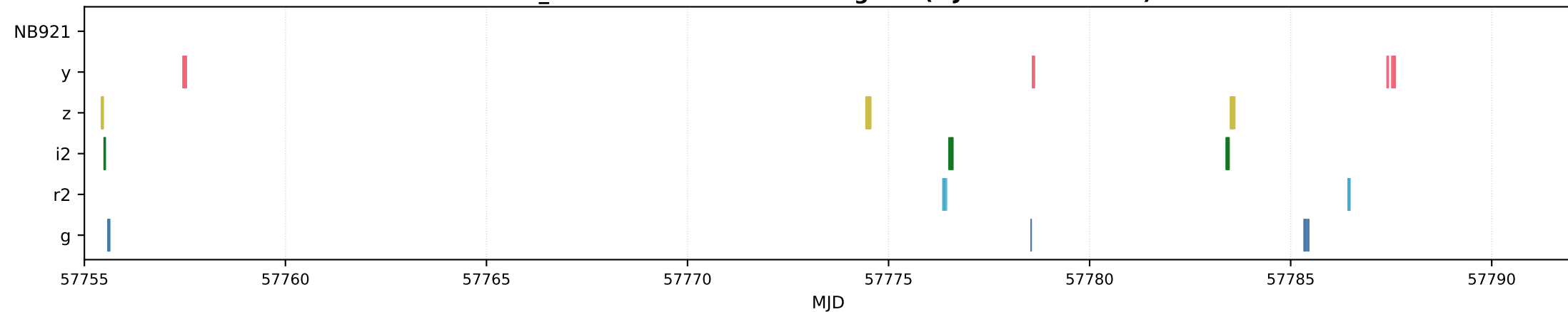
cid_42 — Zoom: first observing run (MJD 57755-57792)
