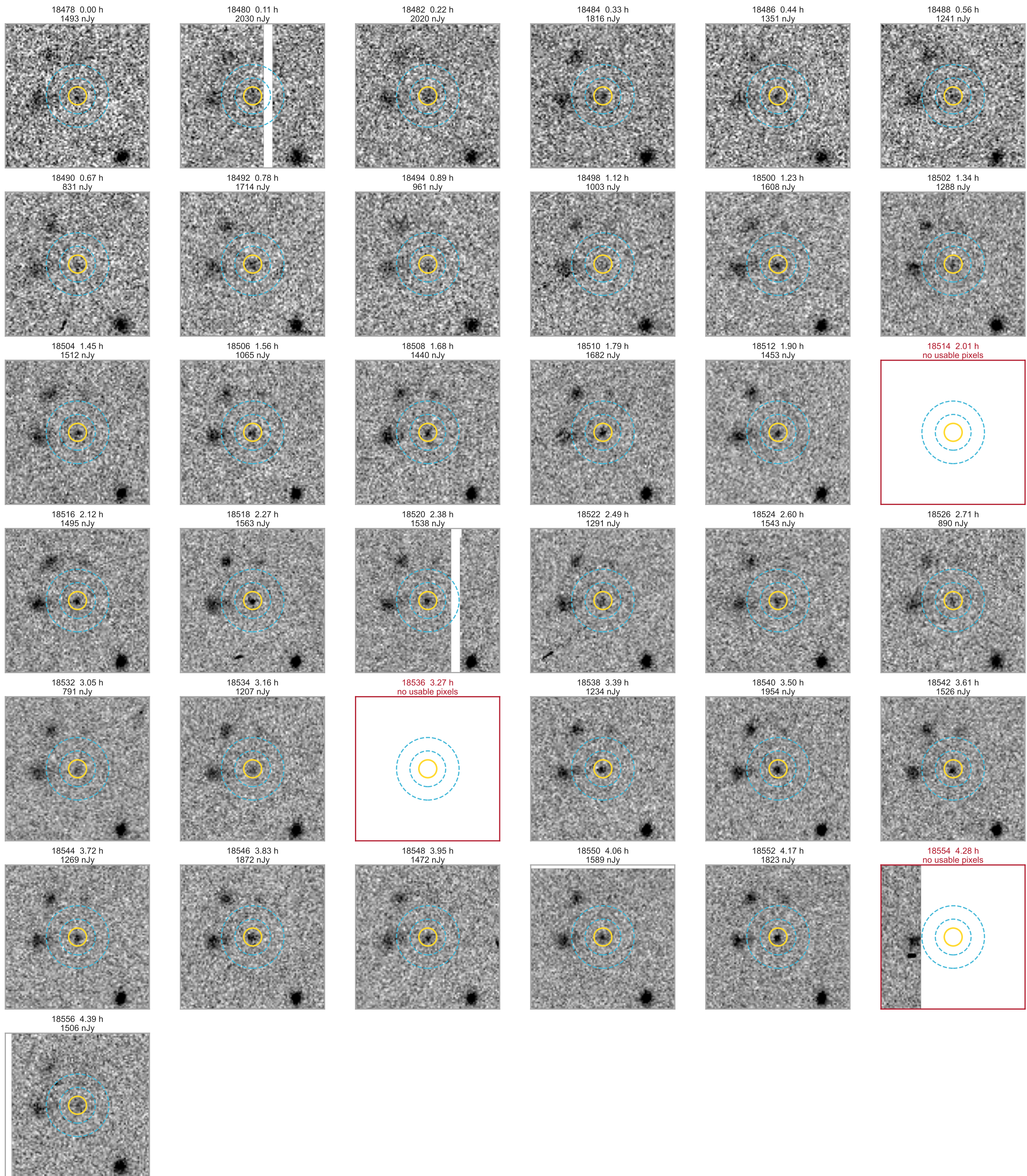
cid_1205 y warp stamps, MJD 57040: r=1.0 arcsec aperture, 2.0-3.5 arcsec sky annulus
