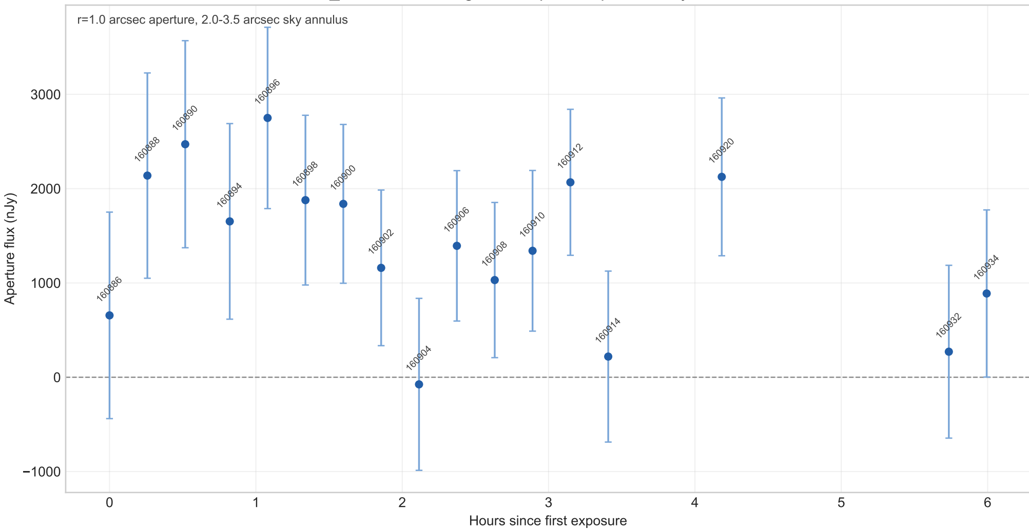
cid_1205 N1010 single-visit aperture photometry, MJD 58488
