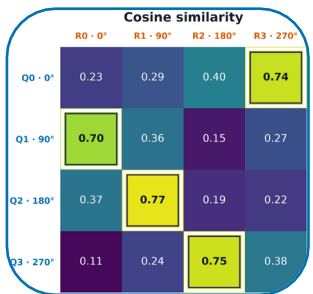
Cyclic SALAD Similarity
