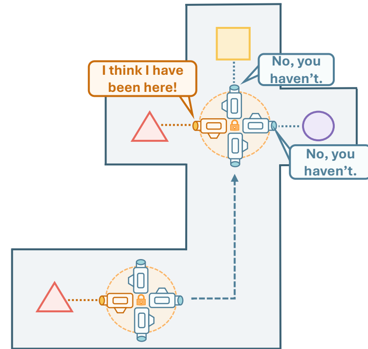
Cyclic Retrieval
