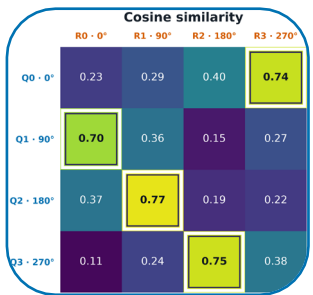
Cyclic SALAD Similarity
