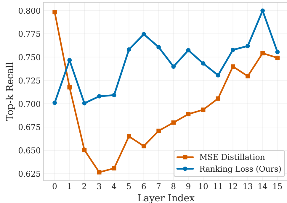
3.2 Layer-wise Recall Comparison
