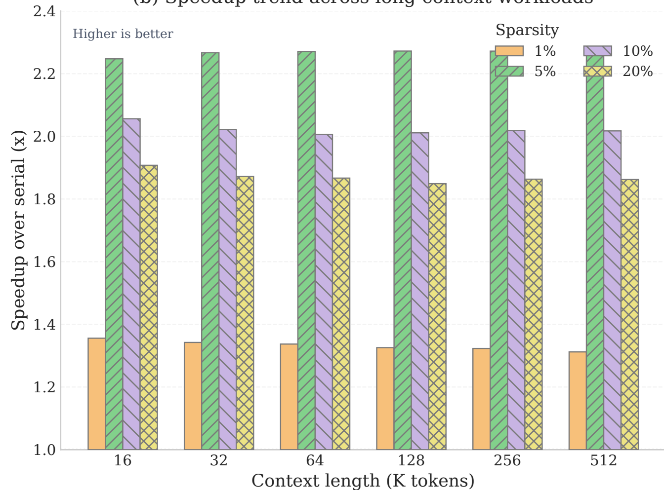
(b) Speedup trend across long-context workloads
