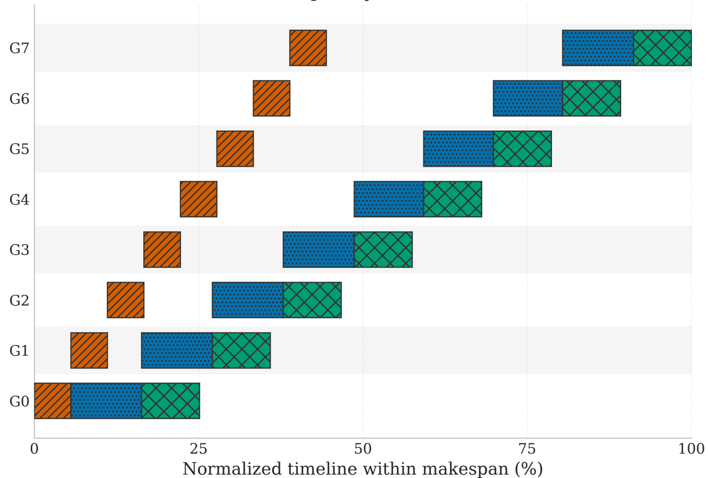
(a) Representative pipeline Gantt chart (64K tokens, 10% sparsity, fixed 16-channel DDR)
