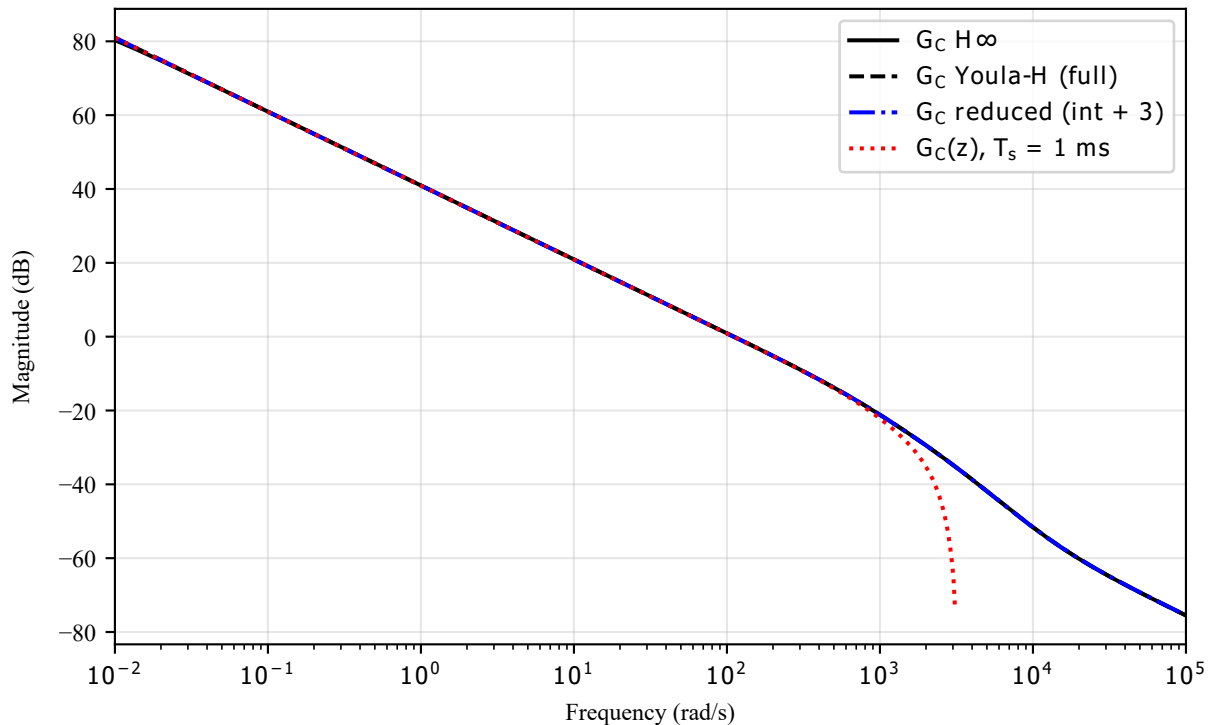
Controller magnitude: H_\infty vs Youla-H (pure integrator at DC)
