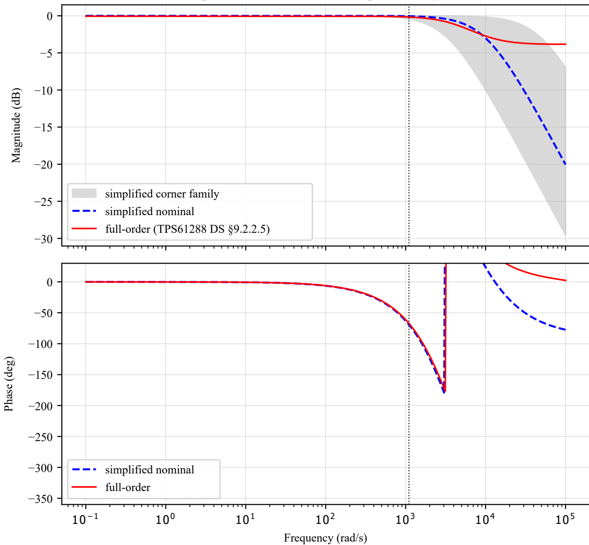
Share plant r \rightarrow \alpha : full-order vs simplified design model
