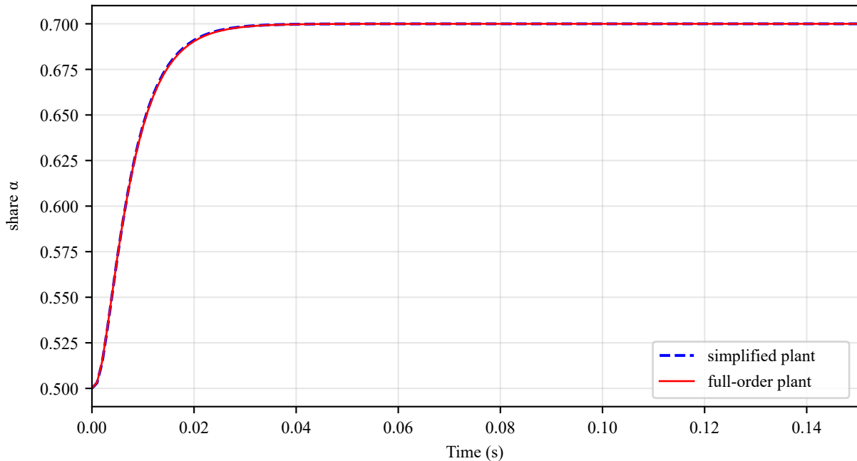
Closed loop with the shipped controller: step 0.5 \rightarrow 0.7
