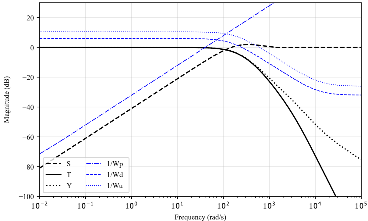
Youla-H closed-loop shapes — droop power-share loop
