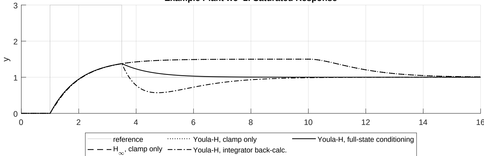
Example Plant \omega_c=1 : Saturated Response
