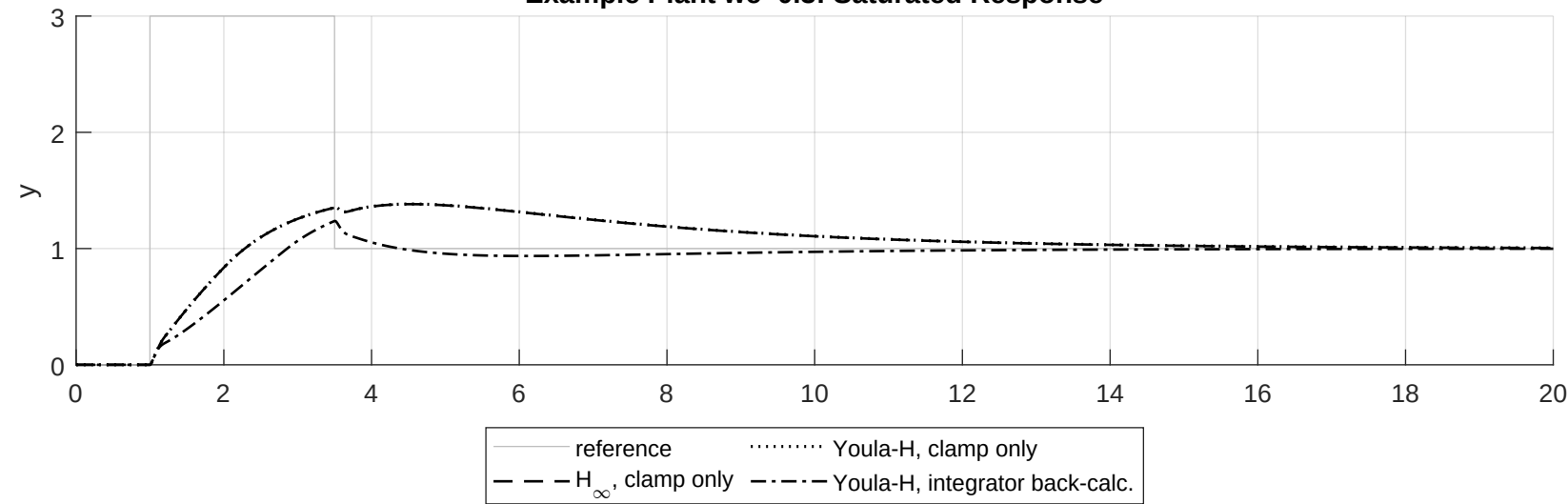
Example Plant w_c=0.3 : Saturated Response
